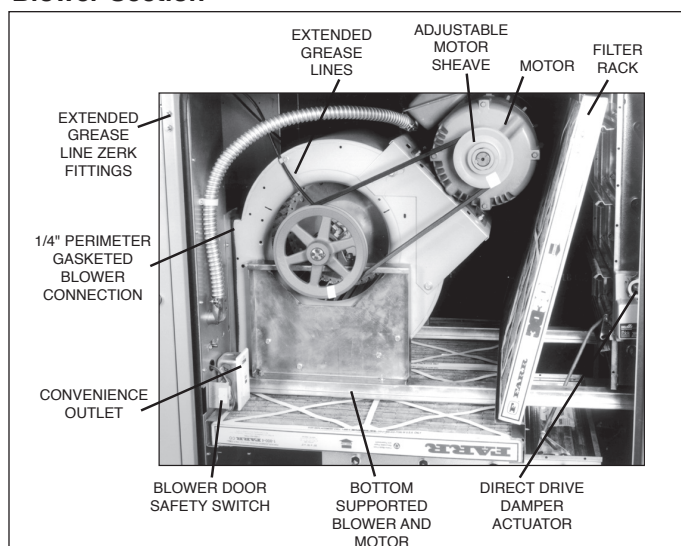
Figure 26.4 Blower Section
