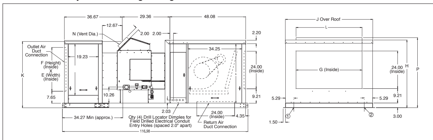
Figure 46.2 DCG Indoor Gravity Vented Cooling Package Unit Dimensions
