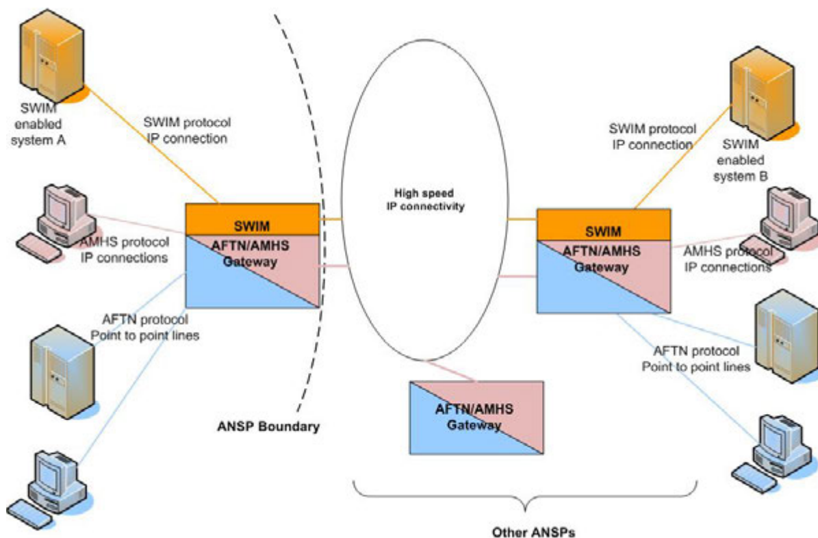
Figure 14. Interoperability ensured in the gateway
