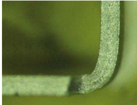
Fig 12. Smooth bending
