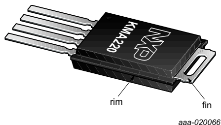
Fig 8. Reading point alignment features
