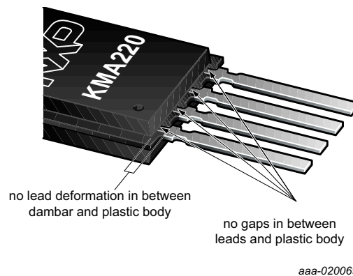
Fig 14. Lead entrance to body check
