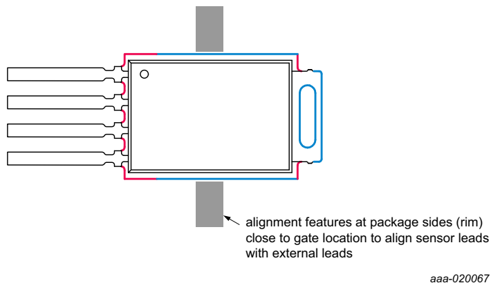
Fig 9. Align pins to external leads at lower body
