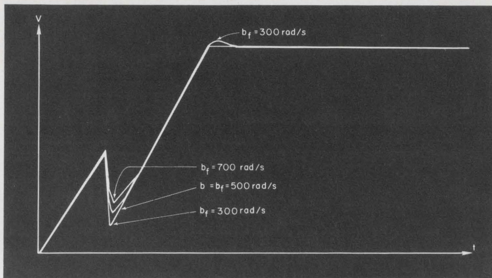
4. Inaccuracy in the high-frequency breakpoint causes errors in sharp corners in the filter output. The deviation from the correct curve is exaggerated to show the effect.
