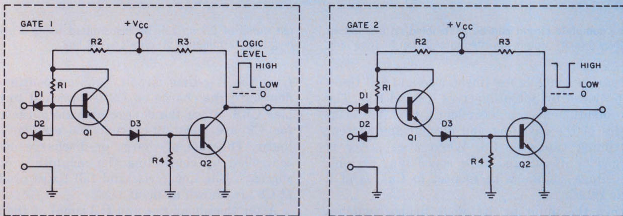
A typical DTL interface between two gating circuits.
