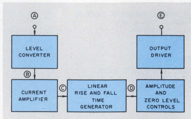
1. Circuit functions performed by the pulse shaper and driver are as shown. Various points are labeled to correspond to the waveshapes shown in Fig. 2.
