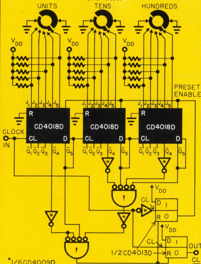
3-DECADE PROGRAMMABLE DIVIDE-BY-"N" COUNTER (N=2 TO 999)
