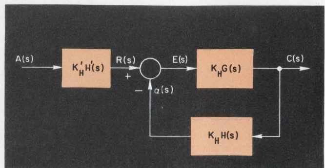
1. The distortion in signal R(s) is corrected by the inverse filter at the right. The feedback transfer function of the filter is a replica of the transducer's.
