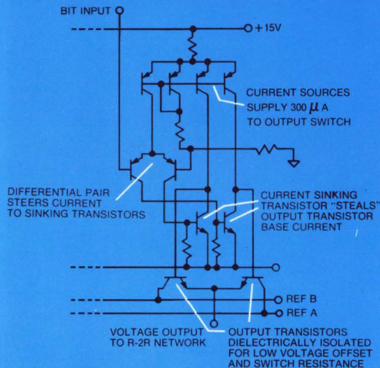
SINGLE SWITCH CELL OF 4 SWITCH QUAD
