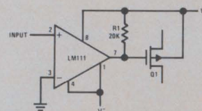
a. Zero Crossing Detector Driving Analog Switch
