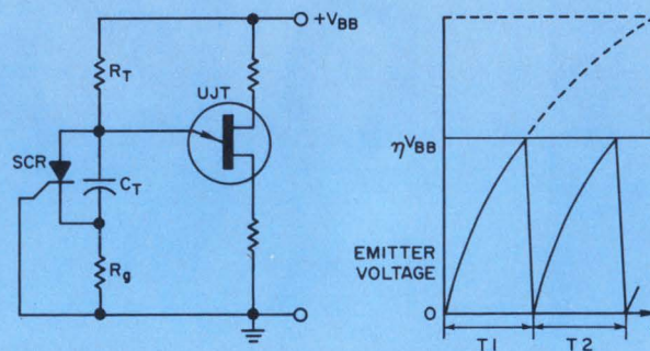
2. Improved UJT oscillator uses an SCR to completely discharge C_T during every cycle. All periods are now of equal duration.
