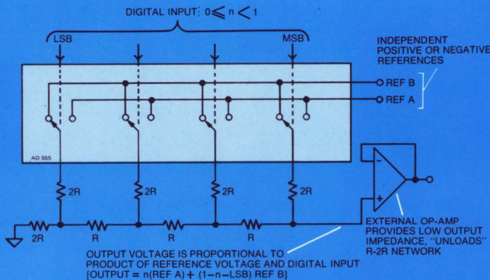
EQUIVALENT CIRCUIT AD555 QUAD SWITCH
