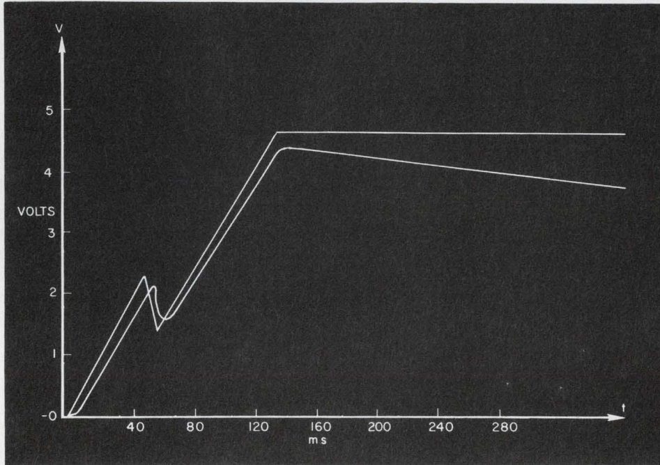
2. A simulated signal of a horizon profile is distorted by its transducer and telemetry (lower curve). The restored waveform is indistinguishable from the original signal (upper curve).
