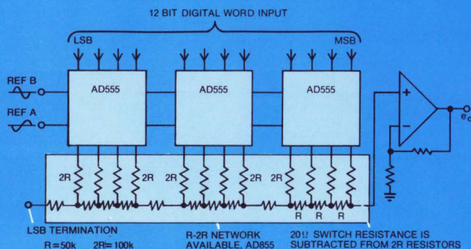
12-BIT MULTIPLYING D/A CONVERTER
