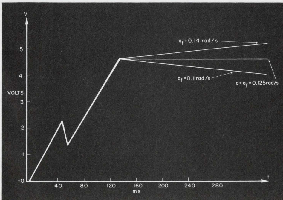
3. Incorrect choice of low-frequency breakpoint in the filter has this effect on signal restoration: The top curve shows the error resulting from too high and the bottom curve from too low a choice. The correct curve is in the center.
