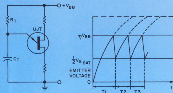
1. Basic UJT oscillator never fully discharges timing capacitor C_T during each cycle. This allows the first period after turn-on to be longer than all others.
