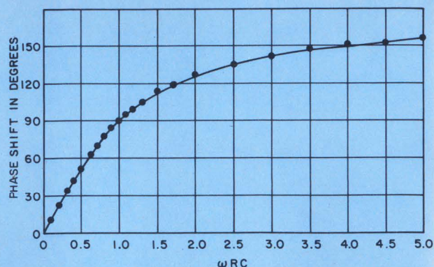
2. Linear phase shift exists over the first 60° of phase adjustment. A wideband transformer allows operation from 1 MHz to 100 MHz.
