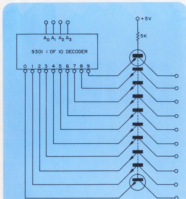
Common base buffer provides an output interface for the one-of-ten decoder.
