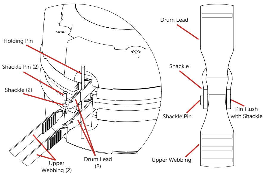
Drum Lead Diagram
