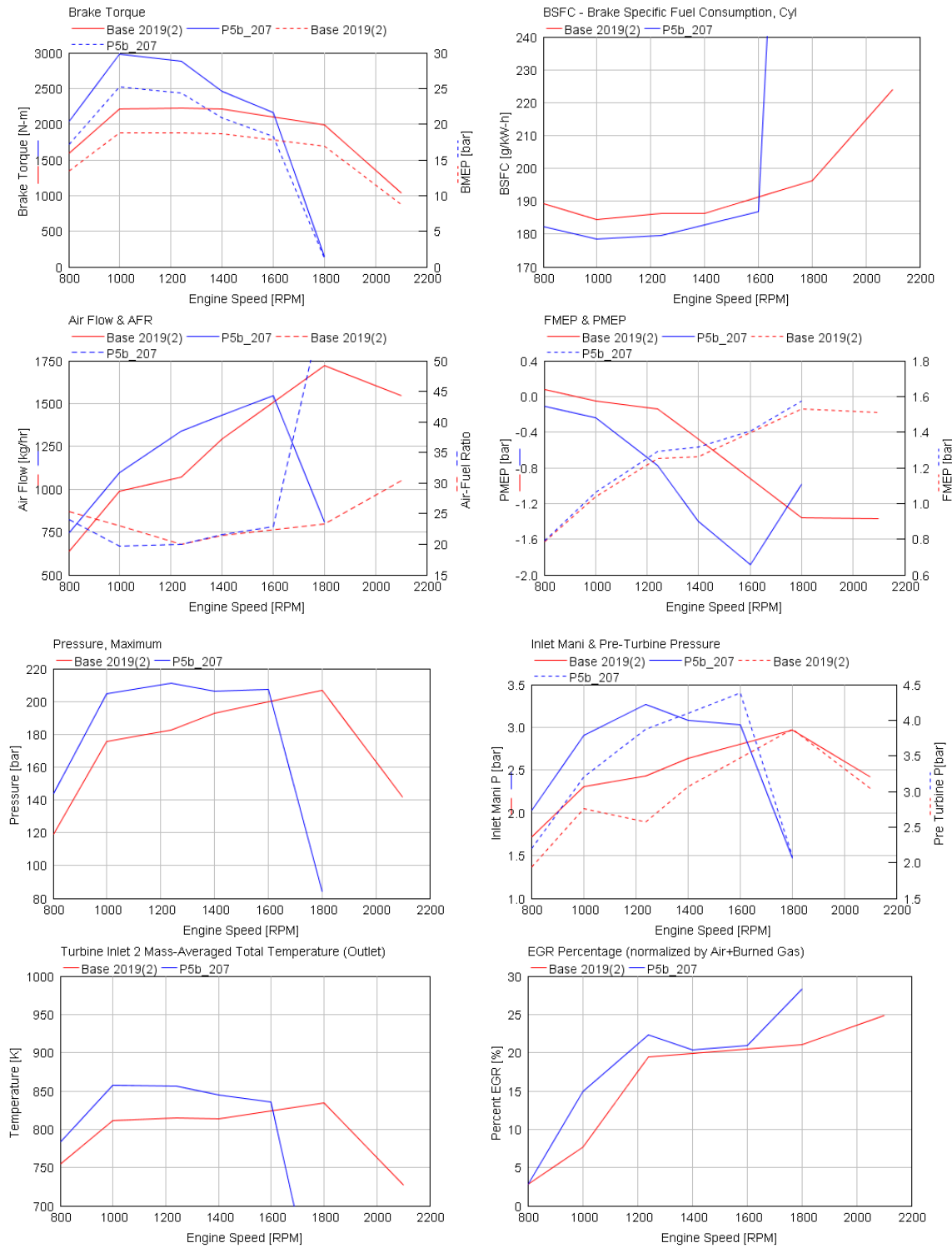
FIGURE B1.6C FULL LOAD PERFORMANCE COMPARISON
