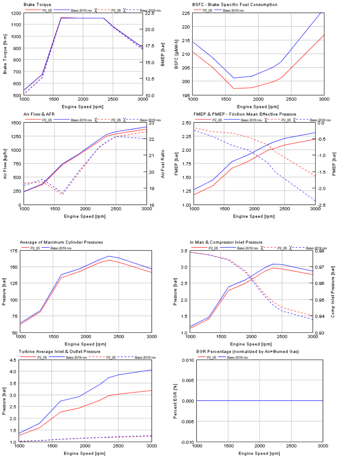
FIGURE B3.3C PACKAGE 12 FULL LOAD PERFORMANCE COMPARISON
