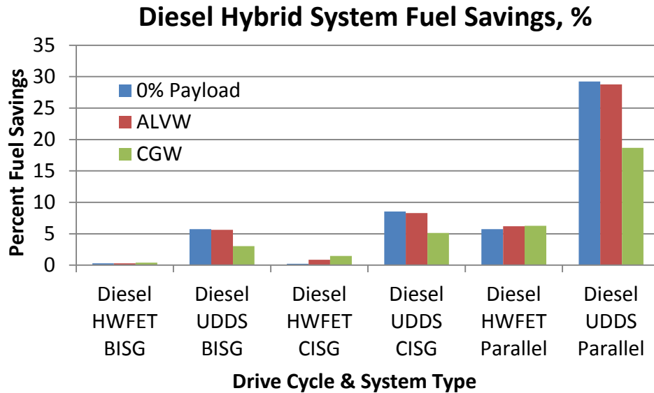
FIGURE D.2 DIESEL HYBRID SYSTEM FUEL CONSUMPTION REDUCTION IN PERCENT
