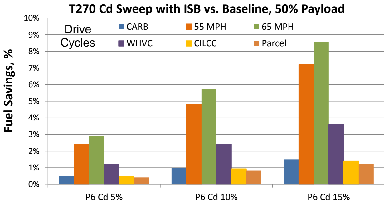
FIGURE 3.2 CD SWEEP OF T270 DELIVERY TRUCK
