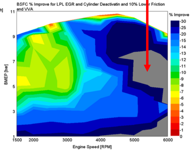
FIGURE A12 BSFC IMPROVEMENT OVER BASELINE
