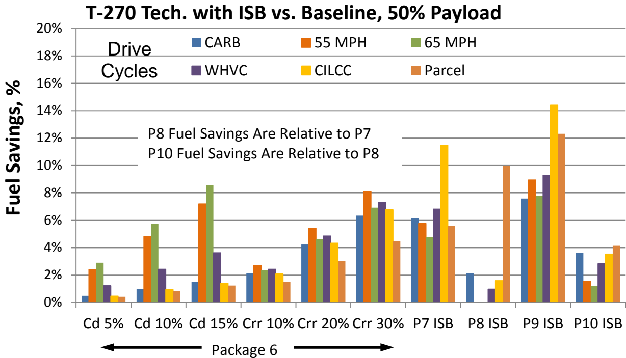
FIGURE 2.15 T270 VEHICLE TECHNOLOGY COMBINATION FUEL SAVINGS RESULTS WITH THE 2019 BASELINE ISB ENGINE. P8 RESULTS ARE RELATIVE TO P7, AND P10 TO P8
