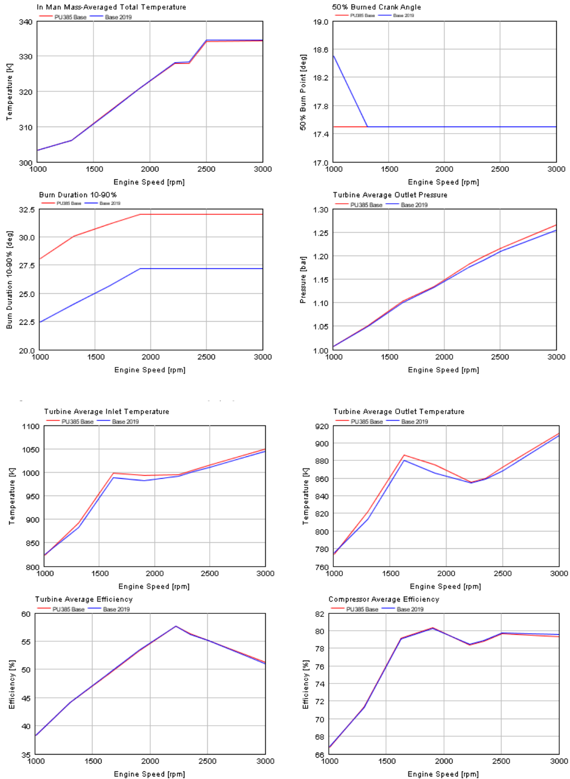
FIGURE B3.1C 2019 BASE ENGINE FULL LOAD COMPARISON
