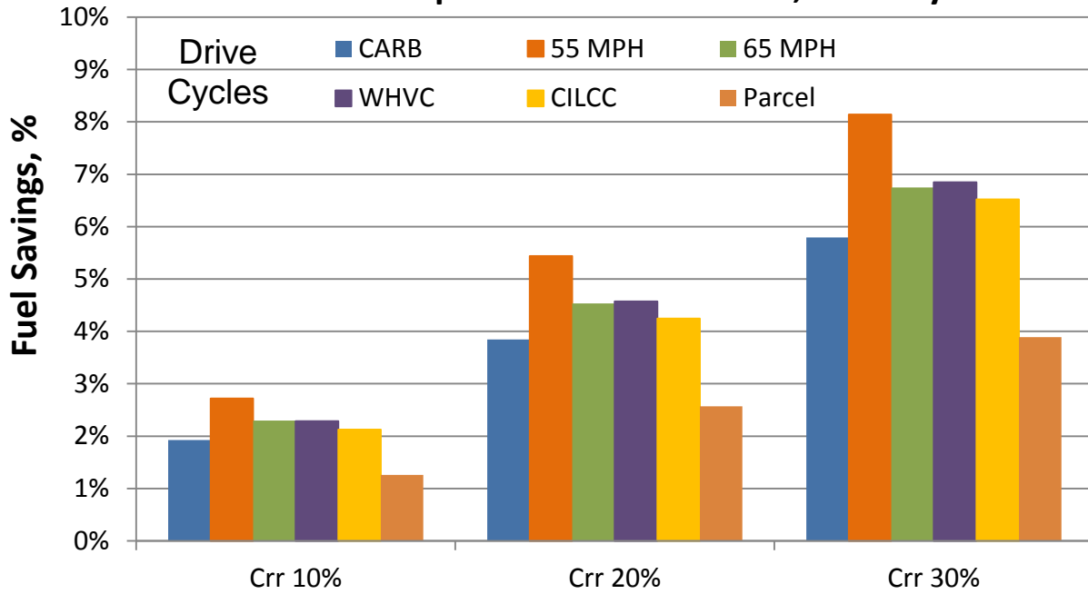
FIGURE 3.4 CRR SWEEP OF THE F-650 TOW TRUCK
