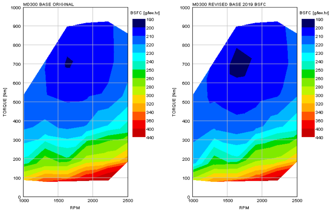
FIGURE B2.1C BSFC MAPS OF 2019 BASE ENGINE (RIGHT) VS. 2012 MEDIUM DUTY ISB
