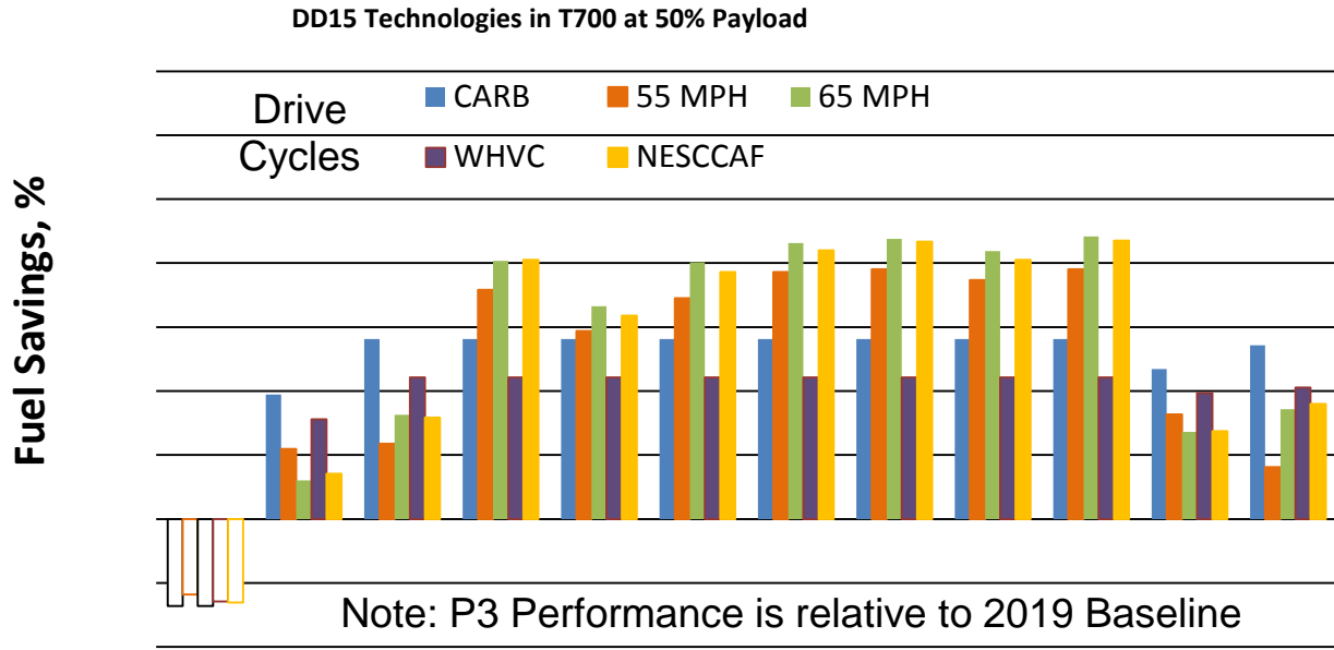
FIGURE 2.2 FUEL SAVING PERFORMANCE OF THE DD15 TECHNOLOGY PACKAGES, SHOWING THE FULL VALUE OF ALL TECHNOLOGY PACKAGES
