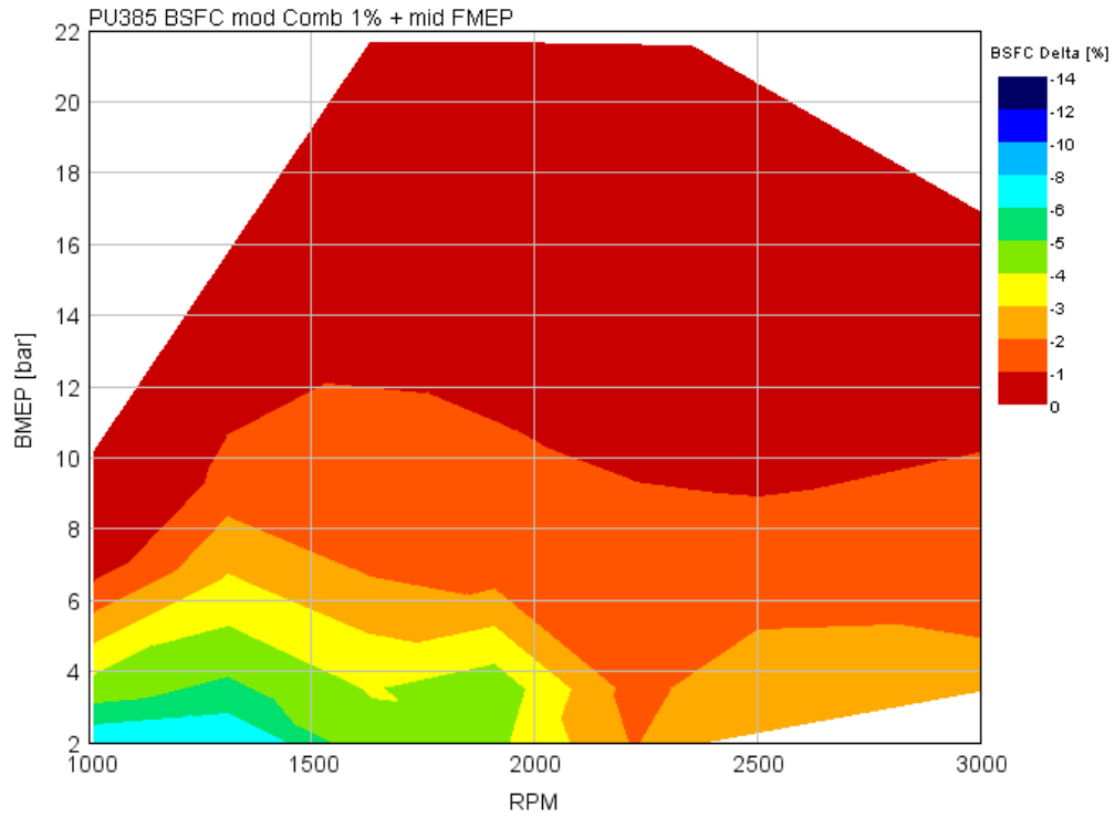
FIGURE B3.1B BSFC IMPROVEMENT OF 2019 BASE ENGINE VS. ORIGINAL BASE ENGINE
