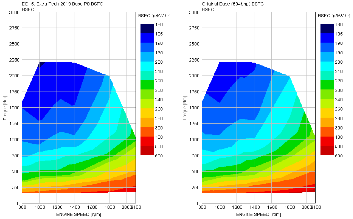
FIGURE B1.1C BSFC COMPARISON OF 2019 BASE DD15 VS. ORIGINAL DD15 (BOTH FEATURING IMPROVED COMBUSTION)
