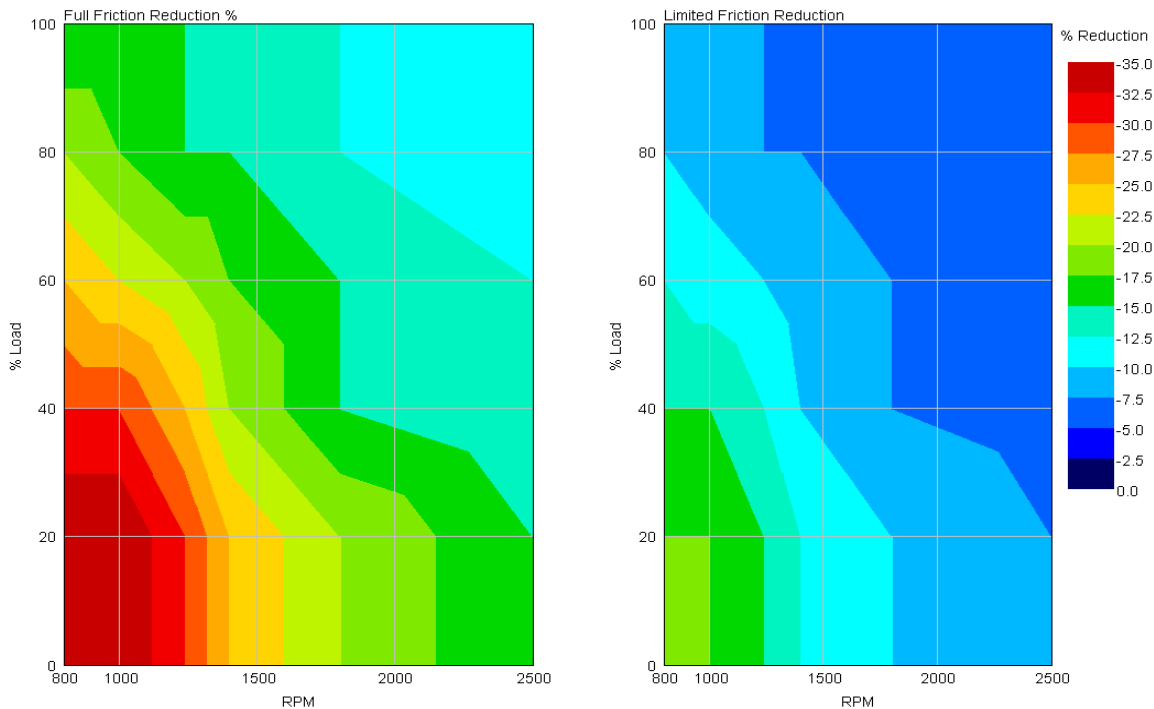
FIGURE B2.1A FRICTION REDUCTION COMPARISON
