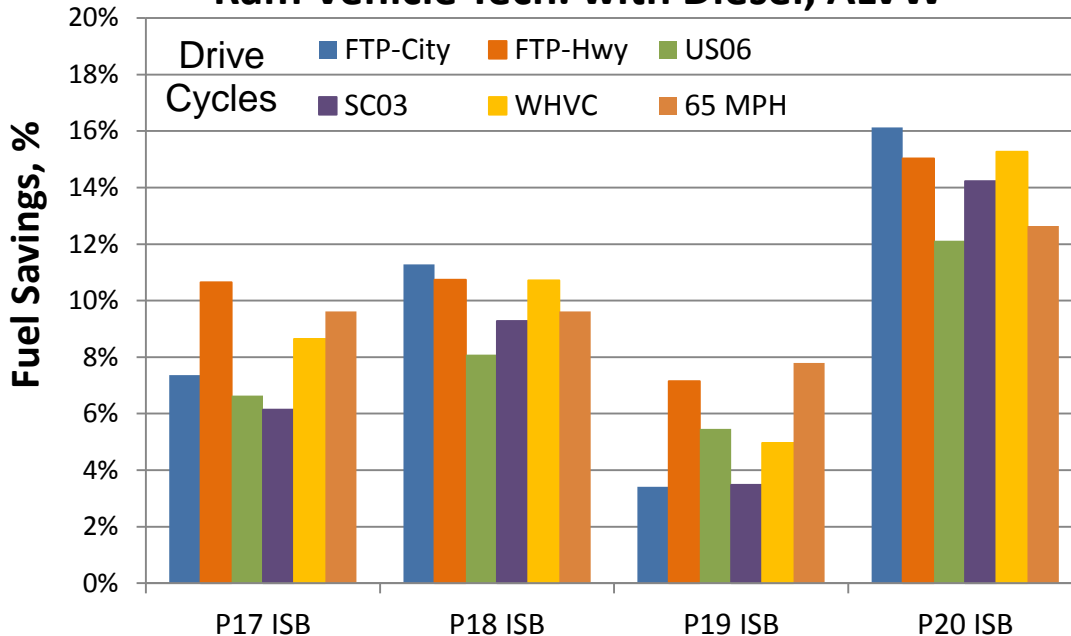
FIGURE 2.25 RAM VEHICLE TECHNOLOGY PACKAGE RESULTS WITH THE 2019 BASELINE DIESEL. THE FULL VALUE OF EACH PACKAGE IS SHOWN
