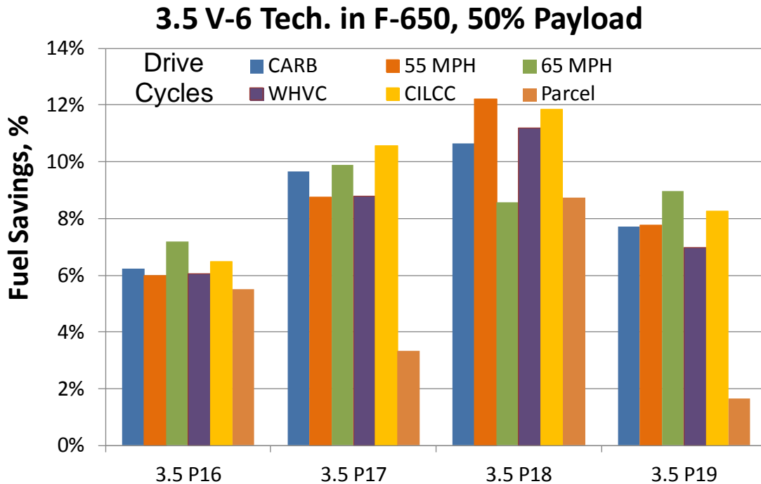
FIGURE 2.5 FUEL SAVING PERFORMANCE OF 3.5 V6 TECHNOLOGY PACKAGES IN THE F-650 TRUCK
