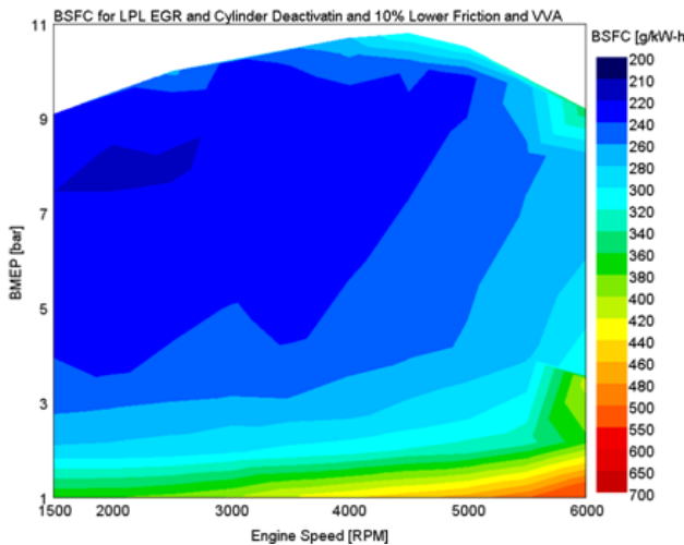
FIGURE A11 PACKAGE 2 COMBINED BSFC MAP
