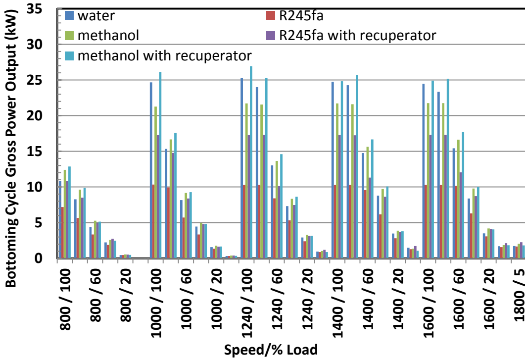
FIGURE B1.4A BOTTOMING CYCLE GROSS (TURBINE MECHANICAL) POWER OUTPUT FOR PACKAGE 3
