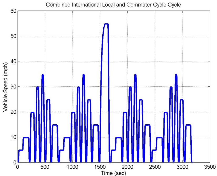
FIGURE C15 COMBINED INTERNATIONAL LOCAL AND COMMUTER DRIVE CYCLE (CILCC)
