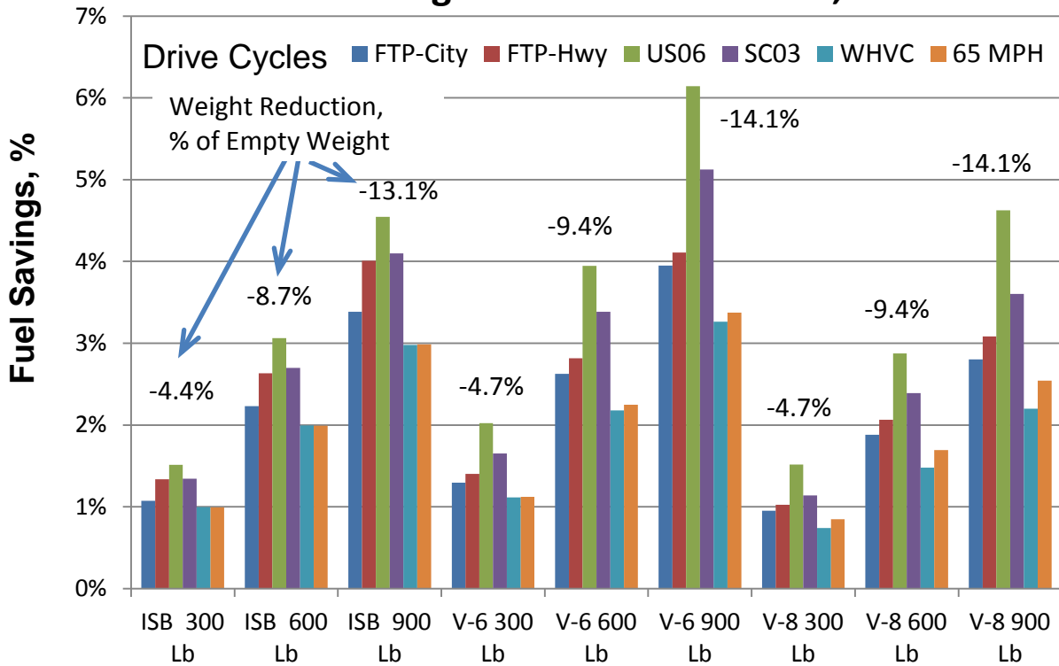
FIGURE 3.9 EFFECT OF EMPTY WEIGHT REDUCTION ON RAM PICKUP
