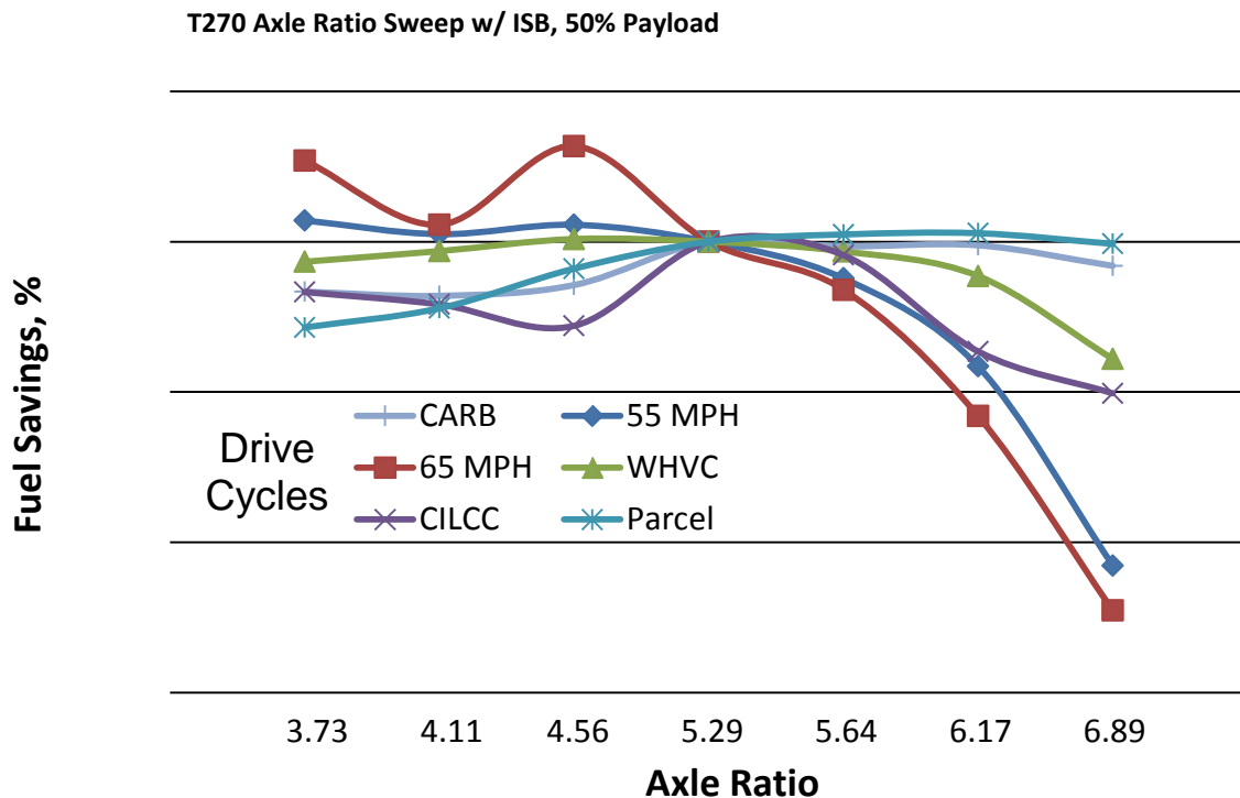
FIGURE 3.13 AXLE RATIO SWEEP ON T270 WITH THE DIESEL
