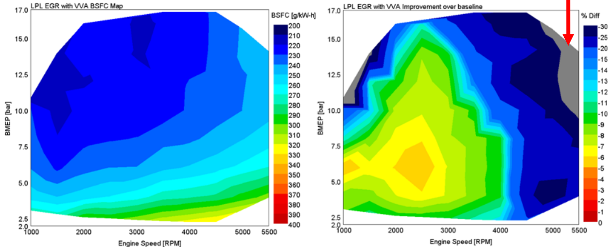
Figure A1 VVA/VL/EGR BSFC Map
