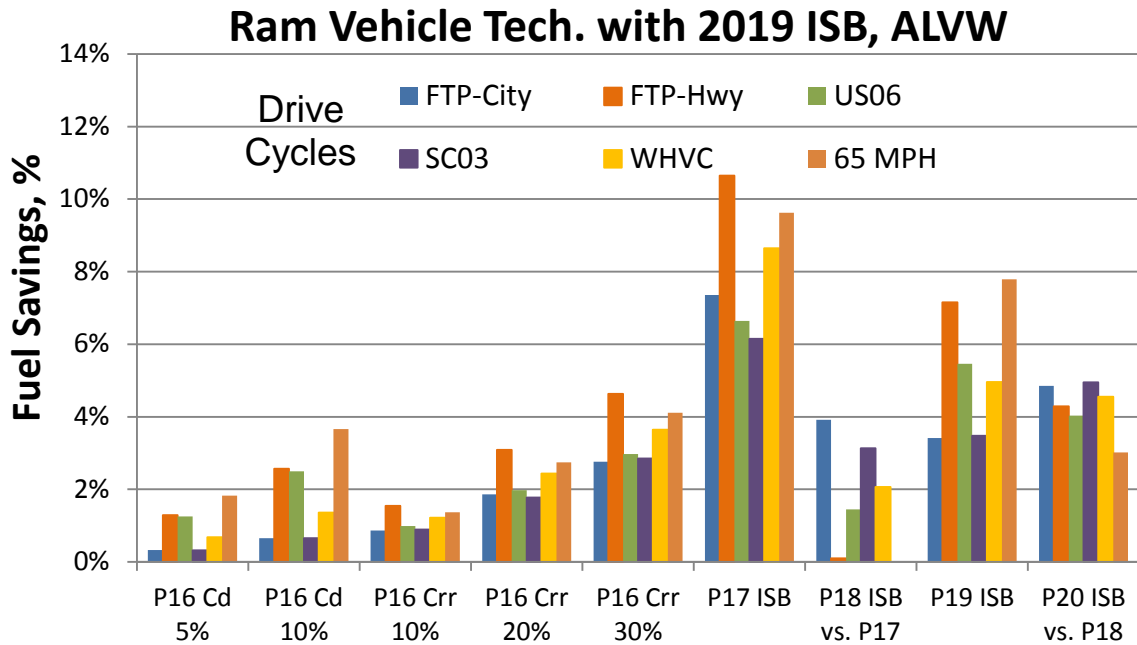
FIGURE 2.23 RAM VEHICLE TECHNOLOGY PACKAGE RESULTS WITH THE 2019 BASELINE DIESEL. P18 IS COMPARED TO P17, AND P20 TO P18
