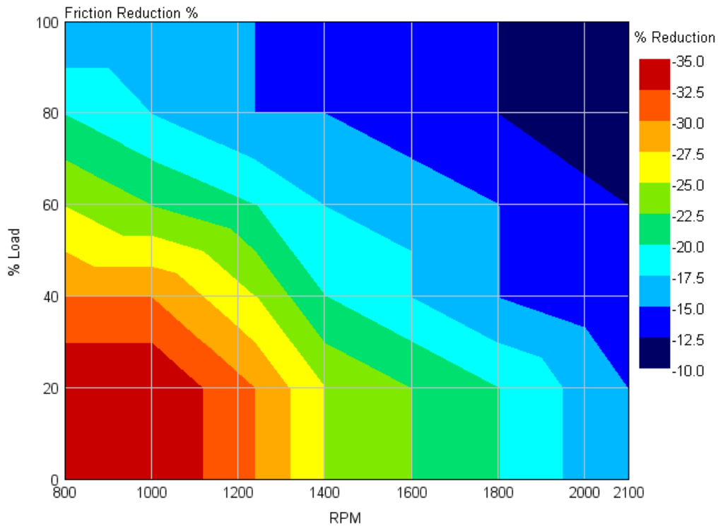
FIGURE B1.2A FRICTION REDUCTION ASSUMPTION
