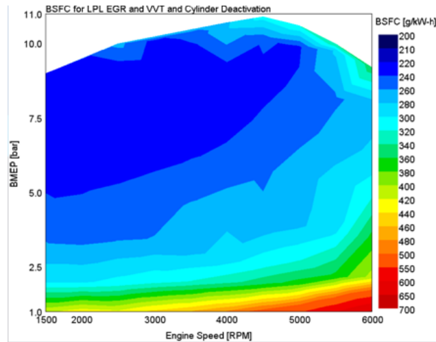
FIGURE A18 PACKAGE 5 COMBINED BSFC MAP
