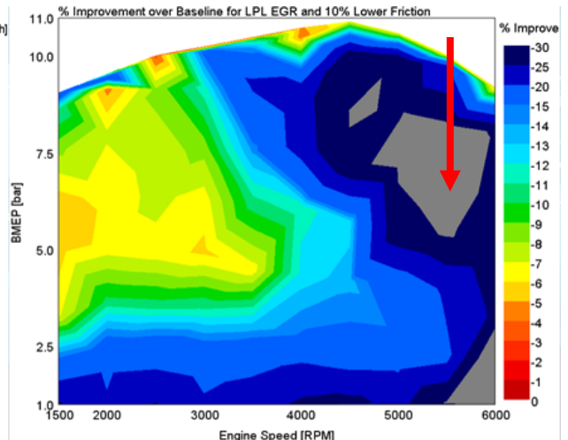
FIGURE A10 BSFC IMPROVEMENT
