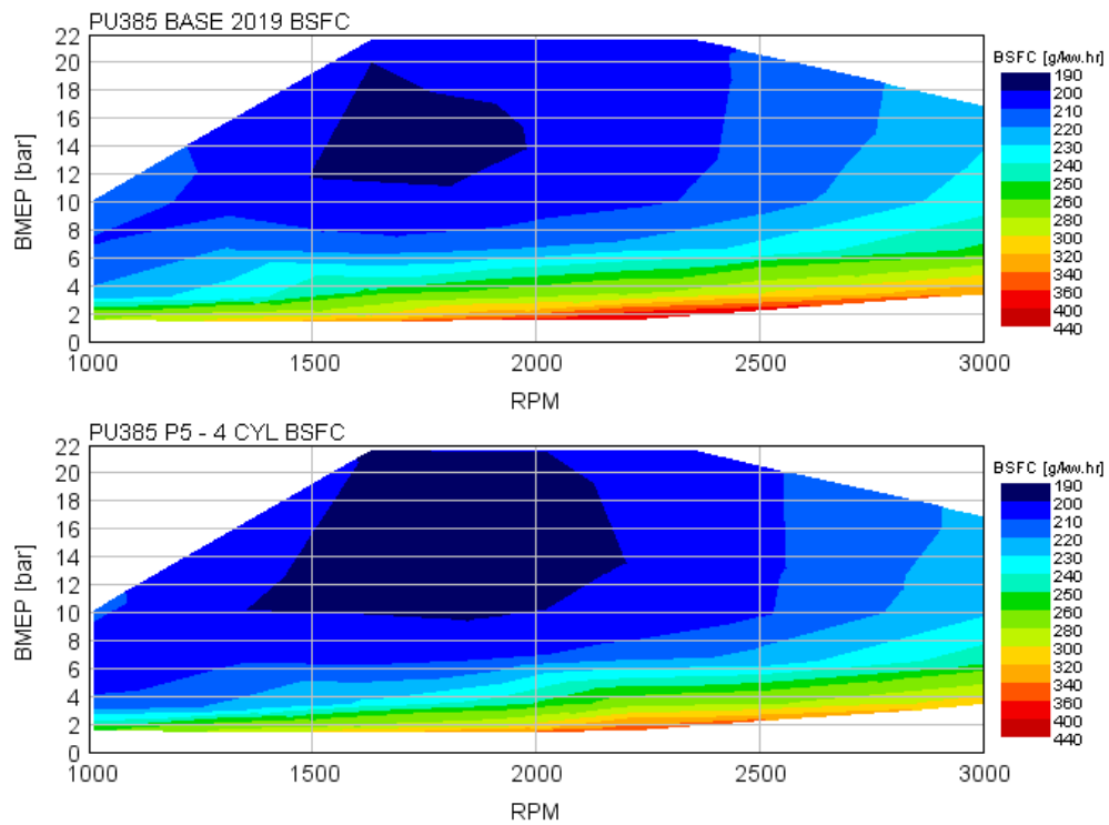
FIGURE B3.6B BSFC COMPARISON OF P15 I4 – BMEP
