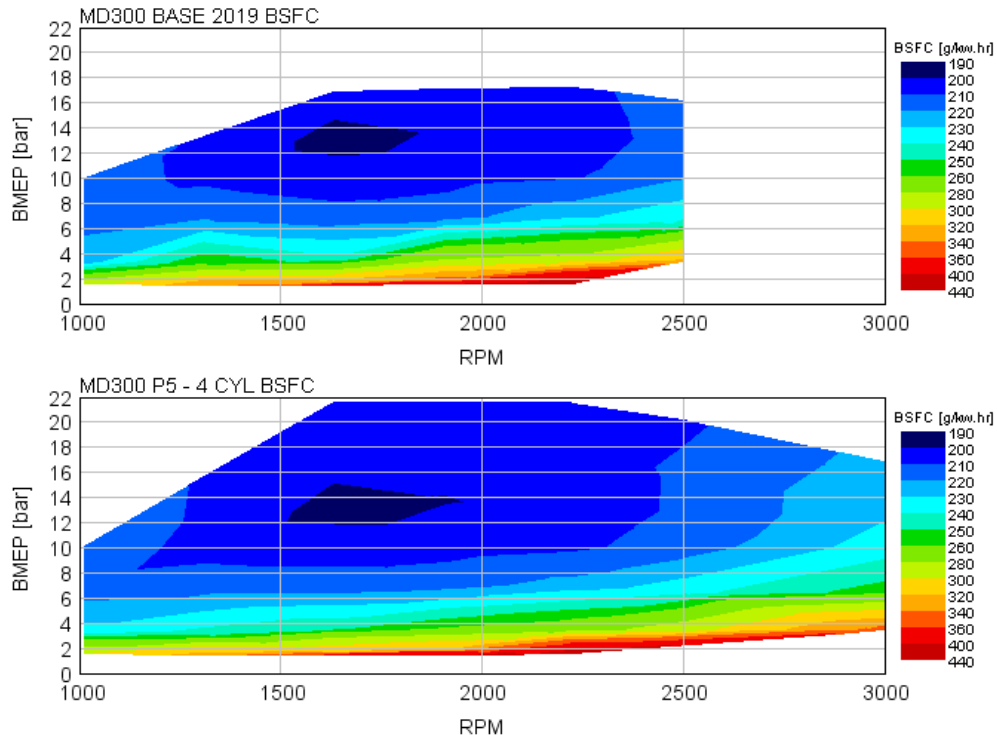
FIGURE B2.6A BSFC MAPS OF BASE 2019 ENGINE AND PACKAGE 10
