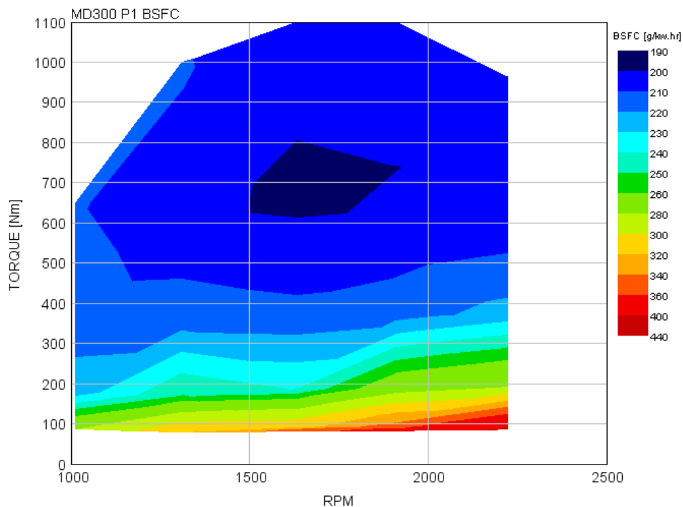
FIGURE B2.2A BSFC MAP FOR COMBO PACKAGE 6
