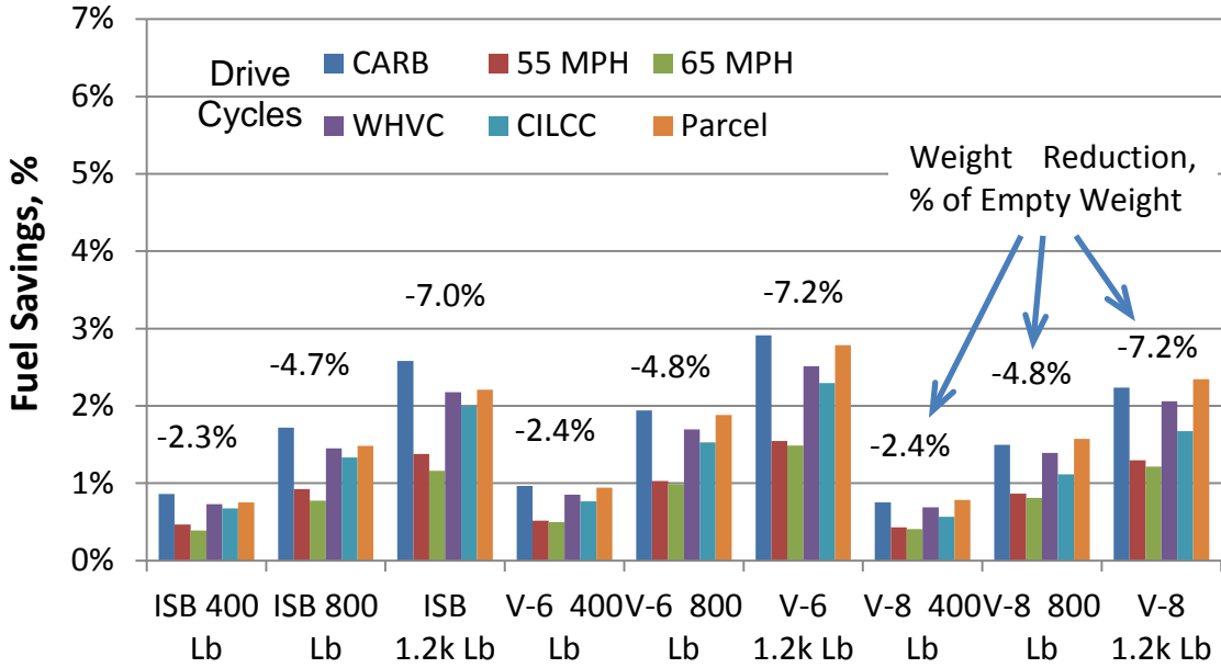
FIGURE 3.8 EFFECT OF EMPTY WEIGHT REDUCTION ON T270
