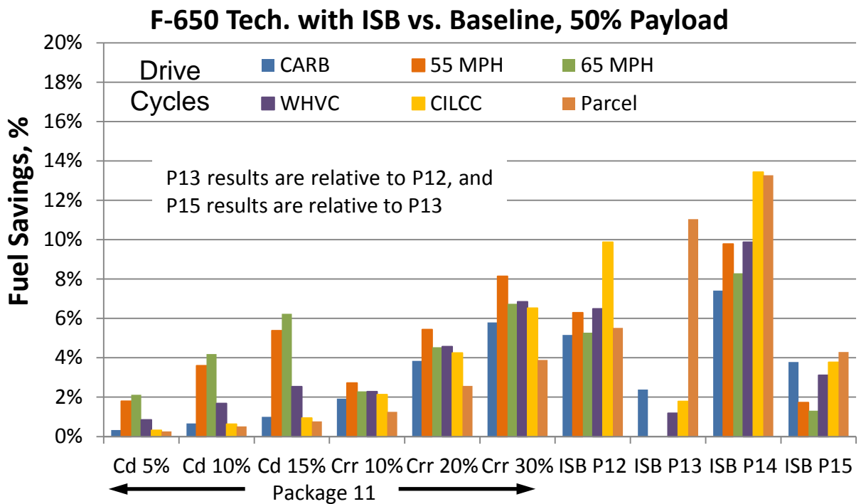
FIGURE 2.8 F-650 VEHICLE TECHNOLOGY COMBINATION FUEL SAVINGS RESULTS WITH THE 2019 BASELINE ISB ENGINE. VP13 RESULTS ARE RELATIVE TO VP12, AND VP15 TO VP13
