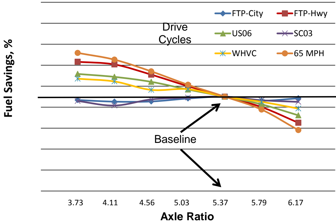
FIGURE 3.17 AXLE RATIO SWEEP ON RAM PICKUP WITH V-6 GASOLINE
