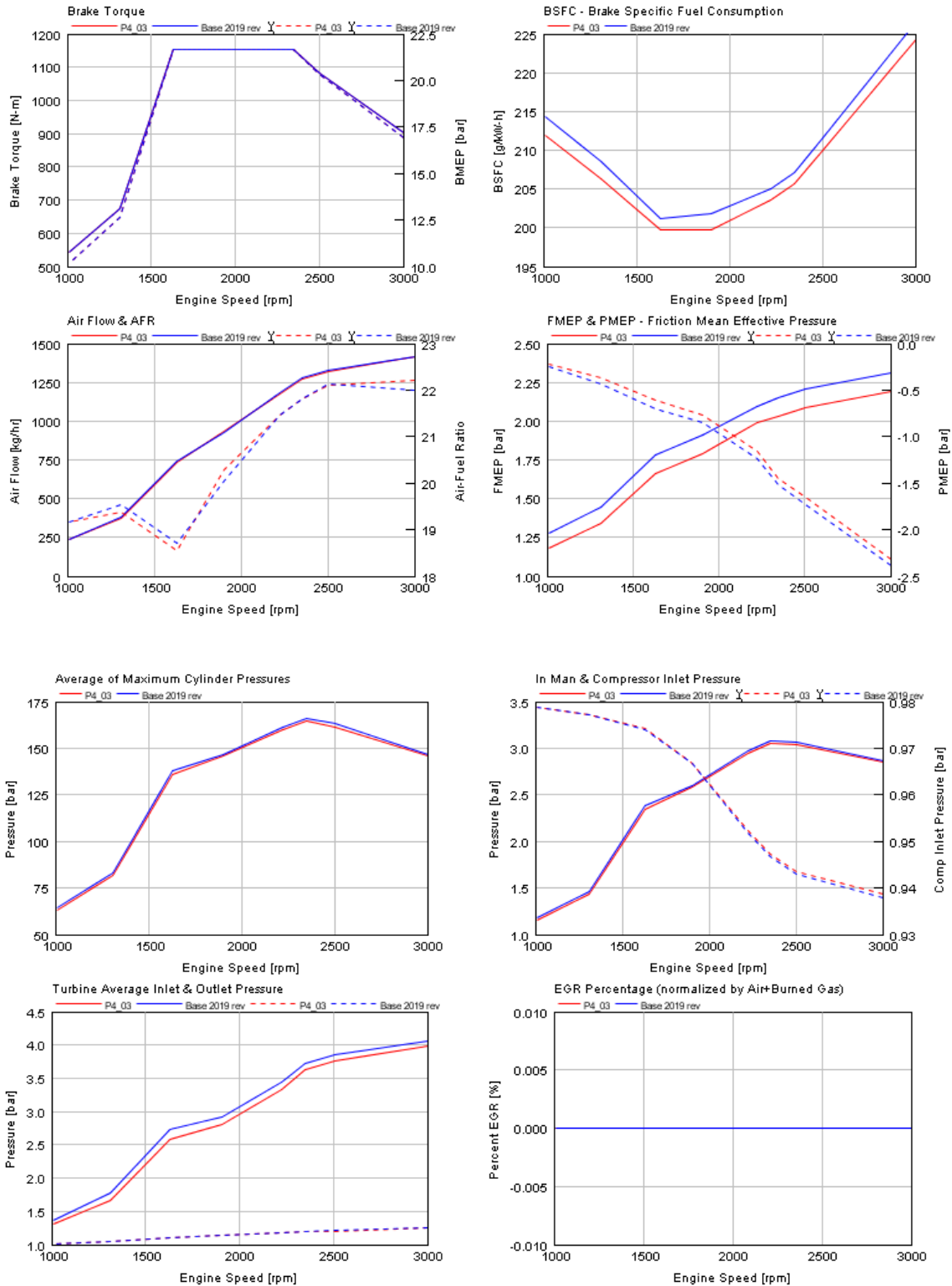
FIGURE B3.5C FULL LOAD PERFORMANCE COMPARISON (P14)
