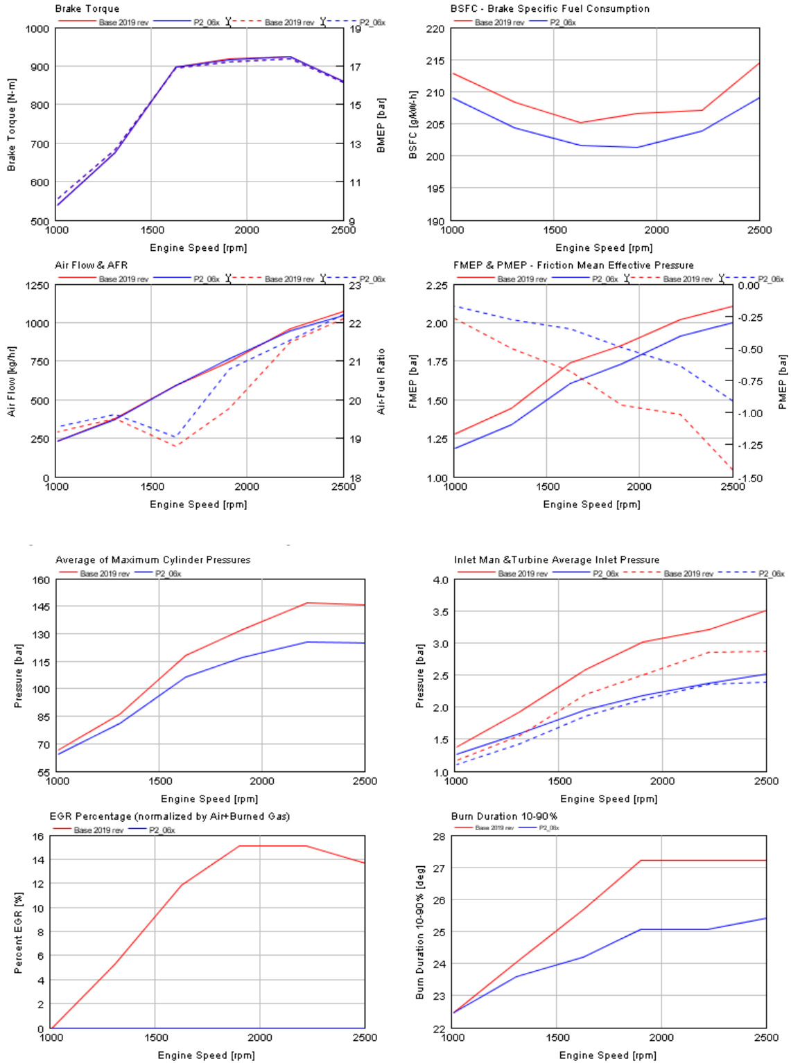
FIGURE B2.3C PACKAGE 7 FULL LOAD PERFORMANCE COMPARISON
