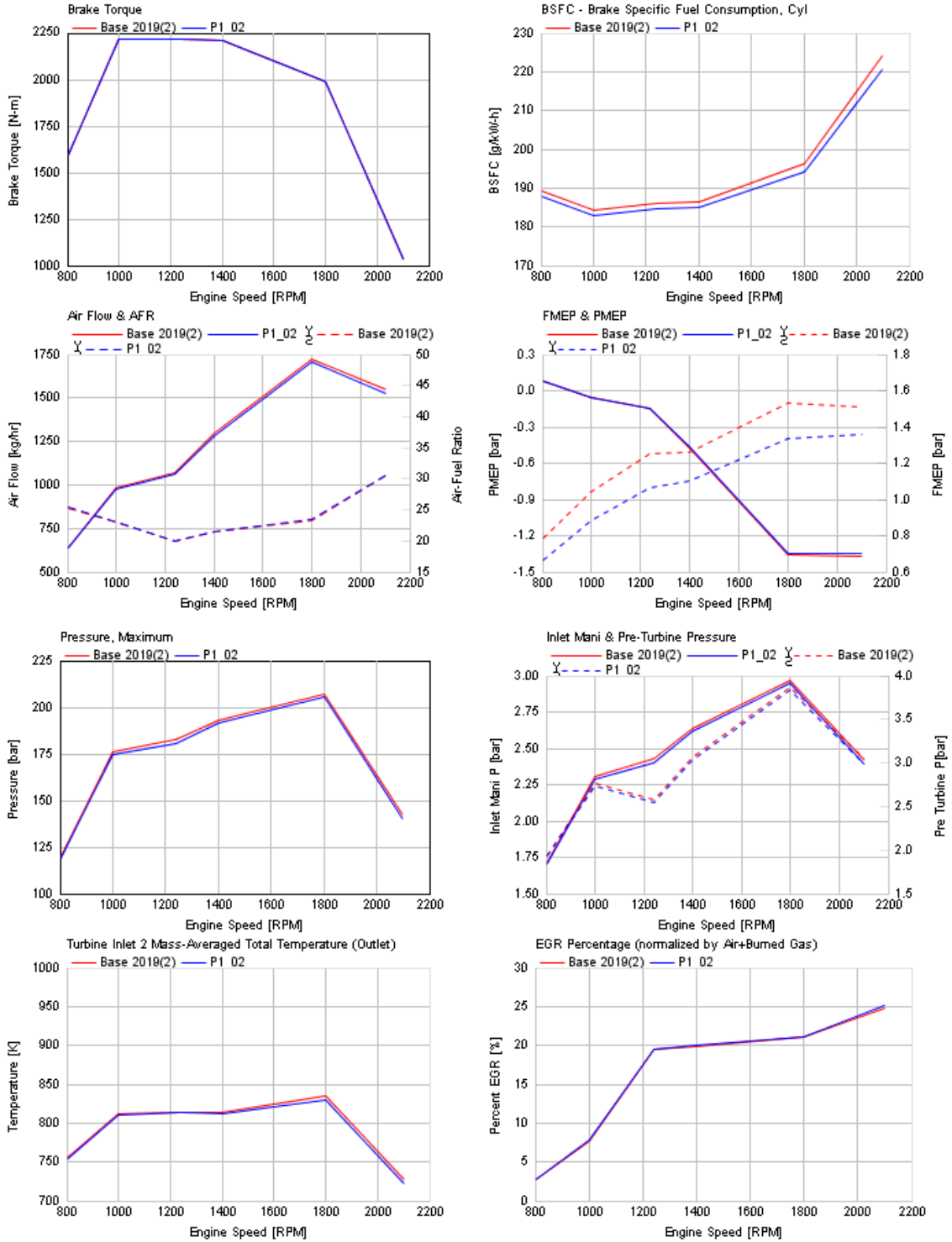
FIGURE B1.2C FULL LOAD PERFORMANCE COMPARISON – PACKAGE 1 VS. 2019 BASELINE
