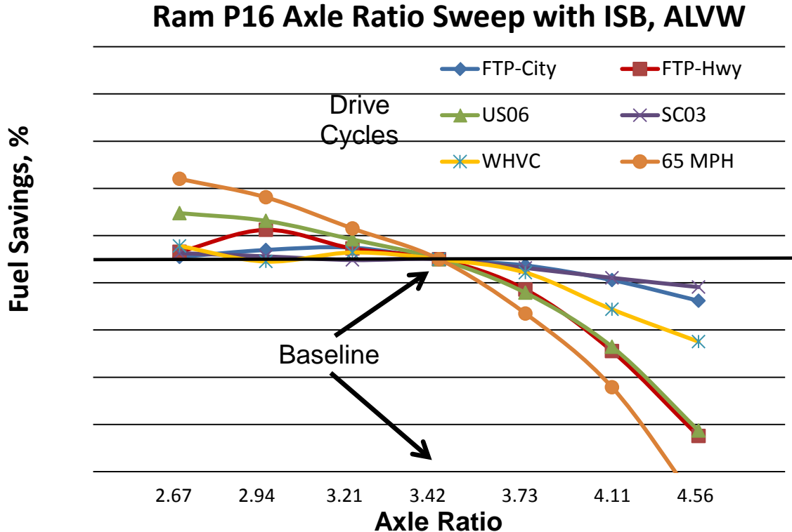
FIGURE 3.16 AXLE RATIO SWEEP ON RAM PICKUP WITH DIESEL
