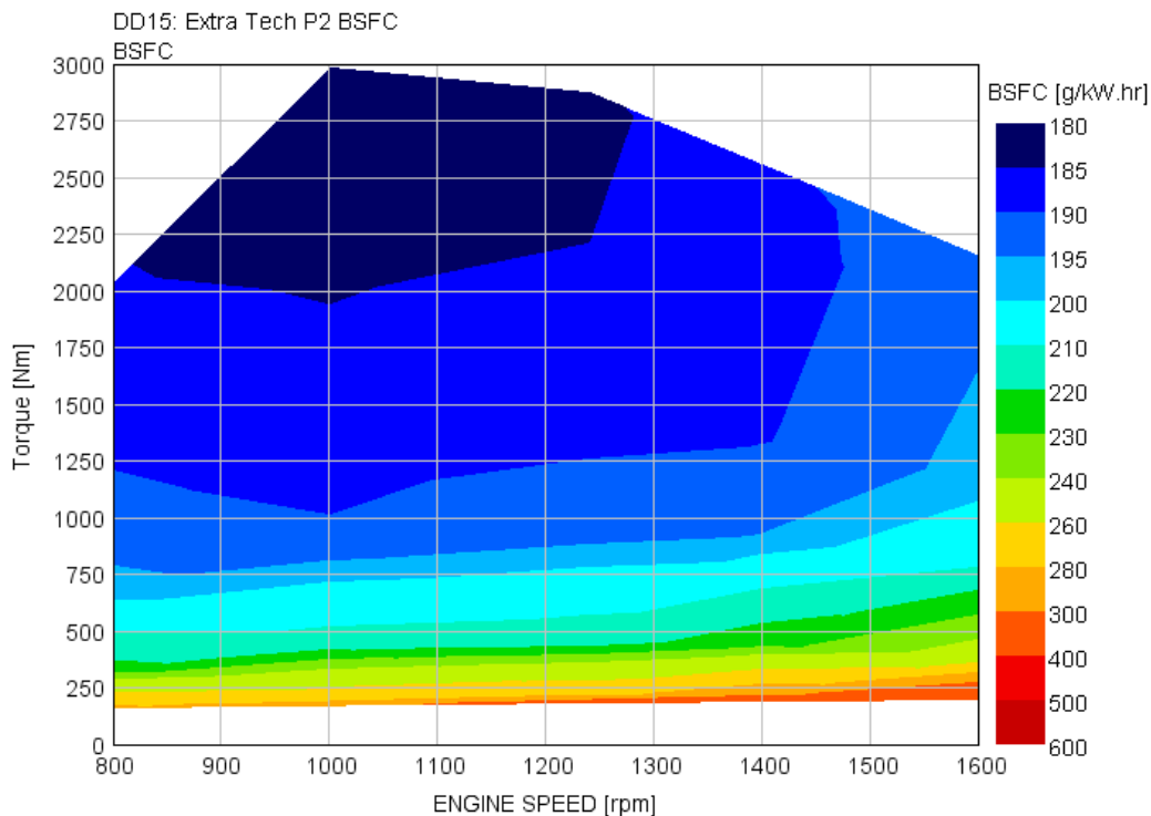
FIGURE B1.3A BSFC MAP OF PACKAGE 2 ENGINE
