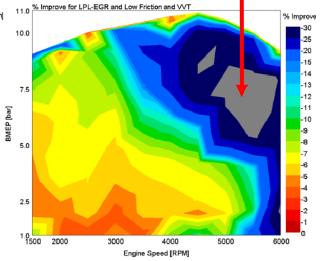
FIGURE A21 BSFC IMPROVEMENT OVER BASELINE
