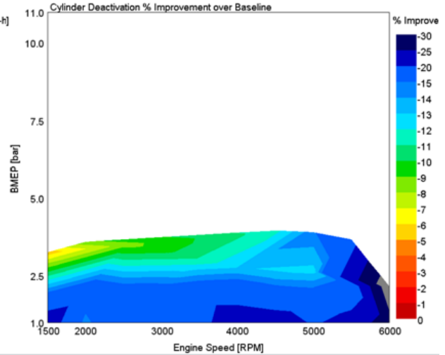
FIGURE A17 BSFC IMPROVEMENT OVER BASELINE
