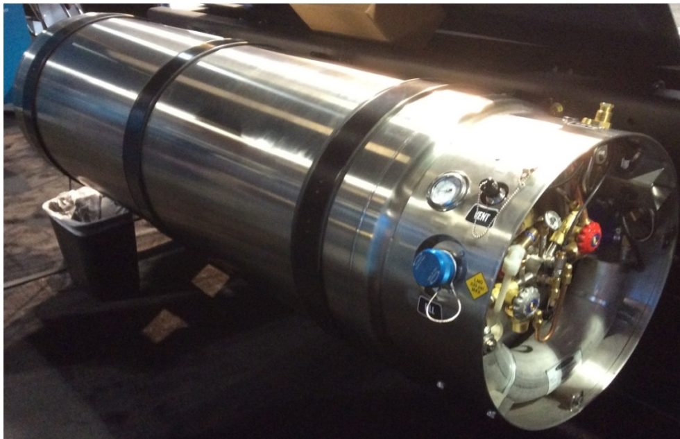
FIGURE 5.4 EXAMPLES OF LNG STORAGE TANKS
