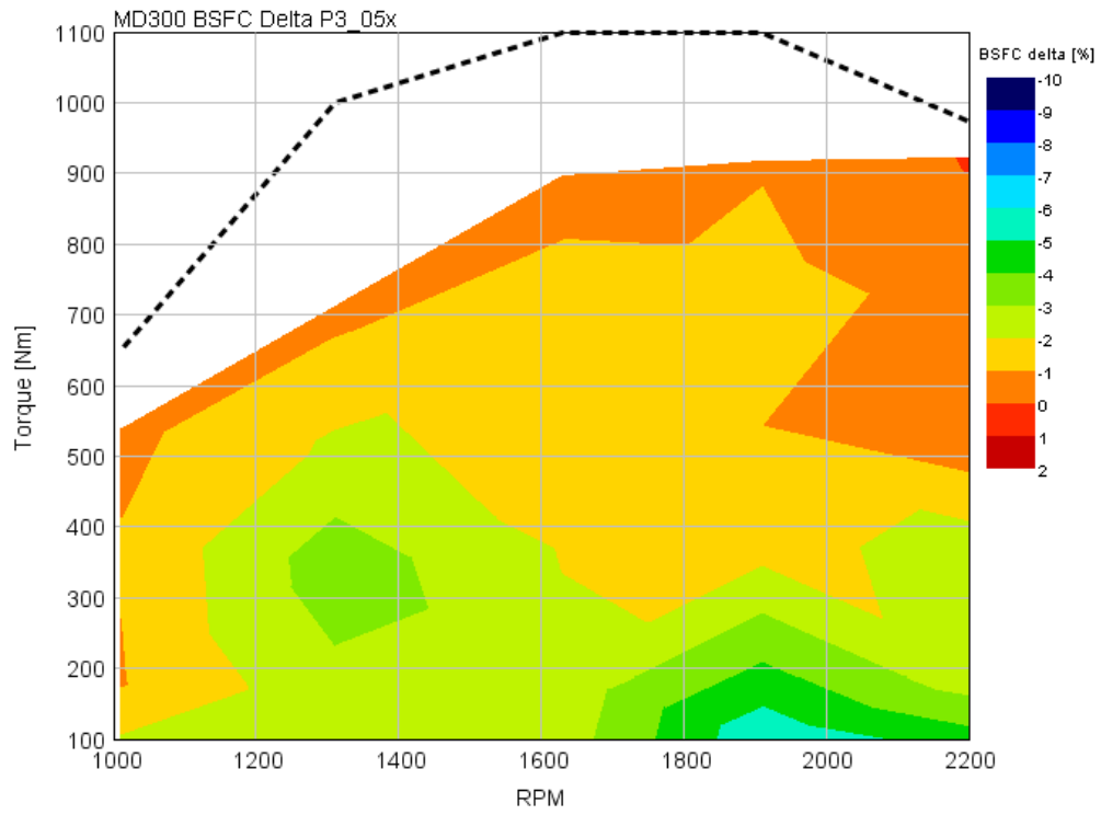
FIGURE B2.4B BSFC IMPROVEMENT MAP OF PACKAGE 8 VS. 2019 BASELINE
