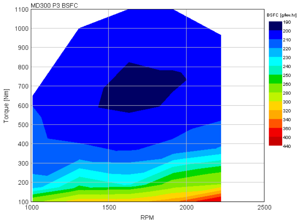
FIGURE B2.4A BSFC MAP OF PACKAGE 8
