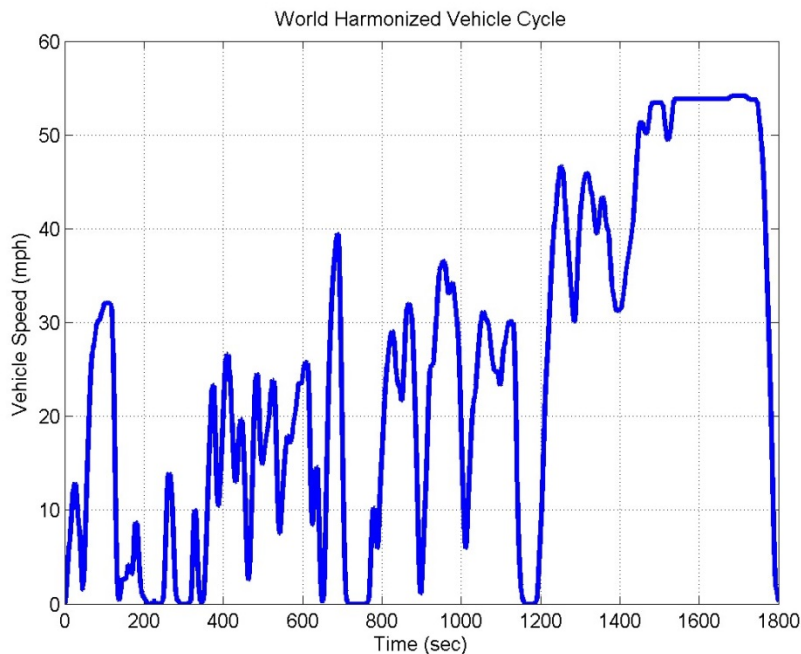
FIGURE C8 WORLD HARMONIZED VEHICLE CYCLE (WHVC)
