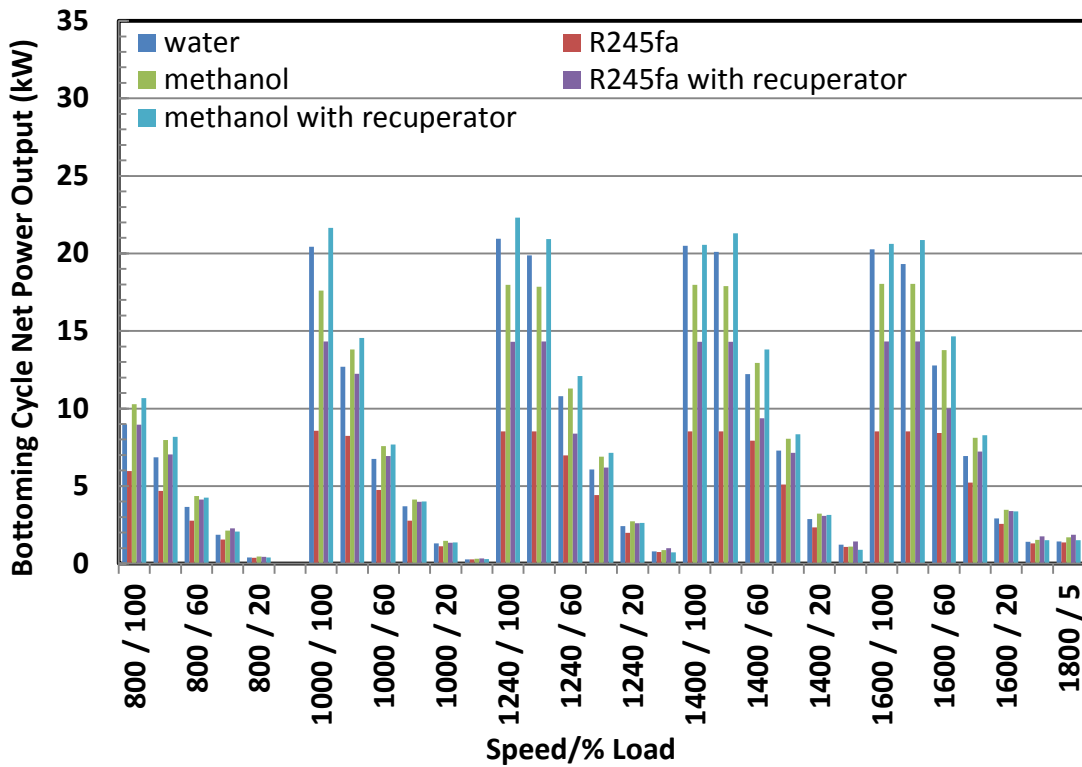
FIGURE B1.4B BOTTOMING CYCLE NET POWER OUTPUT (AFTER GENERATOR AND MOTOR CONVERSIONS) FOR PACKAGE 3
