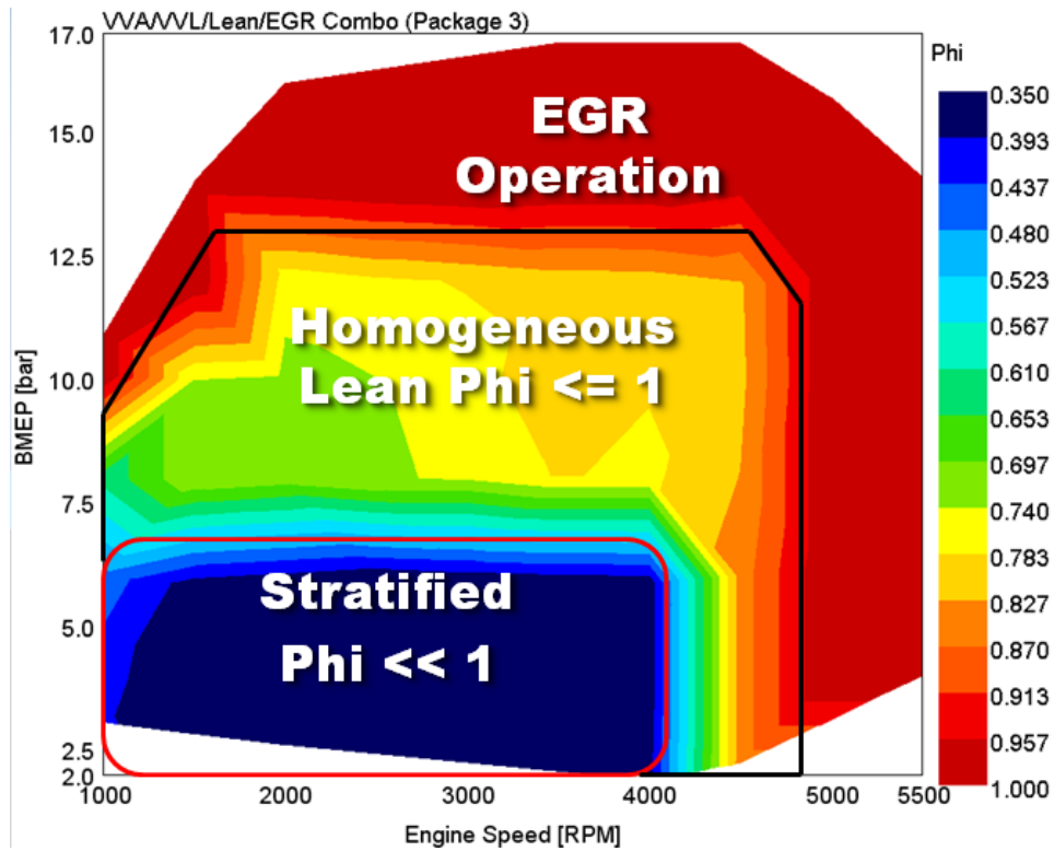
Figure A4 Package 3 Engine Operating Modes
