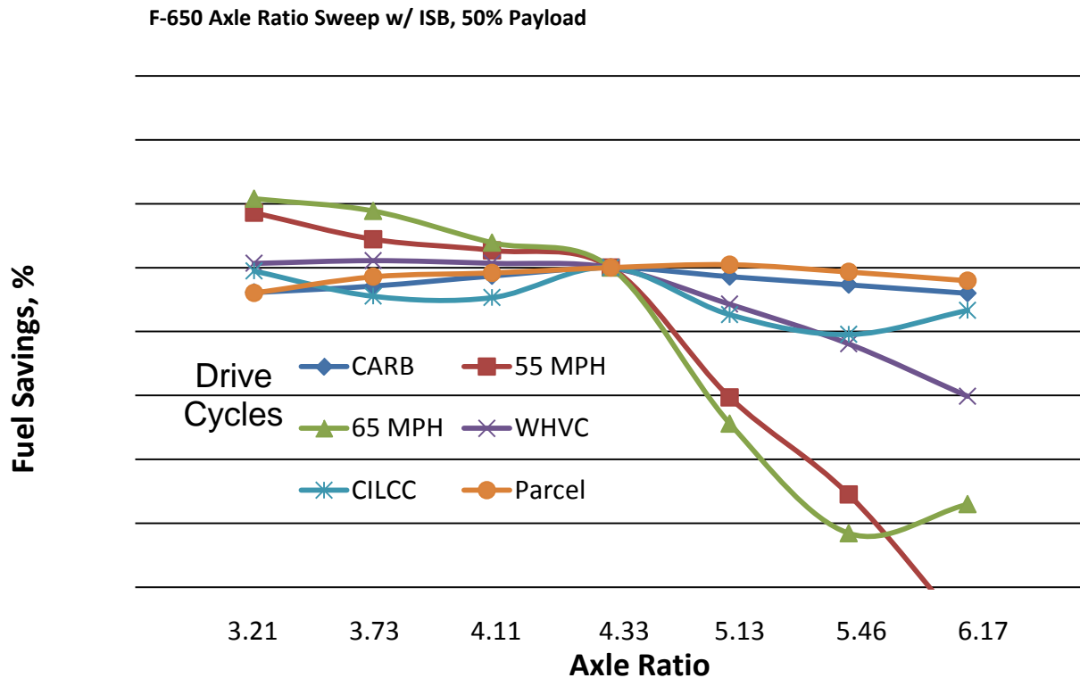
FIGURE 3.10 AXLE RATIO SWEEP ON F-650 WITH THE DIESEL
