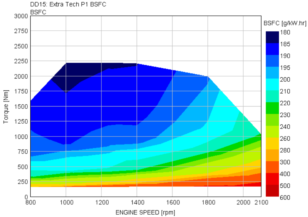
FIGURE B1.2B BSFC MAP OF PACKAGE 1 ENGINE
