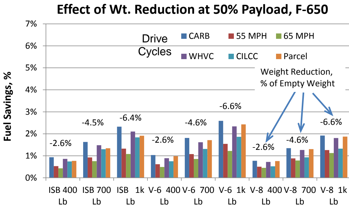
FIGURE 3.7 EFFECT OF EMPTY WEIGHT REDUCTION ON F-650
