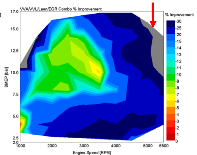
FIGURE A6 BSFC IMPROVEMENT OVER BASELINE
