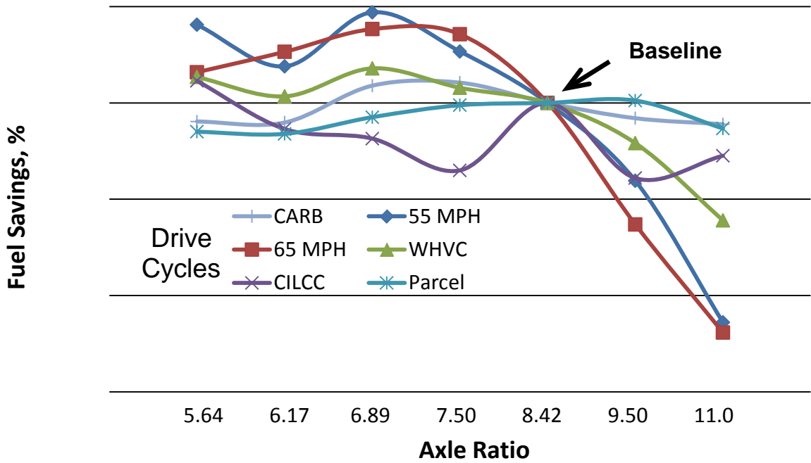
FIGURE 3.15 AXLE RATIO SWEEP ON T270 WITH THE 6.2 V-8
