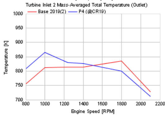
FIGURE B1.5C FULL LOAD PERFORMANCE COMPARISON
