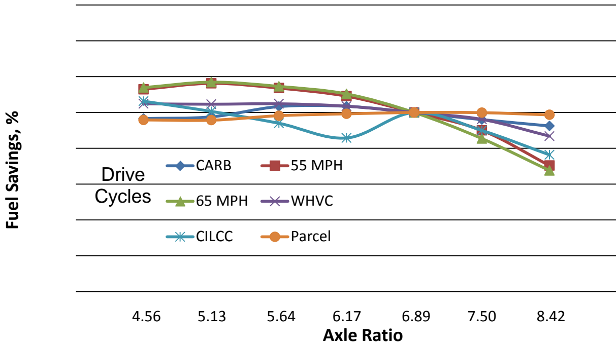
FIGURE 3.11 AXLE RATIO SWEEP ON F-650 WITH THE 3.5 V-6
