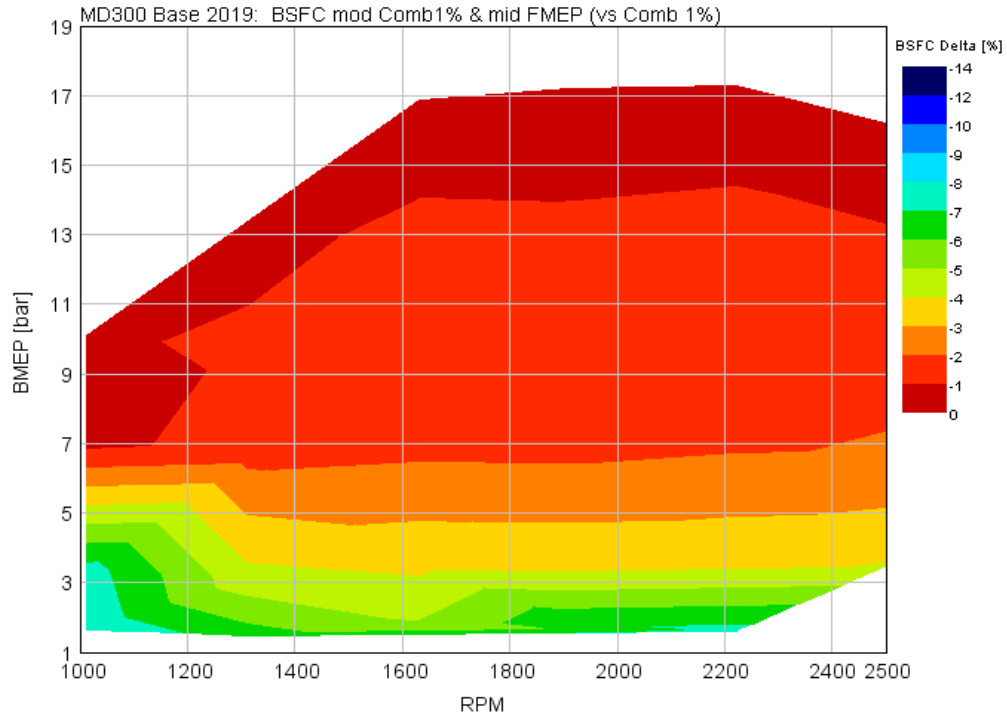
FIGURE B2.1B BSFC IMPROVEMENT MAP OF 2019 BASE ENGINE VS. ORIGINAL MEDIUM DUTY ISB
