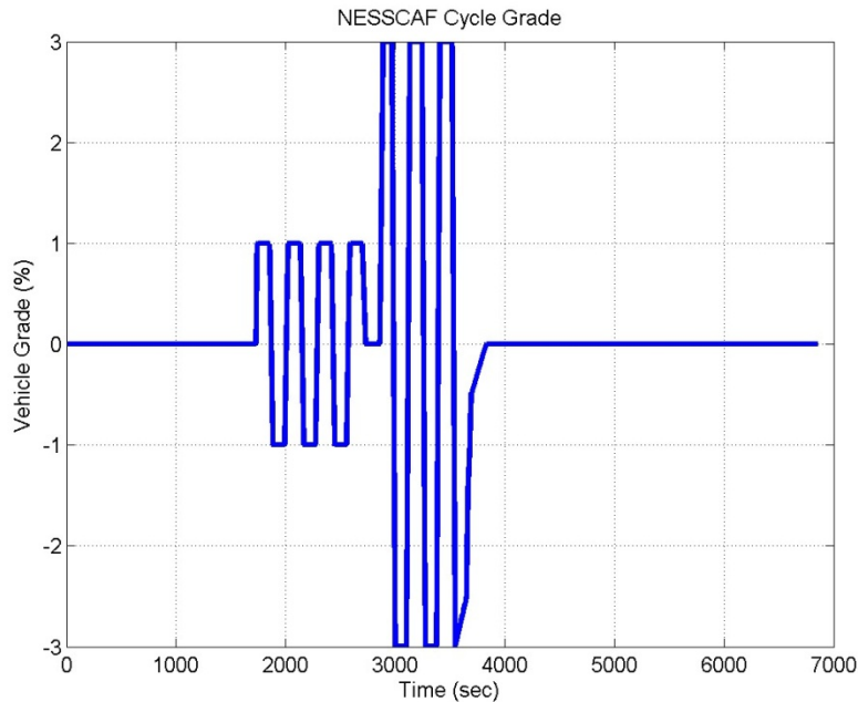
FIGURE C7 GRADE VS. TIME TRACE FOR THE NESSCAF CYCLE
