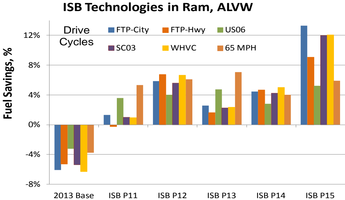
FIGURE 2.19 DIESEL TECHNOLOGY COMBINATIONS IN THE RAM PICKUP
