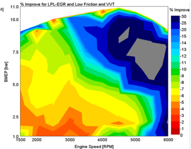
FIGURE A15 BSFC IMPROVEMENT OVER BASELINE
