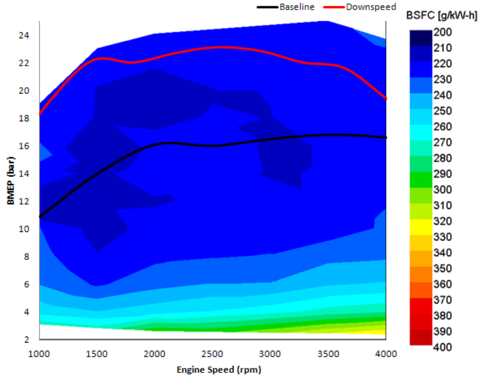
FIGURE A3 BMEP COMPARISON OF STANDARD AND DOWN SPEED TORQUE CURVES
