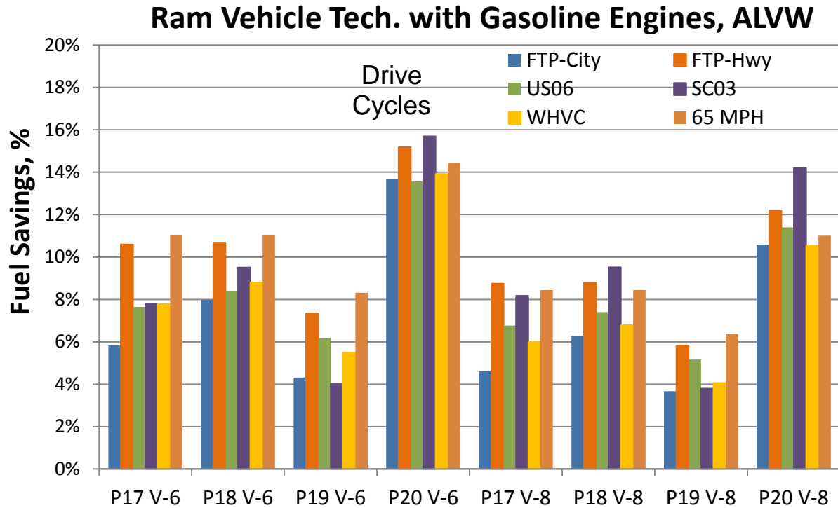
FIGURE 2.26 RAM VEHICLE TECHNOLOGY RESULTS WITH THE BASELINE GASOLINE ENGINES. THE FULL VALUE OF EACH PACKAGE IS SHOWN
