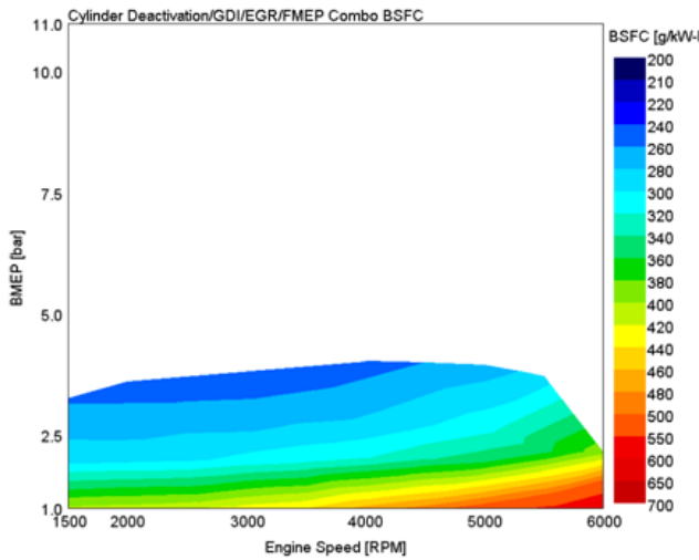
FIGURE A7 CYL. DEACT BSFC MAP
