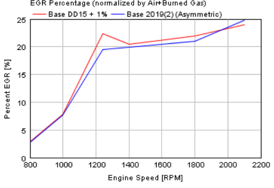
FIGURE B1.1D 2019 BASE ENGINE COMPARISON WITH ORIGINAL DD15 (BOTH FEATURING IMPROVED COMBUSTION)
