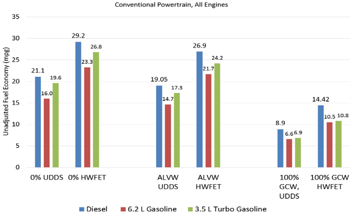
FIGURE D.1 FUEL ECONOMY COMPARISON OF 3 ENGINES IN THE BASELINE RAM PICKUP
