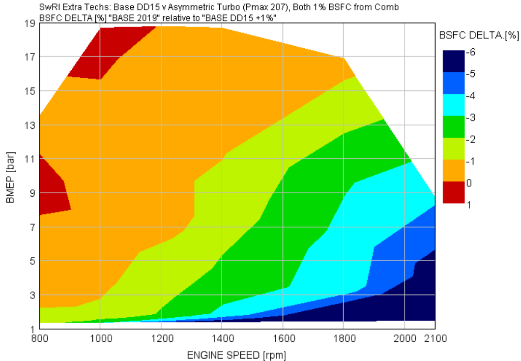
FIGURE B1.1B BSFC IMPROVEMENT OF 2019 BASE DD15 VS. ORIGINAL 2013/2014 NON-TURBOCOMPOUND DD15 (BOTH FEATURING IMPROVED COMBUSTION)
