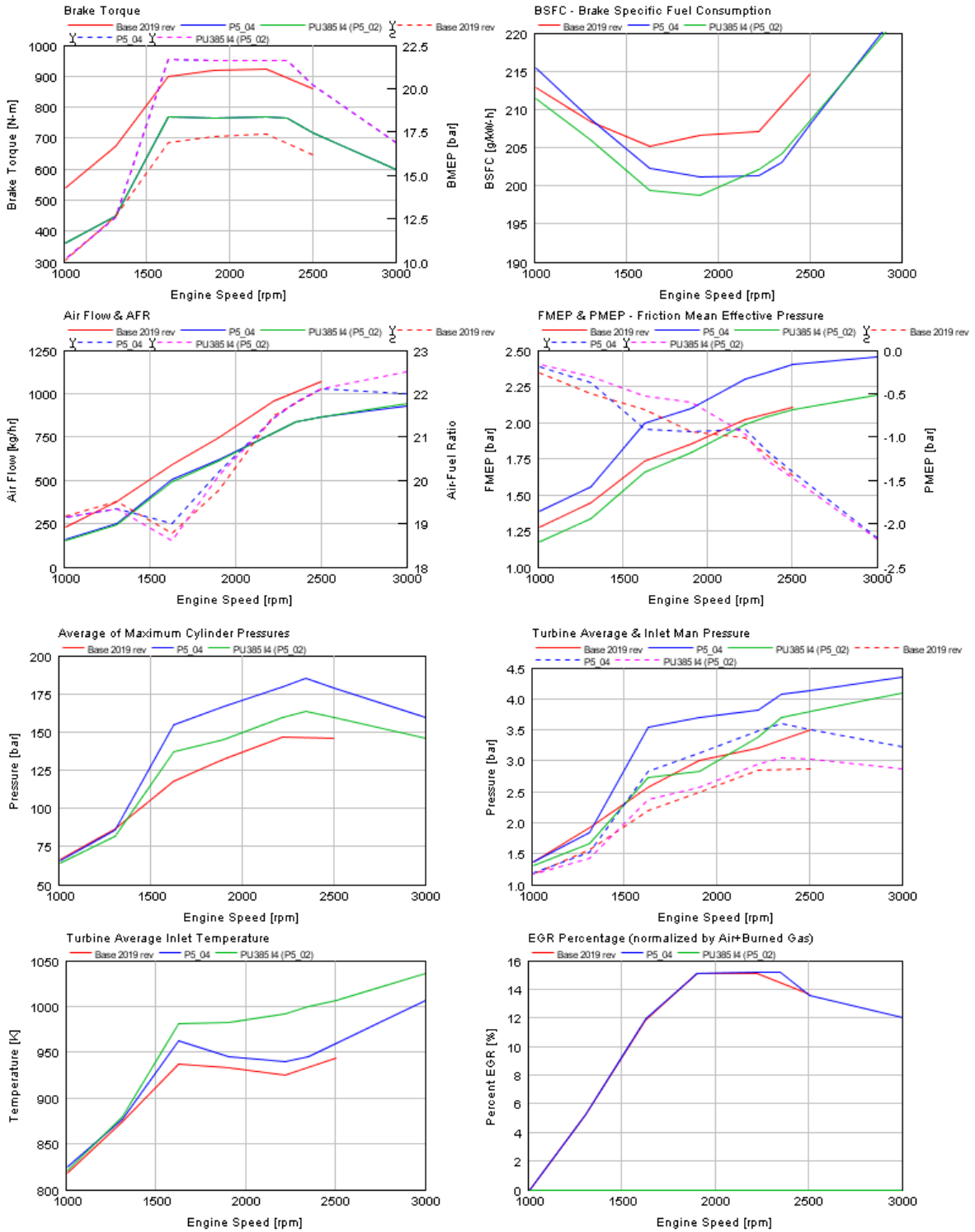
FIGURE B2.6C PACKAGE 10 FULL LOAD PERFORMANCE COMPARISON. NOTE THAT THE BLUE CURVES REPRESENT PACKAGE 10, WHILE GREEN REPRESENTS THE 4-CYLINDER PICKUP VERSION.
