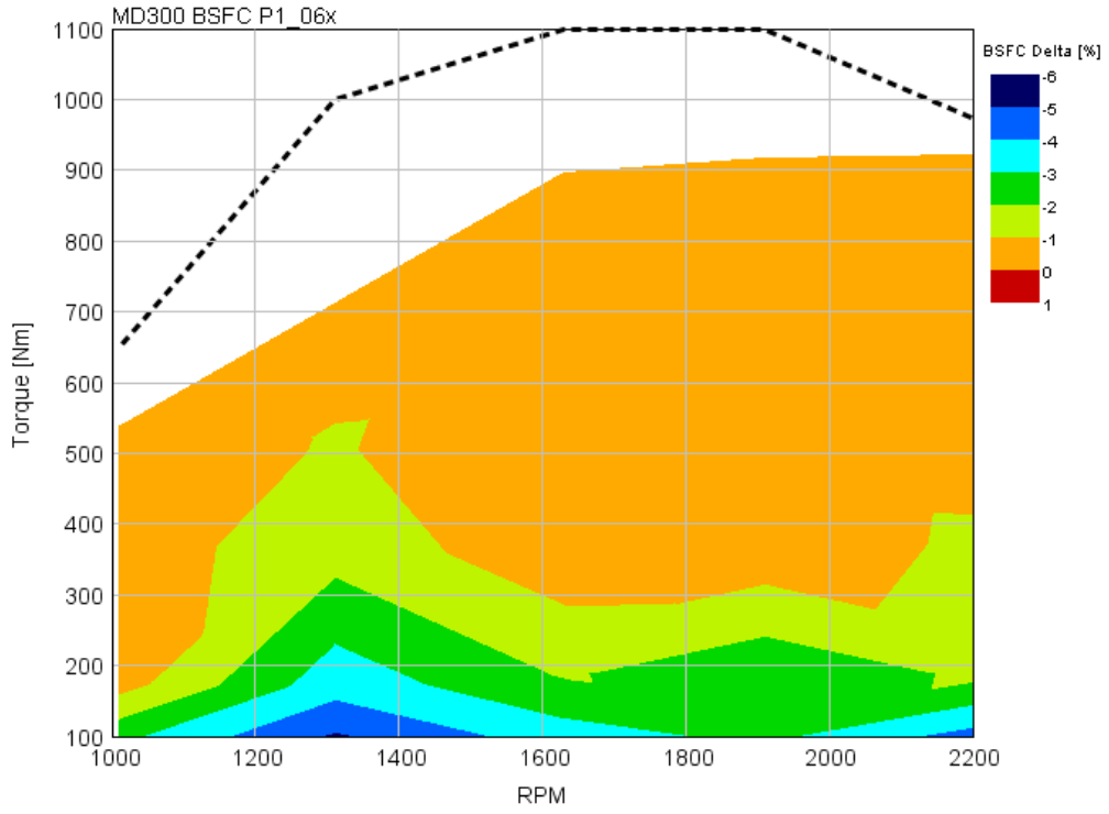
FIGURE B2.2B BSFC IMPROVEMENT MAP FOR COMBO PACKAGE 6 VS. 2019 BASELINE
