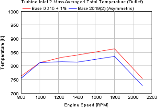
FIGURE B1.1D 2019 BASE ENGINE COMPARISON WITH ORIGINAL DD15 (BOTH FEATURING IMPROVED COMBUSTION)
