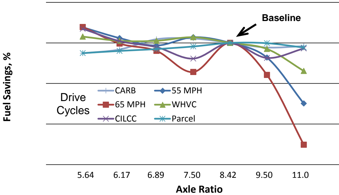
FIGURE 3.14 AXLE RATIO SWEEP ON T270 WITH THE 3.5 V-6
