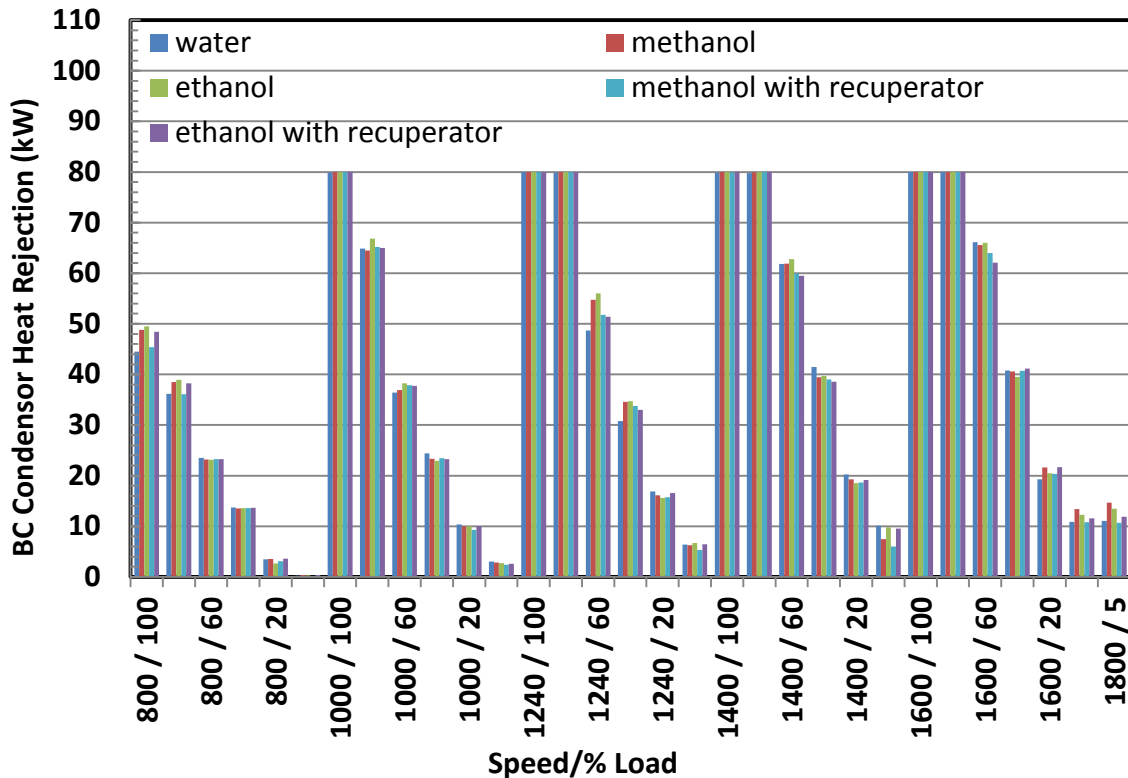
FIGURE X1.4H BC CONDENSER HEAT TRANSFER FOR METHANOL AND ETHANOL
