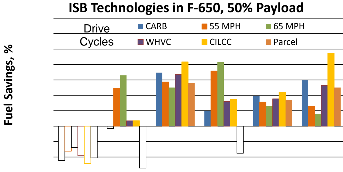
FIGURE 2.4 FUEL SAVING PERFORMANCE OF ISB TECHNOLOGY PACKAGES IN THE F-650 TRUCK
