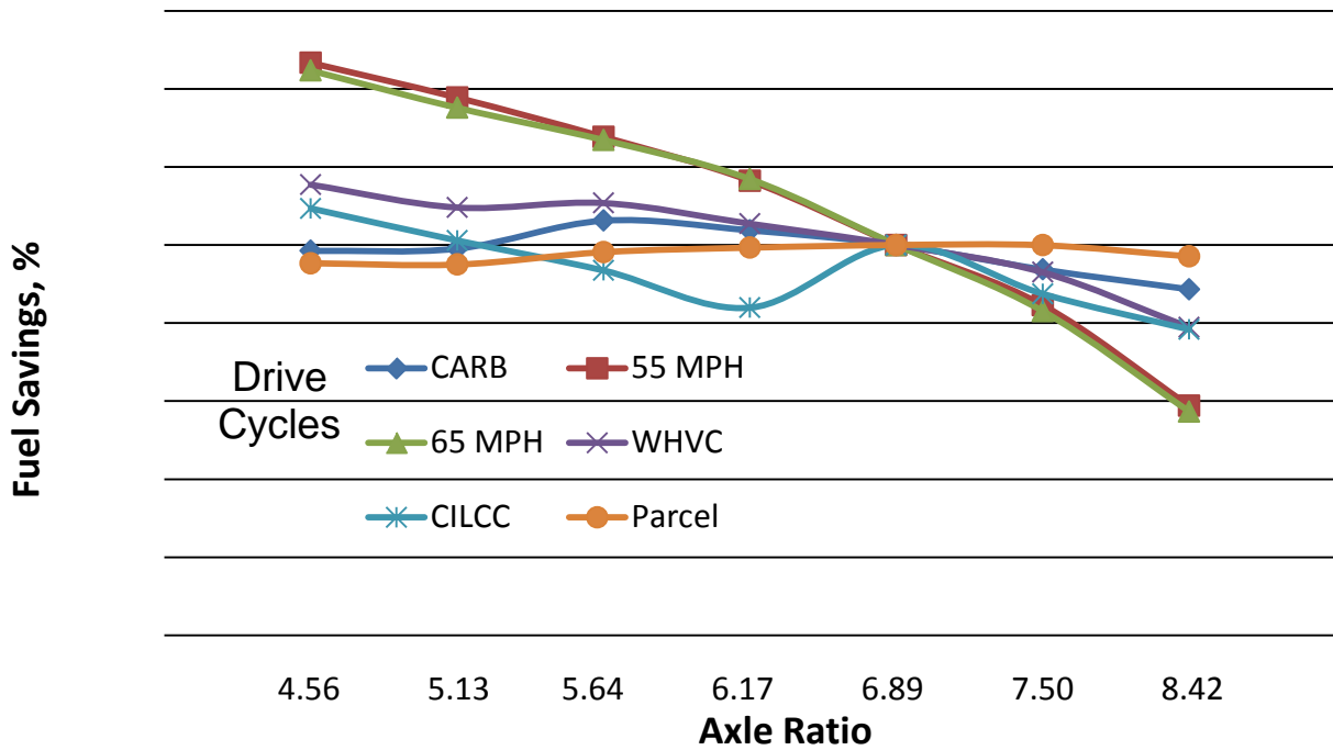
FIGURE 3.12 AXLE RATIO SWEEP ON F-650 WITH THE 6.2 V-8
