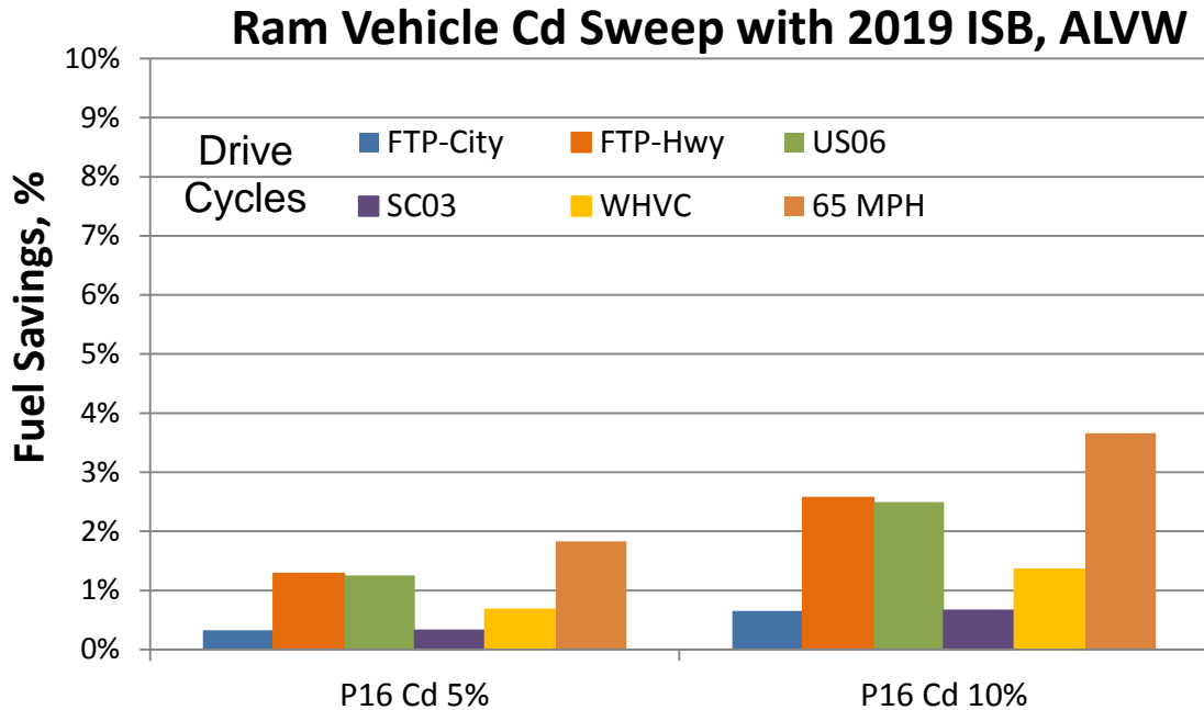
FIGURE 3.3 CD SWEEP OF RAM PICKUP
