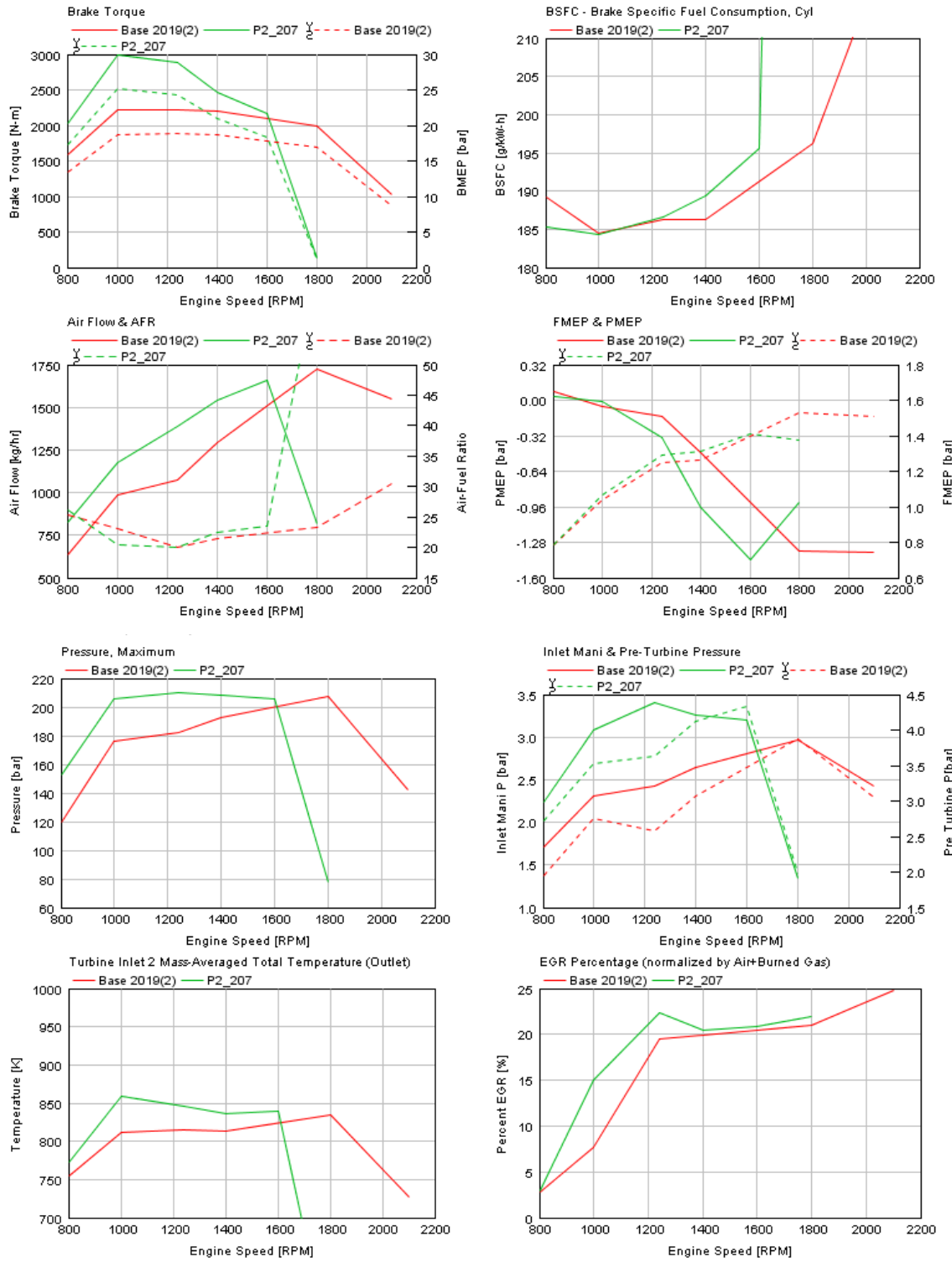
FIGURE B1.3C FULL LOAD PERFORMANCE COMPARISON
