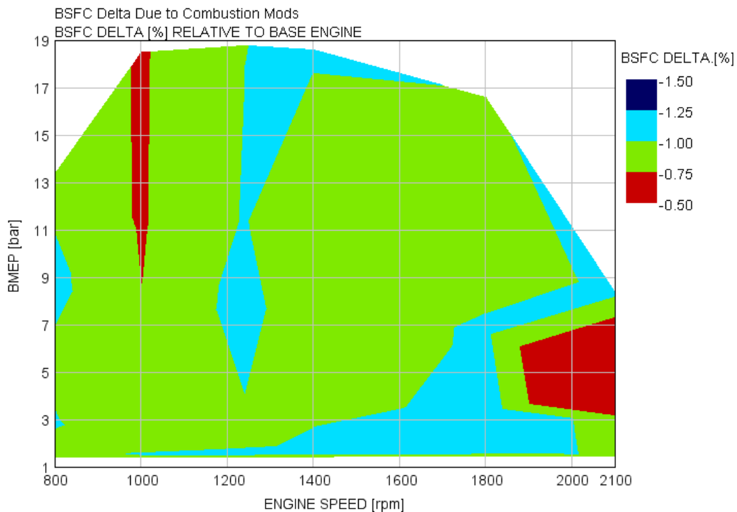
FIGURE B1.1A BSFC IMPROVEMENT DUE TO COMBUSTION MODIFICATION
