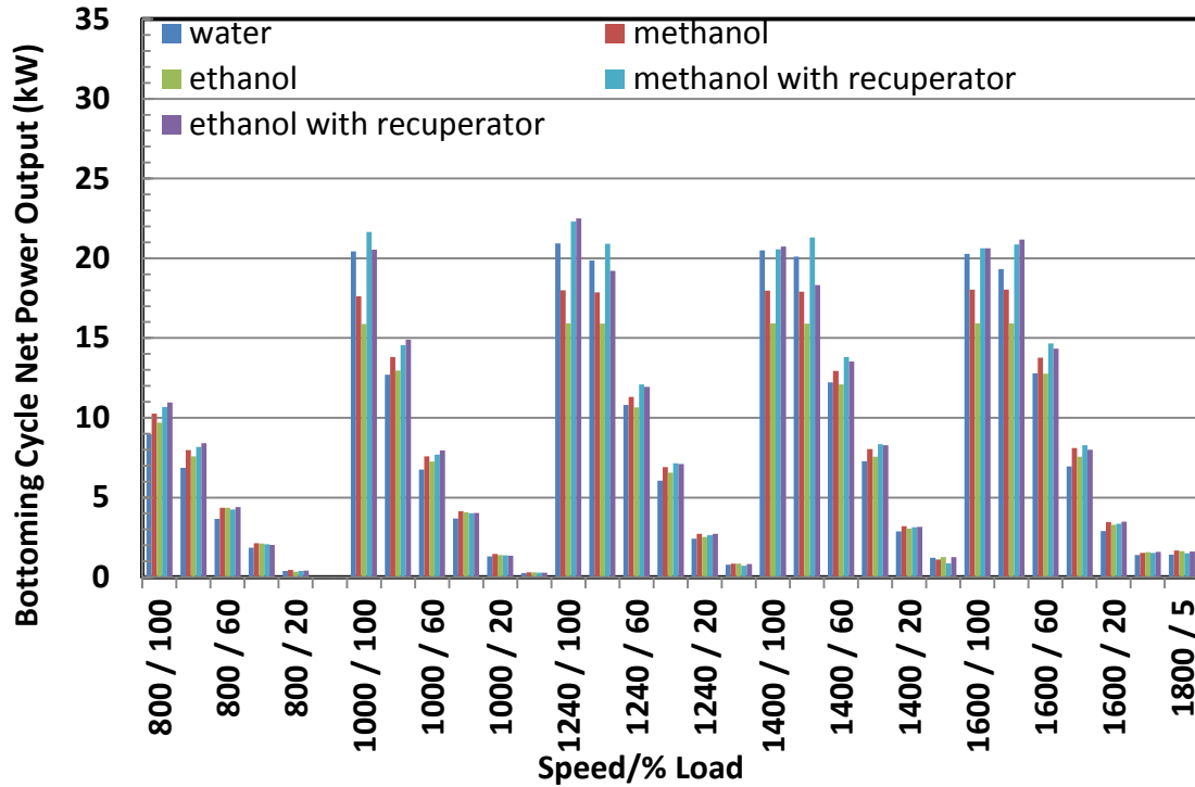
FIGURE B1.4F BC NET POWER OUTPUT FOR METHANOL AND ETHANOL
