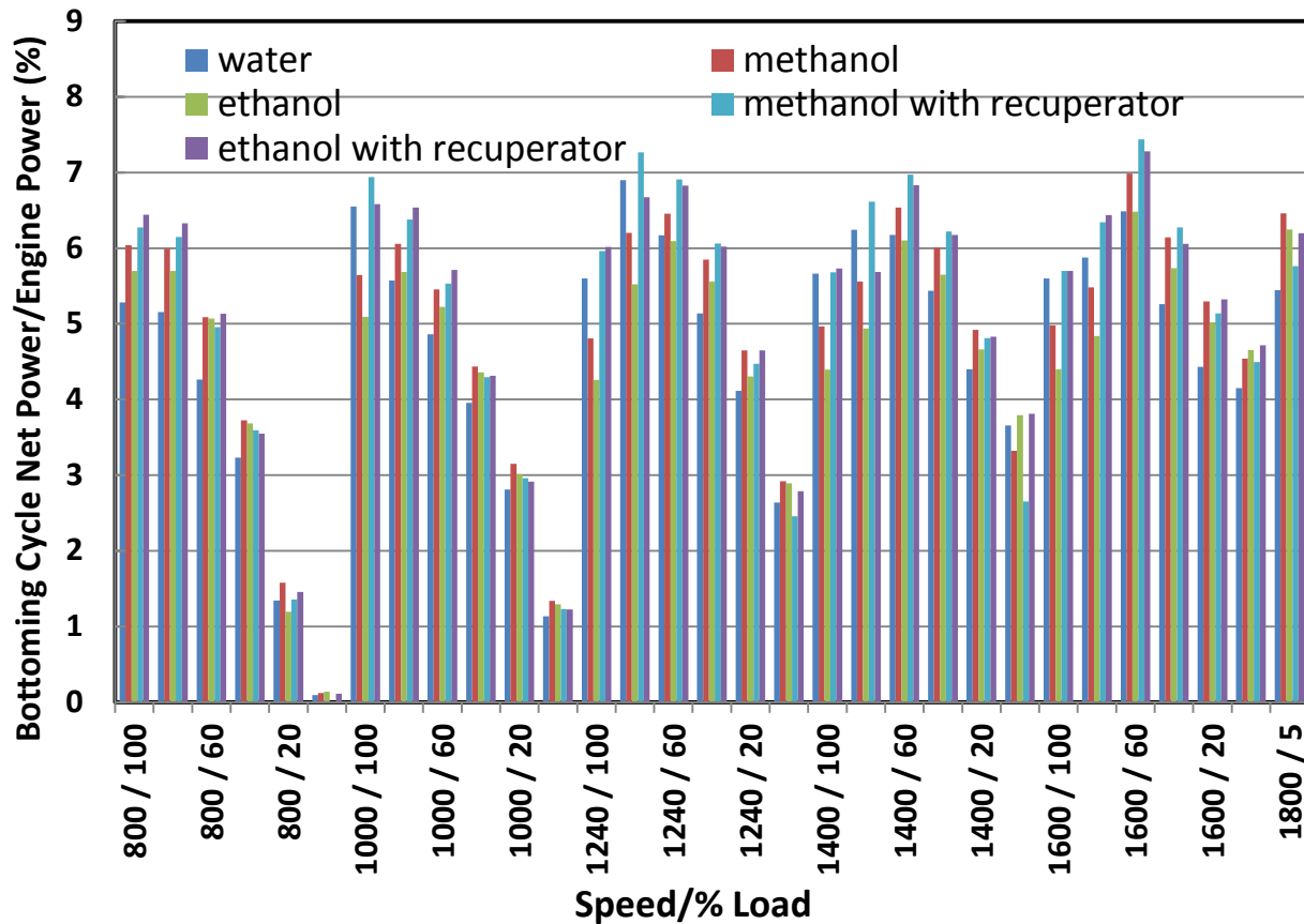
FIGURE X1.4G RATIO OF BC NET POWER TO ENGINE POWER OUTPUT FOR METHANOL AND ETHANOL
