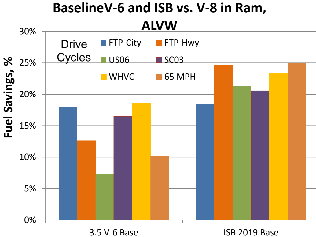
FIGURE 2.22 BASELINE V-6 AND DIESEL VS. V-8 IN RAM AT ALVW
