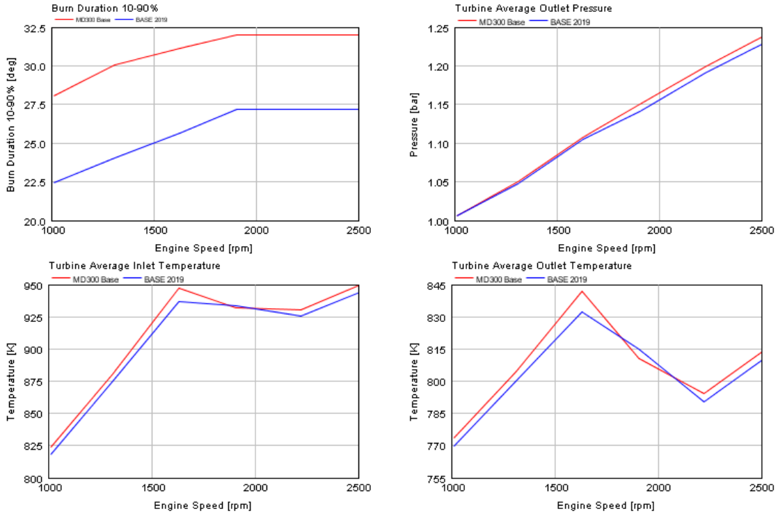
FIGURE B2.1D 2019 BASE ENGINE FULL LOAD COMPARISON
