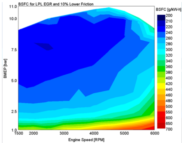
FIGURE A9 COMBINED BSFC MAP
