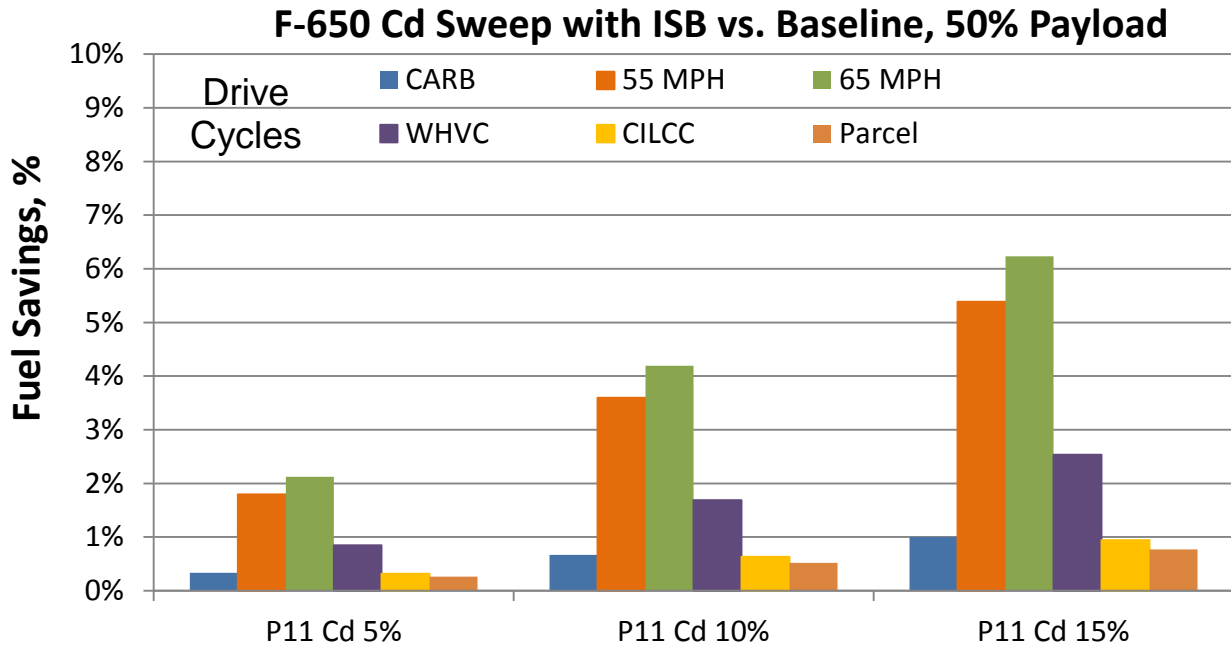
FIGURE 3.1 CD SWEEP OF F-650 TOW TRUCK
