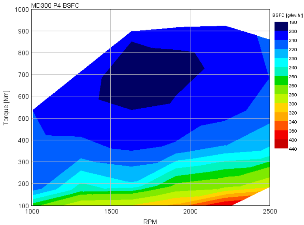
FIGURE B2.5A BSFC MAP OF PACKAGE 9
