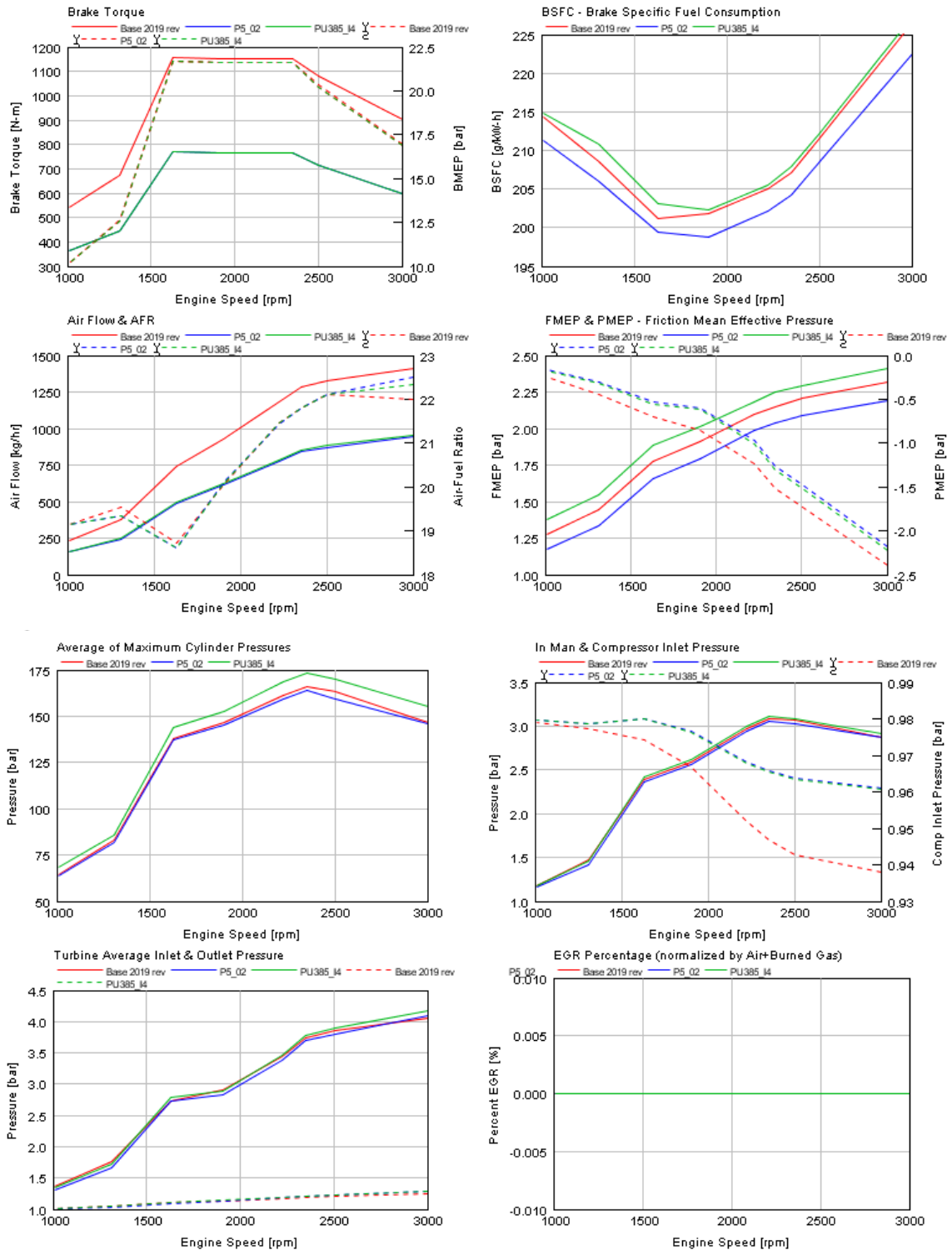
FIGURE B3.6C FULL LOAD PERFORMANCE COMPARISON OF P15
