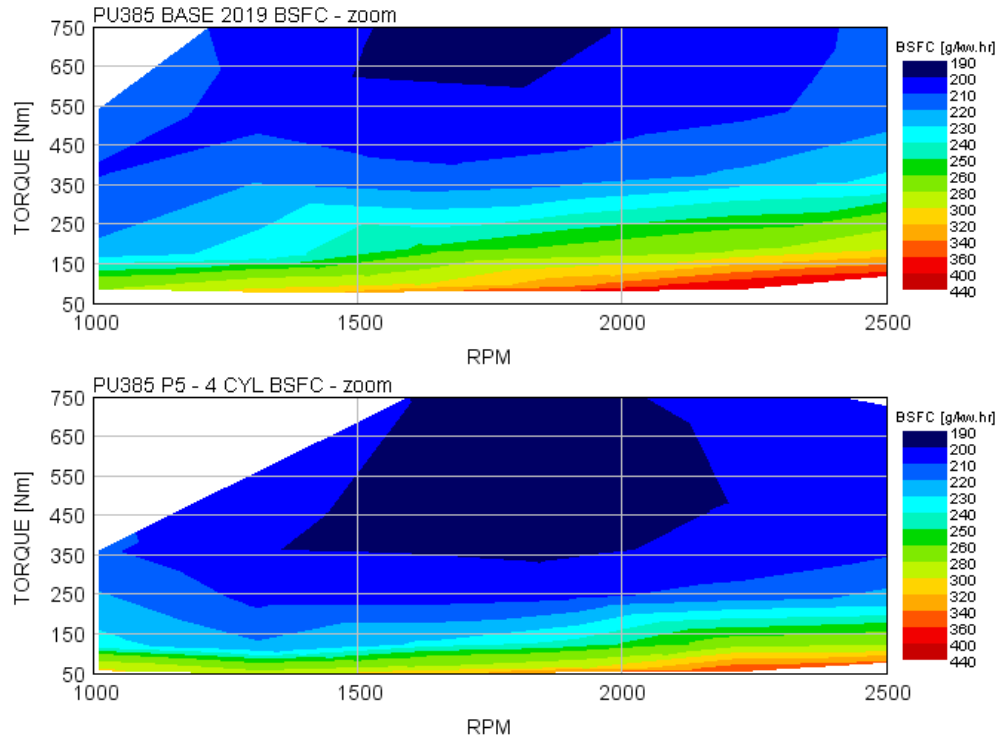
FIGURE B3.6B BSFC COMPARISON P15 I4 – ZOOMED TORQUE
