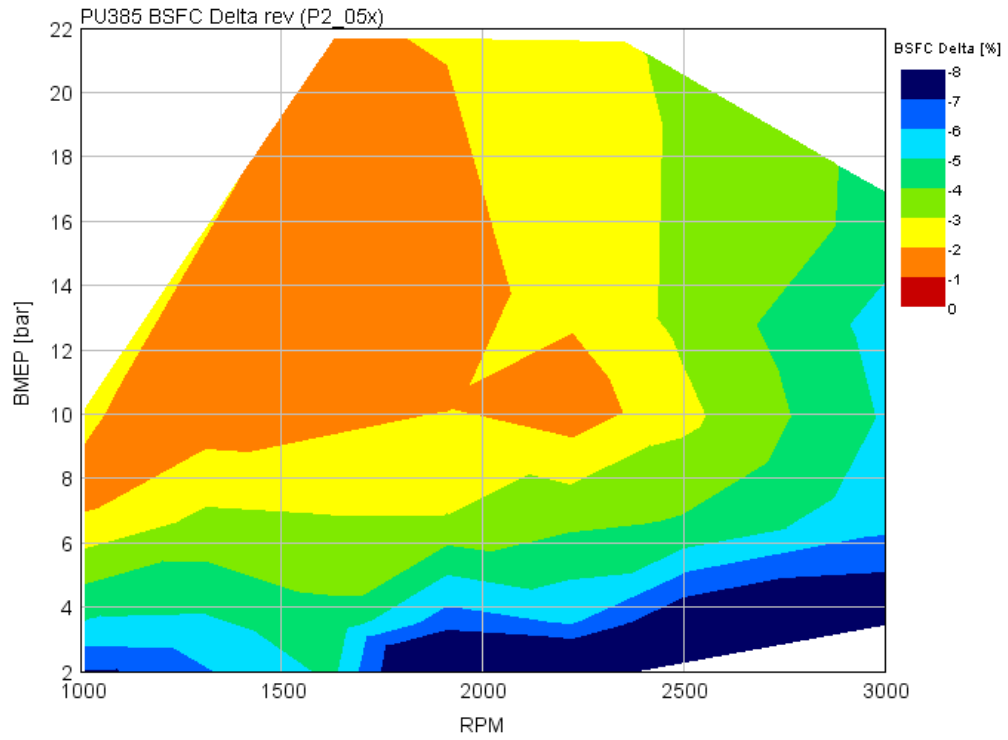
FIGURE B3.3B BSFC IMPROVEMENT MAP OF PACKAGE 12 VS. 2019 BASELINE
