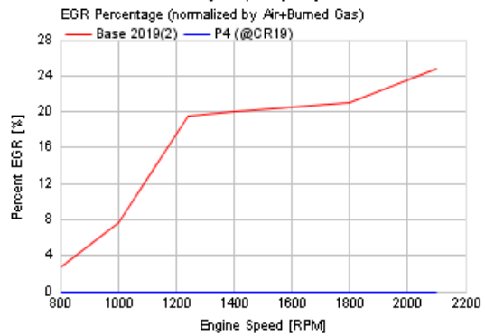
FIGURE B1.5C FULL LOAD PERFORMANCE COMPARISON
