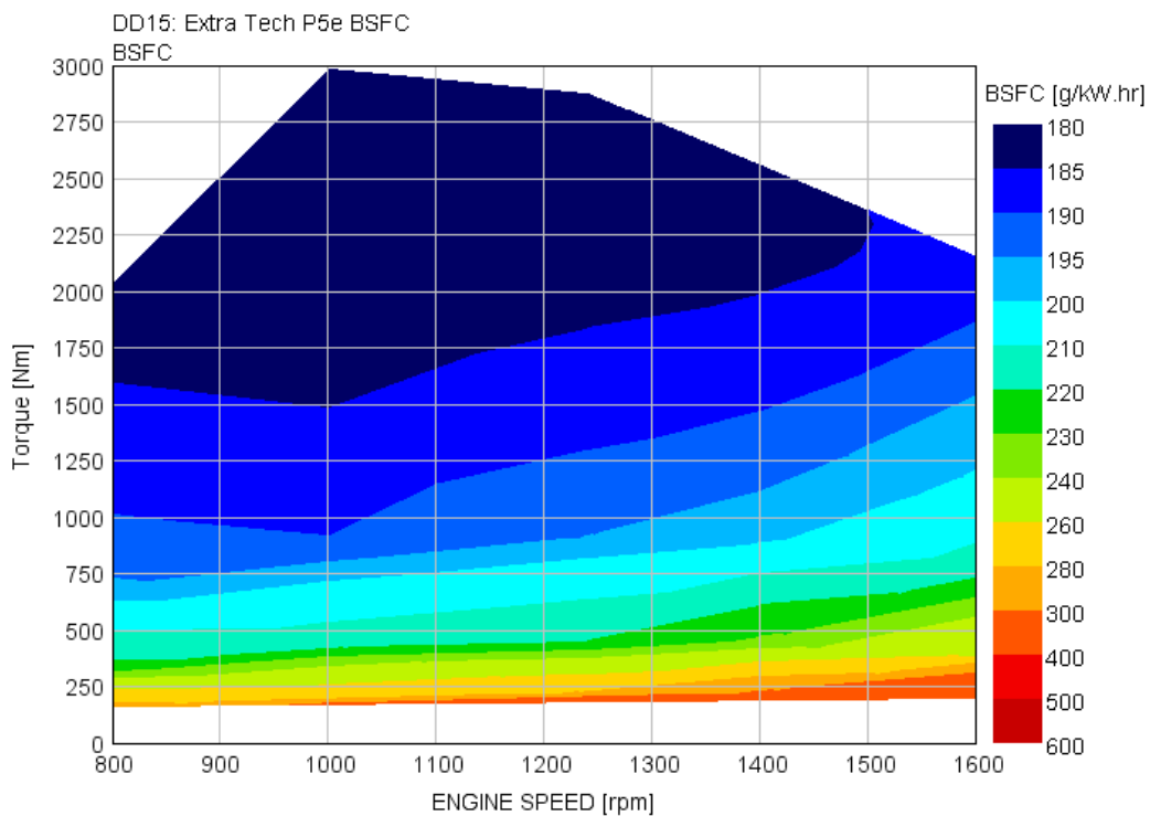
FIGURE B1.6A BSFC MAP OF PACKAGE 5 ENGINE
