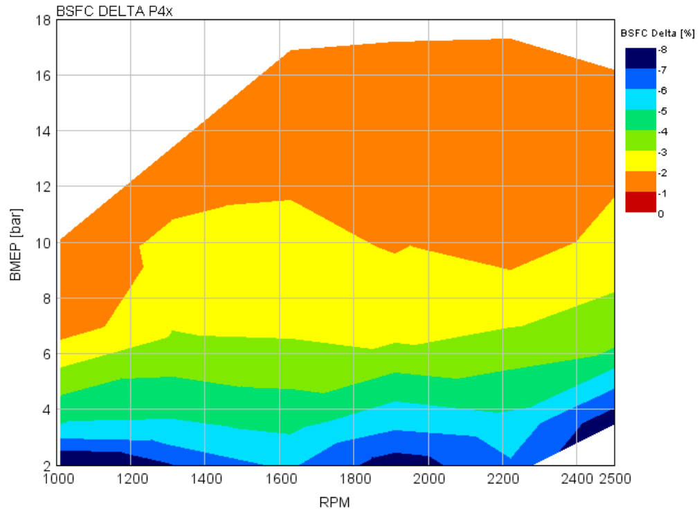
FIGURE B2.5B BSFC IMPROVEMENT MAP OF PACKAGE 9 VS. 2019 BASELINE
