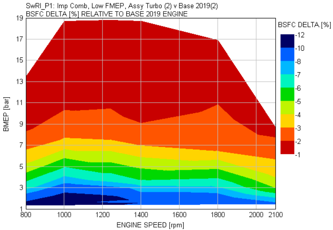
FIGURE B1.2B BSFC IMPROVEMENT MAP OF PACKAGE 1 ENGINE
