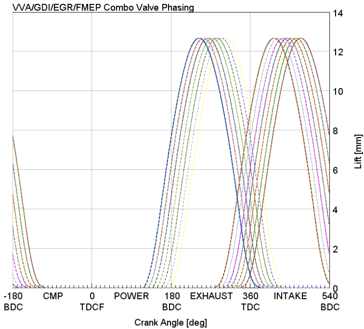
FIGURE A13 6.2L V8 INDEPENDENT CAM PHASING
