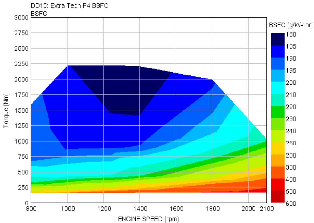
FIGURE B1.5A BSFC MAP OF COMBO PACKAGE 4 ENGINE
