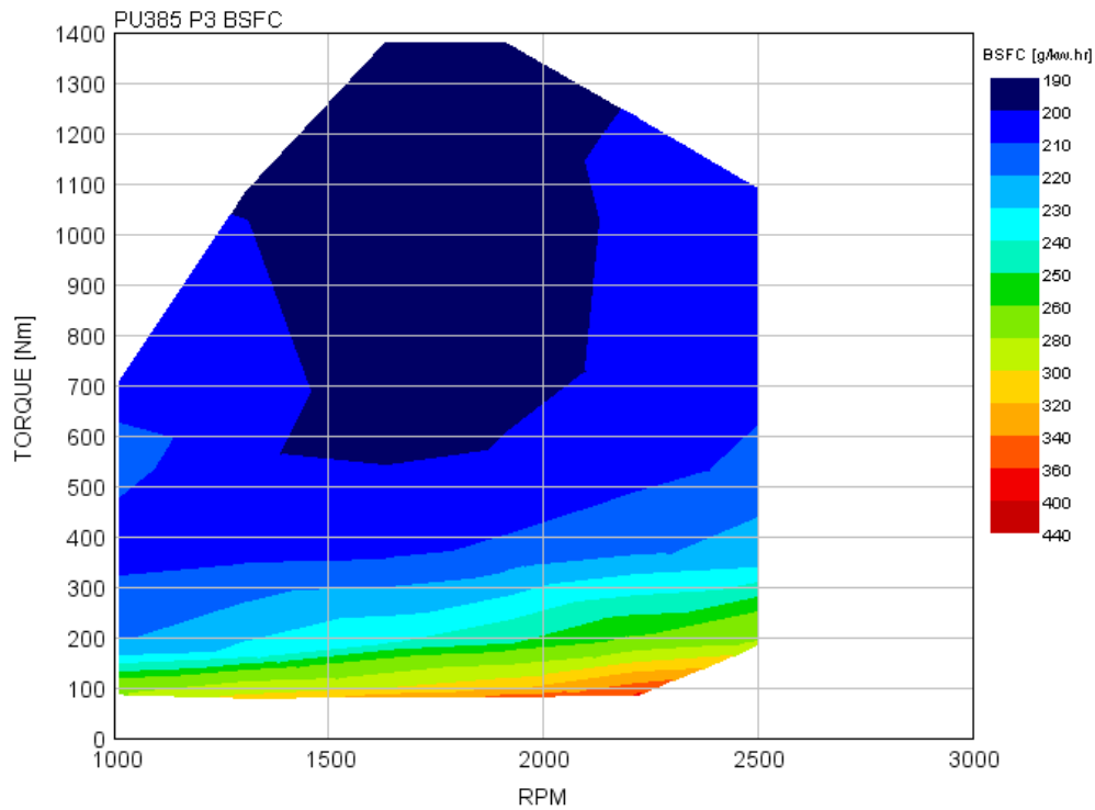
FIGURE B3.4A BSFC MAP OF COMBO PACKAGE 13
