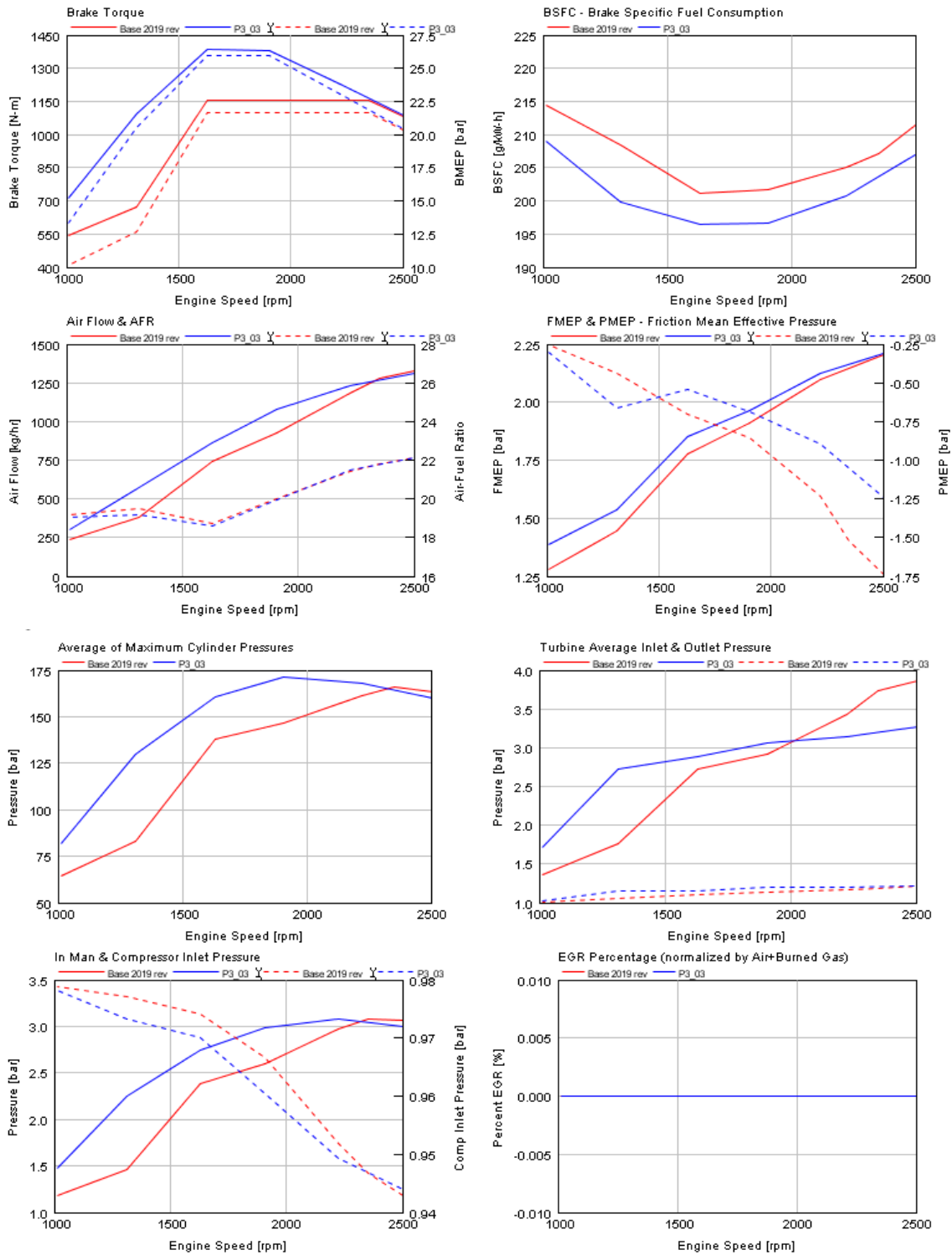
FIGURE B3.4C FULL LOAD PERFORMANCE COMPARISON FOR P13
