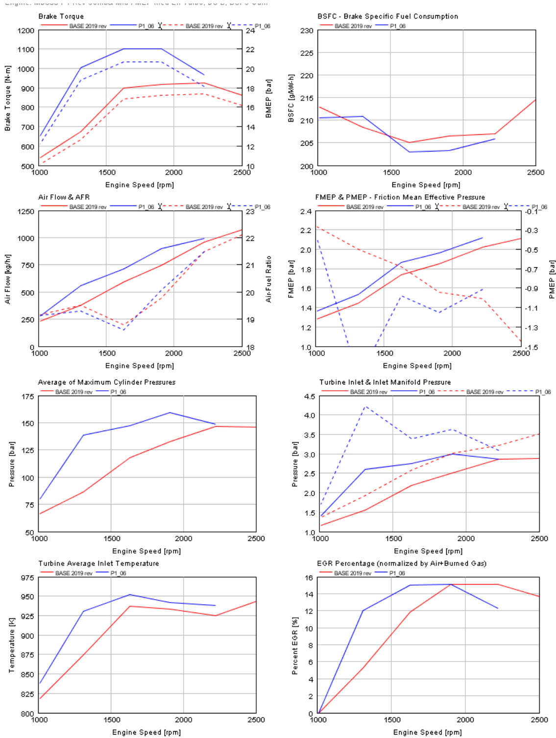
FIGURE B2.2C PACKAGE 6 FULL LOAD PERFORMANCE COMPARISON
