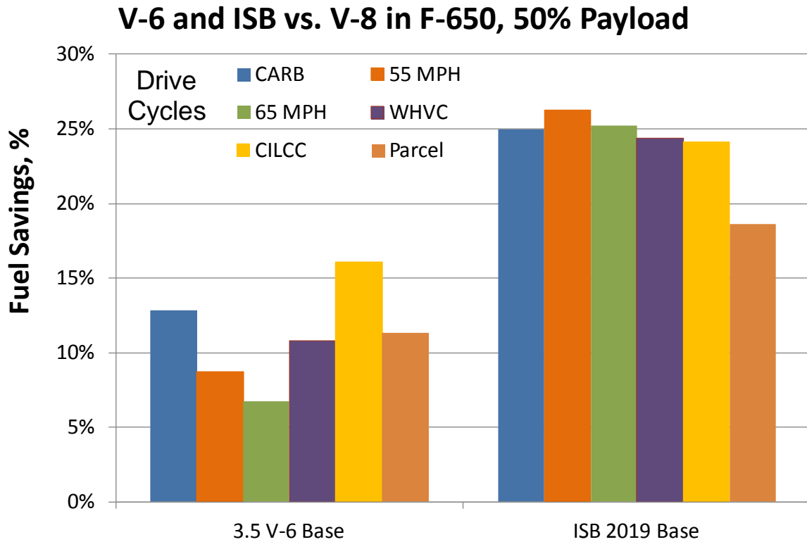
FIGURE 2.7 FUEL CONSUMPTION COMPARISON OF 3.5 V6 AND 2019 DIESEL TO THE V8
