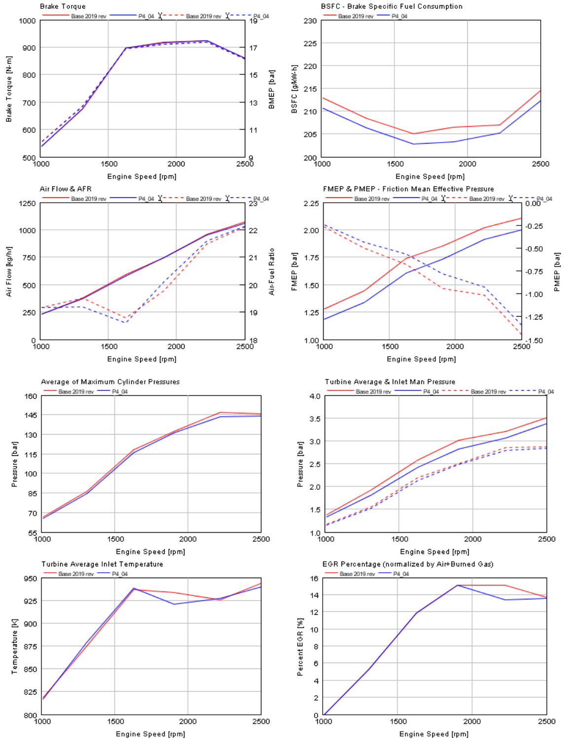
FIGURE B2.5C PACKAGE 9 FULL LOAD PERFORMANCE COMPARISON
