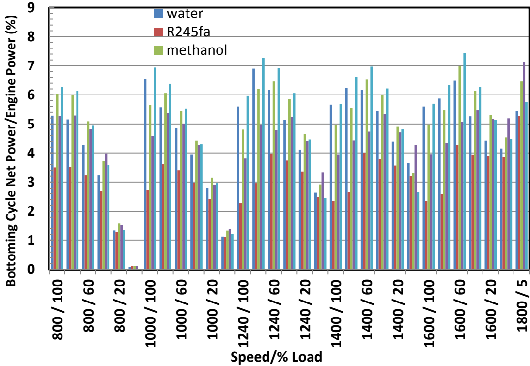
FIGURE B1.4C RATIO OF BOTTOMING CYCLE NET POWER TO ENGINE POWER OUTPUT FOR PACKAGE 3
