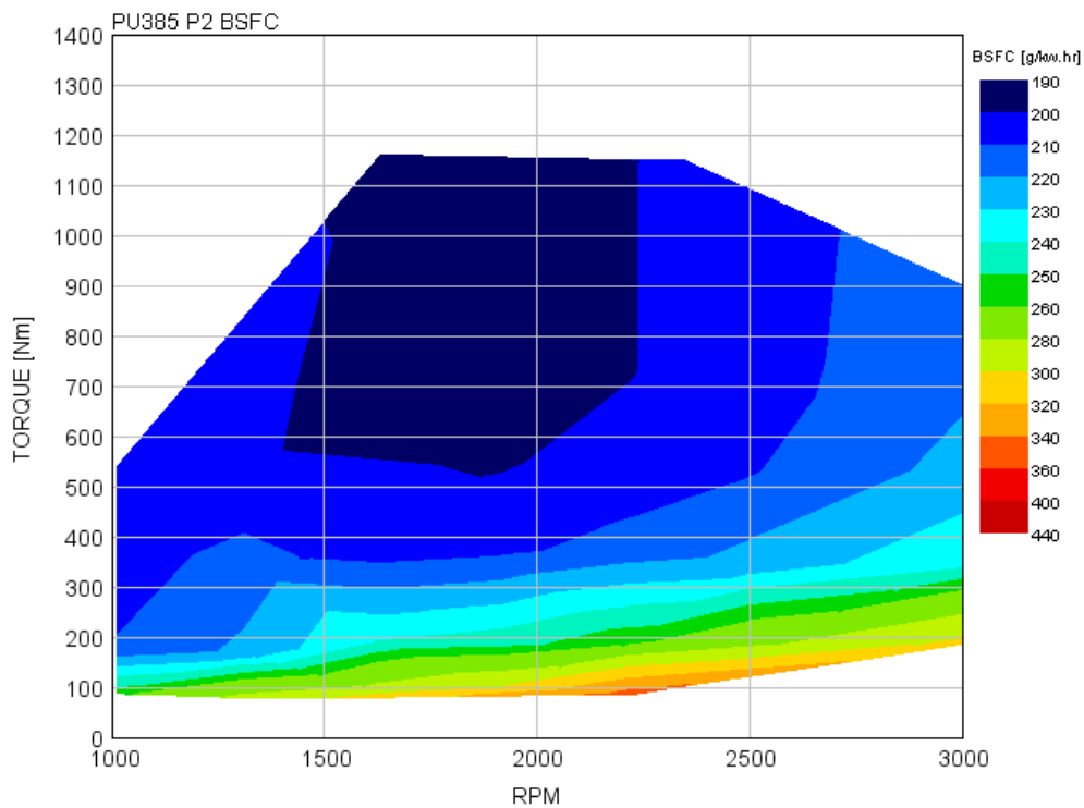
FIGURE B3.3A BSFC MAP OF PACKAGE 12
