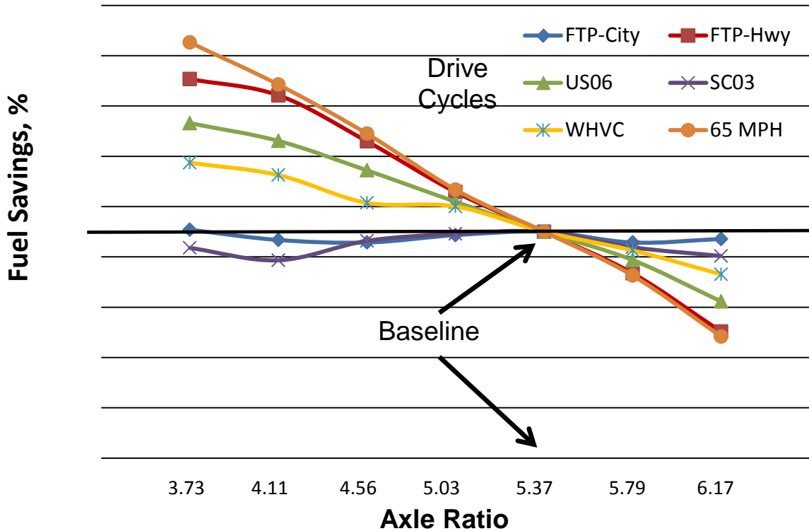
FIGURE 3.18 AXLE RATIO SWEEP ON RAM PICKUP WITH V-8 GASOLINE
