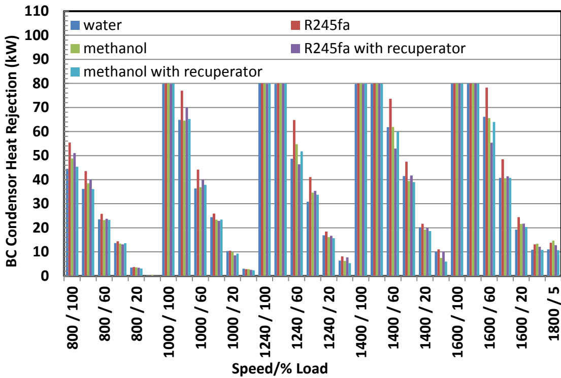
FIGURE B1.4D BOTTOMING CYCLE CONDENSER HEAT TRANSFER FOR PACKAGE 3
