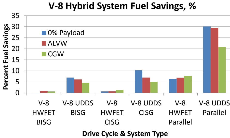
FIGURE D.4 V-8 GASOLINE HYBRID SYSTEM FUEL CONSUMPTION REDUCTION IN PERCENT
