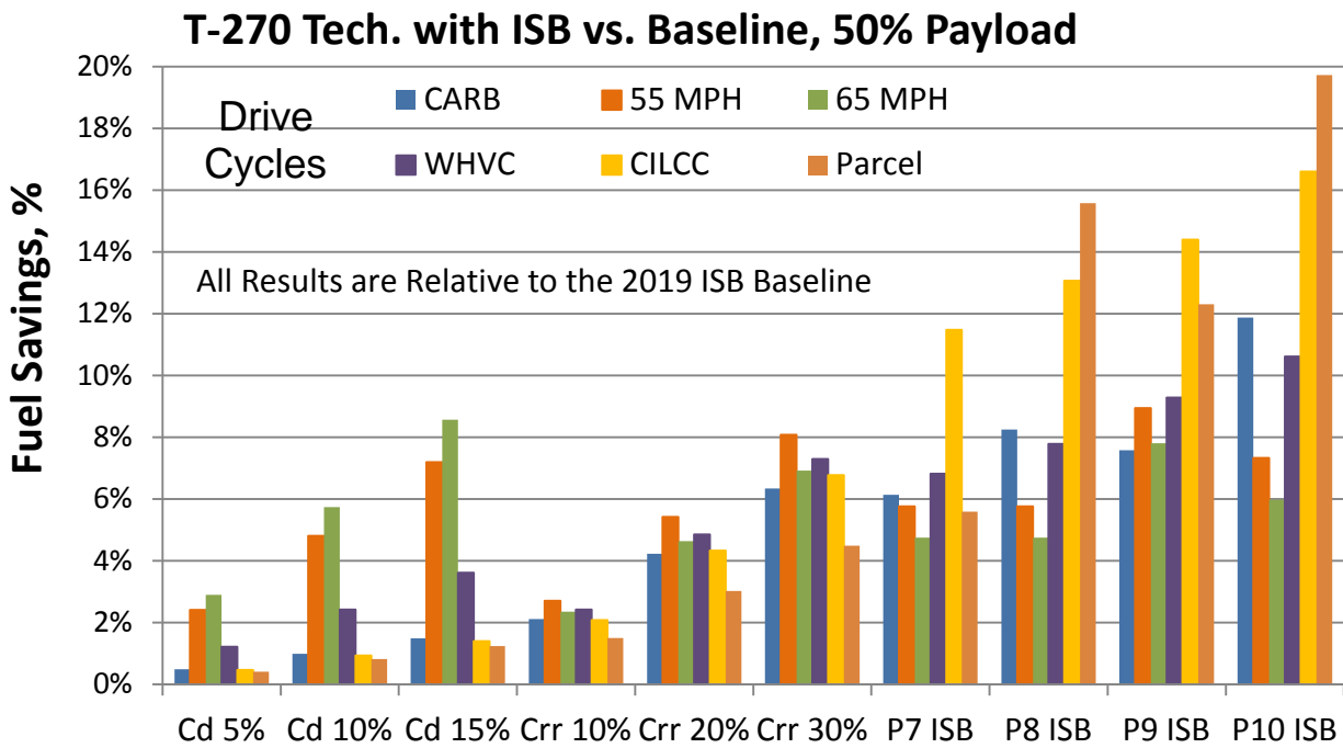
FIGURE 2.17 T270 VEHICLE TECHNOLOGY COMBINATION FUEL SAVINGS RESULTS WITH THE 2019 BASELINE ISB ENGINE. ALL RESULTS ARE RELATIVE TO THE 2019 ISB BASELINE
