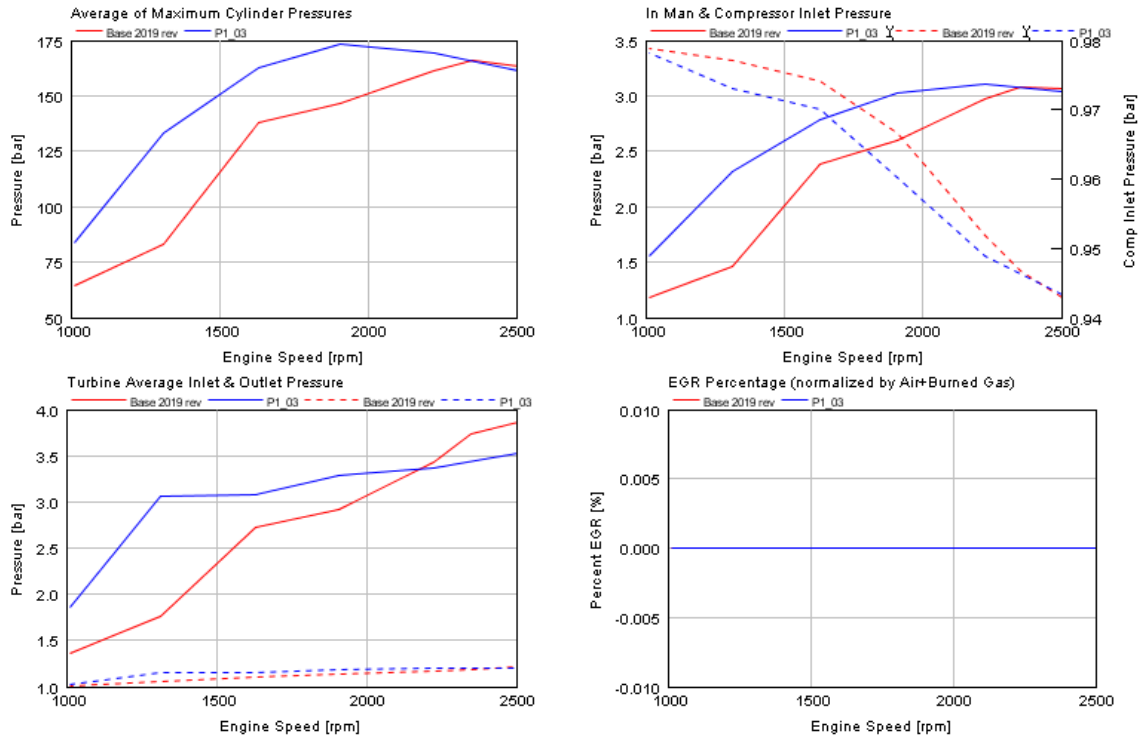
FIGURE B3.2C PACKAGE 11 FULL LOAD PERFORMANCE COMPARISON
