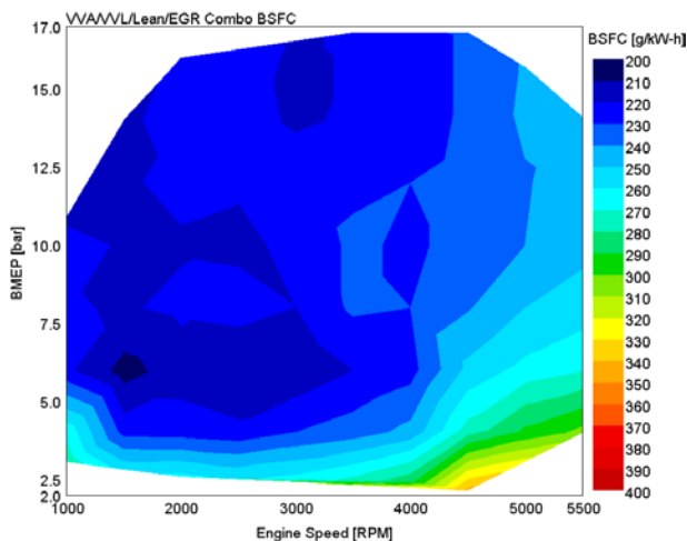
FIGURE A5 COMBINED BSFC MAP
