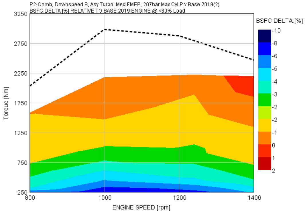
FIGURE B1.3B BSFC IMPROVEMENT MAP OF PACKAGE 2 ENGINE VS. 2019 BASELINE
