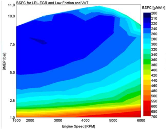
FIGURE A20 PACKAGE 7 COMBINED BSFC MAP
