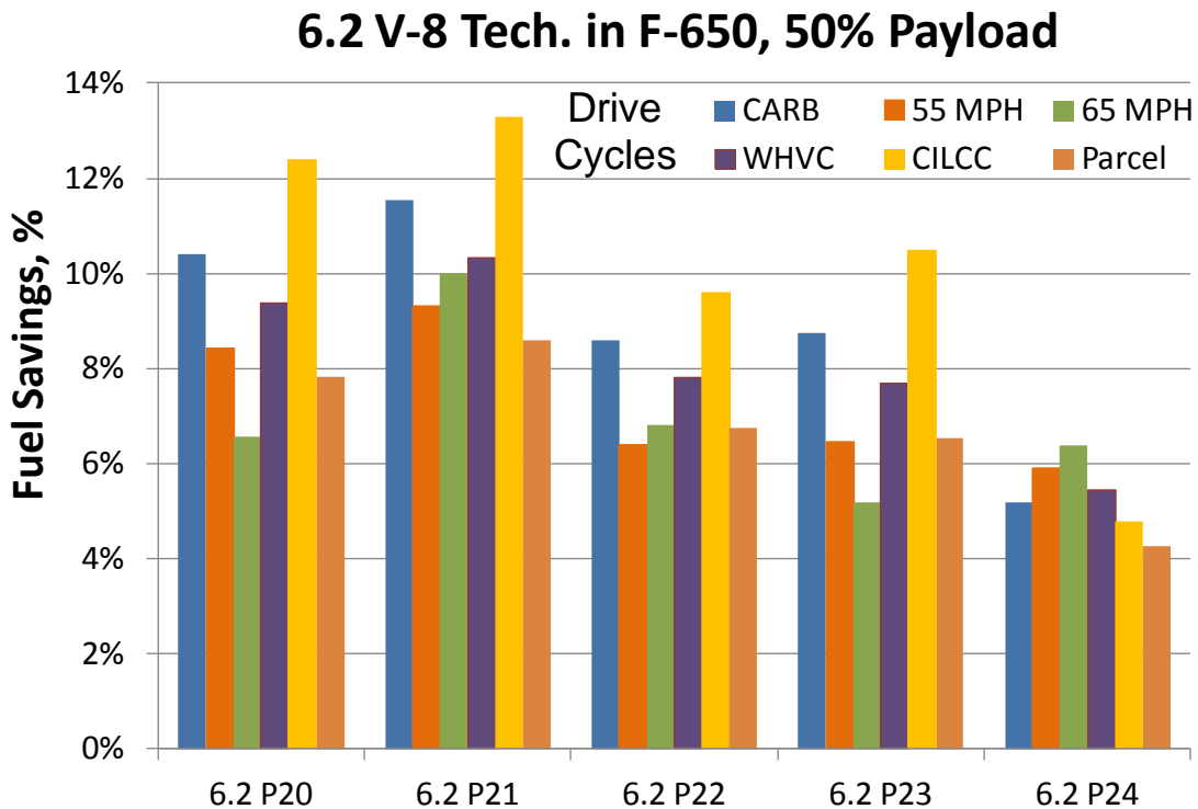
FIGURE 2.6 FUEL SAVING PERFORMANCE OF 6.2 V8 TECHNOLOGY PACKAGES IN THE F-650 TRUCK
