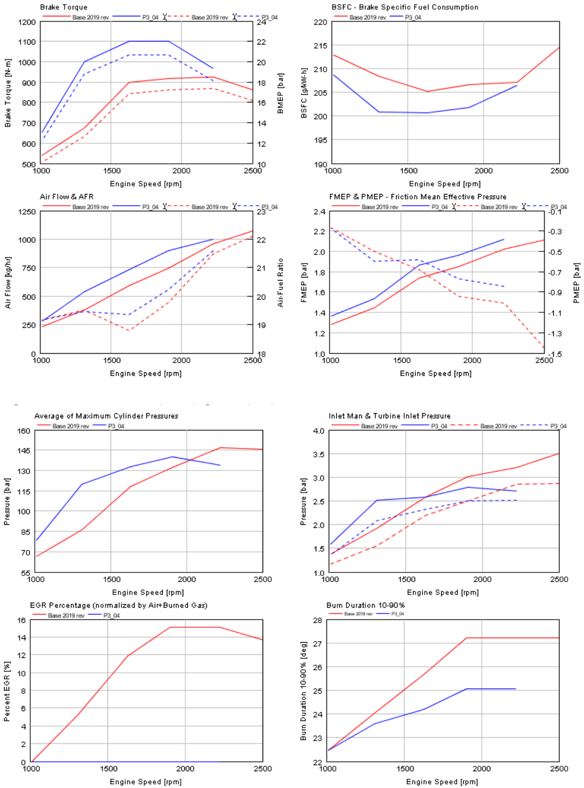
FIGURE B2.4C PACKAGE 8 FULL LOAD PERFORMANCE COMPARISON
