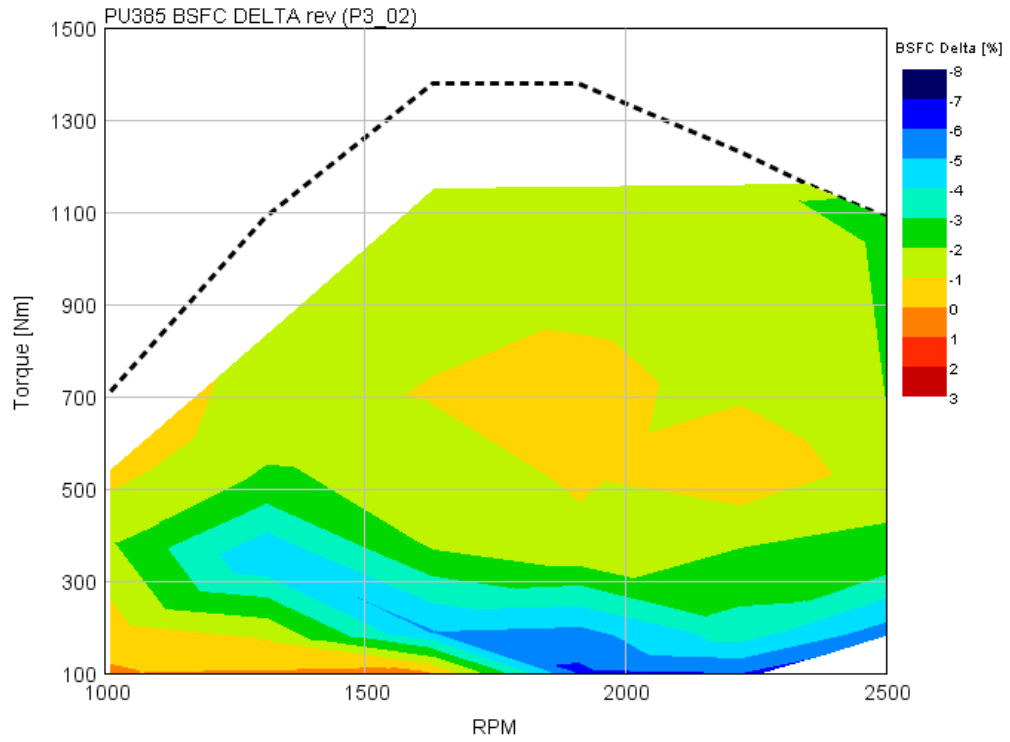
FIGURE B3.4B BSFC IMPROVEMENT OF P13 DOWNSPEED, NO EGR, TURBO EFFICIENCY INCREASE and LIMITED FRICTION REDUCTION
