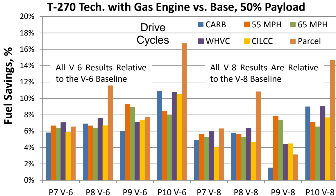
FIGURE 2.18 T270 VEHICLE TECHNOLOGY COMBINATION FUEL SAVINGS WITH BASELINE GASOLINE ENGINES. ALL RESULTS ARE RELATIVE TO THE BASELINE FOR EACH ENGINE
