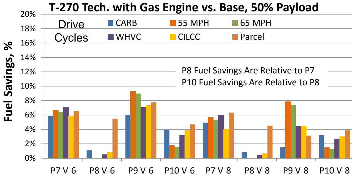
FIGURE 2.16 T270 TECHNOLOGY COMBO FUEL SAVINGS RESULTS WITH BASE GASOLINE ENGINES
