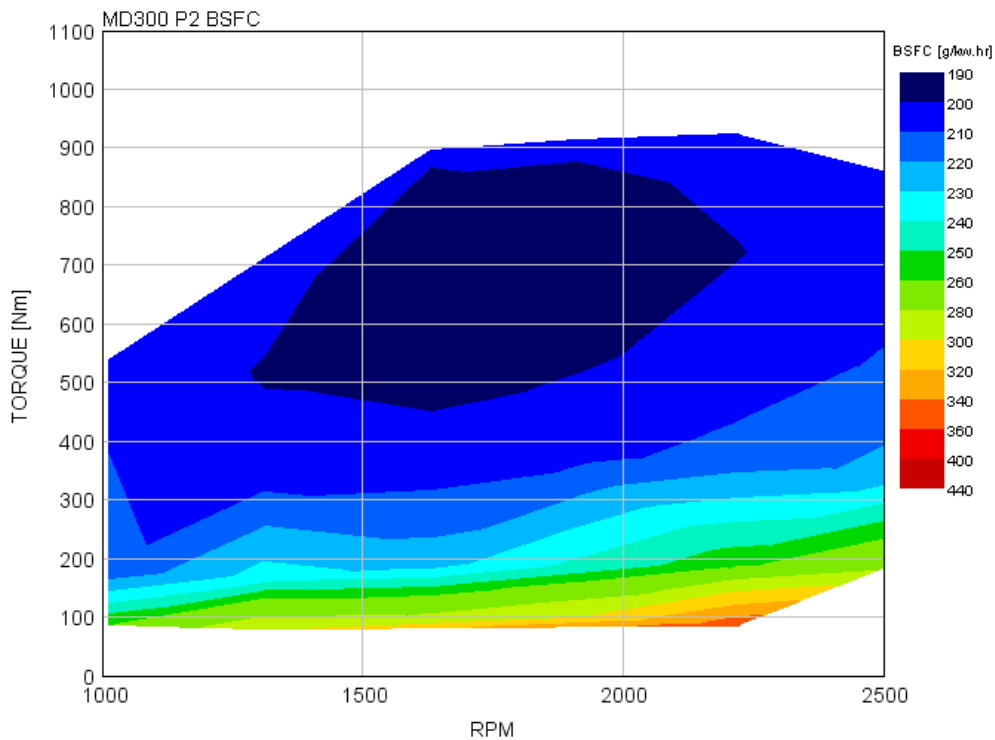
FIGURE B2.3A BSFC MAP OF COMBO PACKAGE 7
