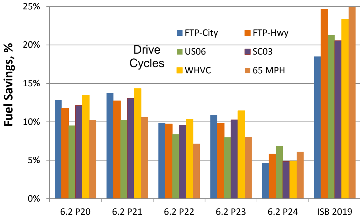
FIGURE 2.21 6.2 V-8 TECHNOLOGY COMBINATIONS IN THE RAM PICKUP
