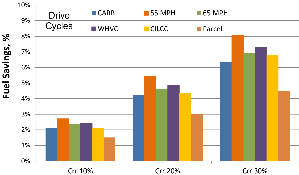
FIGURE 3.5 CRR SWEEP OF THE T270 DELIVERY TRUCK
