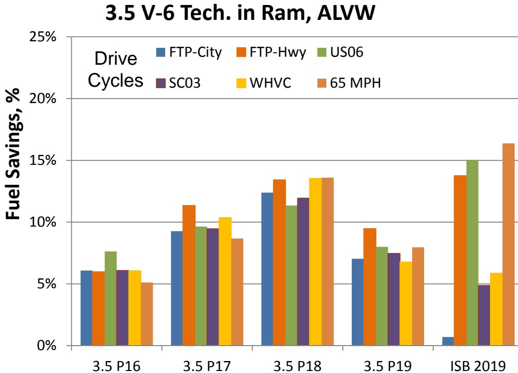
FIGURE 2.20 3.5 V6 TECHNOLOGY COMBINATIONS IN THE RAM PICKUP
