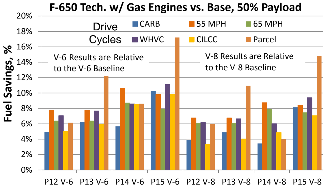
FIGURE 2.11 F-650 VEHICLE TECHNOLOGY COMBINATION FUEL SAVINGS WITH BASELINE GASOLINE ENGINES. ALL RESULTS ARE RELATIVE TO THE BASELINE FOR EACH ENGINE
