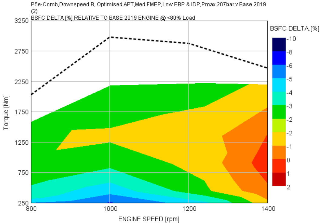
FIGURE B1.6B BSFC IMPROVEMENT MAP OF PACKAGE 5 ENGINE VS. 2019 BASELINE
