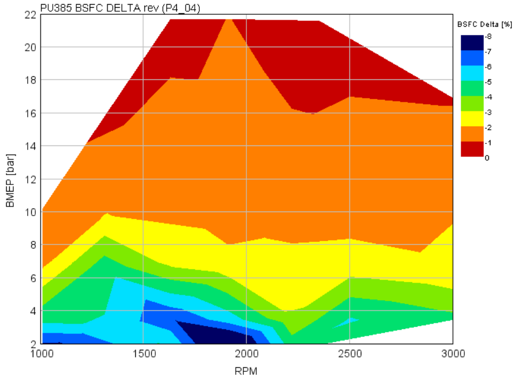
FIGURE B3.5B BSFC IMPROVEMENT 2.5% TURBINE AND COMPRESSOR EFFICIENCY INCREASE (P14)
