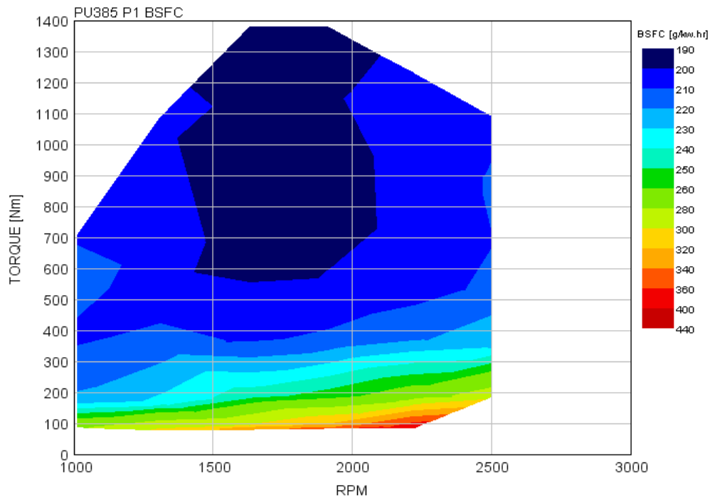
FIGURE B3.2A BSFC MAP OF COMBO PACKAGE 11
