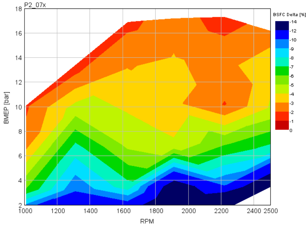
FIGURE B2.3B BSFC IMPROVEMENT MAP OF COMBO PACKAGE 7 VS. 2019 BASELINE
