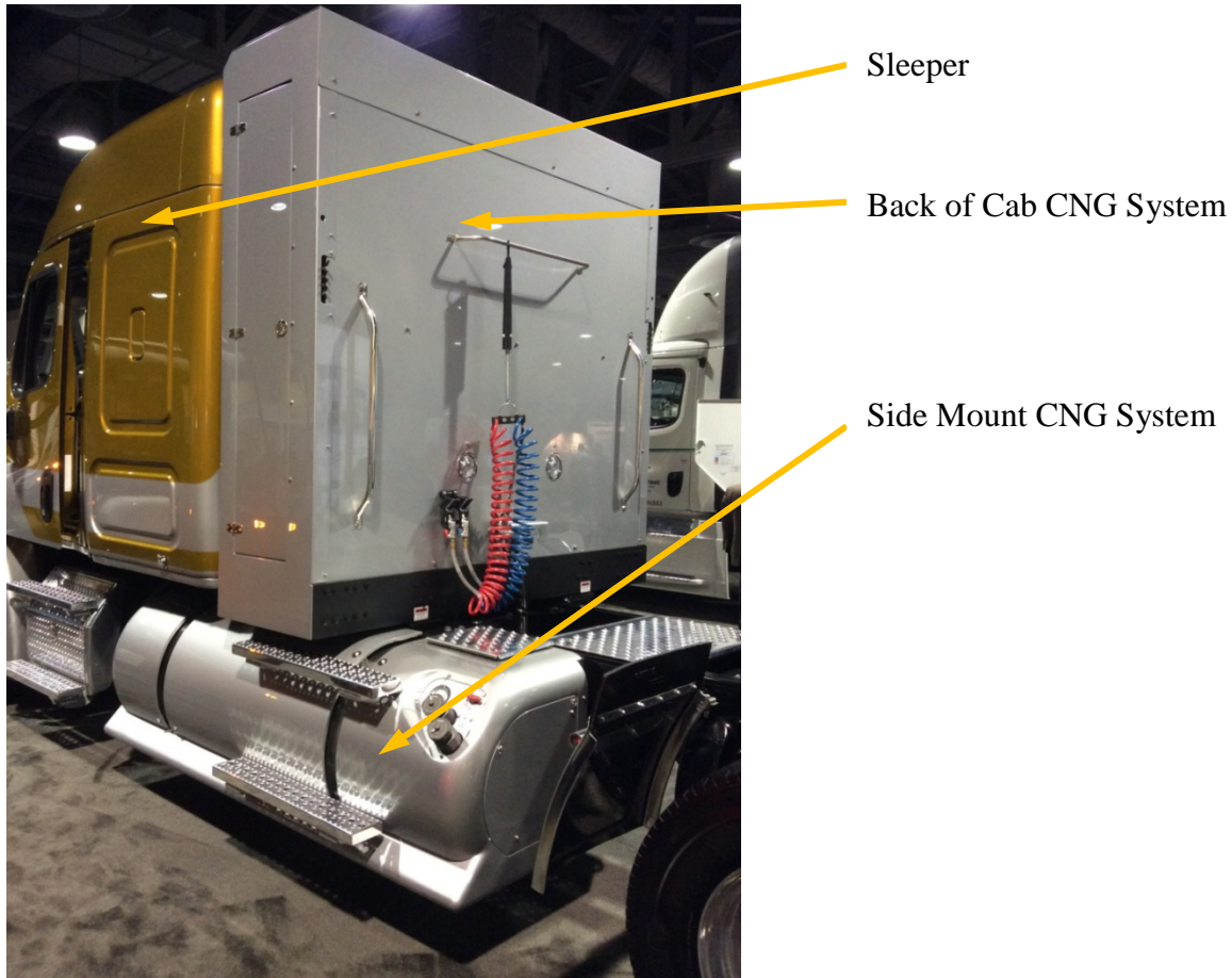
FIGURE 5.2 A 100 DGE BACK OF CAB SYSTEM, COMBINED WITH A 40 DGE SIDE MOUNT SYSTEM, ON A SLEEPER CAB TRACTOR
