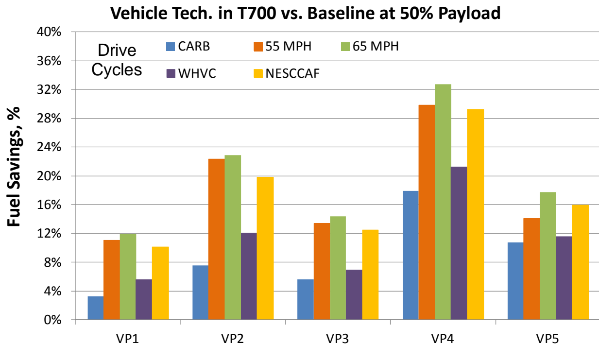
FIGURE 2.3 T700 VEHICLE TECHNOLOGY COMBINATION FUEL SAVINGS RESULTS
