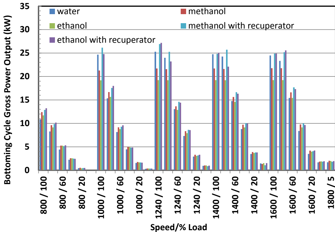
FIGURE B1.4E BC GROSS (TURBINE MECHANICAL) POWER OUTPUT FOR METHANOL AND ETHANOL
