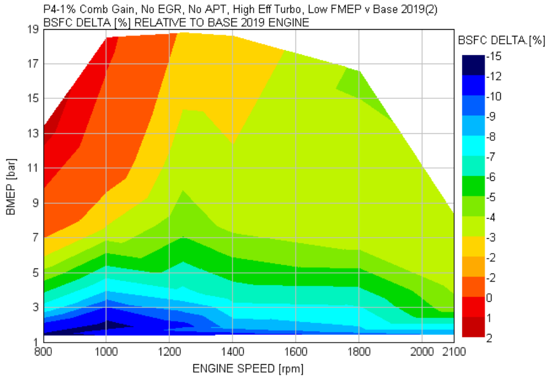
FIGURE B1.5B BSFC IMPROVEMENT MAP OF COMBO PACKAGE 4 ENGINE VS. THE 2019 BASELINE
