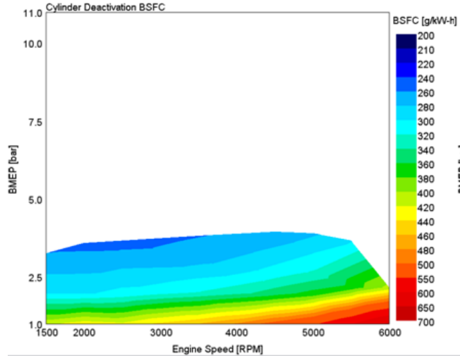
FIGURE A16 CYL. DEACT BSFC MAP
