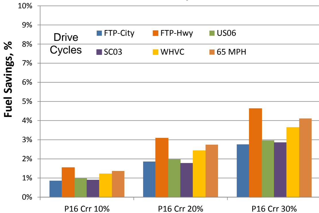
FIGURE 3.6 CRR SWEEP OF THE RAM PICKUP
