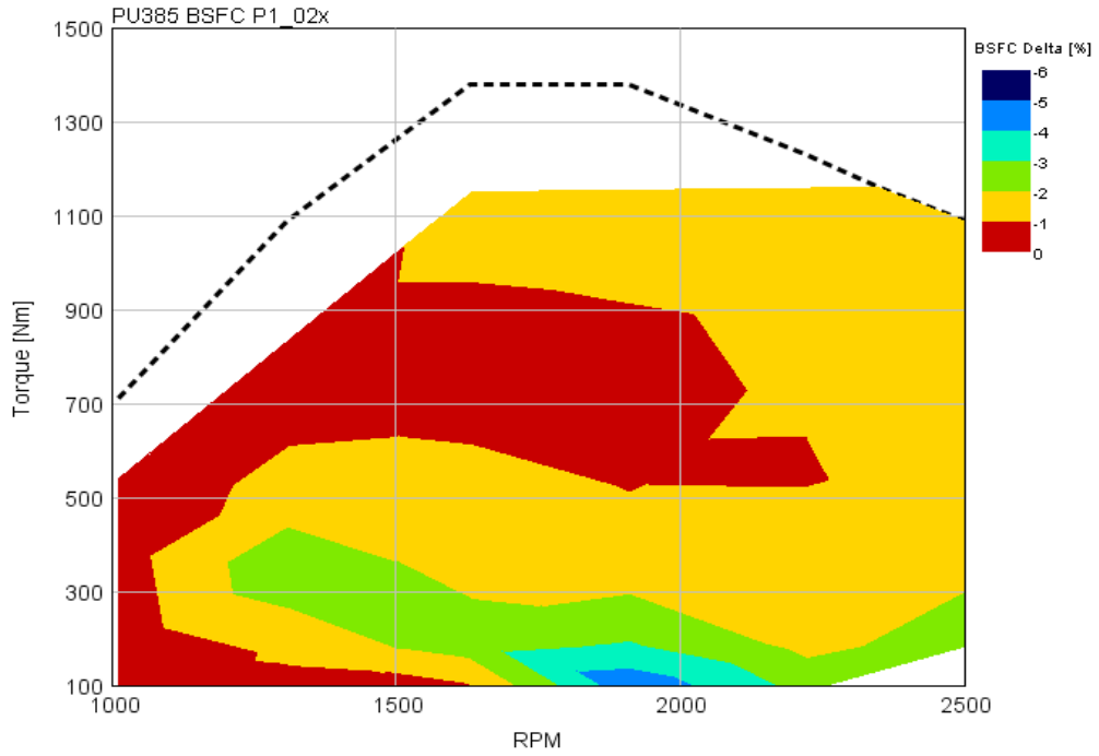
FIGURE B3.2B BSFC IMPROVEMENT MAP OF COMBO PACKAGE 11 VS. THE 2019 BASELINE
