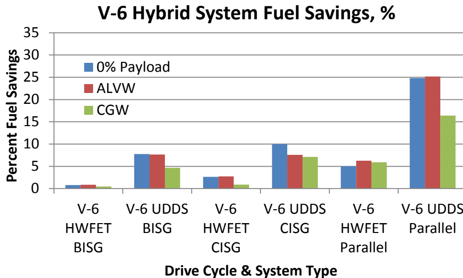
FIGURE D.3 V-6 GASOLINE HYBRID SYSTEM FUEL CONSUMPTION REDUCTION IN PERCENT
