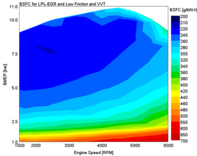
FIGURE A14 PACKAGE 4 COMBINED BSFC MAP
