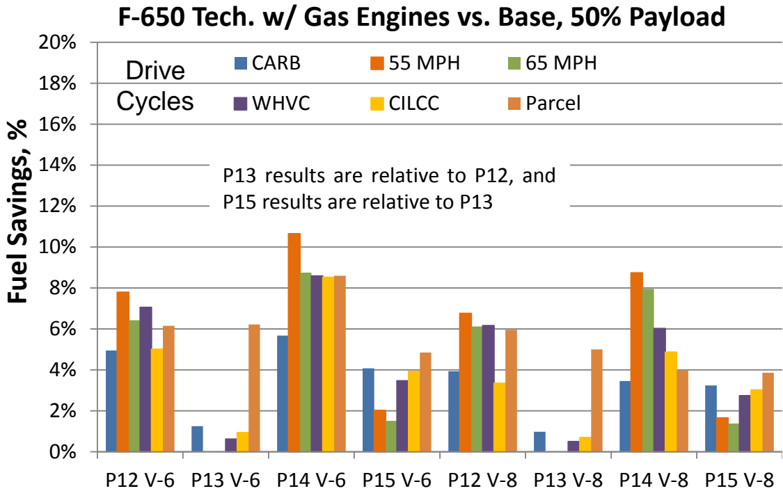
FIGURE 2.9 F-650 TECHNOLOGY COMBO FUEL SAVINGS RESULTS WITH BASE GASOLINE ENGINES
