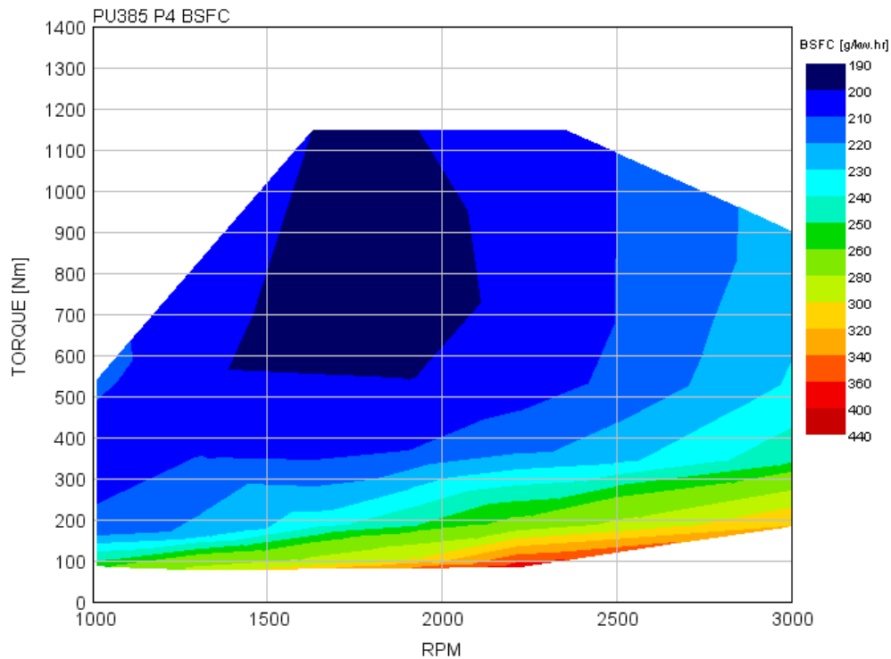
FIGURE B3.5A BSFC OF 2.5% TURBINE and COMPRESSOR EFFICIENCY INCREASE (P14)
