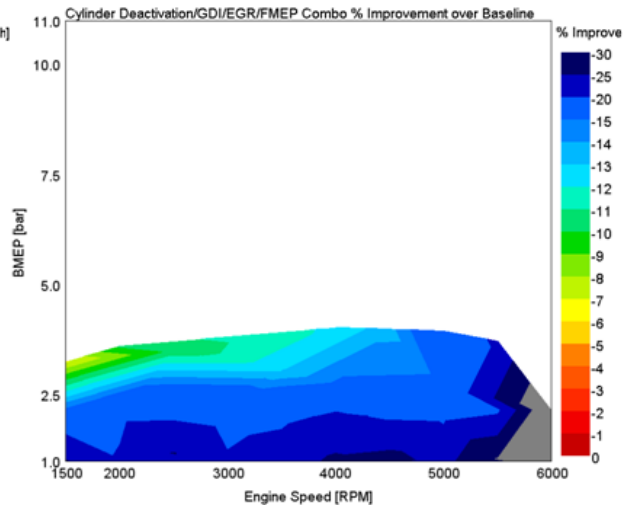
FIGURE A8 BSFC IMPROVEMENT OVER BASELINE
