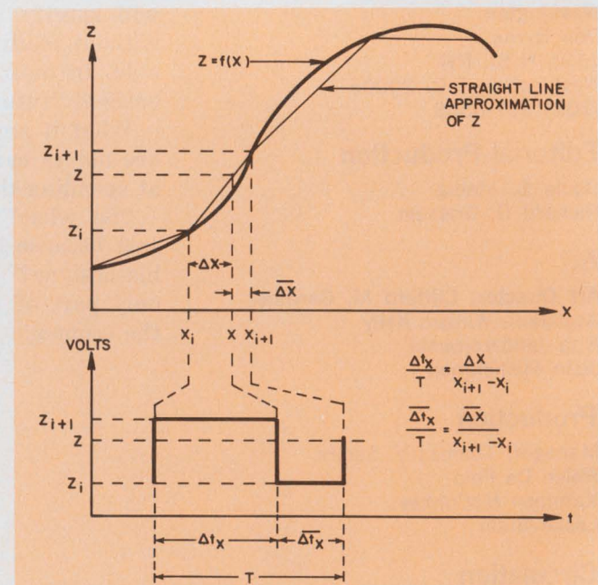
1. The approximate output, Z , is obtained by time-averaging Z_i and Z_{i+1} for intervals that are proportional to \Delta X and \Delta X . The timing diagram (bottom) relates \Delta X and \Delta X to \Delta t_x and \Delta t_x .
