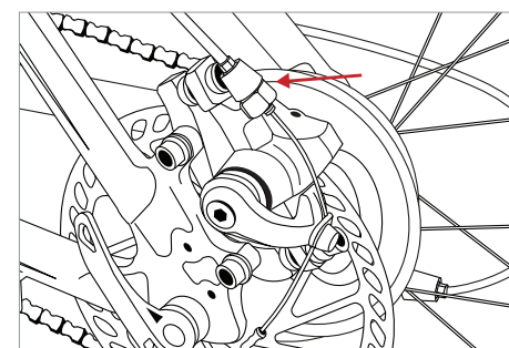
Barrel adjuster on rear brake
