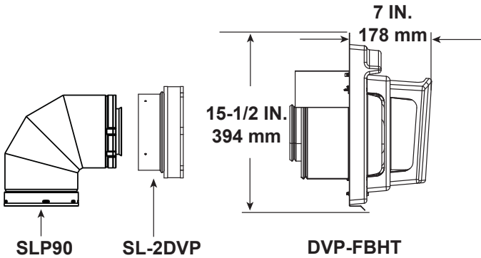
Figure 16.4 SLP Series Vent Components
