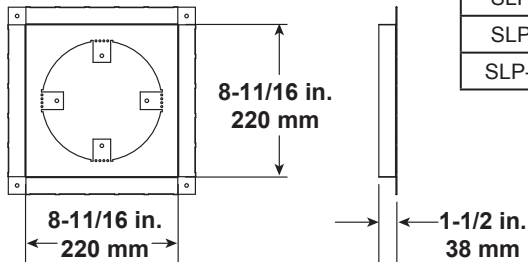
SLP-FS Ceiling Firestop
