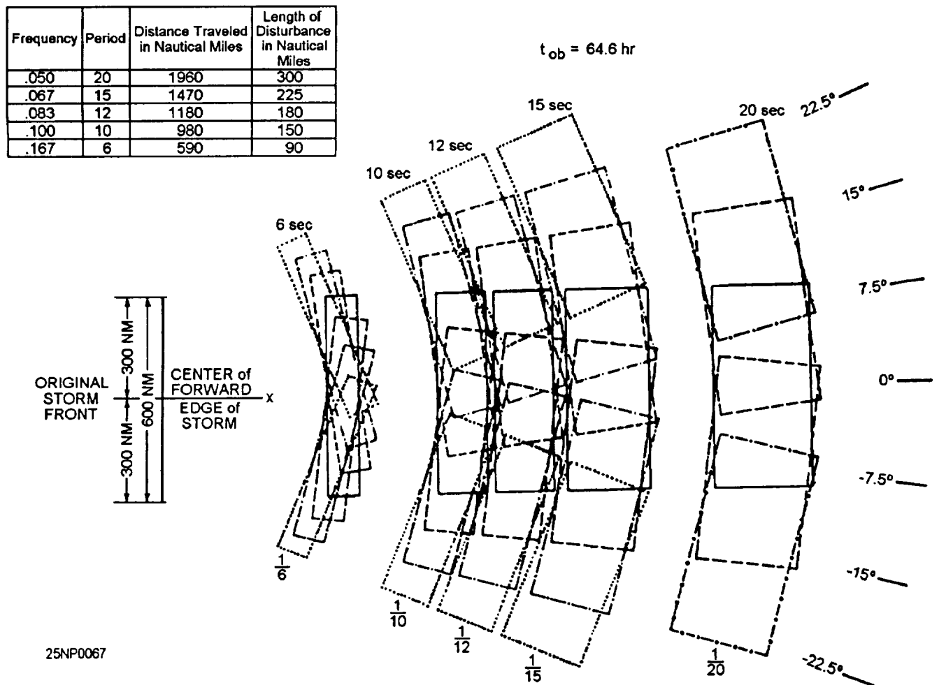
Figure 6-6.-Angular spreading.
