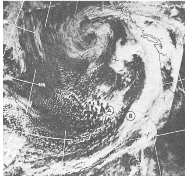
Figure 3-2.-Frontal wave development.
