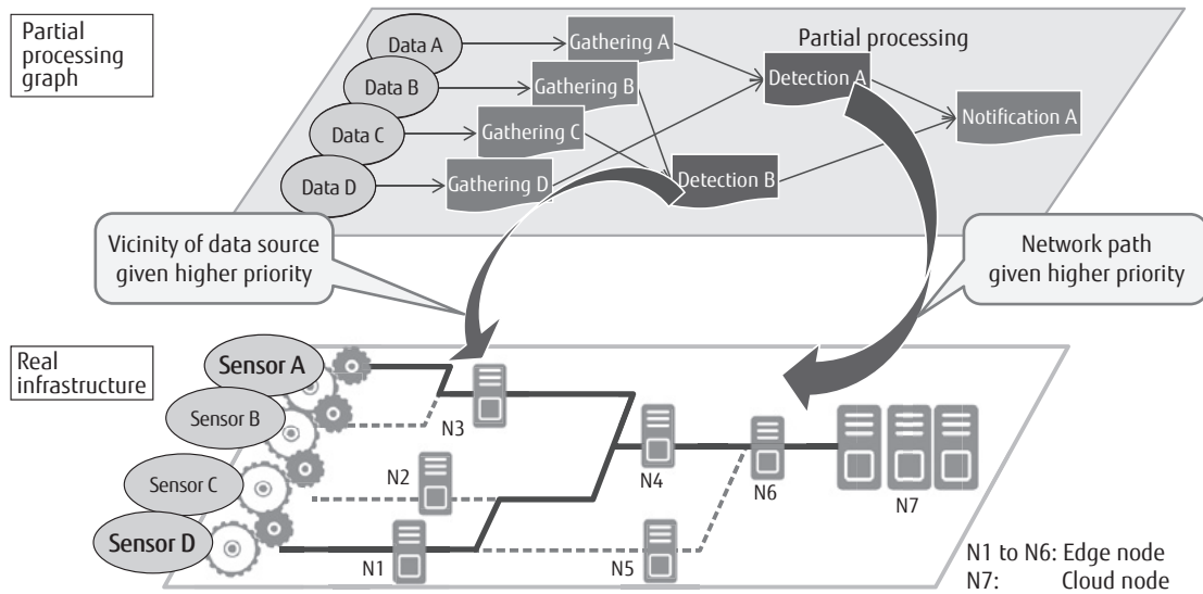
Figure 5 Refining search for partial process execution locations.
