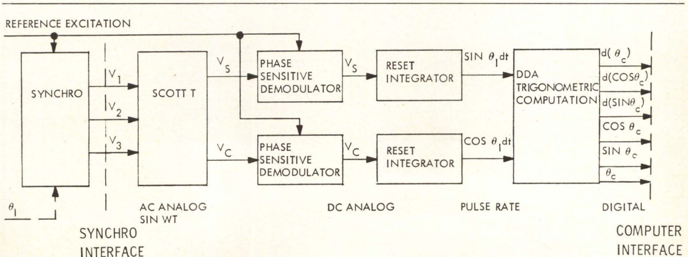
Fig. 3 Alternative mechanization of the solid-state synchro to digital converter.
