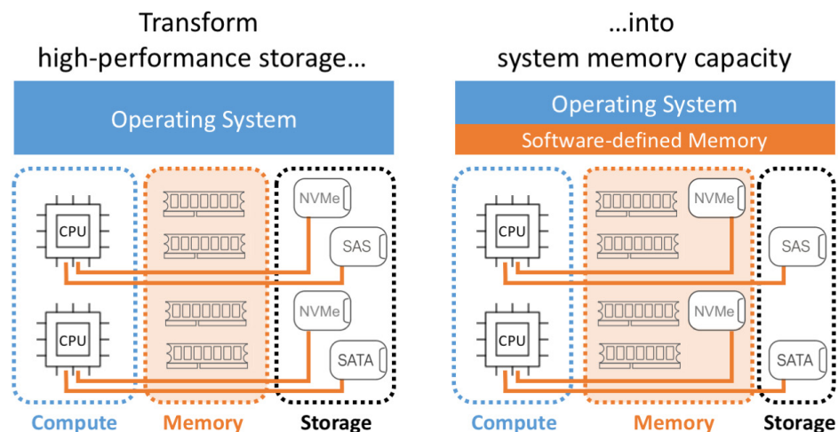
Figure 1-1. Block Diagram of the Ultrastar Memory Drive
