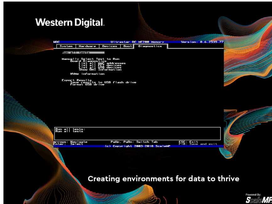
Figure 3-15. Diagnostics Tab
