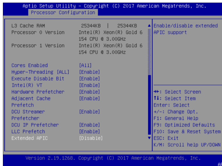
Figure 2-4. Intel Virtualization Technology Configuration
