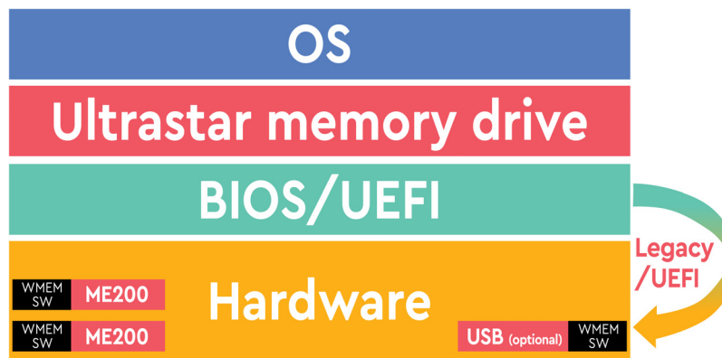
Figure 2-1. Preloaded Software
