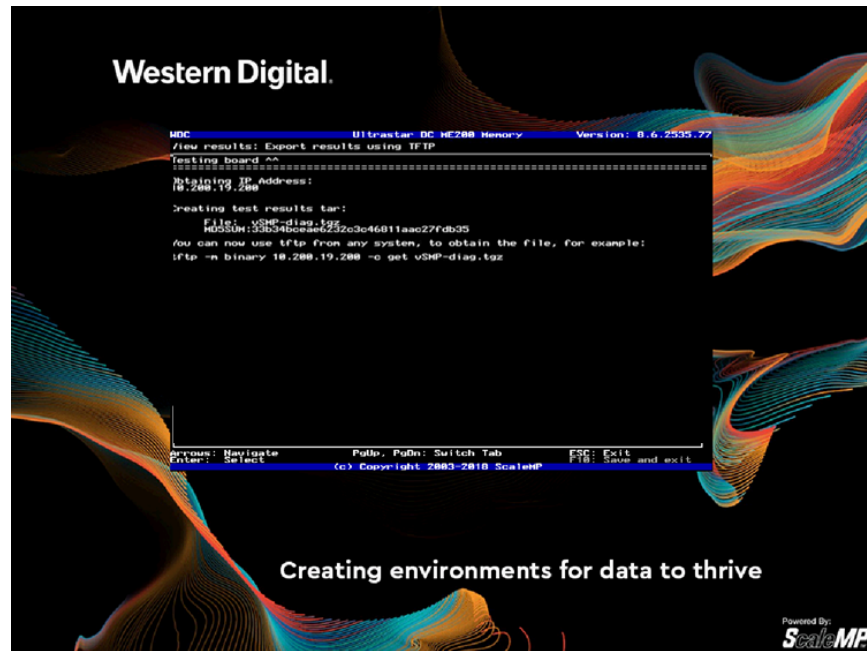
Figure 3-18. TFTP Option
