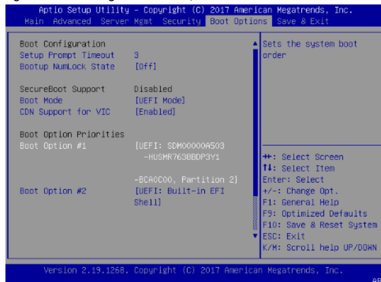
Figure 2-3. Change Boot Order / Priorities
