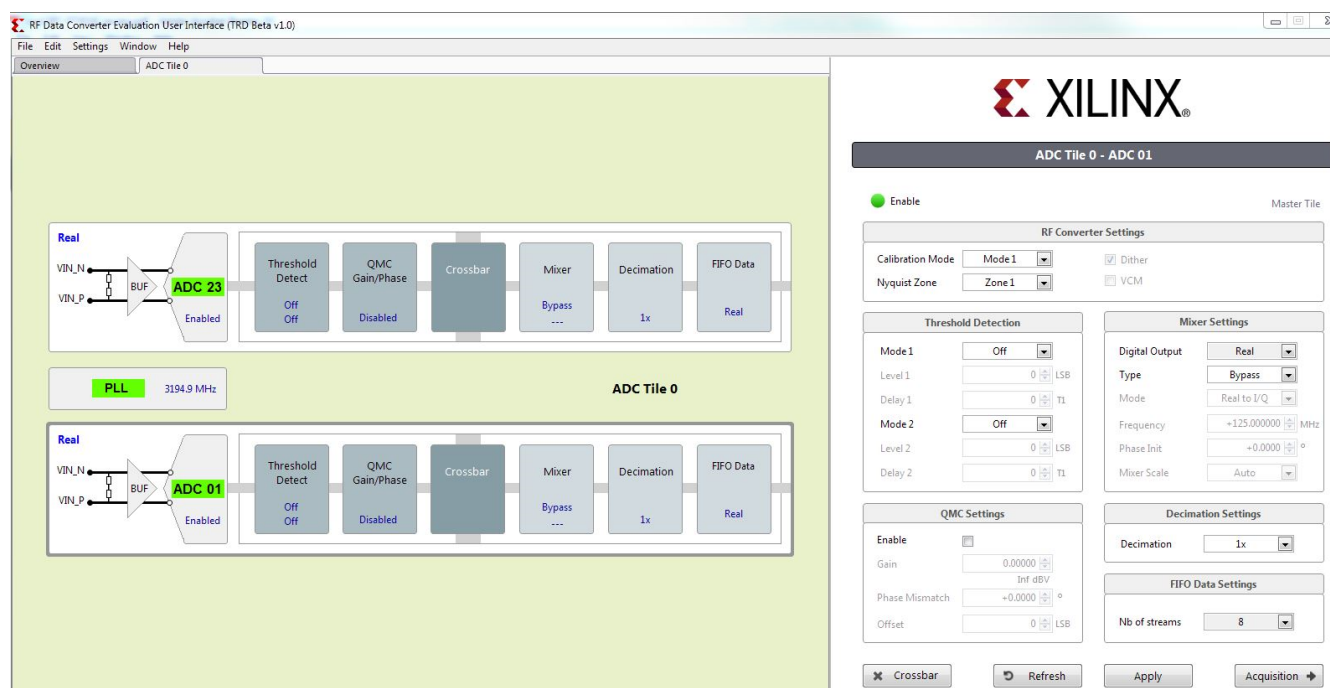
Figure 5-3: ADC Configuration
