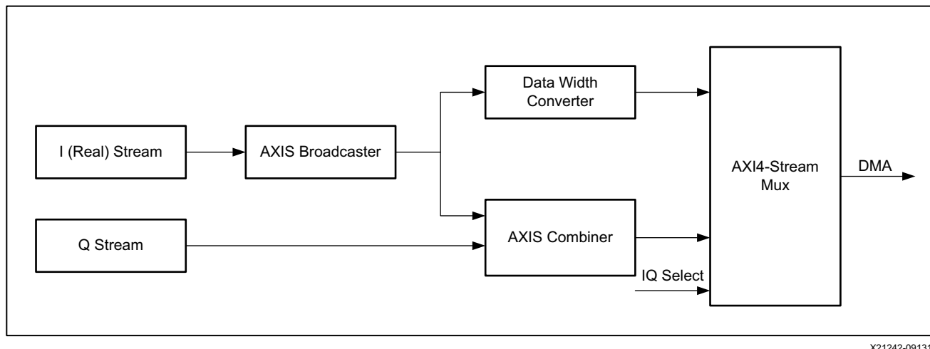
Figure 3-10: IQ Datapath
