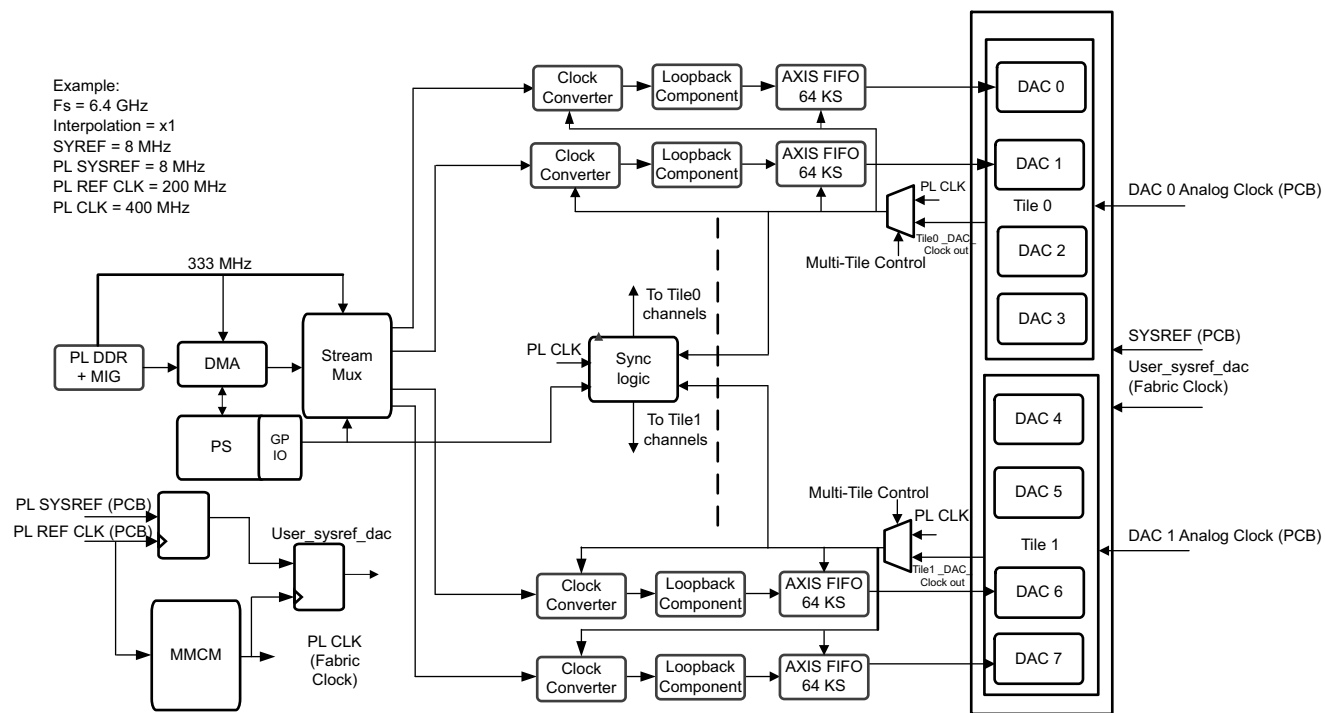
Figure 4-7: RF-DAC Multi-Tile Sync Clocking Structure
