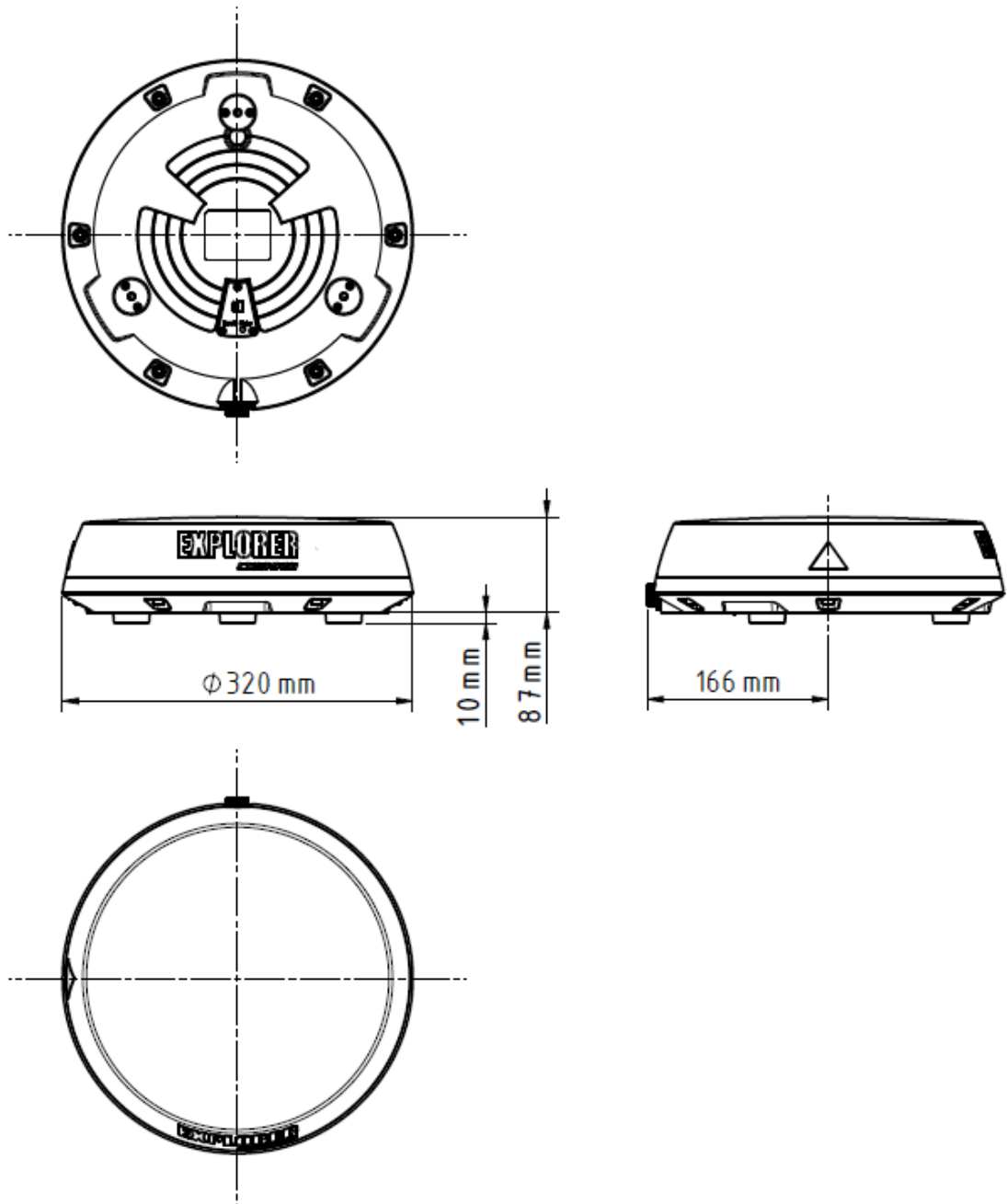
Figure 1-1: EXPLORER 323 outline dimensions drawing
