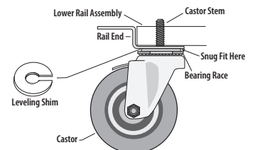
Fig. 7. Install shim(s).
