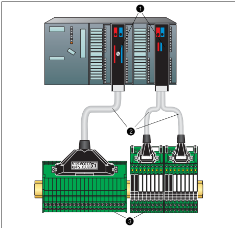
Figure 2: Example of control cabinet wiring with front adapters 1, pre-assembled system cables 2, and termination boards 3
