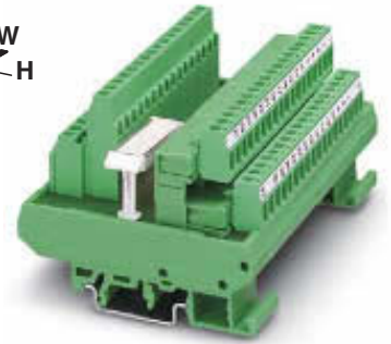
32-pos. with screw connection
