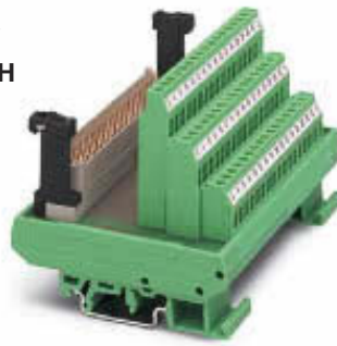
Design F, 48-position, z, b, d assembled
