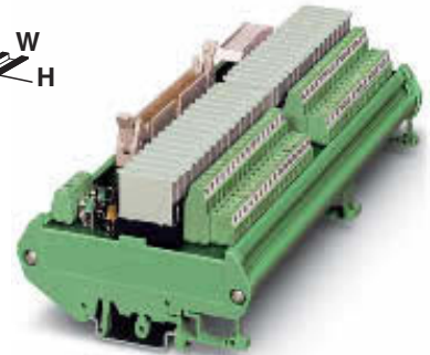
Output modules with 32 miniature relays, one N/O contact
