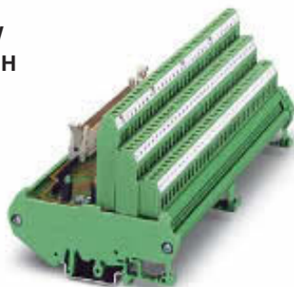
Initiator modules for 32 channels, with screw connection
