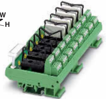
8-channel for relays with two PDT contacts
