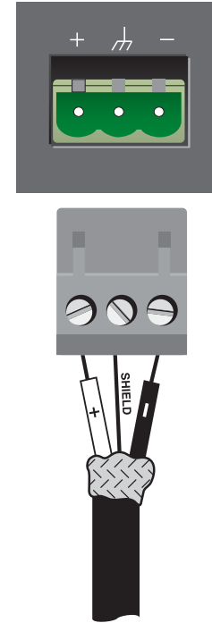
Figure 2.7 Connections to the Preamp Output Connector
