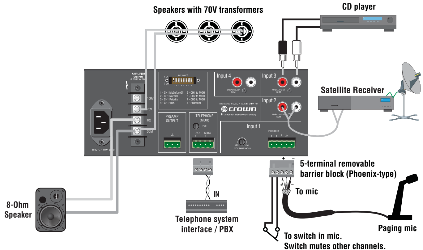
Figure 2.9 Input-Output Wiring
