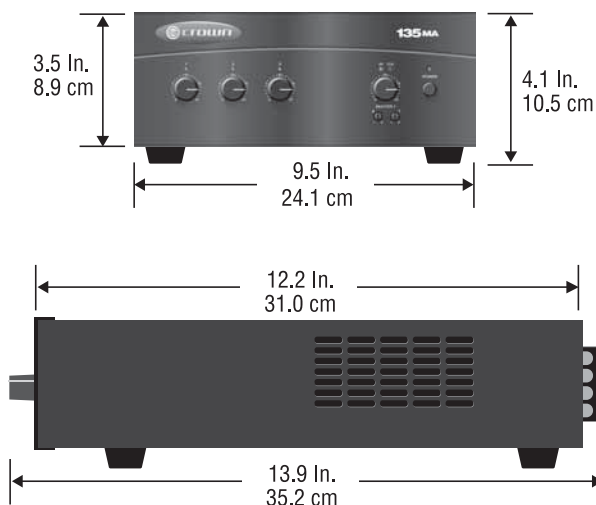
Figure 2.1 Dimensions
