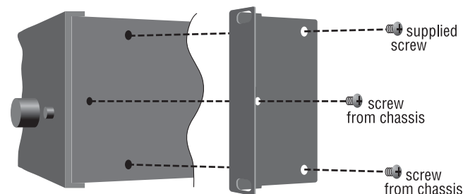
Figure 2.2 How to Connect Rack Ears (Not to Scale)
