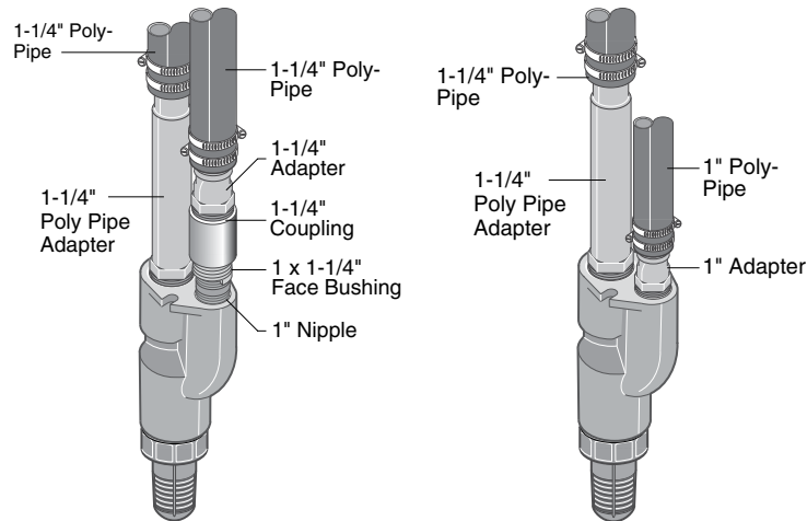
Poly Pipe – 1-1/4" x 1-1/4"
