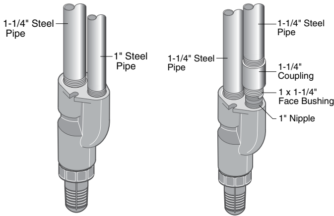
Steel Pipe – 1" x 1-1/4"
