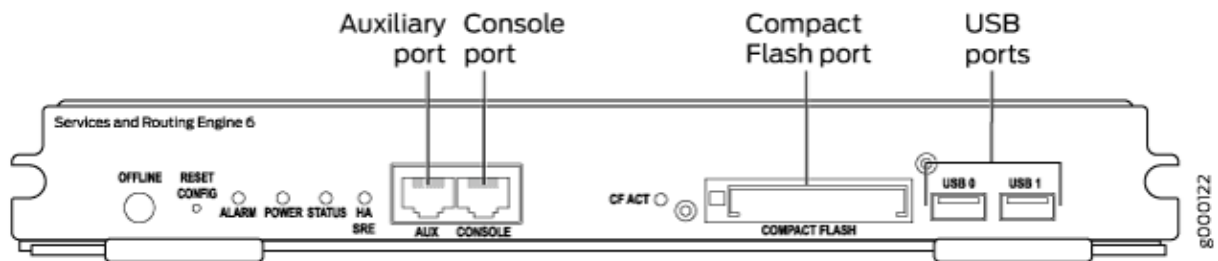
Figure 17: SRX5800 Device Routing Engine
