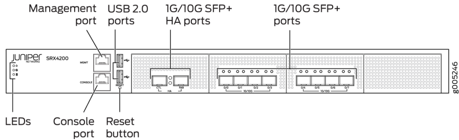
Figure 15: SRX4200 Services Gateway Front Panel
