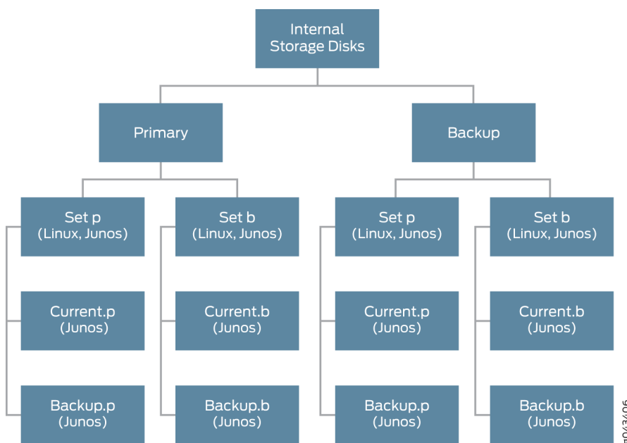
Figure 5: SSD Partitioning
