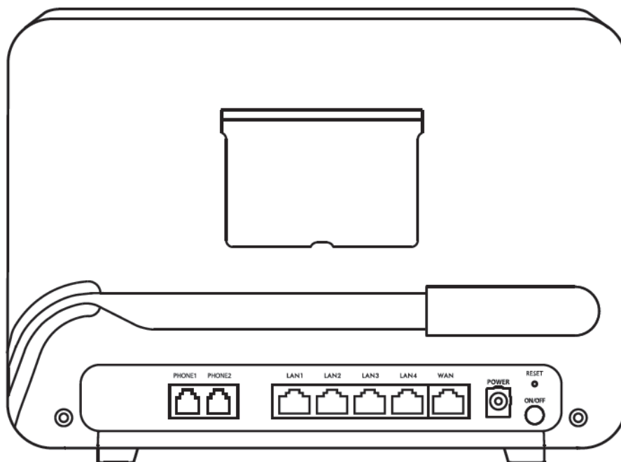
Figure 16 EX5401-B0 Back Panel
