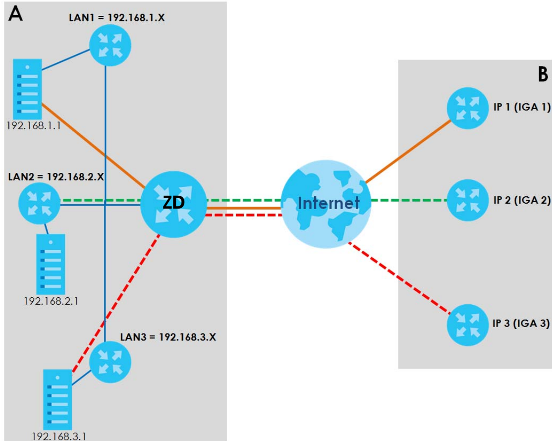
Figure 140 NAT Application With IP Alias
