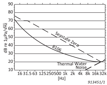
Fig. 13 Typical equivalent noise pressure level of Type 8106
