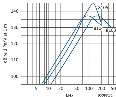
Fig. 9 Typical transmitting response to voltage of Types 8103, 8104 and 8105
