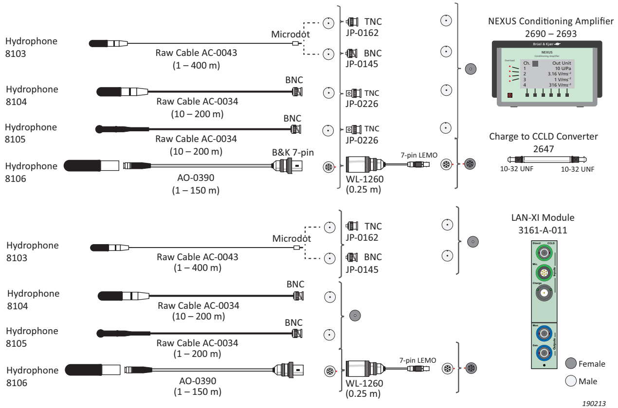
Fig. 11 Measurement chain connections
