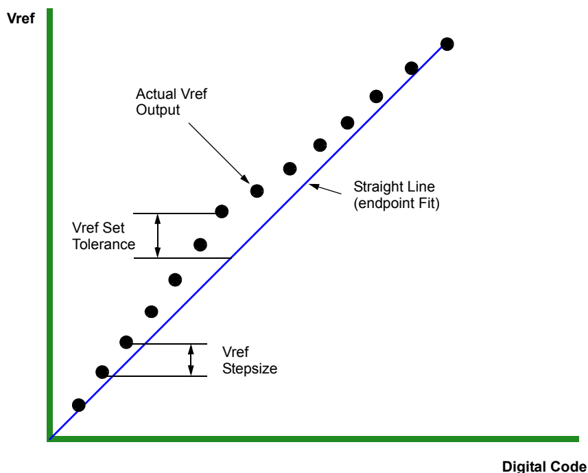
Figure 22. Example of Vref set tolerance(max case only shown) and stepsize
