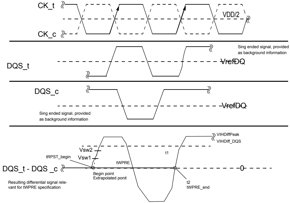
Figure 106. Method for calculating tWPRE transitions and endpoints
