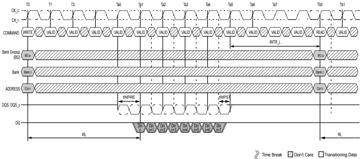
Figure 59. tWTR_L Timing (WRITE to READ, Same Bank Group, CRC and DM Disabled)
