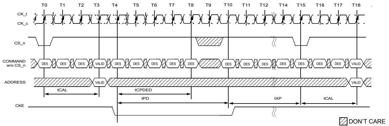
Figure 39. Active Power Down Entry and Exit Timing
