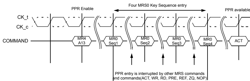
Figure 165. Timing Diagram for soft PPR Key Sequence
