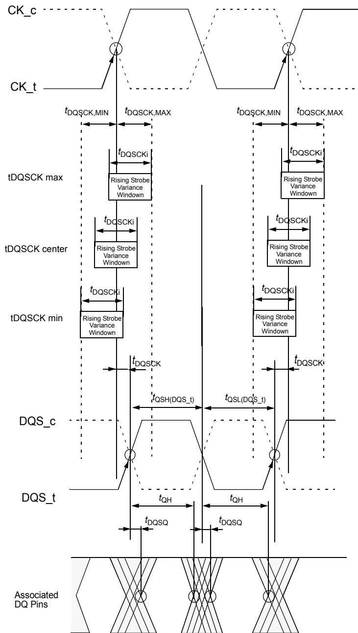
Figure 63. READ Timing Definition
