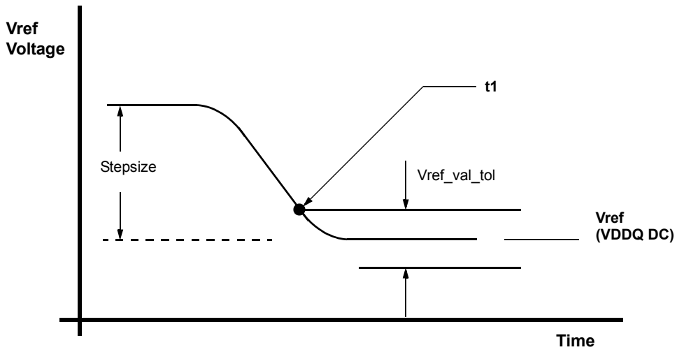
Figure 26. Vref step single stepsize decrement case
