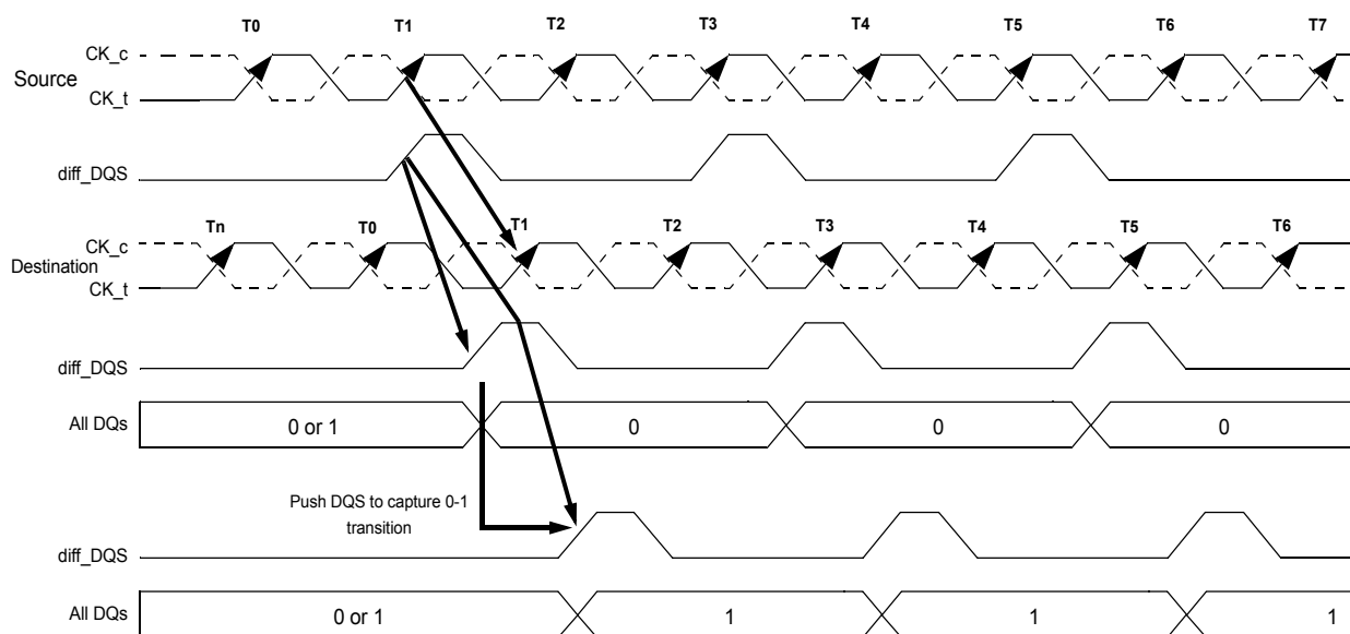
Figure 8. Write Leveling Concept
