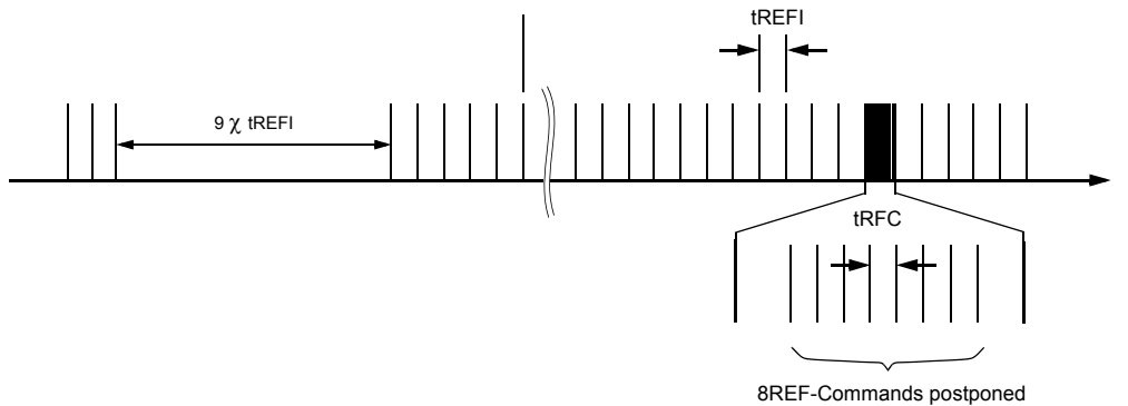
Figure 138. Postponing Refresh Commands (Example of 1X Refresh mode)
