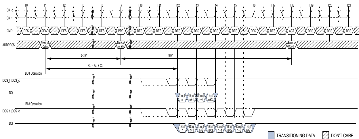
Figure 92. READ to PRECHARGE with 1tCK Preamble
