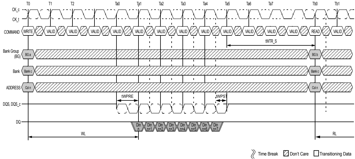
Figure 58. tWTR_S Timing (WRITE to READ, Different Bank Group, CRC and DM Disabled)
