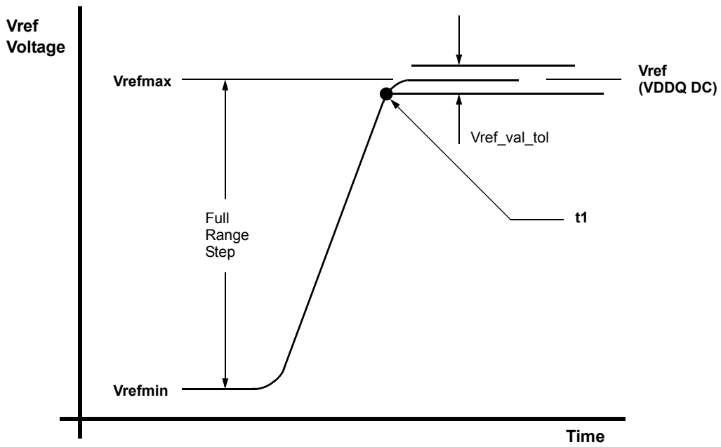
Figure 27. Vref full step from Vrefmin to Vrefmax case
