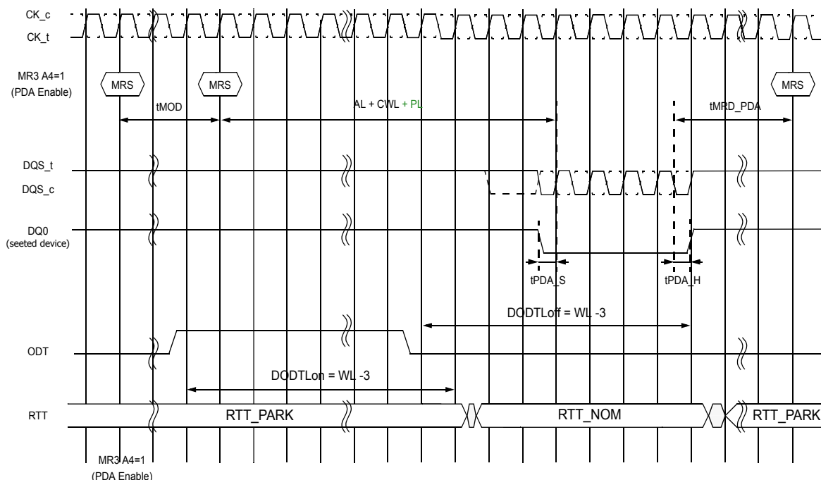
Figure 29. MRS w/ per DRAM addressability (PDA) issuing before MRS
