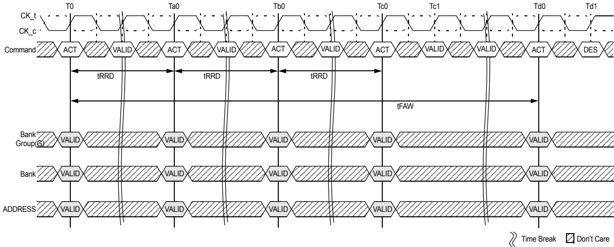
Figure 57. tFAW Timing
