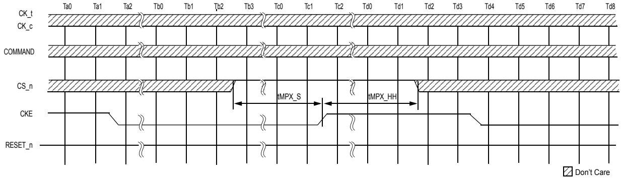
Figure 156. CKE Transition Limitation to hold Maximum Power Saving Mode
