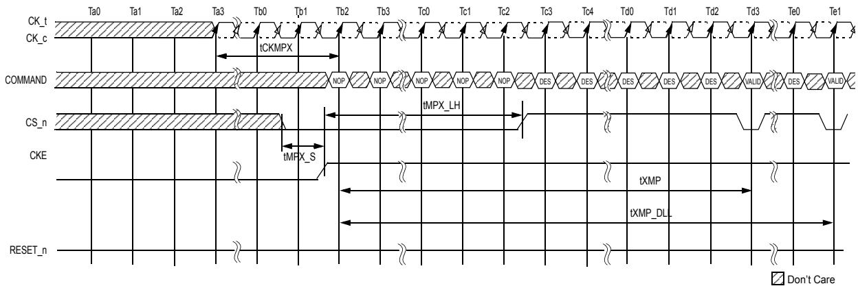
Figure 157. Maximum Power Saving Mode Exit Sequence
