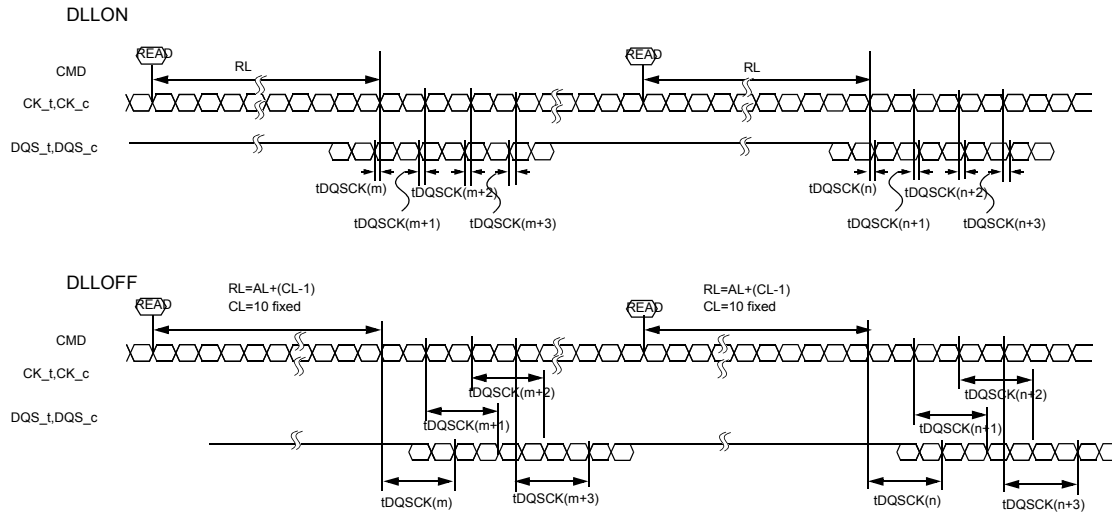
Figure 162. tDQSCK Definition Difference between DLL ON and DLL OFF
