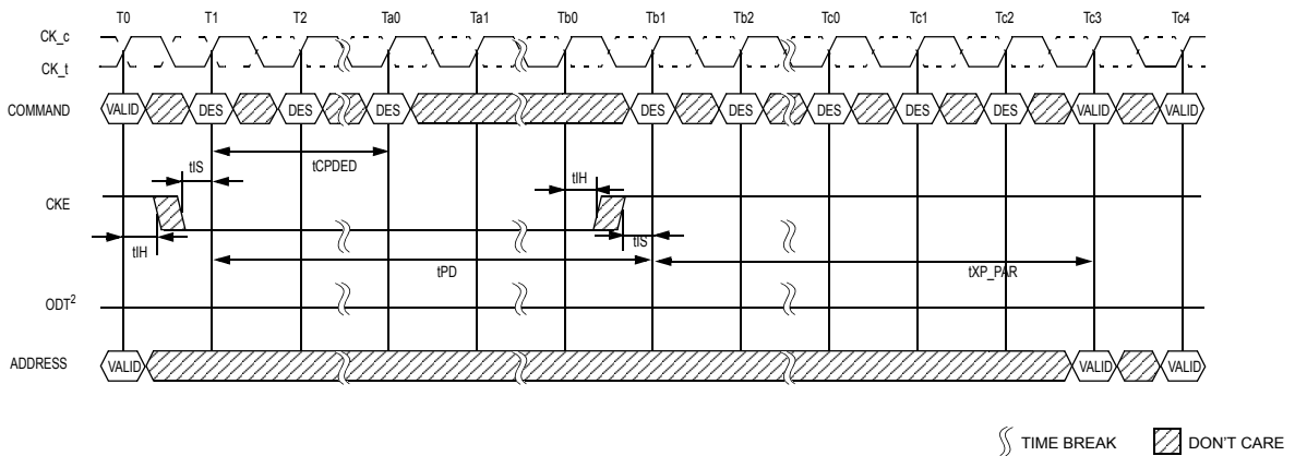
Figure 153. Power Down Entry and Exit Timing with C/A Parity
