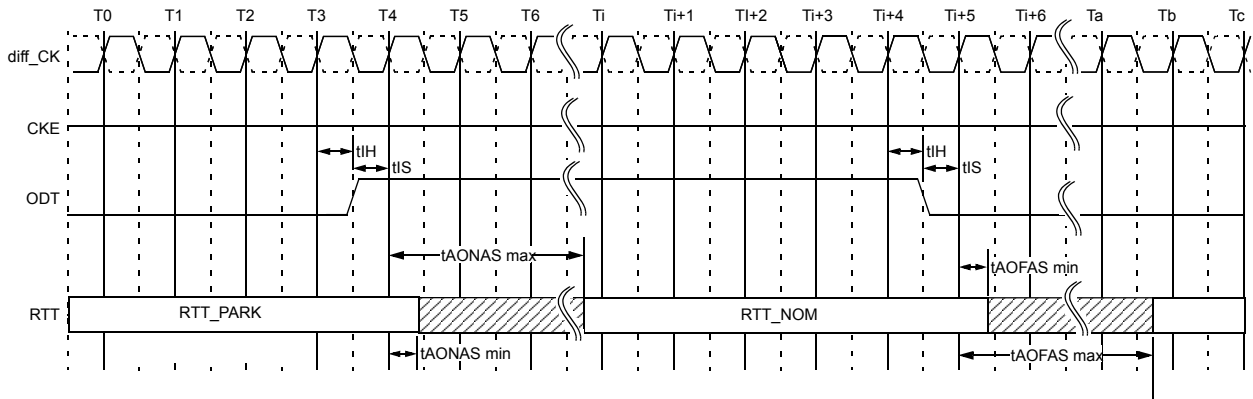
Figure 178. Asynchronous ODT Timing on DDR4 SDRAM with DLL-off
