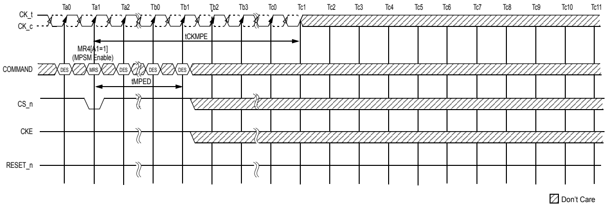
Figure 154. Maximum Power Saving mode Entry
