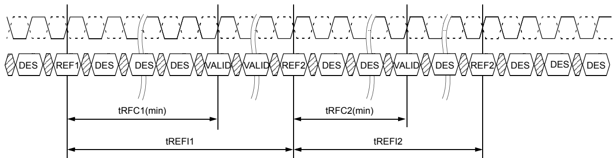
Figure 11. On-the-fly Refresh Command Timing
