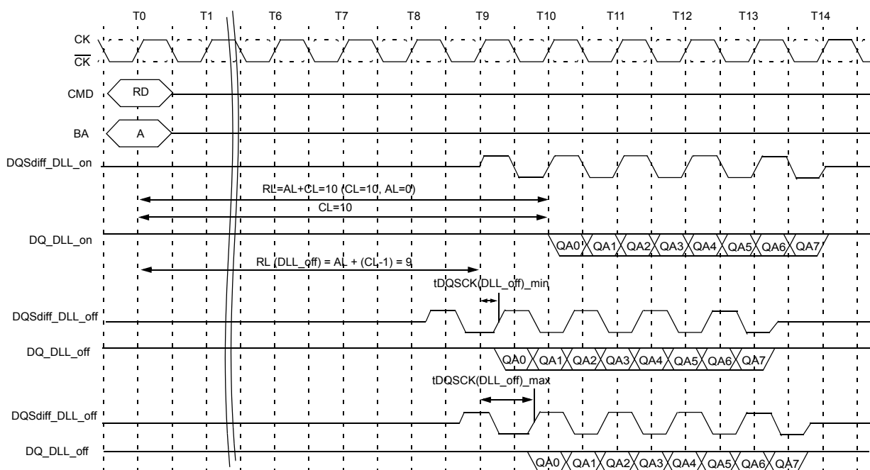
Figure 7. READ operation at DLL-off mode
