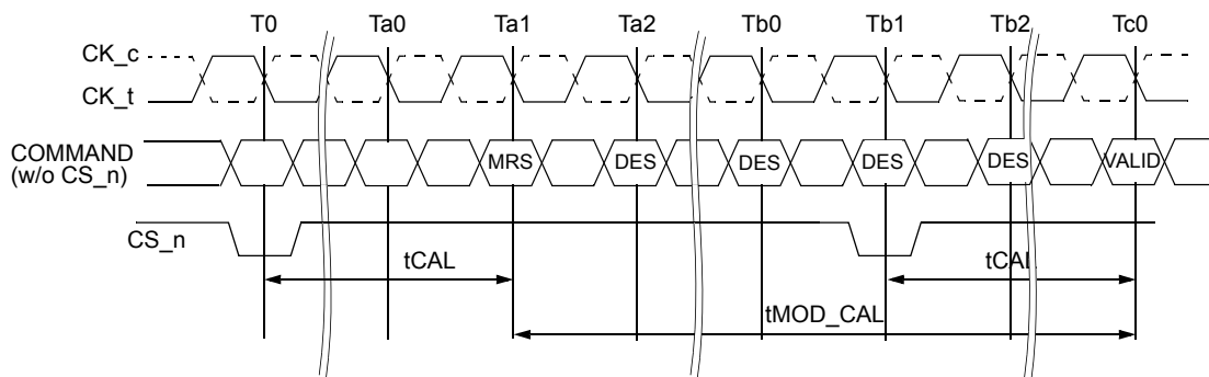
Figure 34. CAL enable timing - t_{MOD\_CAL}
