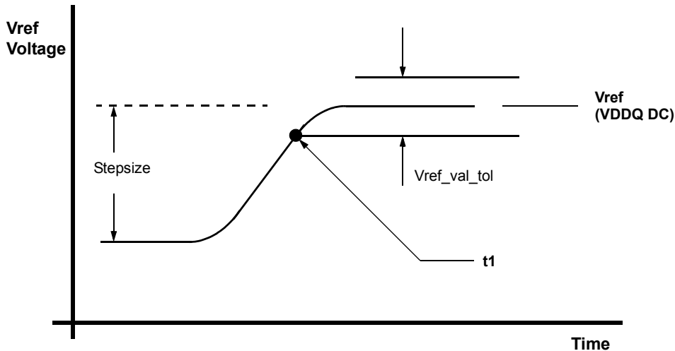
Figure 25. Vref step single stepsize increment case
