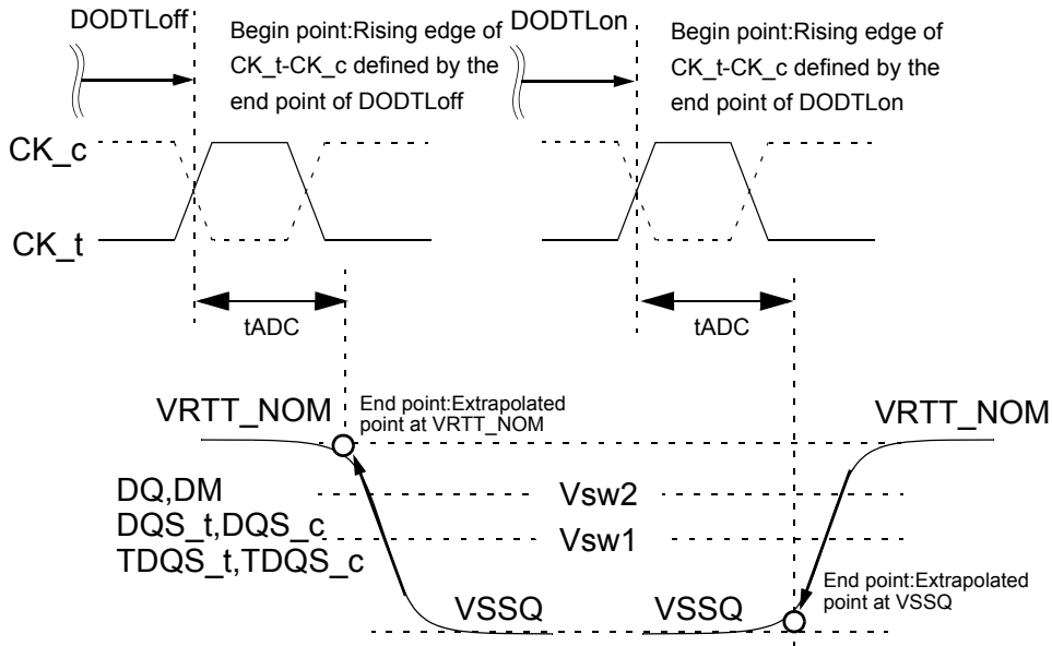
Figure 182. Definition of tADC at Direct ODT Control
