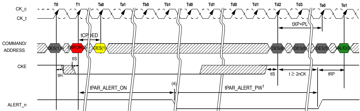
Figure 44. CA Parity Error Checking - PDE/PDX
