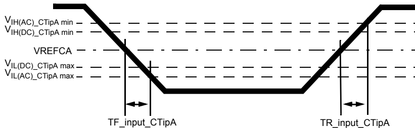
Figure 160. CS_n and Input A Slew Rate Definition
