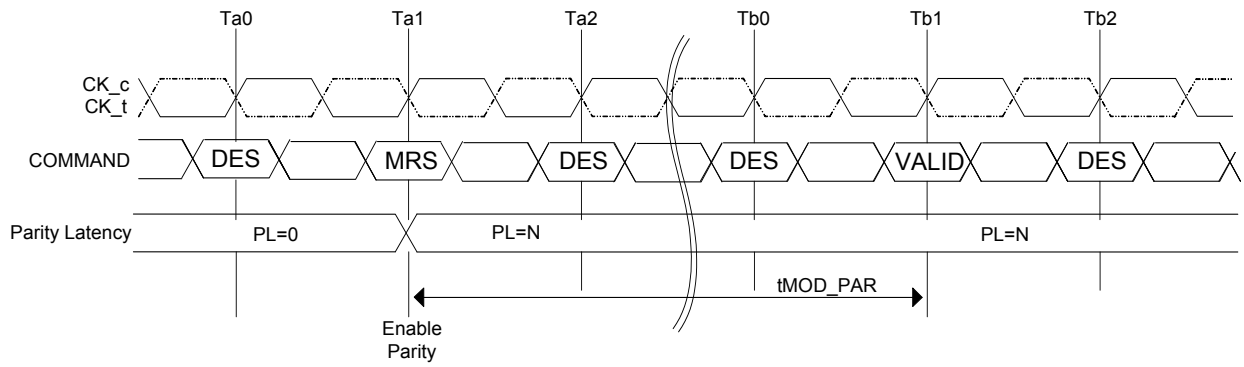
Figure 48. Parity entry timing example - tMOD_PAR
