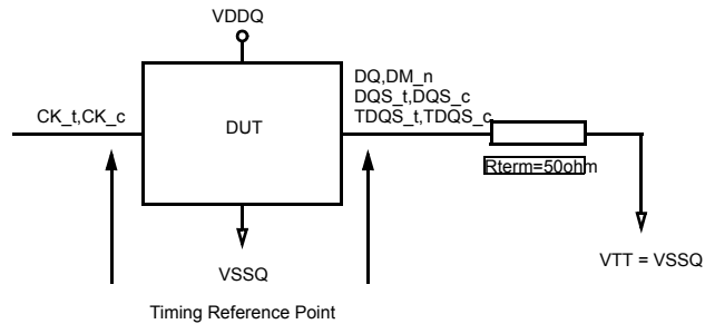
Figure 181. ODT Timing Reference Load
