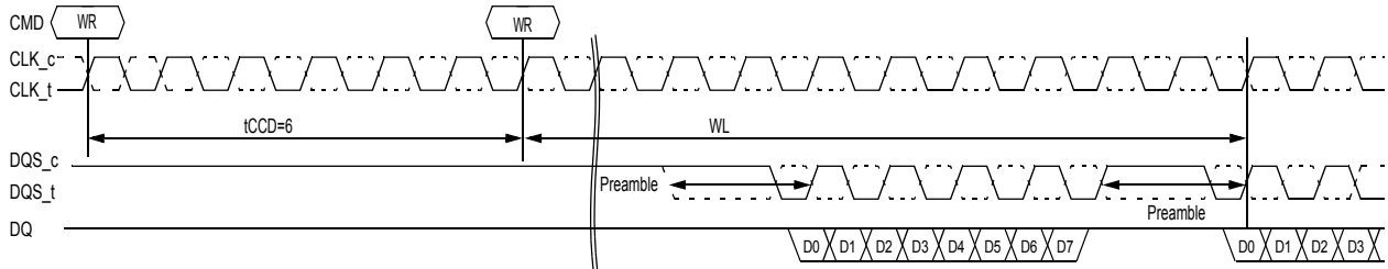
Figure 62. t_{CCD}=6 (AL=PL=0)
