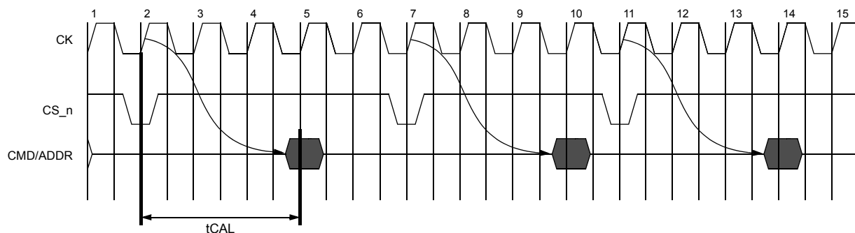
Figure 32. Definition of CAL
