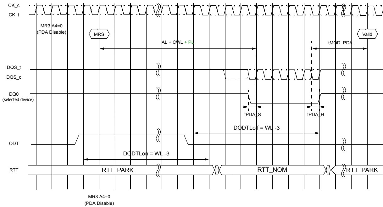
Figure 30. MRS w/ per DRAM addressability (PDA) Exit
