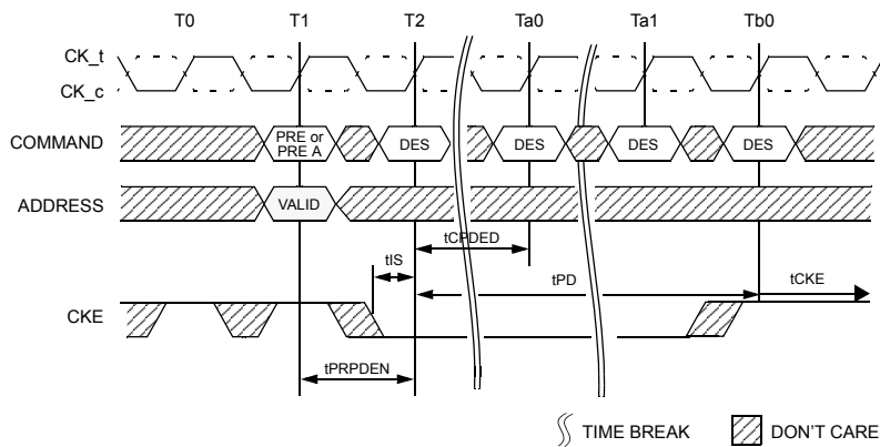
Figure 150. Precharge/Precharge all Command to Power-Down Entry
