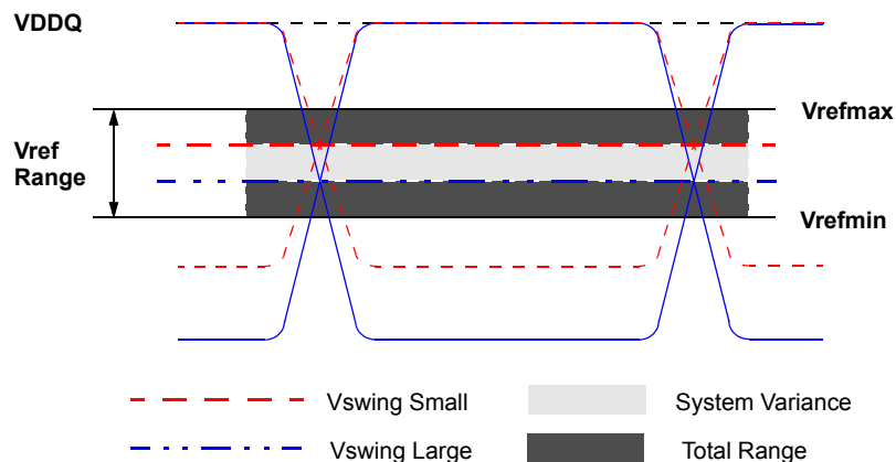
Figure 21. Vref operating range(Vrefmin, Vrefmax)
