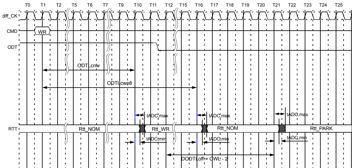
Figure 177. Dynamic ODT overlapped with Rtt_NOM (CL=14, CWL=11, BL=8, AL=0, CRC Disabled)
