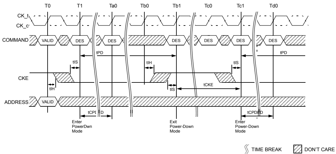
Figure 152. Power-Down Entry/Exit Clarification
