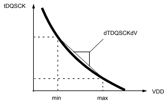
Figure 163. dTDQSCKdT Definition
