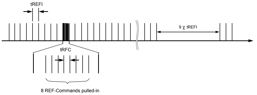
Figure 139. Pulling-in Refresh Commands (Example of 1X Refresh mode)
