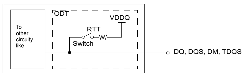
Figure 171. Functional Representation of ODT
