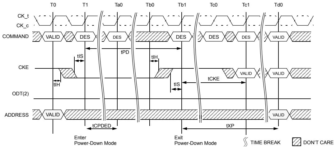
Figure 142. Active Power-Down Entry and Exit Timing Diagram MR5 bit A5 =0
