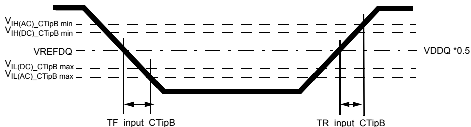
Figure 161. Input B Slew Rate Definition
