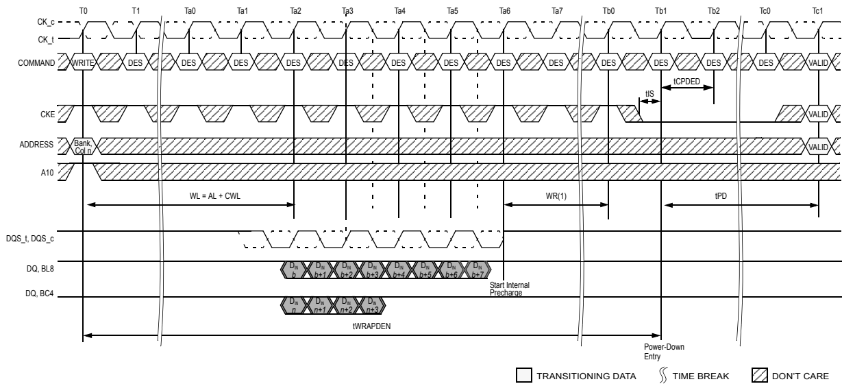
Figure 145. Power-Down Entry After Write with Auto Precharge
