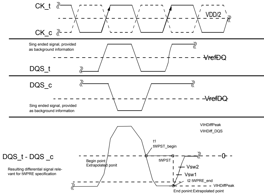
Figure 107. Method for calculating tWPST transitions and endpoints
