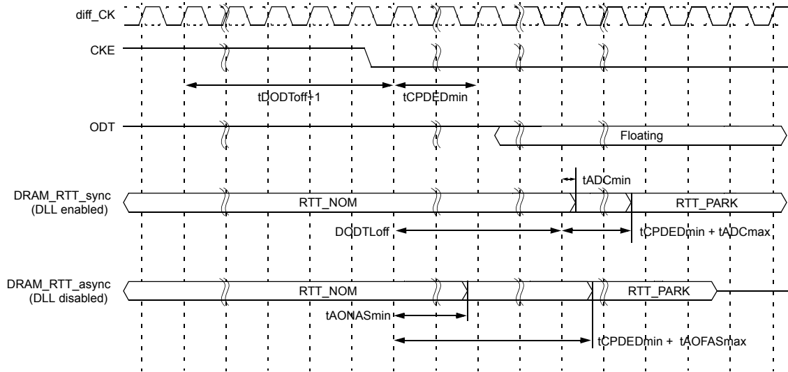
Figure 179. ODT timing for power down entry with ODT buffer disable mode
