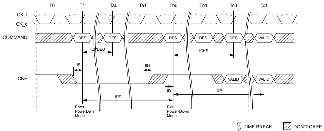
Figure 147. Precharge Power-Down Entry and Exit
