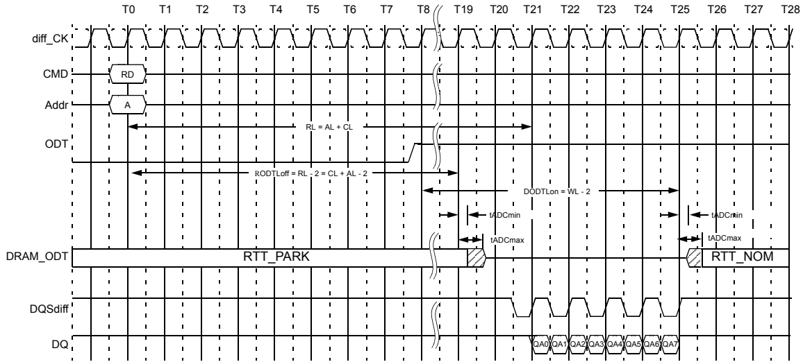
Figure 175. Example: CL=11, PL=0; AL=CL-1=10; RL=AL+PL+CL=21; CWL=9; DODTLon=AL+CWL-2=17; DODTLoff=AL+CWL-2=17; 1tCK preamble)
