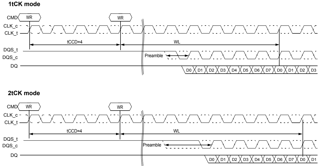
Figure 60. tCCD=4 (AL=PL=0)
