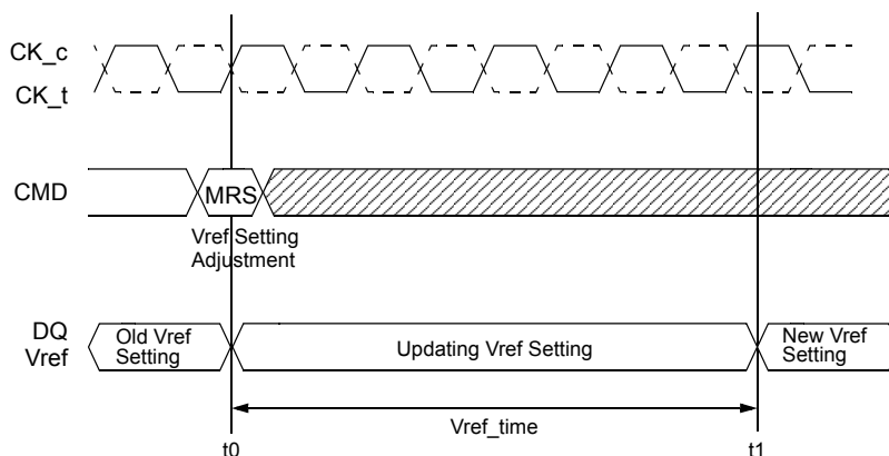
Figure 23. Vref_time timing diagram
