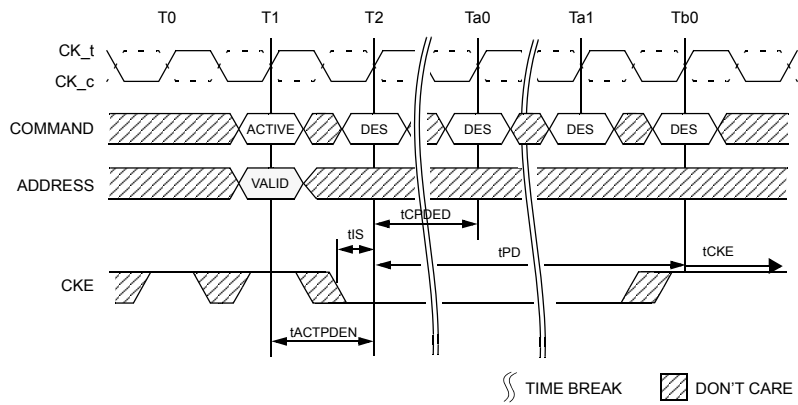
Figure 149. Activate Command to Power-Down Entry
