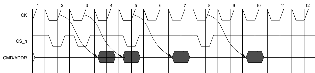
Figure 33. CAL operational timing for consecutive command issues
