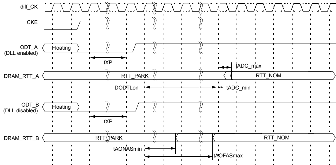
Figure 180. ODT timing for power down exit with ODT buffer disable mode
