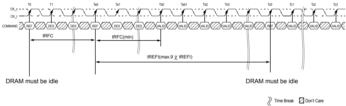
Figure 137. Refresh Command Timing (Example of 1x Refresh mode)
