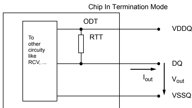
Figure 172. On Die Termination
