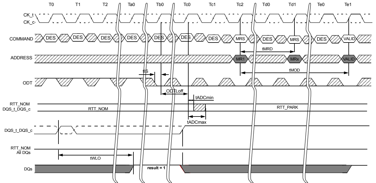
Figure 10. Timing details of Write leveling exit
