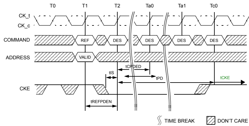
Figure 148. Refresh Command to Power-Down Entry
