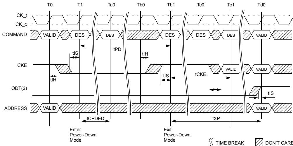
Figure 143. Active Power-Down Entry and Exit Timing Diagram MR5 bit A5=1
