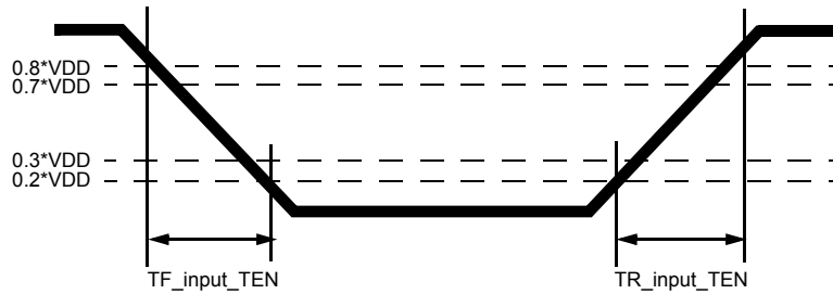
Figure 159. TEN Input Slew Rate Definition
