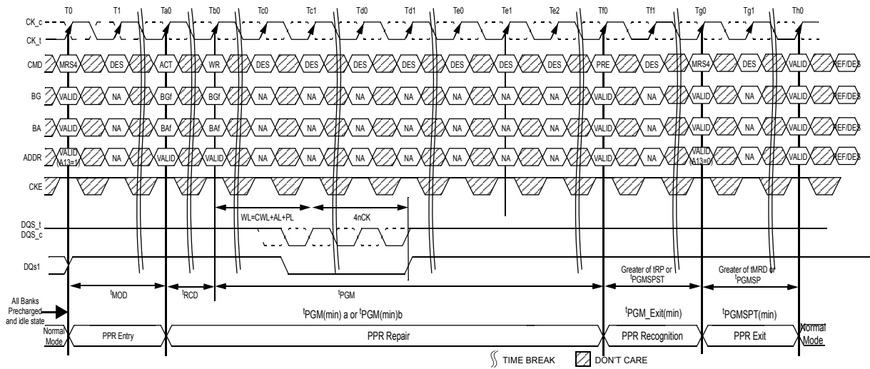
Figure 167. Fail Row Repair (WR Case)
