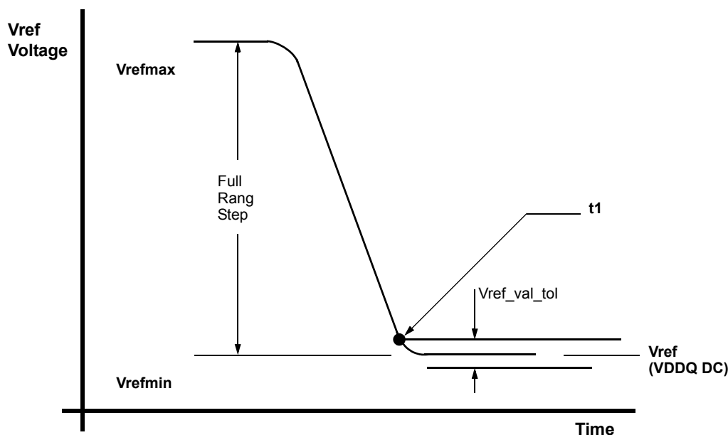
Figure 28. Vref full step from Vrefmax to Vrefmin case
