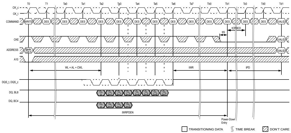
Figure 146. Power-Down Entry after Write
