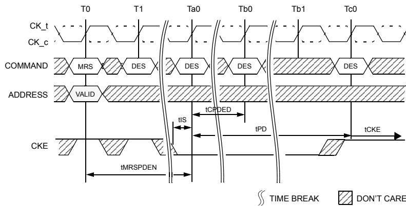
Figure 151. MRS Command to Power-Down Entry
