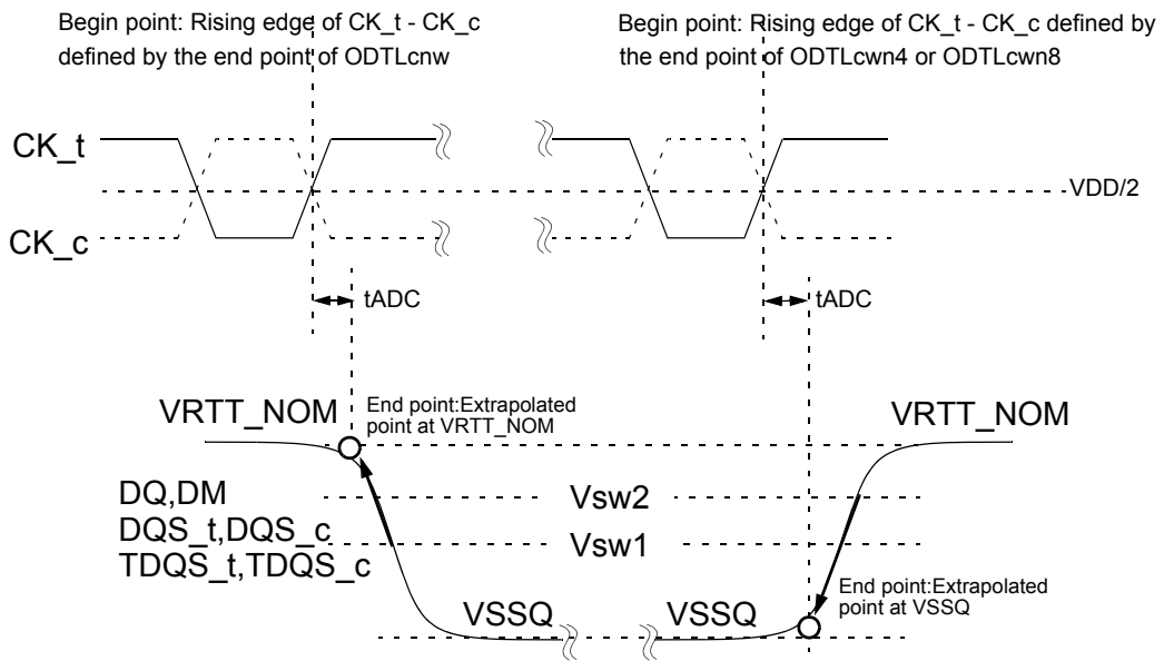
Figure 183. Definition of tADC at Dynamic ODT Control
