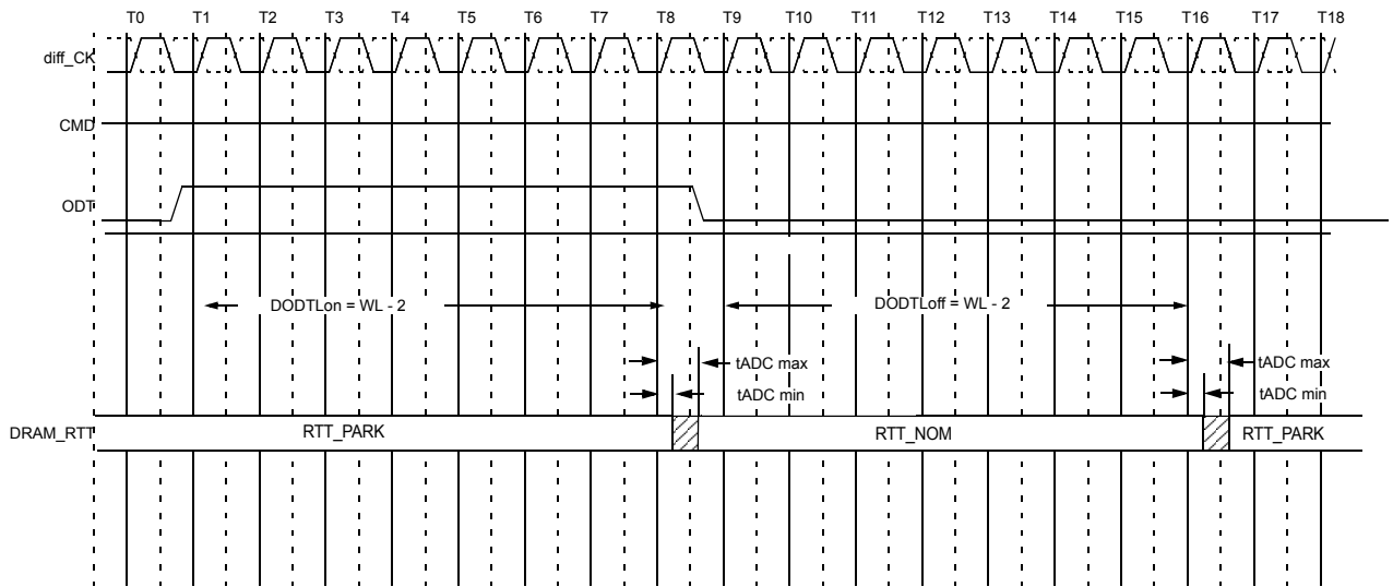
Figure 173. Synchronous ODT Timing Example for CWL=9, AL=0, PL=0; DODTLon=WL-2=7; DODTLoFF=WL-2=7
