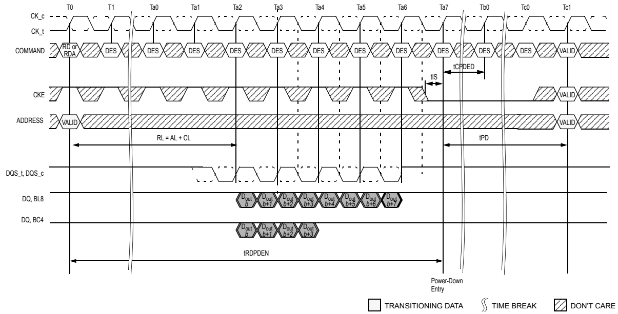
Figure 144. Power-Down Entry after Read and Read with Auto Precharge
