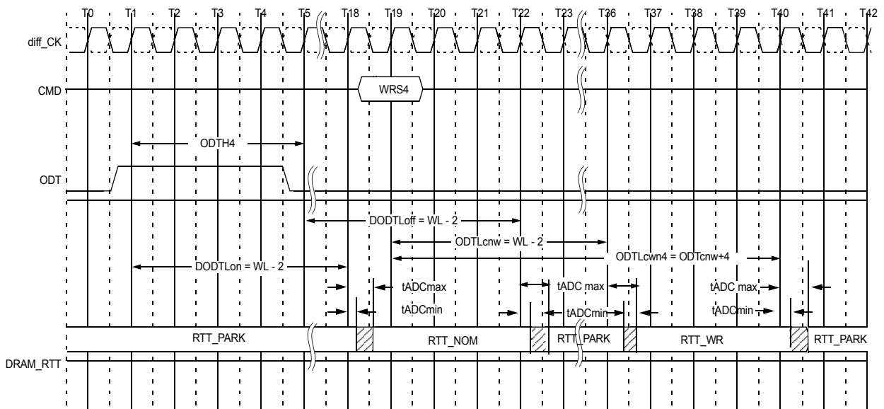
Figure 174. Synchronous ODT example with BL=4, CWL=9, AL=10, PL=0; DODTLon/off=WL-2=17, ODTcnw=WL-2=17
