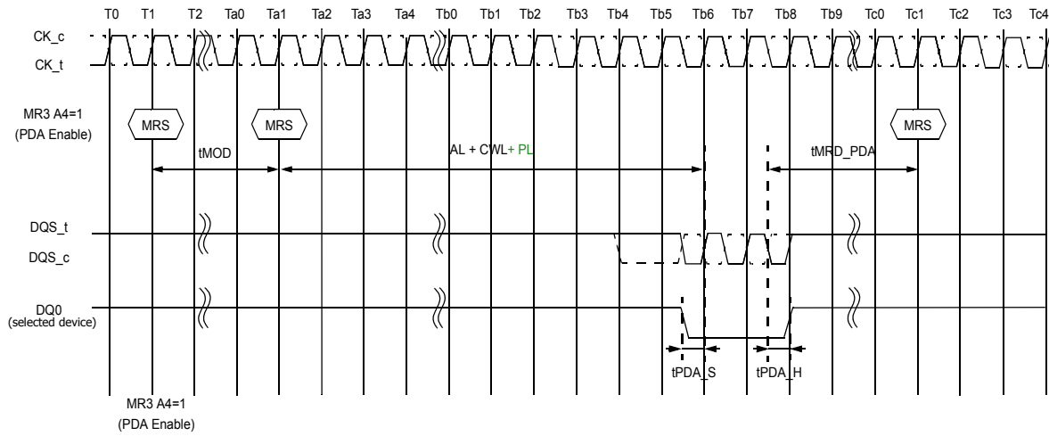
Figure 31. PDA using Burst Chop 4
