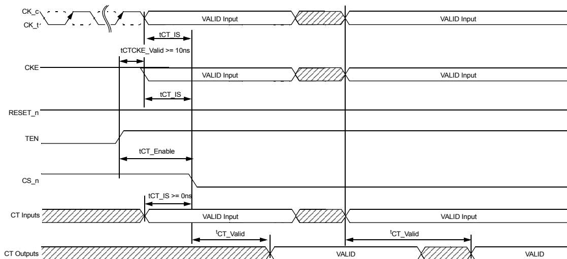
Figure 158. Timing Diagram for Connectivity Test(CT) Mode
