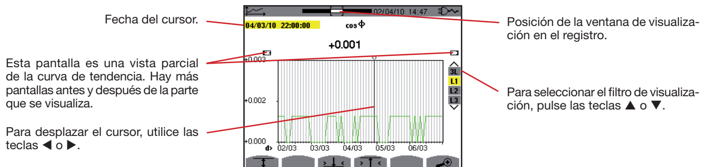
Figura 103: cos \Phi (L1) sin MIN-AVG-MAX
