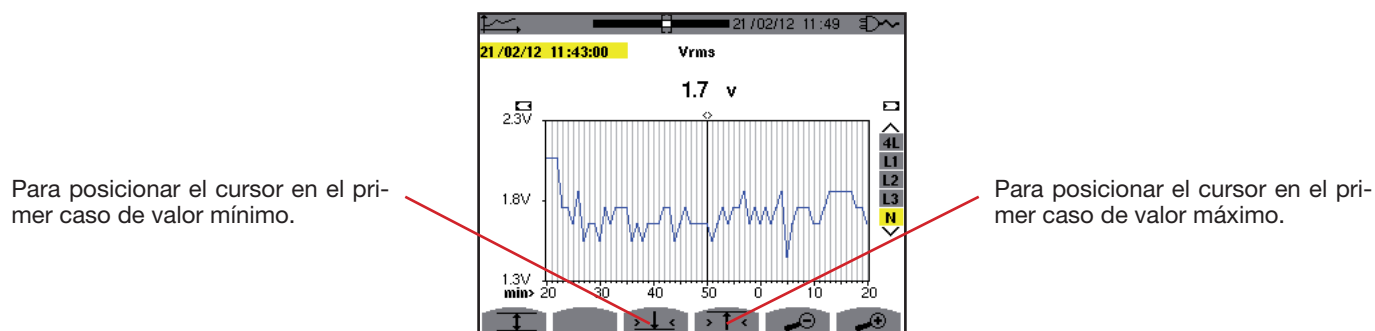
Figura 93: Vrms (N) sin MIN-AVG-MAX
