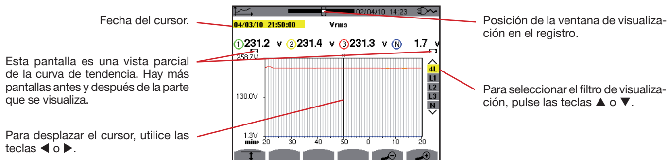
Figura 91: Vrms (4L) sin MIN-AVG-MAX
