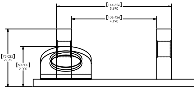
MODEL FB-SW3 FRONT VIEW
