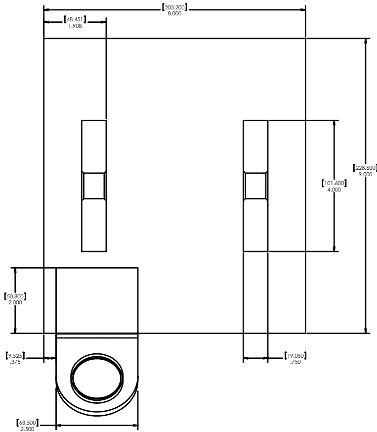
MODEL FB-SW3 TOP VIEW
