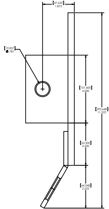
MODEL FB-SW3 SIDE VIEW
