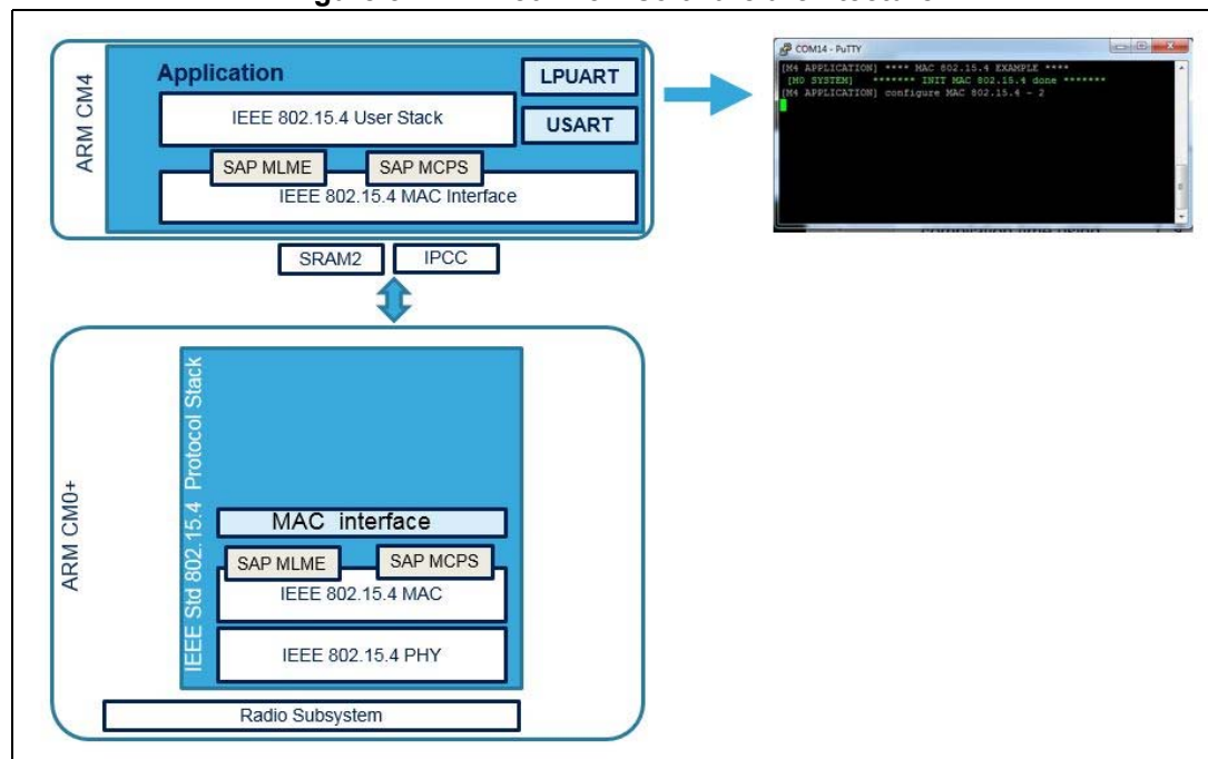
Figure 52. MAC 802.15.4 software architecture
