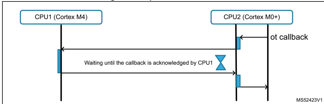
Figure 38. OpenThread callback
