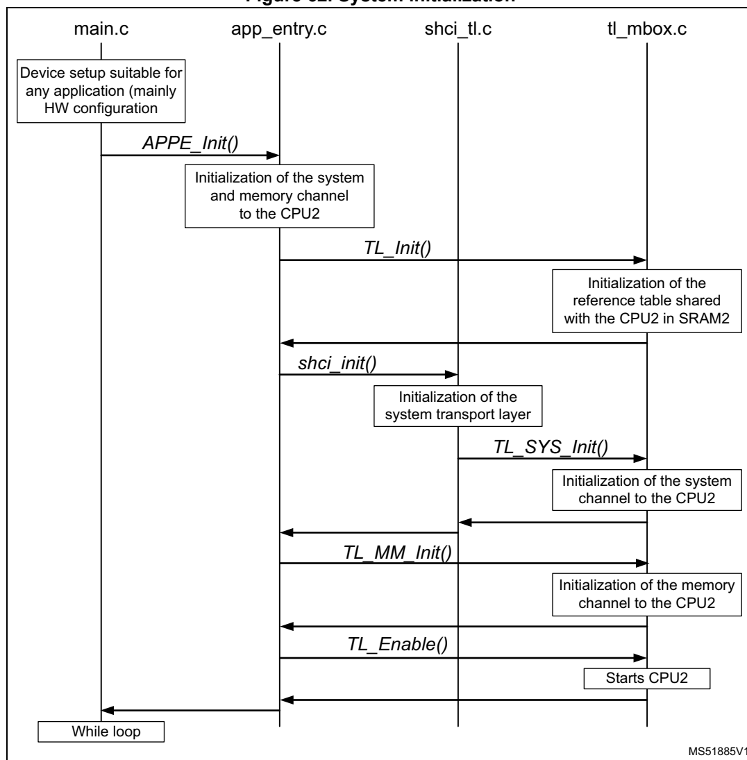
Figure 62. System initialization
