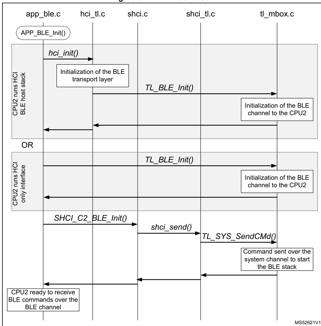
Figure 64. BLE initialization
