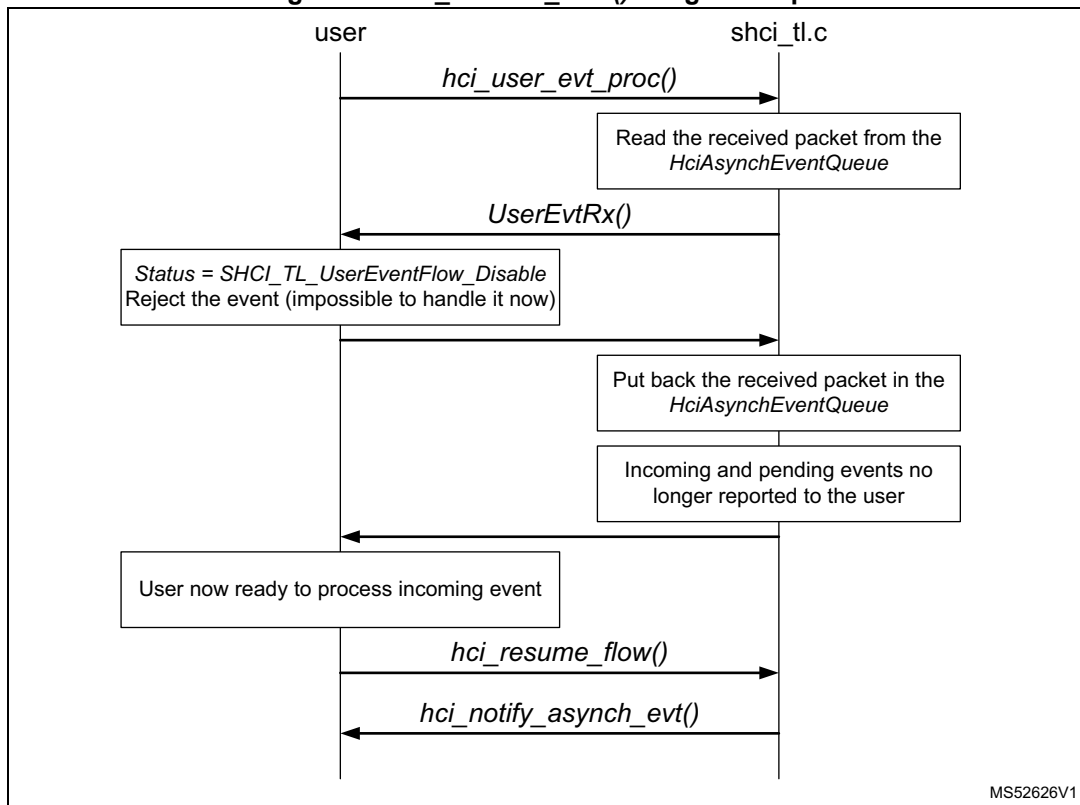
Figure 78. hci_resume_flow() usage example
