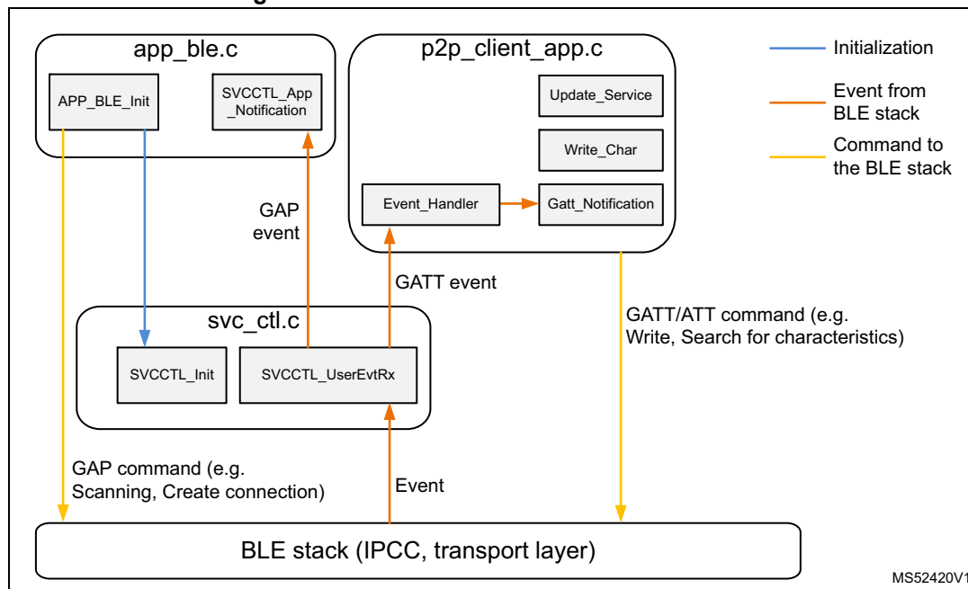
Figure 28. P2P client software communication
