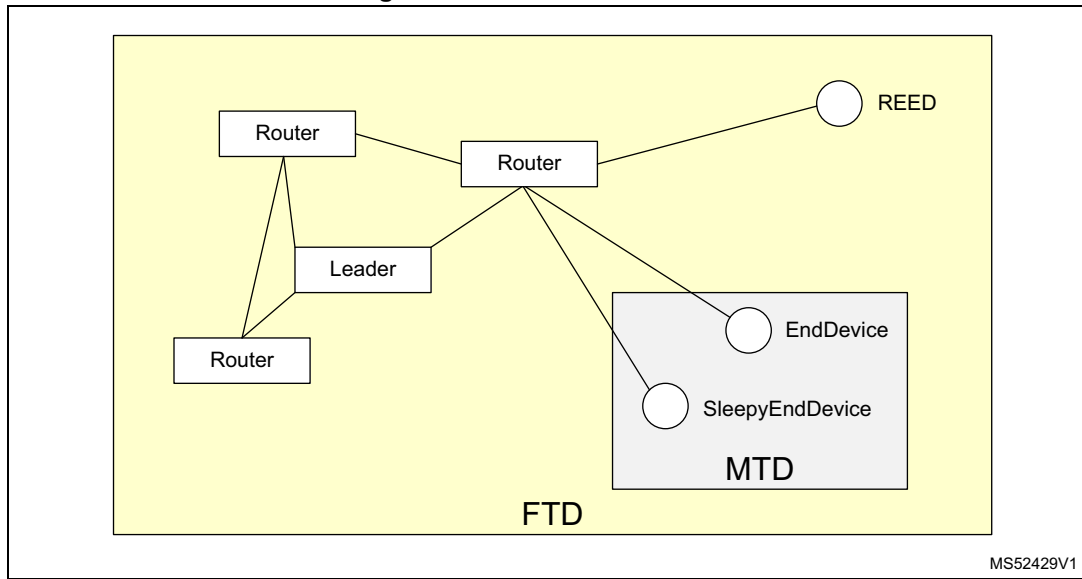
Figure 88. Thread device roles
