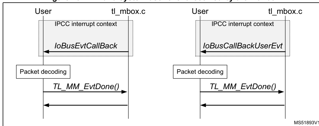
Figure 70. BLE and system user event received by the mailbox
