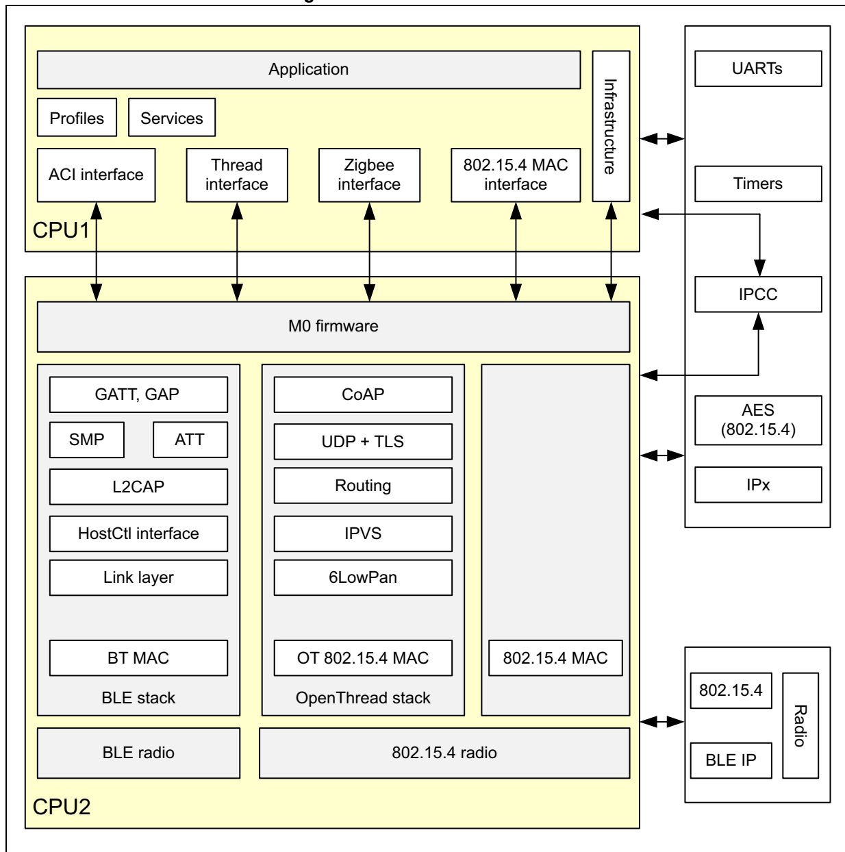
Figure 36. Software architecture
