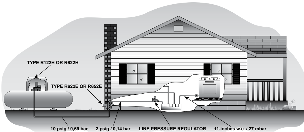
Figure 3. Two-Stage Regulation, One at Tank and One at Building, Reducing Pressure Down to Burner Pressure (11-inches w.c. / 27 mbar)
