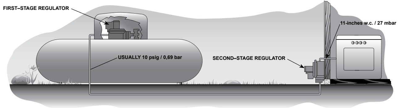
Figure 3. Two-Stage Regulation, One at Tank and One at Building, Reducing Pressure Down to Burner Pressure (11-inches w.c. / 27 mbar)
