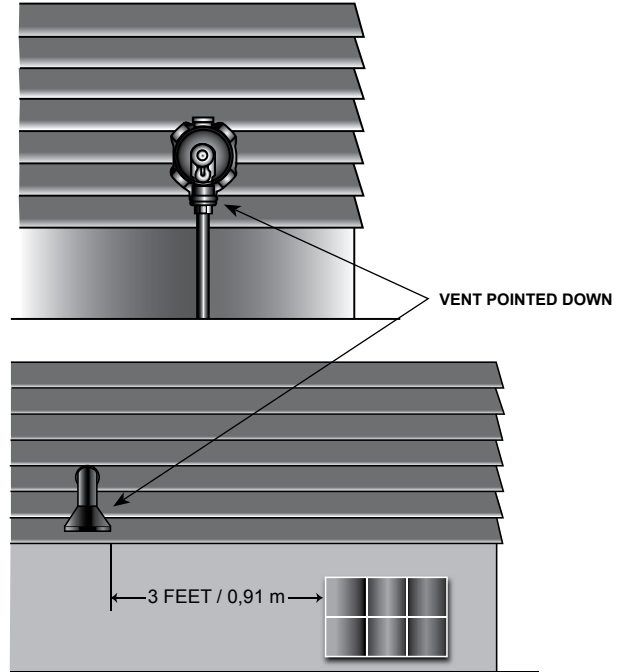
Figure 12. Vent Installation Away from Windows, Basement Air Intakes, and other Openings
