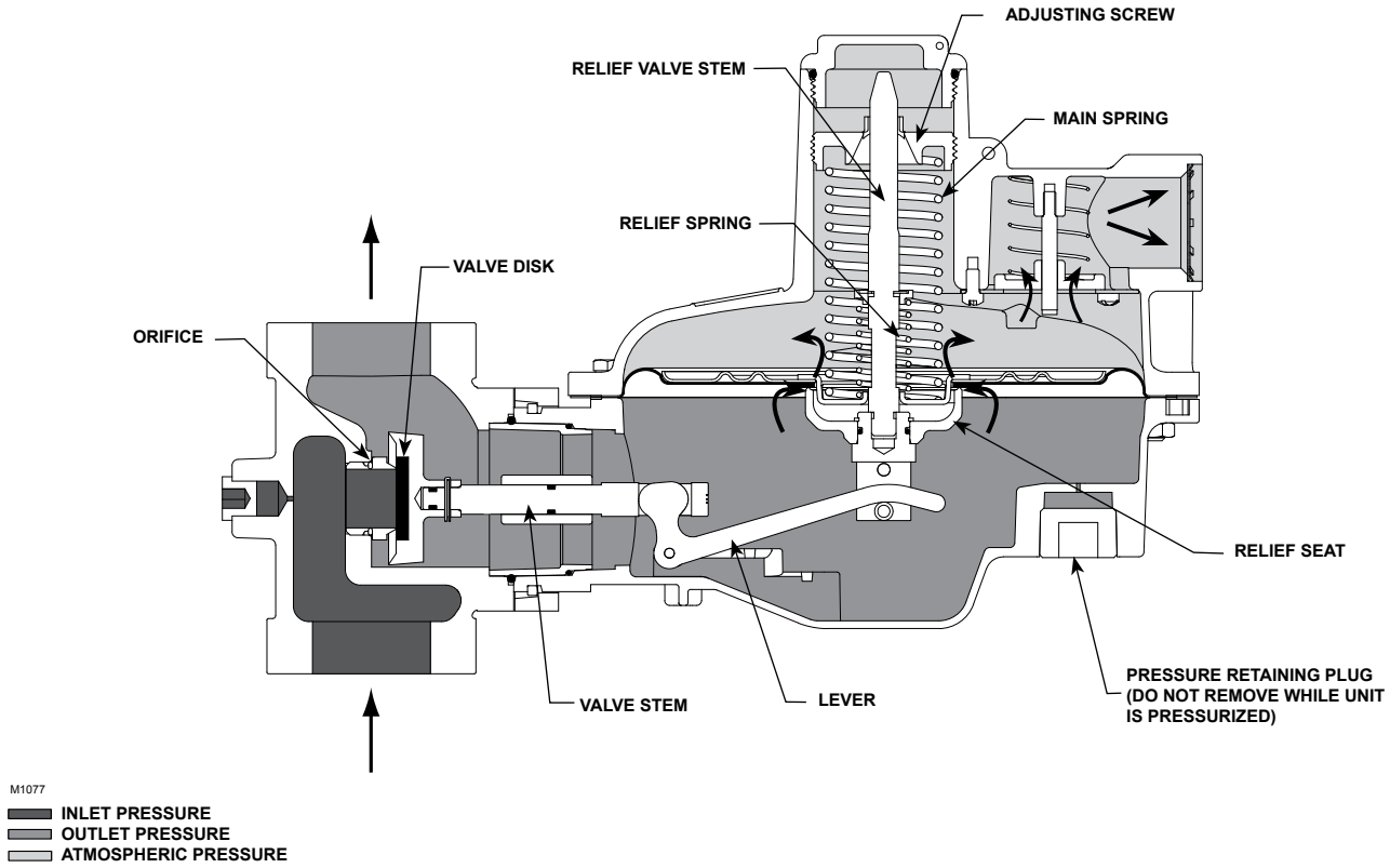
Figure 6. Type CS400IR Internally Registered Regulator with Internal Relief Operational Schematic
