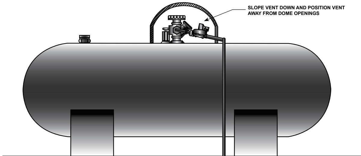
Figure 8. Tank Installation
