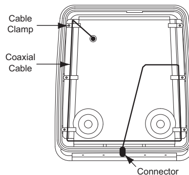
Figure 5-11. Routing the Coaxial Cable for GPS
