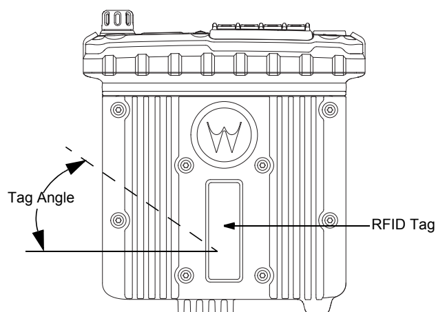
Figure 2-67. Tag Angle for APX 2500/APX 4500 Mid Power Radio
