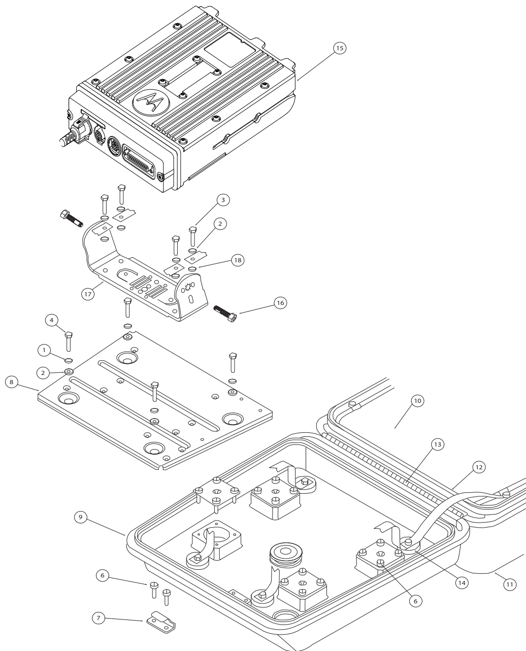
Figure 5-17. Installing the Transceiver
