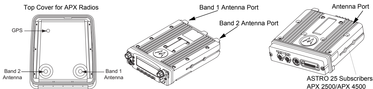
Figure 5-8. Location of Band 1 or Band 2 (Depending on the Antenna Port They Align to)
