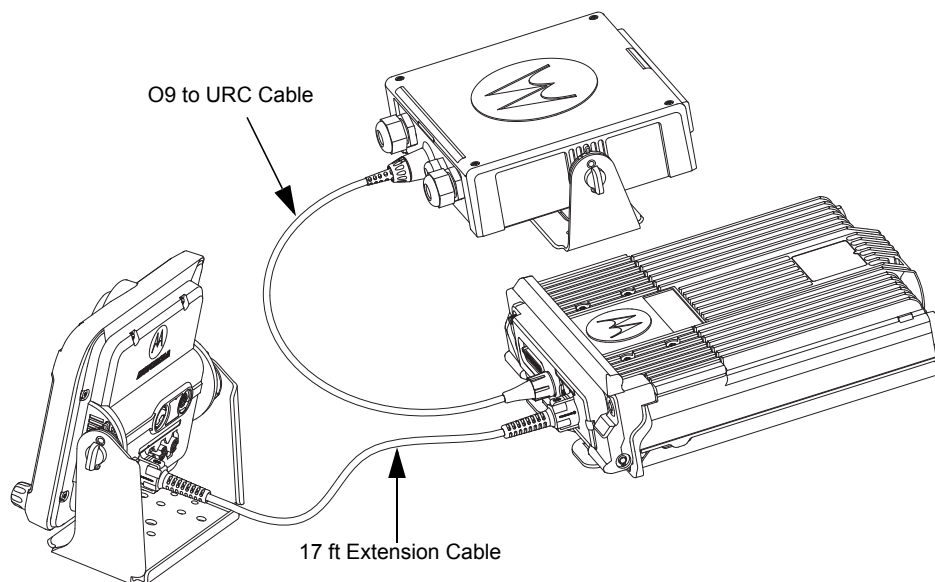
Figure 1-40. Remote Mount Configuration with High Power (100W) Radio Transceiver, Universal Relay Controller and O9 Control Head (URC is optional)
