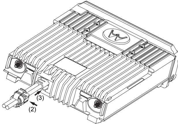
Figure 2-42. Bracket Installation
