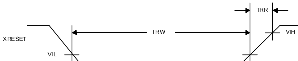
Figure 15. Reset Signal
