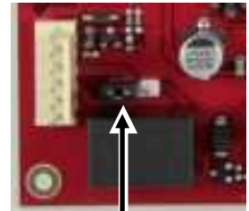
Relay Polarity Jumper shown in the normally-open position
