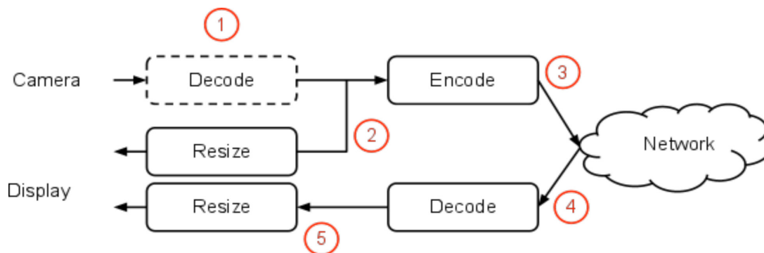
Figure 2. Two-way Video Calling - Non-Encoding Webcam
