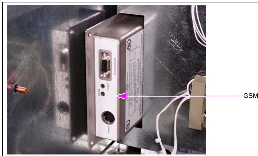
Figure 5: Securing the GSM
