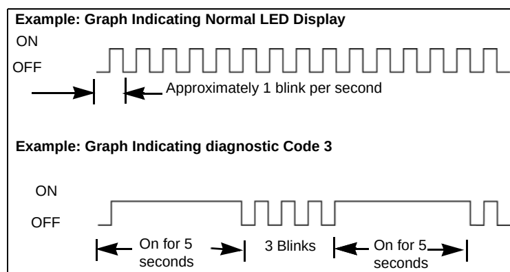
Figure 7: LED Status
