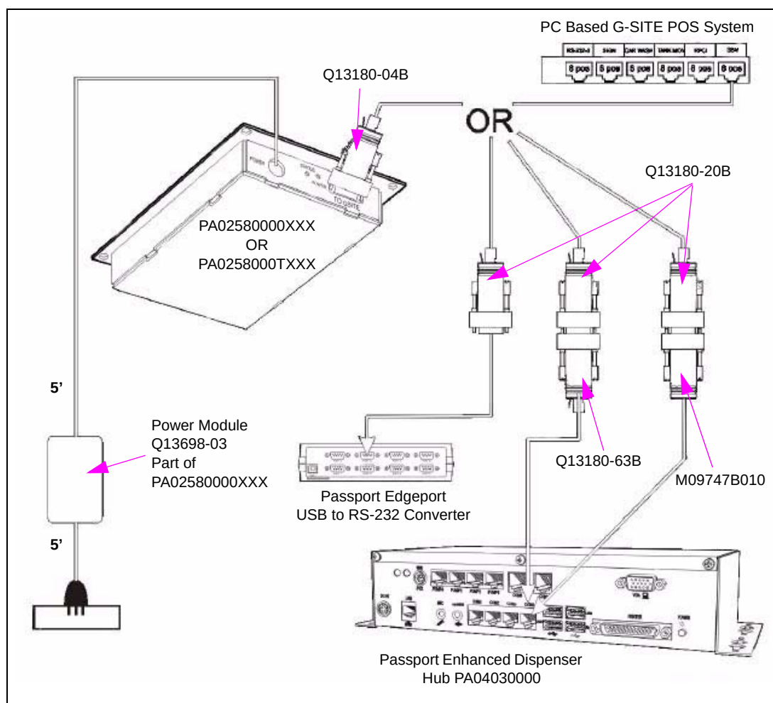
Figure 2: Connecting the CAT-5 Cable
