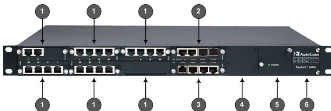
Figure 3-1: Front Panel
