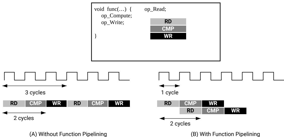
Figure 67: Function Pipelining Behavior
