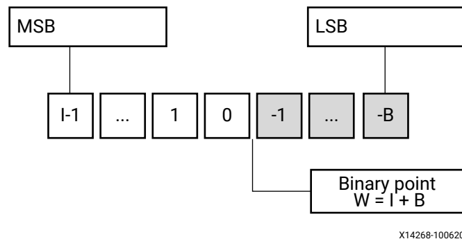
Figure 95: Fixed-Point Data Type
