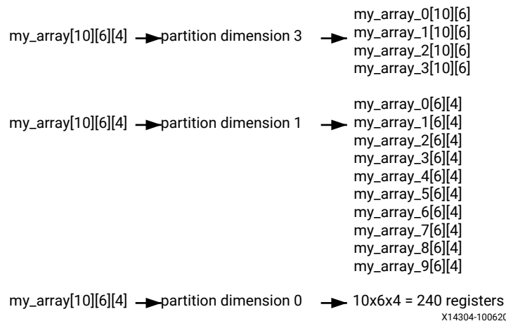
Figure 74: Partitioning Array Dimensions
