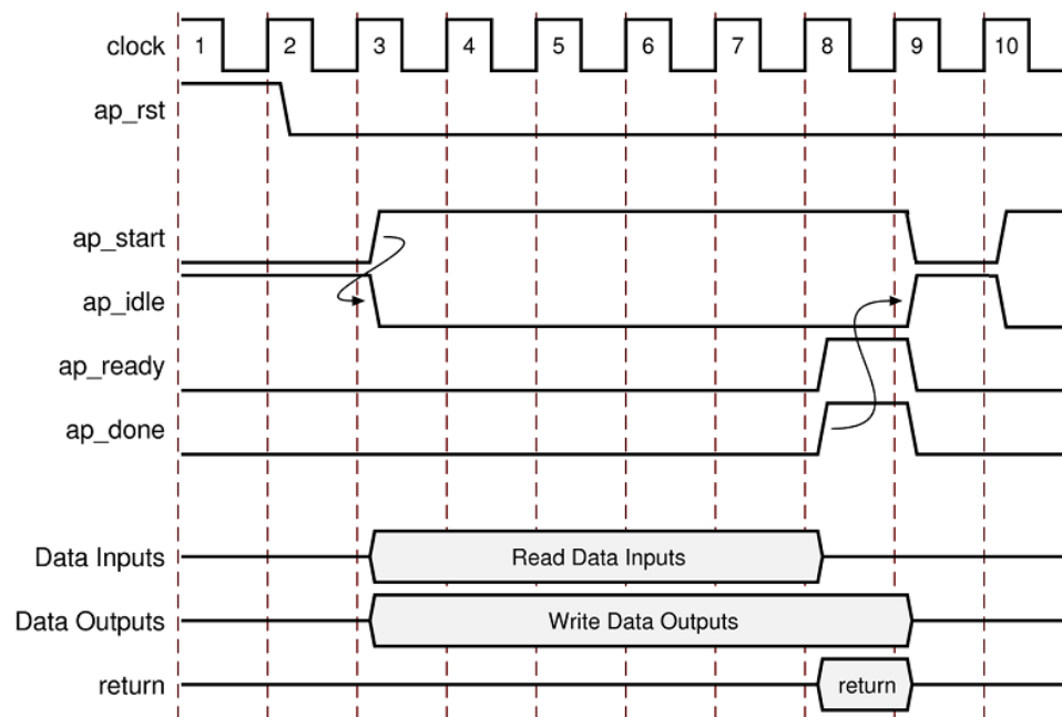
Figure 60: RTL Port Timing with Default Synthesis
