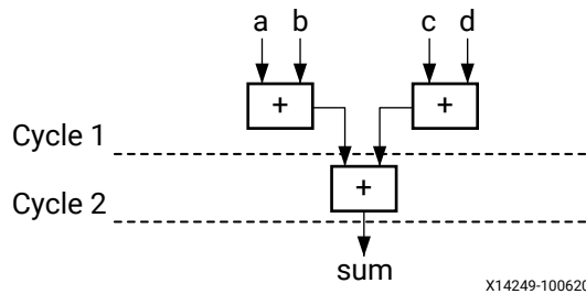
Figure 84: Adder Tree After Balancing
