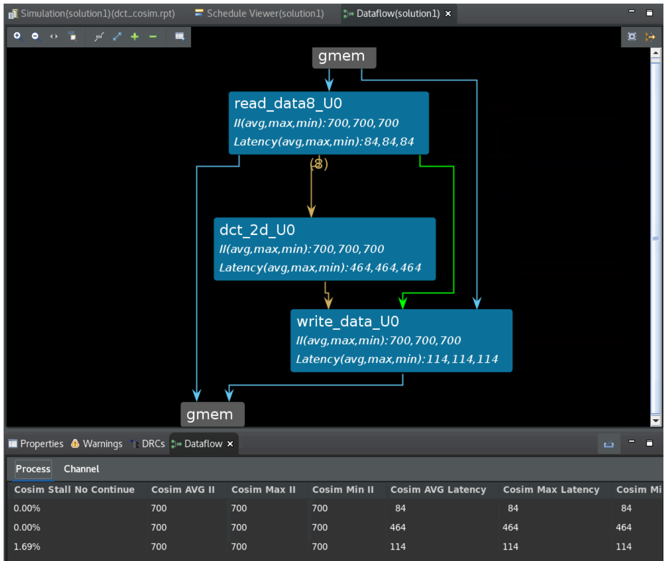
Figure 26: Dataflow Viewer
