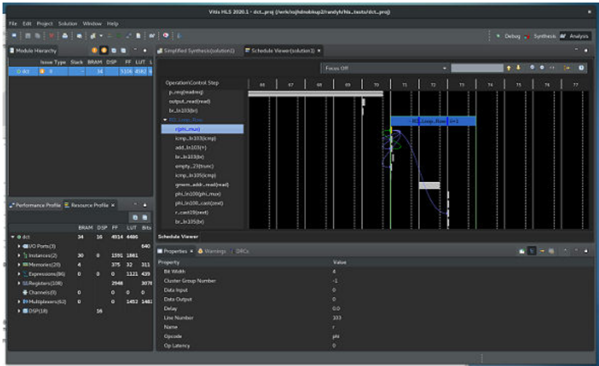
Figure 23: Analysis Perspective
