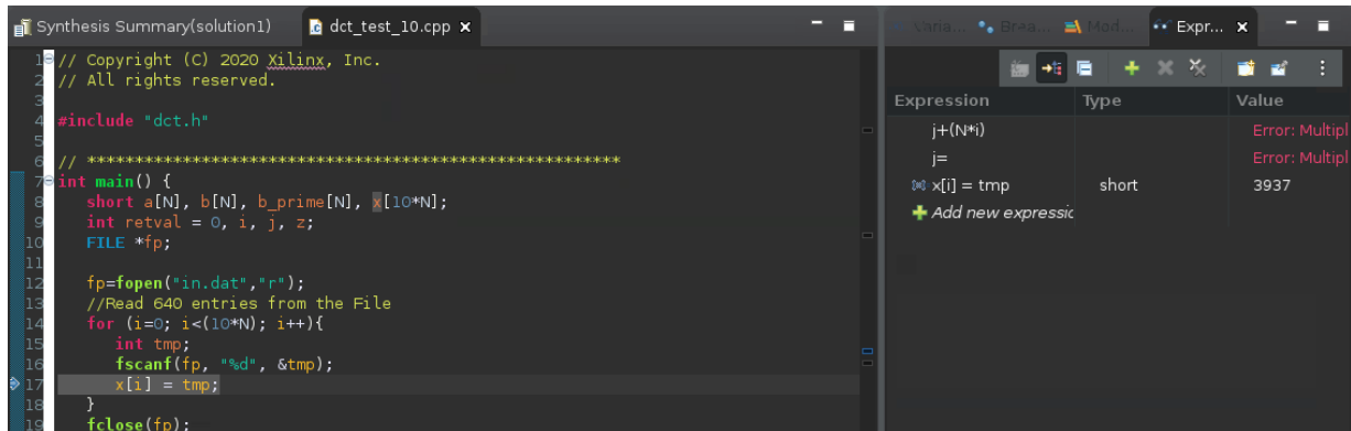
Figure 15: Monitoring Expressions
