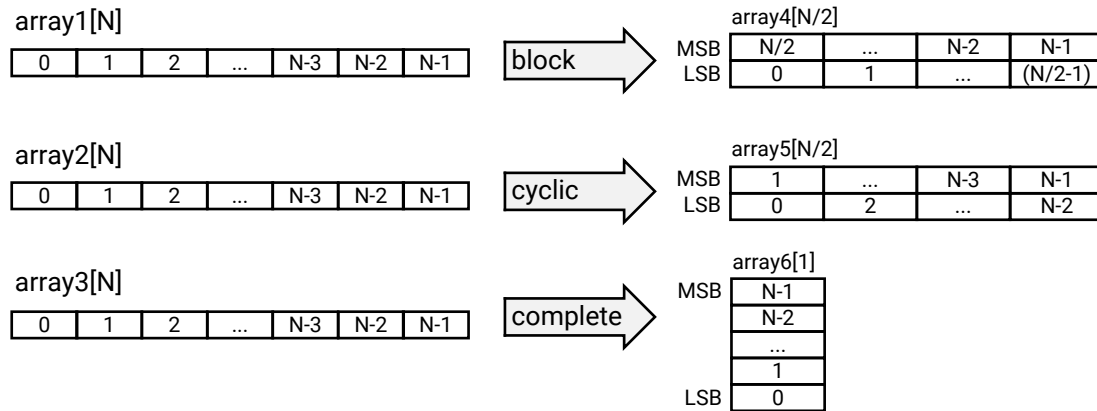
Figure 92: ARRAY_RESHAPE Pragma
