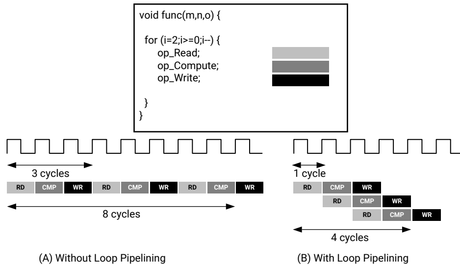
Figure 94: Loop Pipeline
