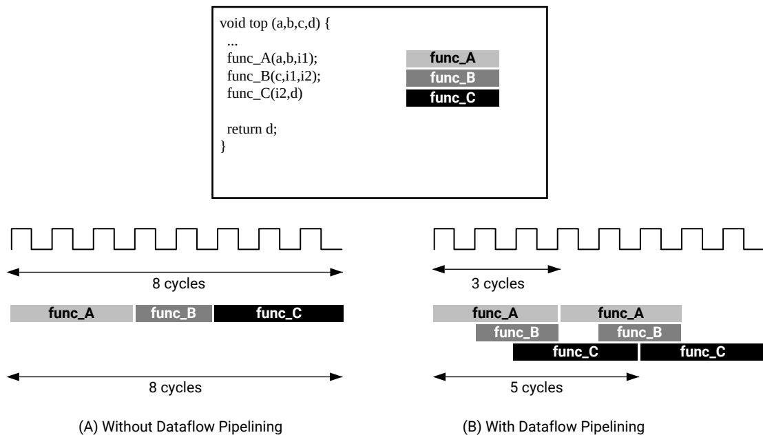
Figure 79: Dataflow Optimization
