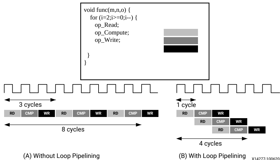
Figure 68: Loop Pipelining
