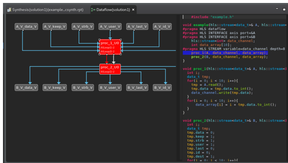
Figure 32: Deadlock Viewer
