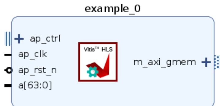
Figure 52: offset=direct
