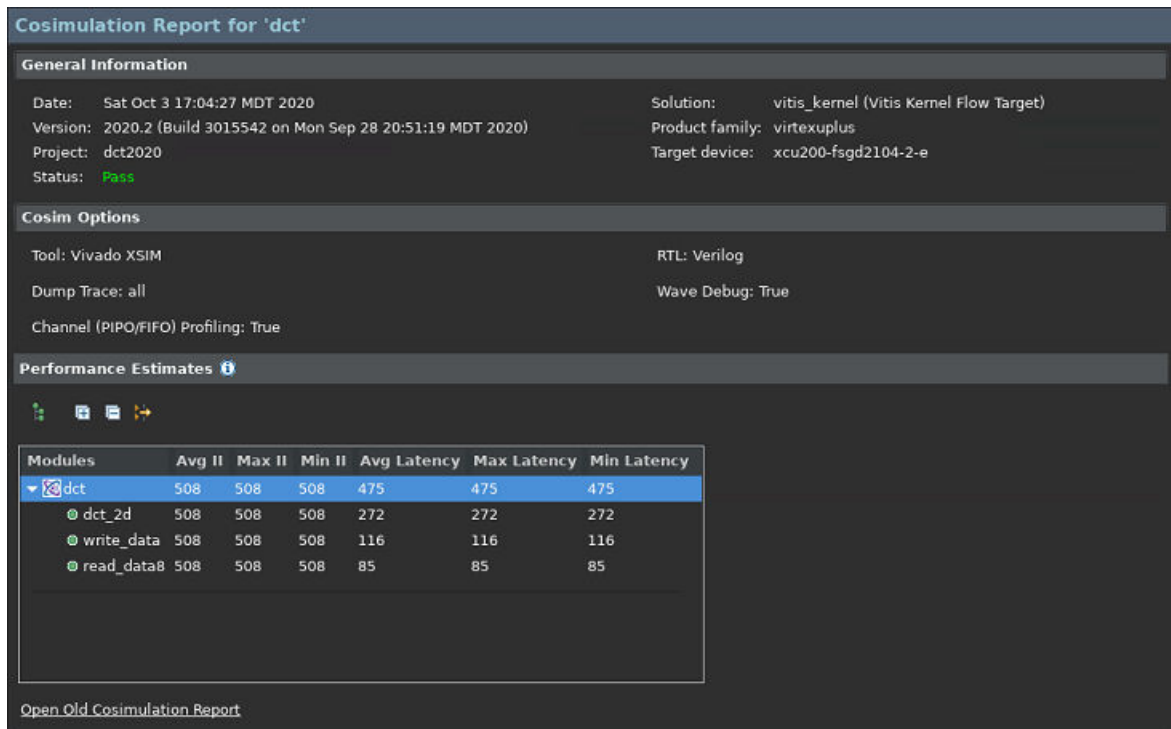
Figure 29: Cosimulation Report
