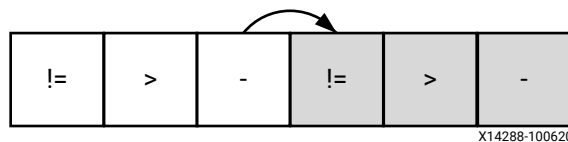
Figure 76: Scalar Dependency
