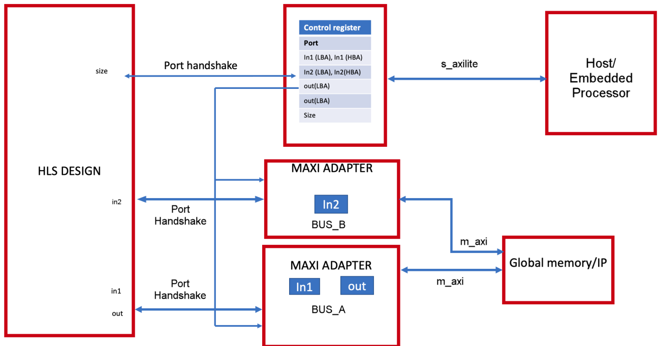
Figure 55: 2 MAXI Bundles
