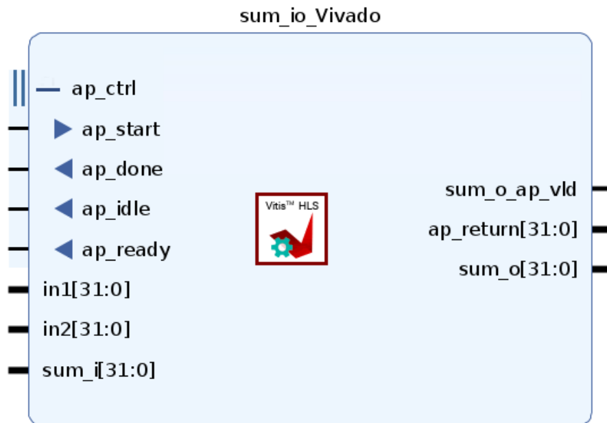
Figure 46: RTL Ports After Default Interface Synthesis
