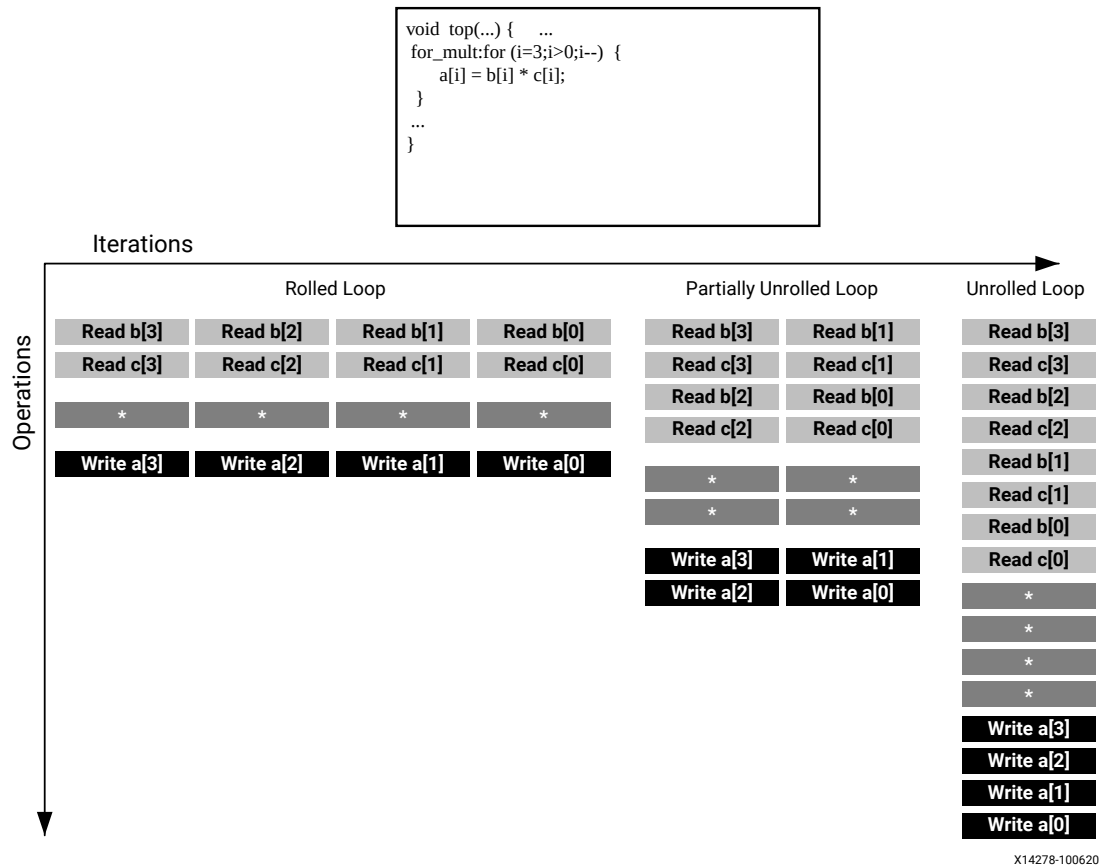
Figure 72: Loop Unrolling Details
