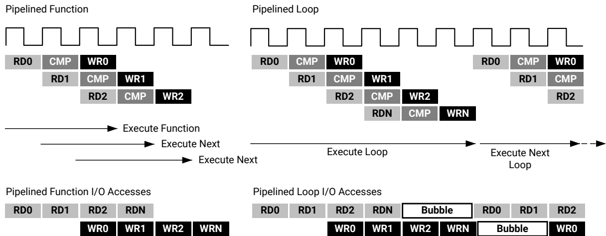
Figure 69: Function and Loop Pipelining Behavior
