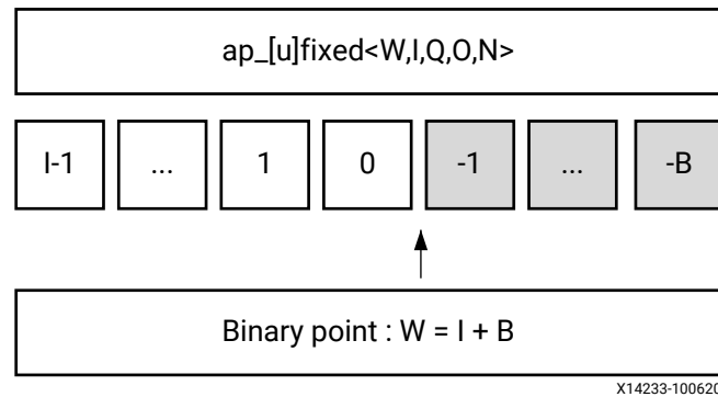
Figure 96: Arbitrary Precision Fixed-Point Types
