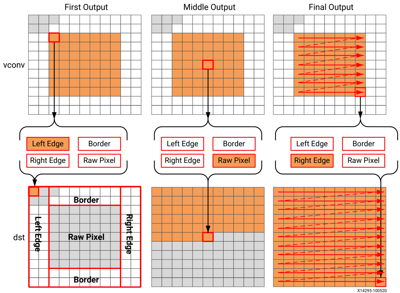
Figure 45: Streaming Border Samples
