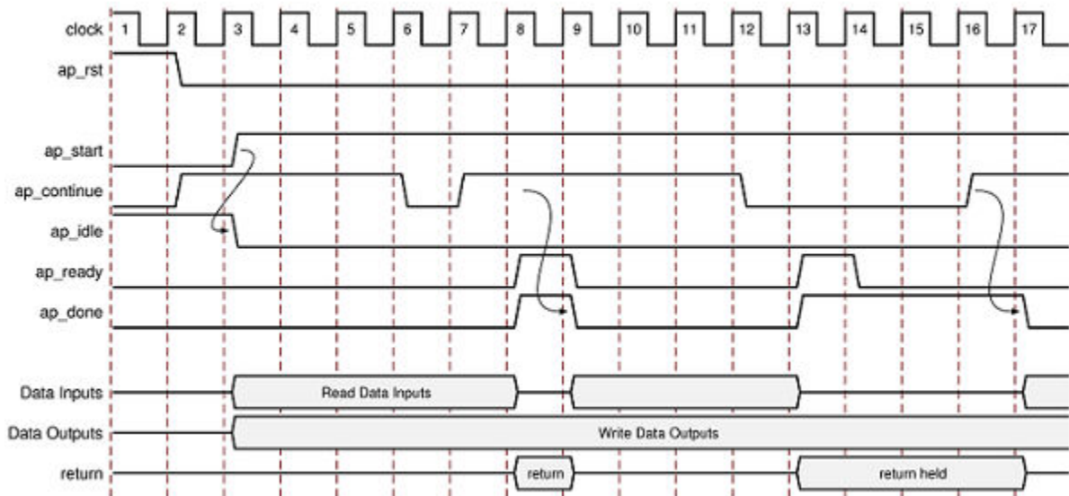
Figure 65: Behavior of ap_ctrl_chain Interface
