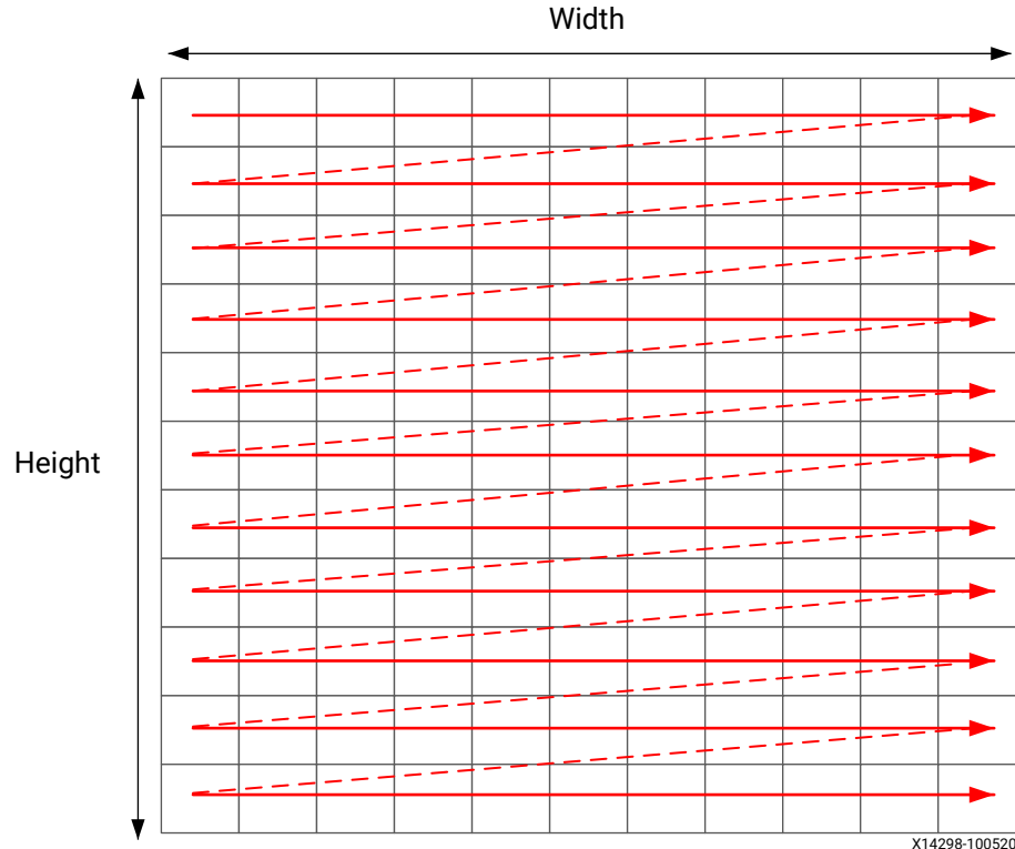
Figure 42: Raster Scan Order
