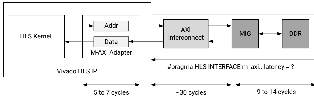
Figure 86: Burst Transaction Diagram
