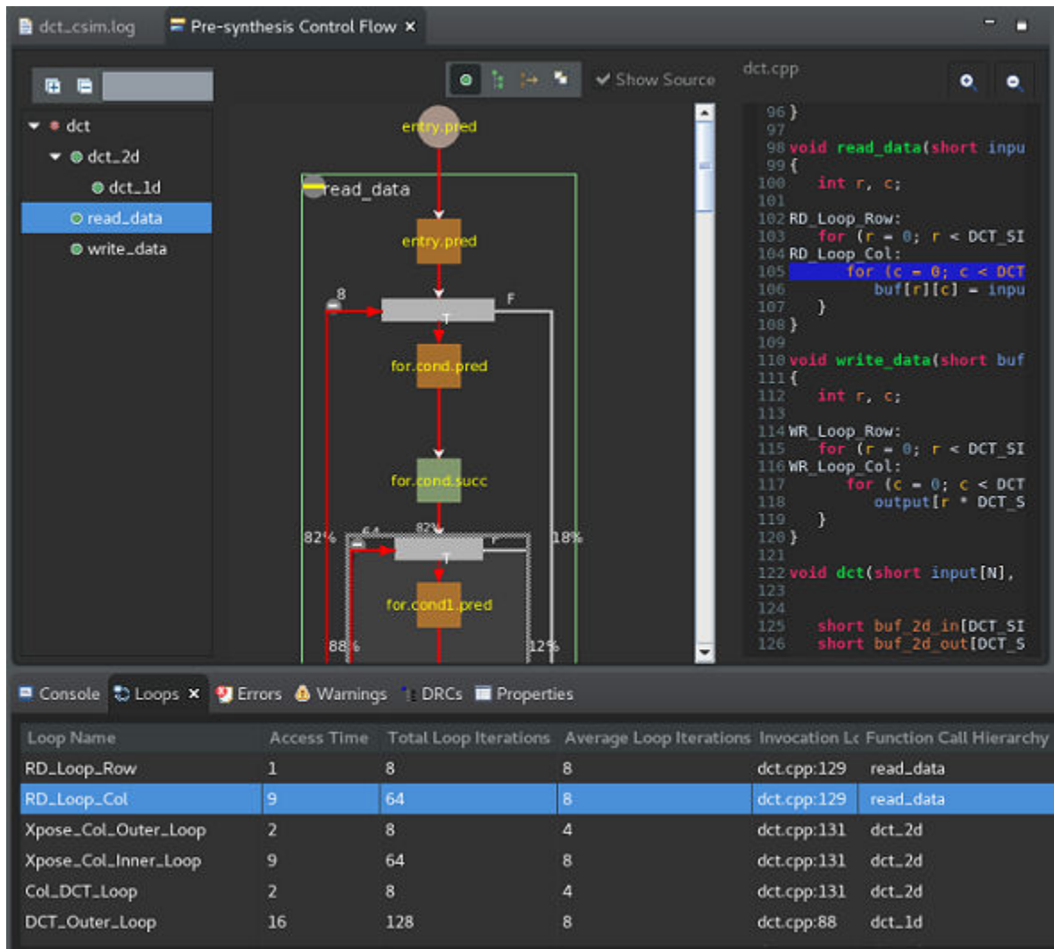
Figure 16: Pre-Synthesis Control Flow Viewer
