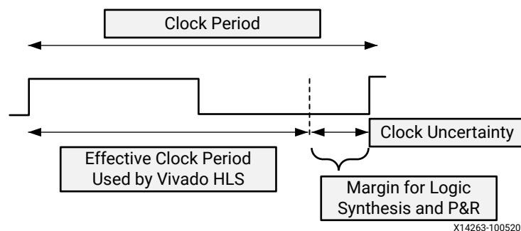
Figure 11: Clock Period and Margin
