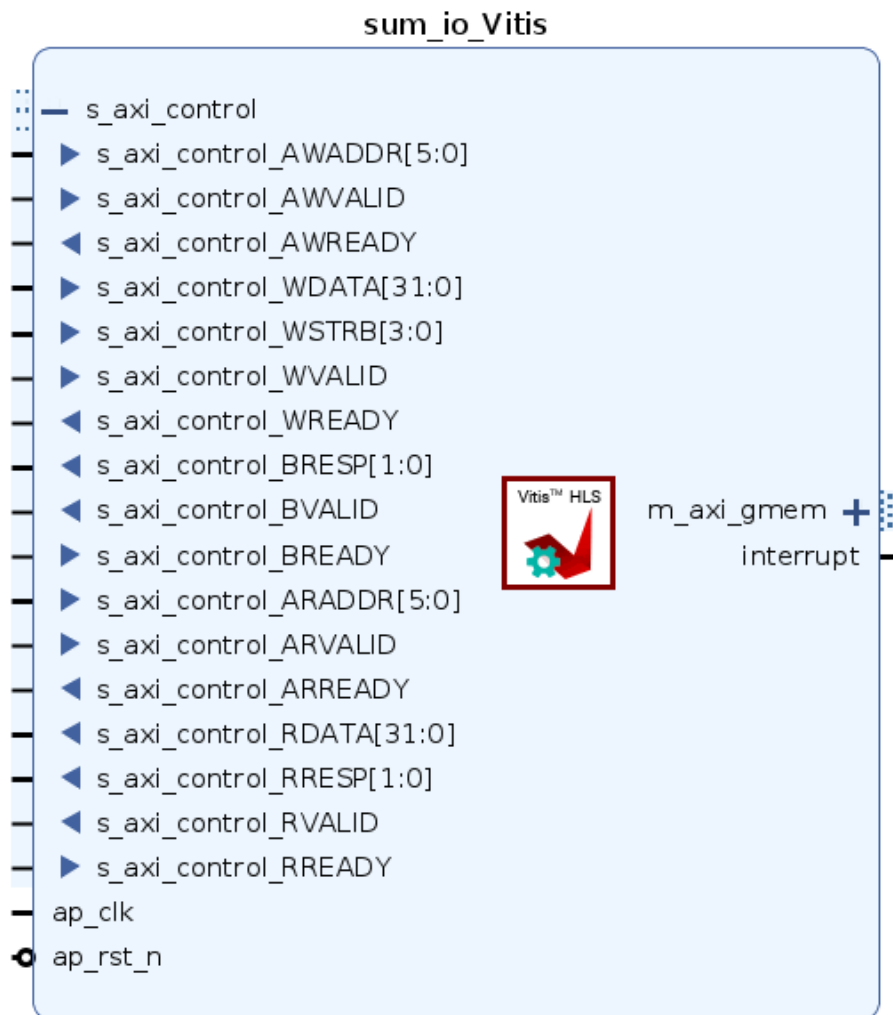
Figure 47: RTL Ports After Default Interface Synthesis
