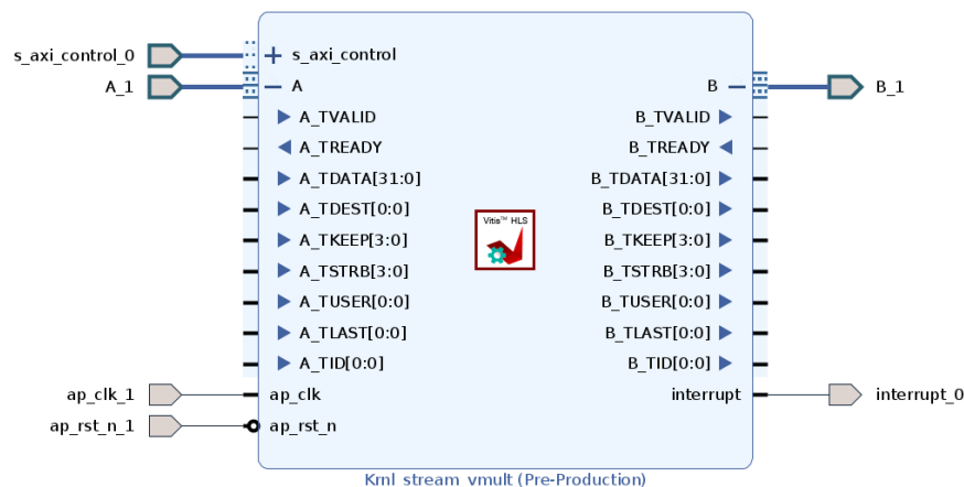
Figure 59: AXI4-Stream Interfaces with Side-Channels
