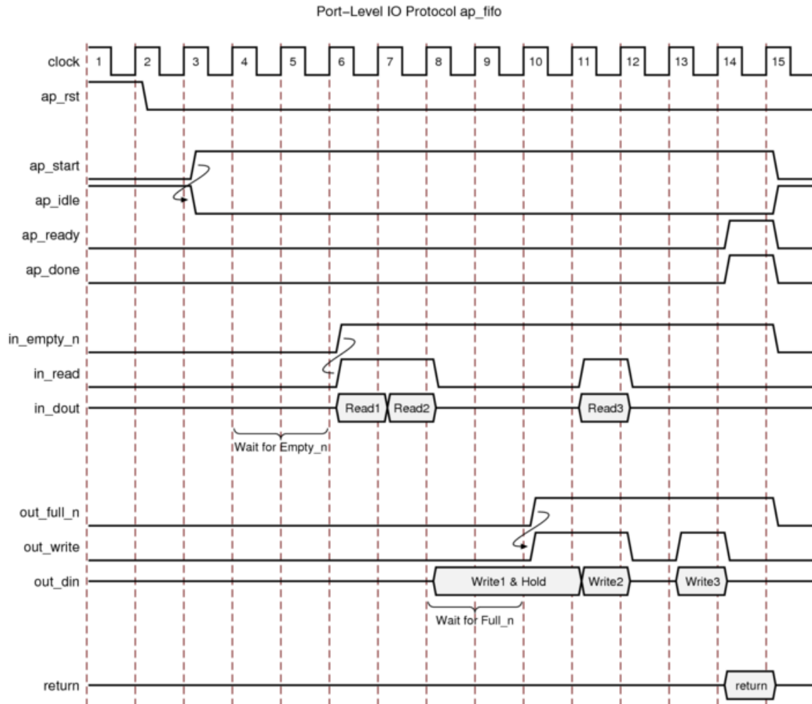
Figure 63: Behavior of ap_fifo Interface
