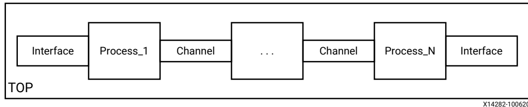
Figure 78: Parallel Process Architecture
