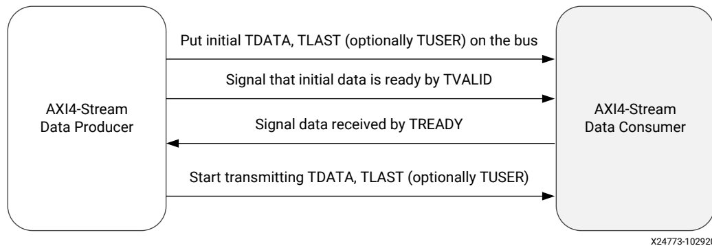
Figure 57: AXI4-Stream Handshake
