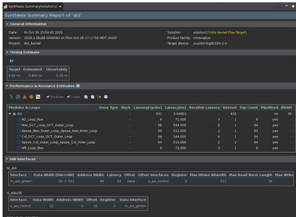
Figure 19: Synthesis Summary Report
