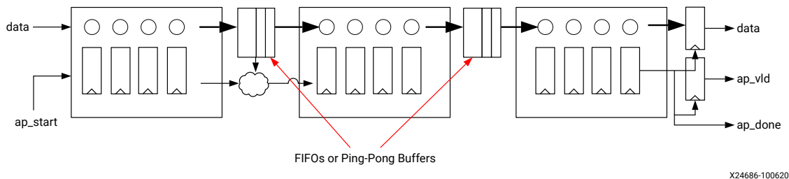
Figure 80: Structure Created During Dataflow Optimization
