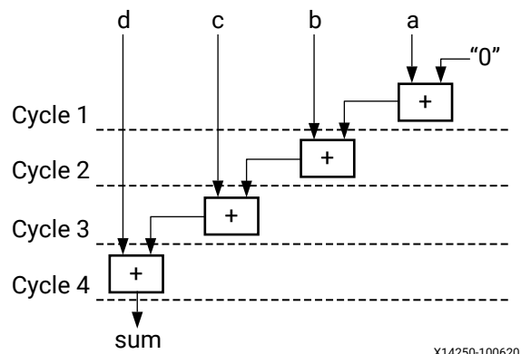
Figure 83: Adder Tree
