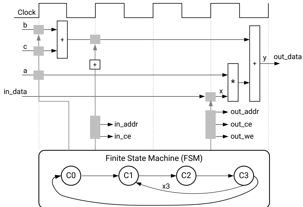
Figure 2: Control Logic Extraction and I/O Port Implementation Example
