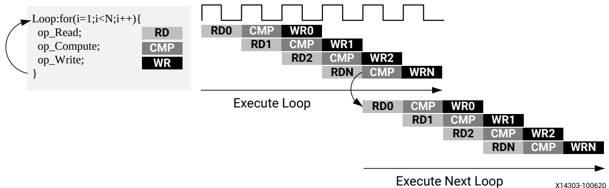
Figure 70: Loop Pipelining with Rewind Option
