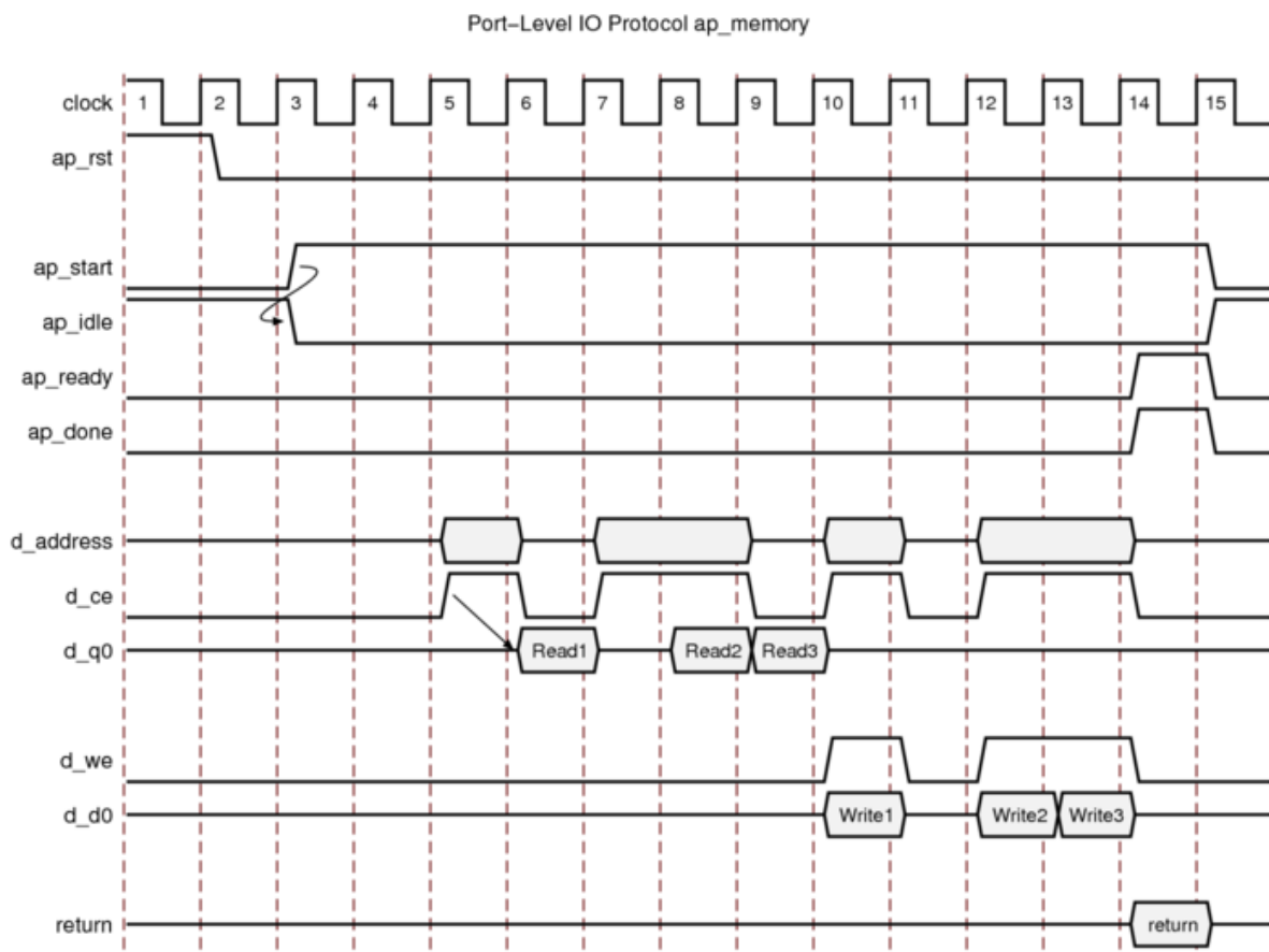
Figure 62: Behavior of ap_memory Interface
