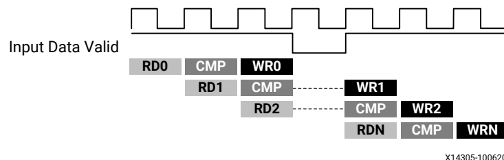
Figure 71: Loop Pipelining with Stall
