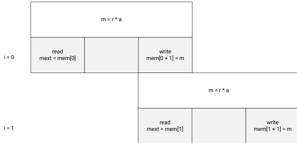
Figure 75: Dependency Example
