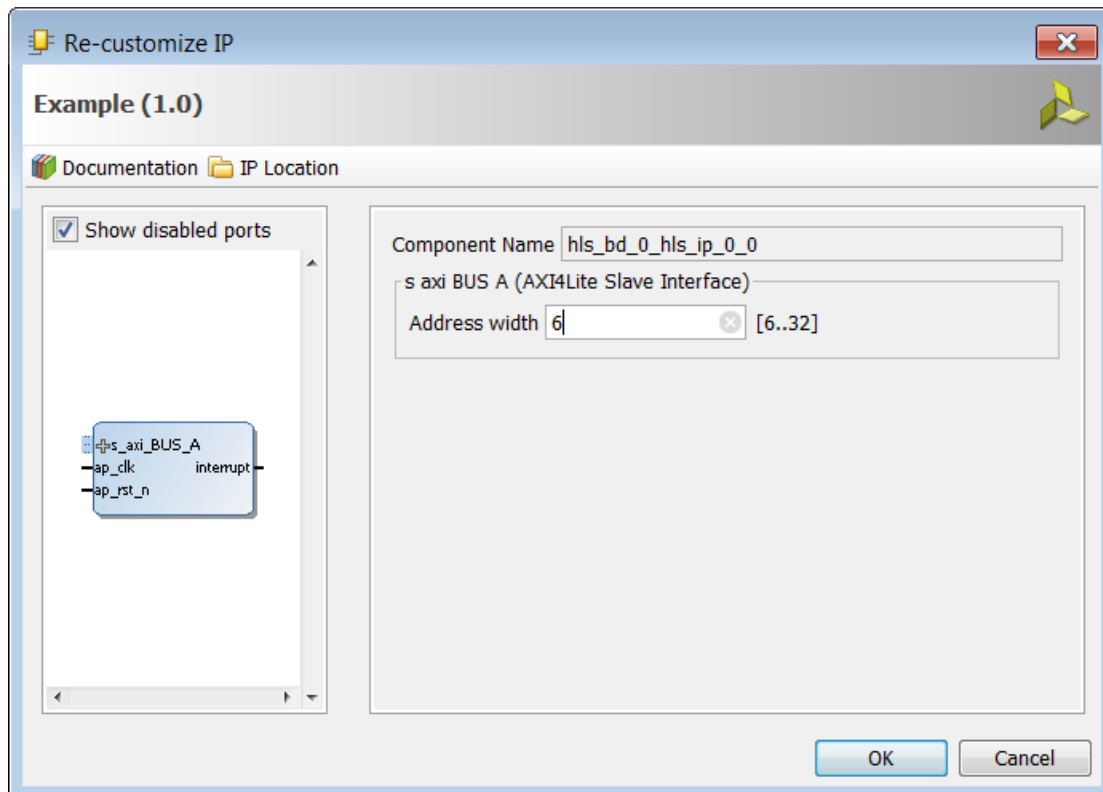
Figure 50: Customizing AXI4-Lite Slave Interfaces in IP Integrator
