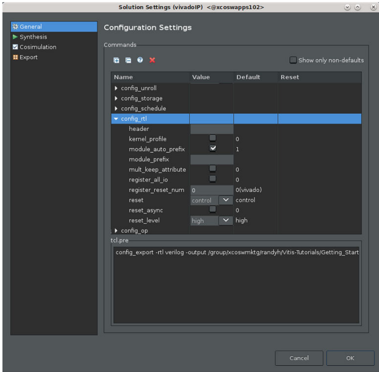
Figure 66: RTL Configurations
