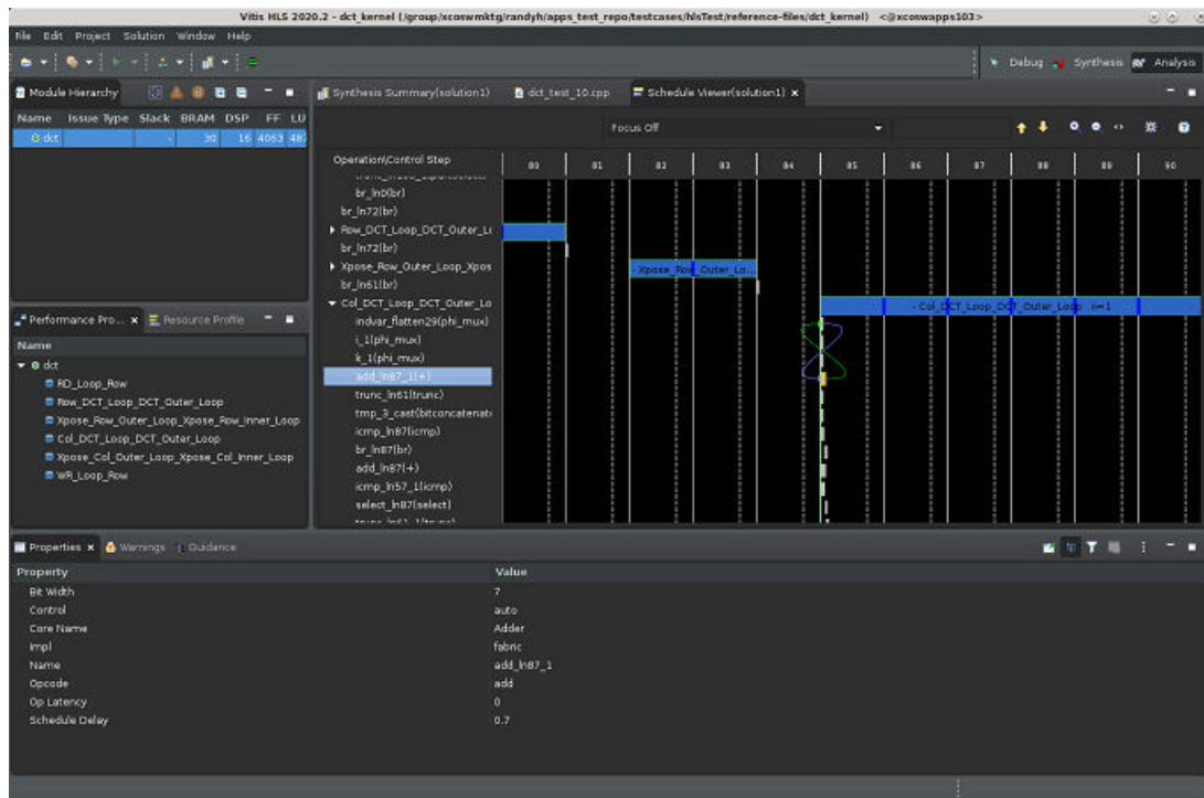
Figure 24: Schedule Viewer
