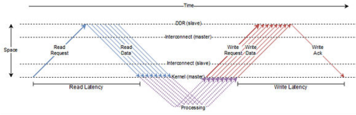
Figure 85: AXI Protocol
