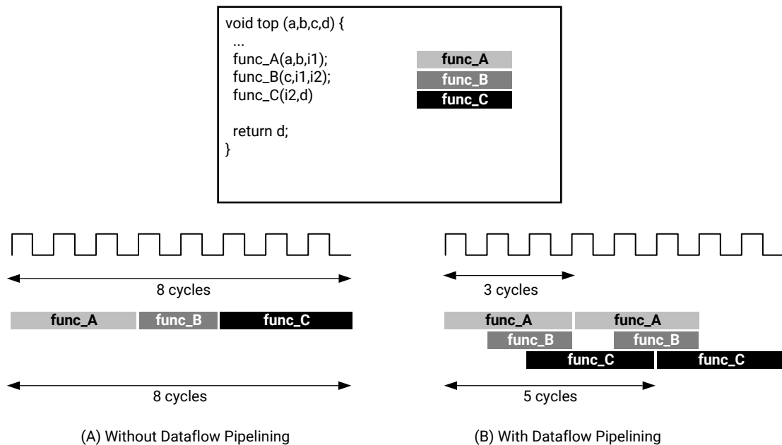
Figure 93: DATAFLOW Pragma
