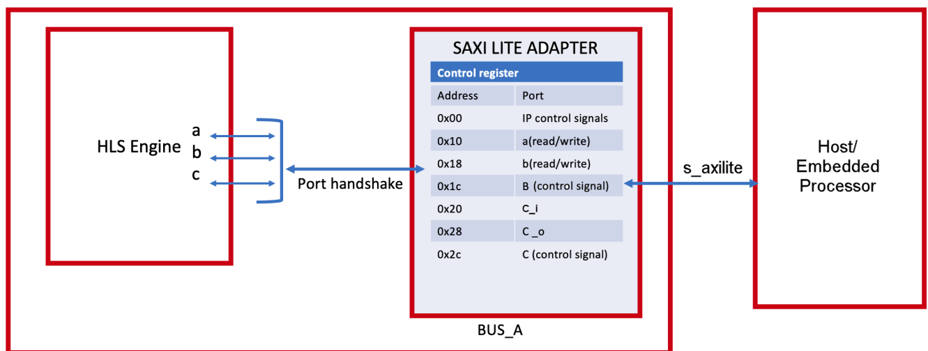
Figure 49: S_AXILITE Adapter
