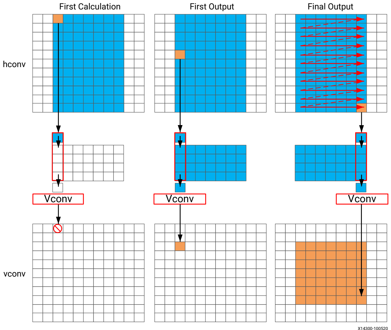
Figure 44: Streaming Vertical Convolution
