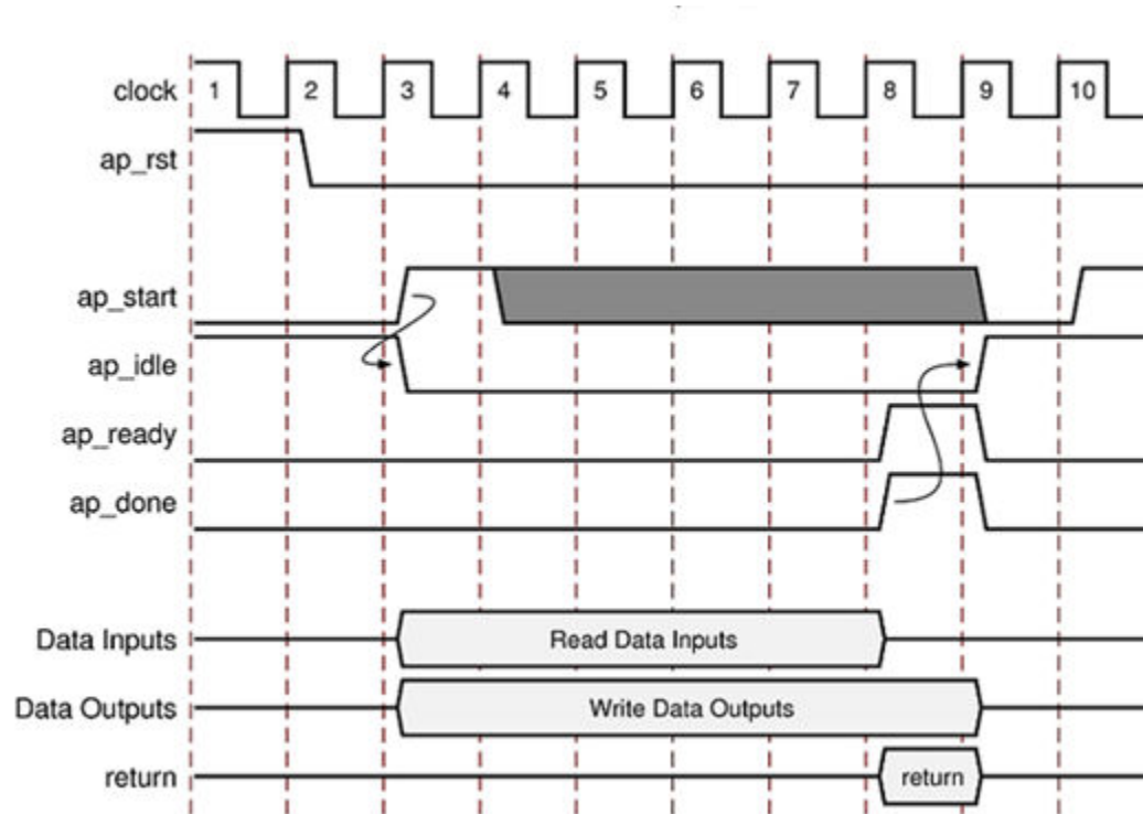
Figure 64: Behavior of ap_ctrl_hs Interface
