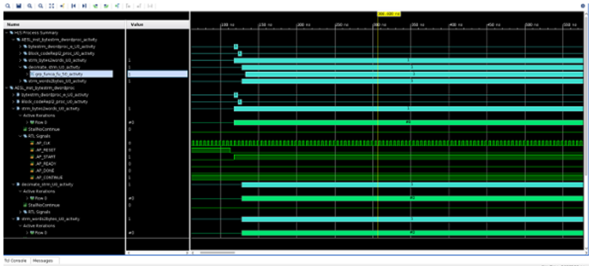
Figure 31: Waveform Viewer
