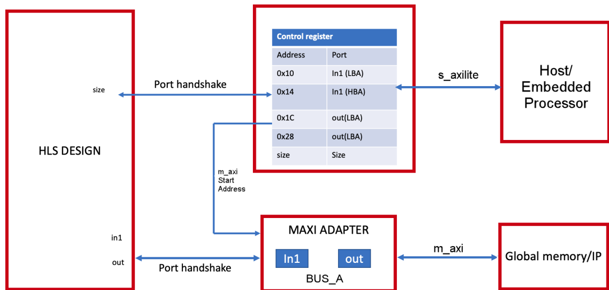
Figure 54: MAXI and S_AXILITE
