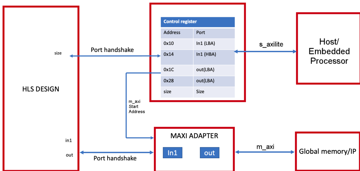
Figure 53: AXI Adapters in Slave Mode
