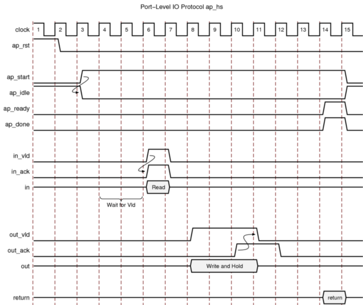
Figure 61: Behavior of ap_hs Interface
