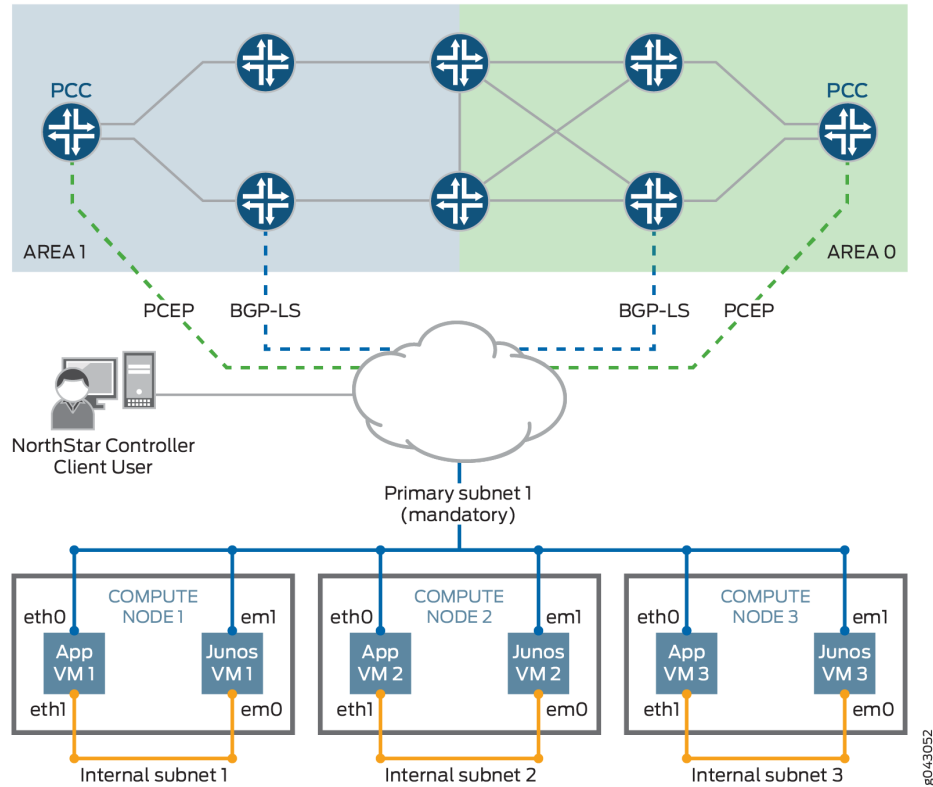
Figure 20: OpenStack Environment, Cluster Mode
