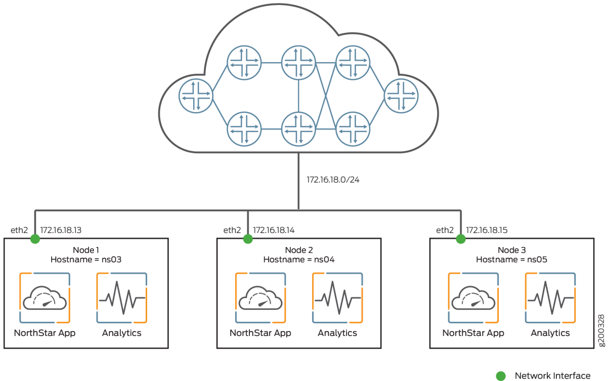
Figure 23: NorthStar HA Cluster Nodes with Analytics
