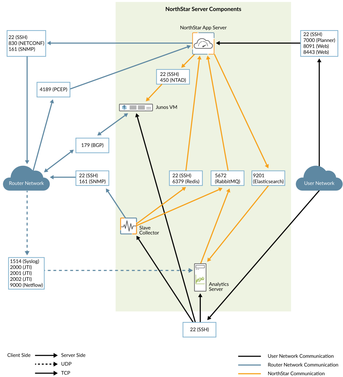
Figure 2: NorthStar Main Port Map
