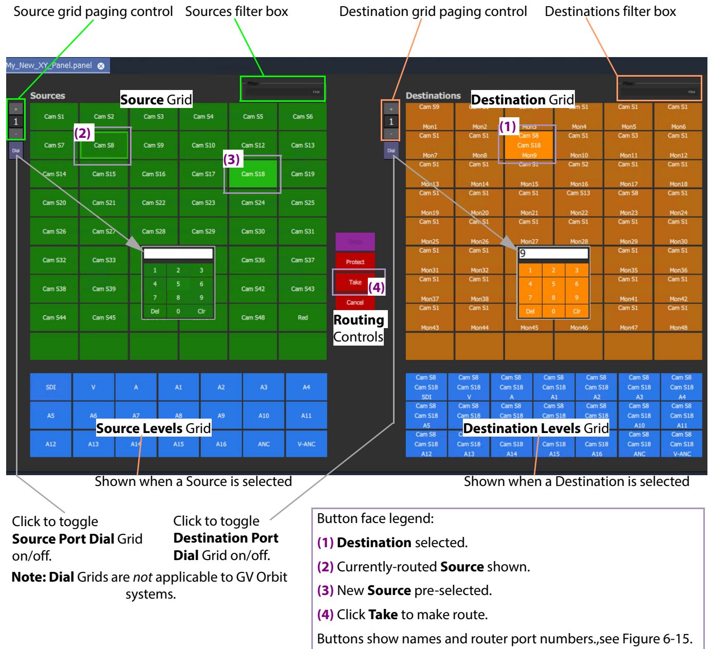
Fig. 6-12: New XY Panel Layout and Controls (Annotated, 'Run' Mode)
