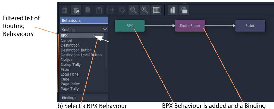
Fig. 6-51: Adding a BPX Behaviour
