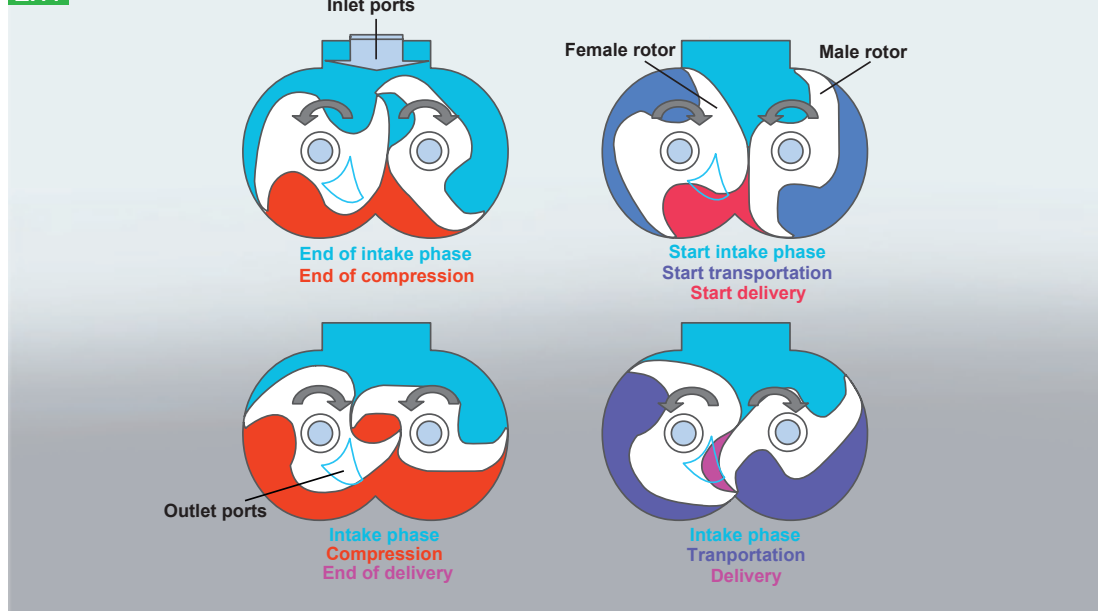
Compression principle of the double tooth compressor.
