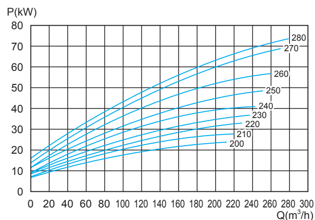
性能曲线 Performance Curve
