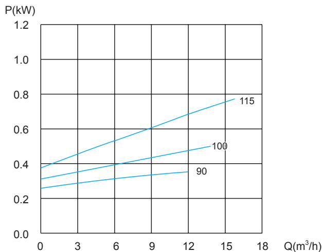
性能曲线 Performance Curve
