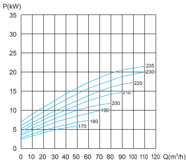
性能曲线 Performance Curve
