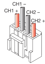
Loudspeaker wires housing: JST VHR-4N
