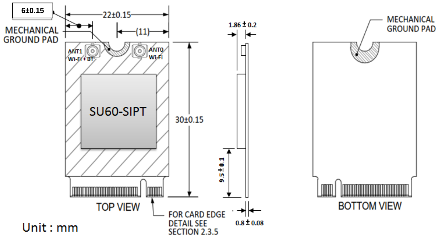
Figure 8: Module dimension of ST60-2230C/ST60-2230C-SS/ST60-2230C-U/ST60-2230C-UU
