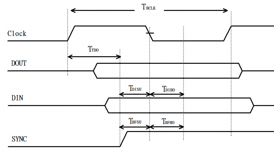
Figure 7: PCM Timing Specification – Slave Mode
