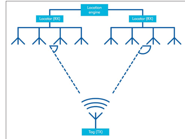
Bluetooth 5.1 Direction Finding supported by the nRF52833 SoC enables positioning applications that not only rely on received signal strength indication (RSSI) but also the signal direction. Illustrated here is an example of a real time location system (RTLS) where the principle of Angle-of-Arrival is used to determine tag location
