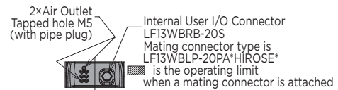
VIEW D
