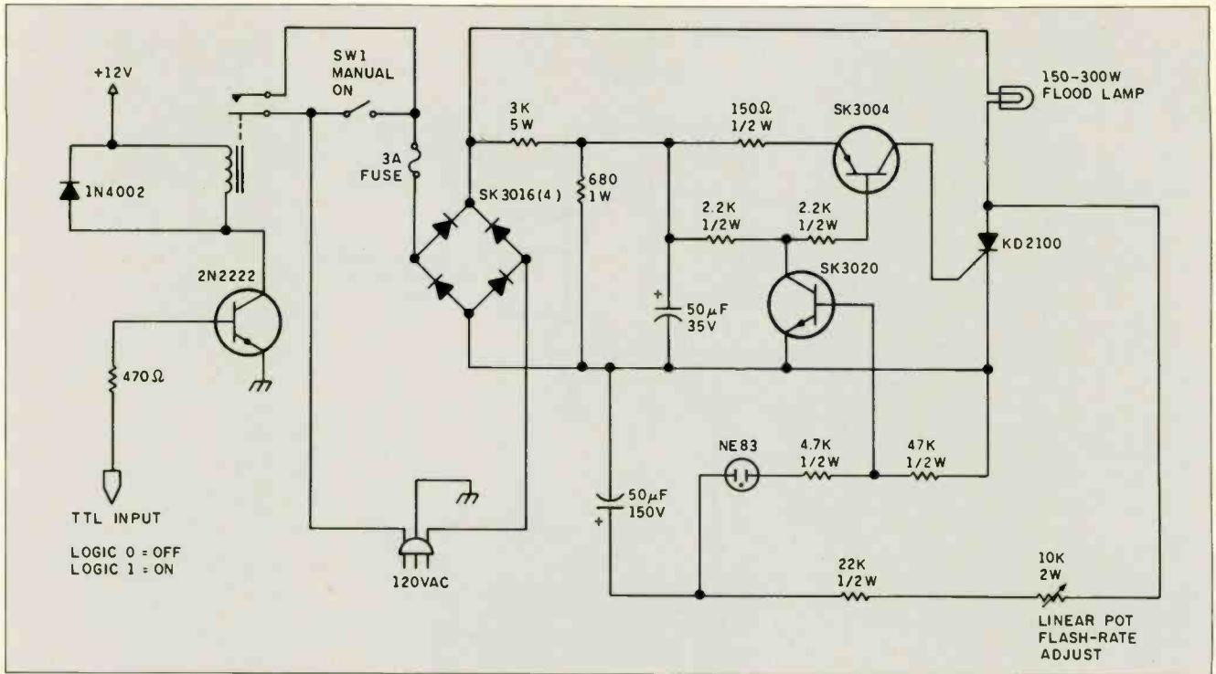
Figure 23: A 115-V AC incandescent lamp flasher.
