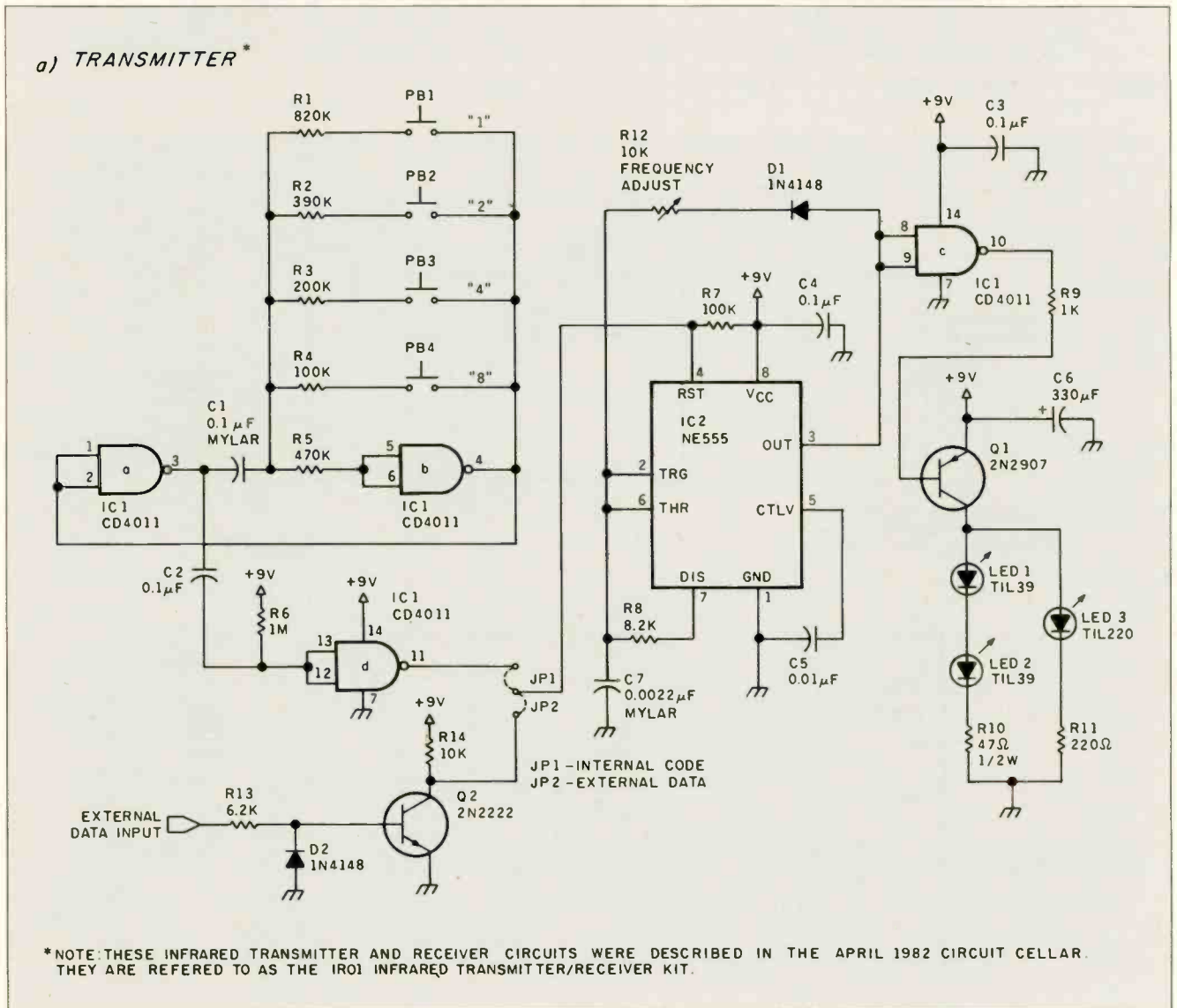
Figure 12: The IRO1 Infrared Transmitter/Receiver.
