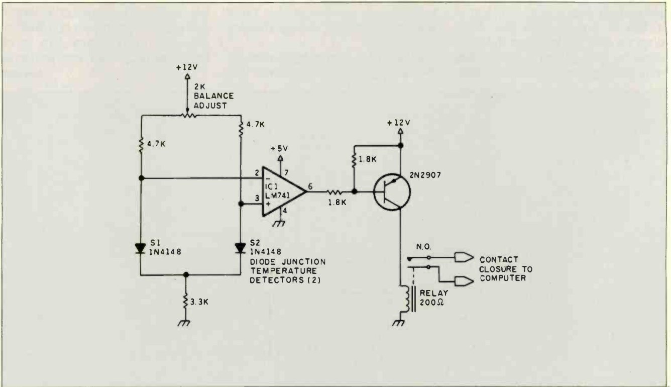
Figure 17: A differential-input temperature detector.
