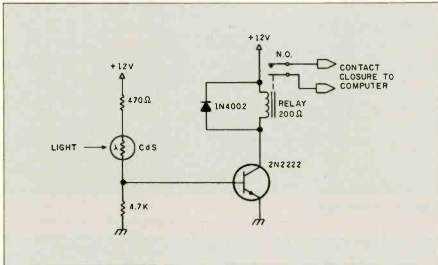
Figure 9: A day/night sensor.
