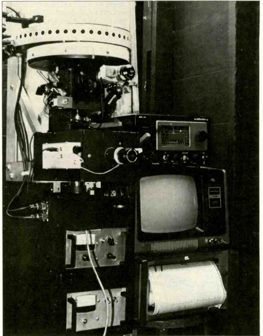
Photo 2: The early data-logging system as installed at the Fairborn Observatory (East) in 1979. The photometer, mid-left, was attached to the telescope, upper left. Photometer electronics are on the lower left. The video monitor on the right was tied to the Radio Shack TRS-80 located some distance away in a warm room. We communicated with the computer via a hand-held hexadecimal keypad. The system was used for several years to make observations of spotted RS Canum Venaticorum binary stars for Douglas Hall at Vanderbilt University. It has been superseded by a fully automatic system that was recently moved from Ohio to Arizona, the location of the Fairborn Observatory (West).
