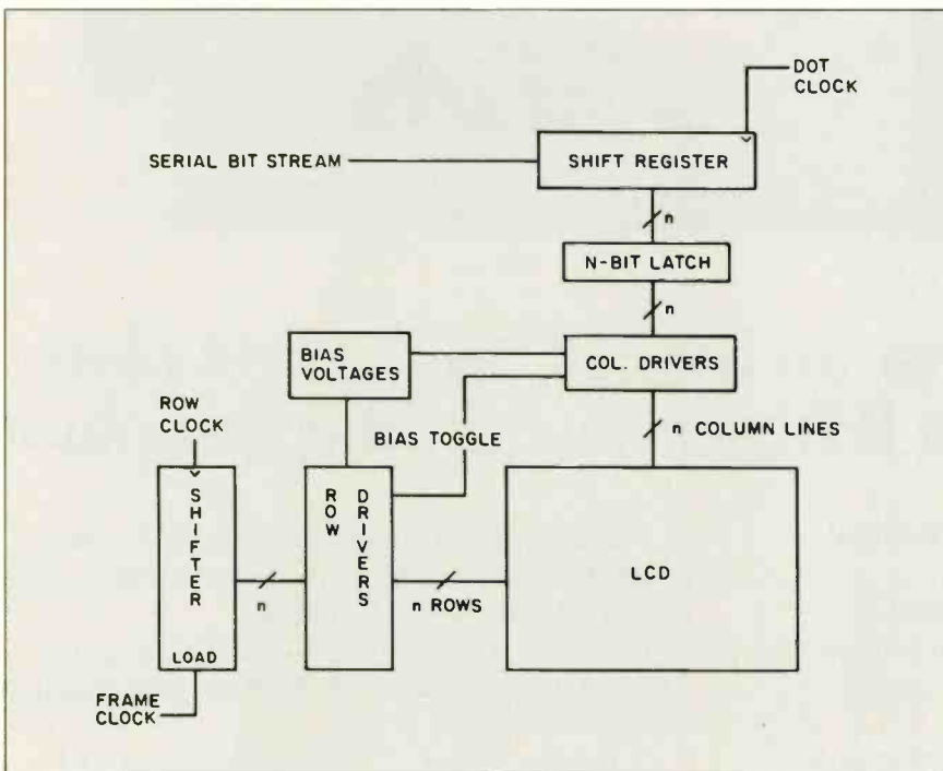
Figure 6: Circuit schematic for an LCD quadrant. Dots are shifted on the fall of dot clock. Values are moved from the serial shifter to the n-bit latch and a new row is selected by the fall of row clock. Frame clock resets the row sequencer and initiates the next frame. The bias toggle along with the dot value determines the voltages driven on the row and column lines.
