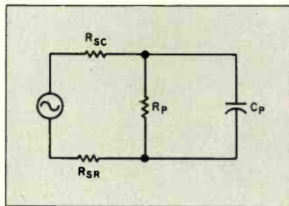
Figure 3: C_p and R_p represent the capacitance and resistance, respectively, of a pixel: Typical values are 2\text{ nF/cm}^2 for C_p and 12\text{ Mohm/cm}^2 for R_p . R_{sc} and R_{sr} are sheet resistances of the row and column conductors. For indium-tin-oxide their value lies between 10 and 300 ohms per square.
