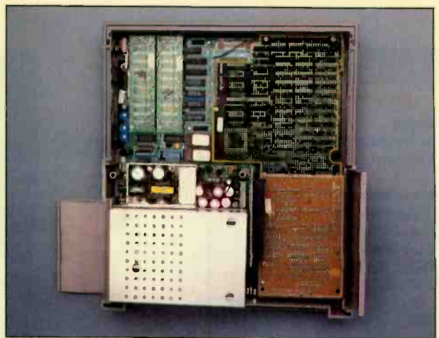
A top view inside the Pro-Lite
