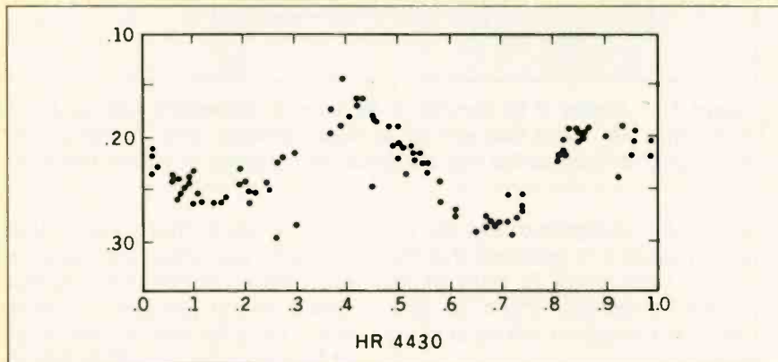
Figure A: Light curve for HR 4430.
