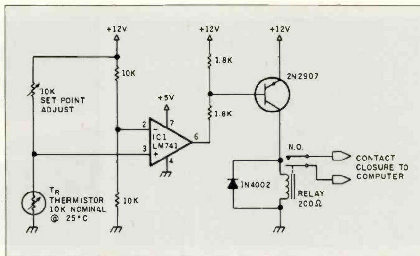
Figure 16: An under-temperature alarm.
