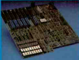
80286 motherboard, 256K standard memory, upgradable to 1M. Clock upgradable to 8MHz.
