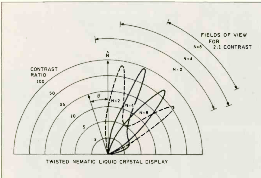
Figure 5: Multiplexing as it relates to contrast and viewing angle for a transmission mode LCD. Concentric rings represent measured contrast ratio (CR) of "off" to "on" pixels. Theta, \theta , is the displacement of viewing angle from the normal direction, \hat{N} . The response of a liquid-crystal medium for three different levels of multiplexing, N , is shown.
