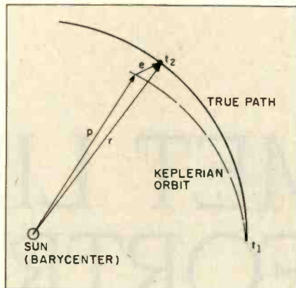
Figure 1: Illustration of Encke's model for calculating orbits around the sun; p is the radius vector of the Keplerian orbit, r is the radius vector of the true orbit, and e is the perturbation (the difference between p and r ).
