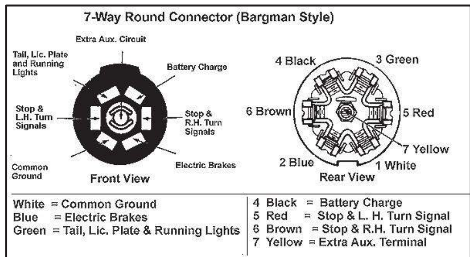
Figure 9-14: Seven-Pin Connector
