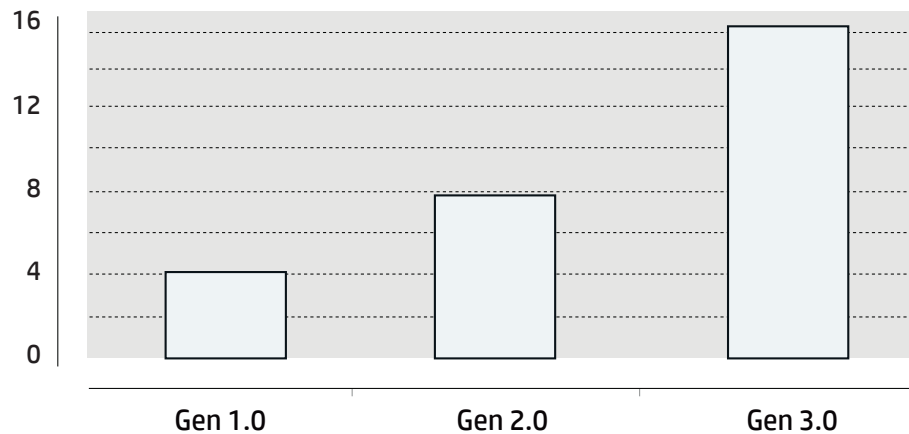
Figure 2. x16 Peak Bandwidth per Direction- GB/s
