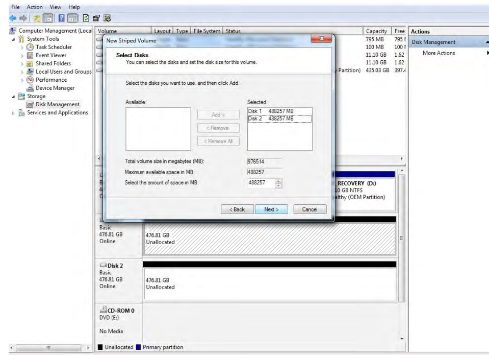
Figure 9. Drive selection
