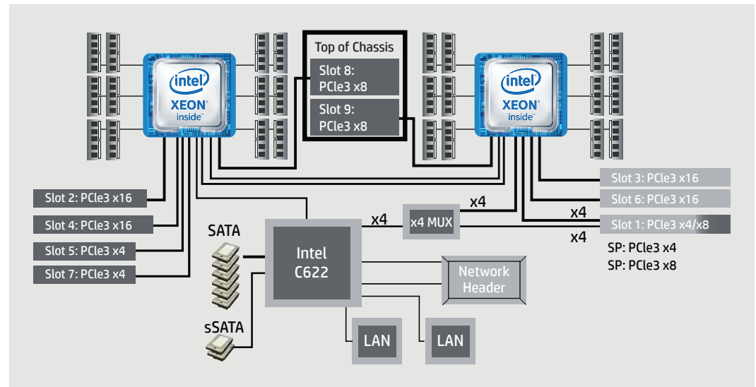
Figure 1. HP Z8 Workstation Block Diagram
