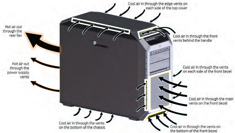
Figure 17. – HP Z8 G4 System Airflow
