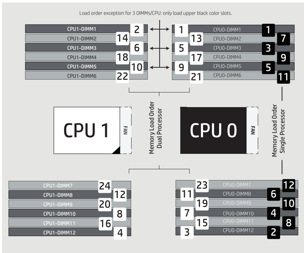
Figure 16. Loading order for single and dual CPU configurations.
