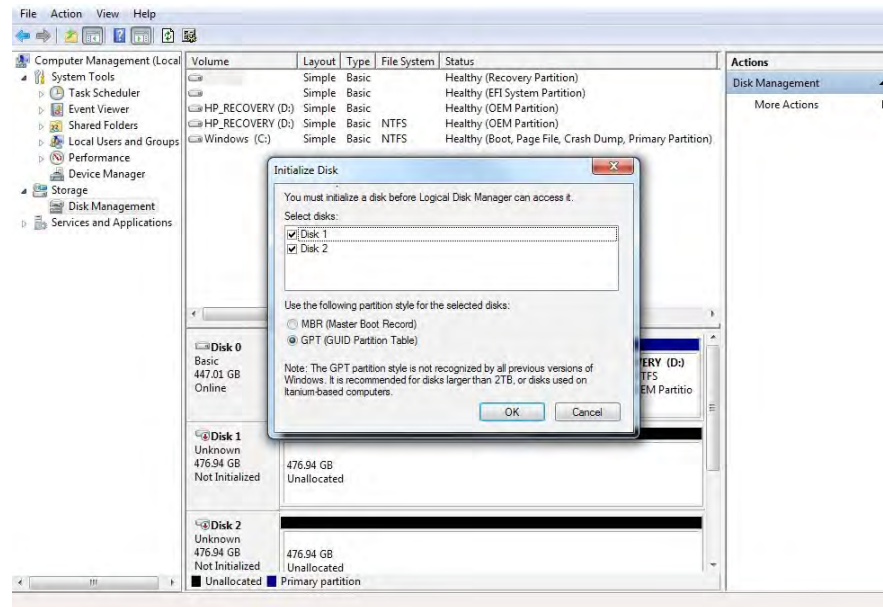
Figure 4. Initialize disk
