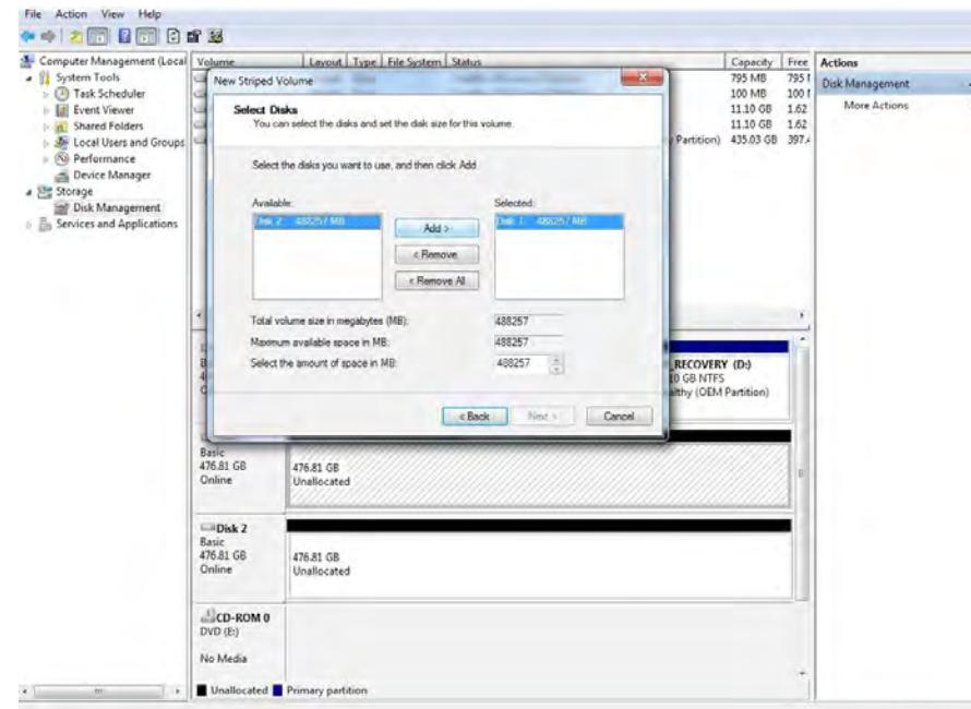
Figure 8. Drive selection
