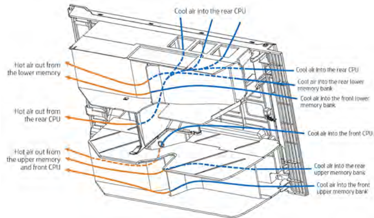
Figure 18 – HP Z8 G4 Memory and CPU Duct Airflow
