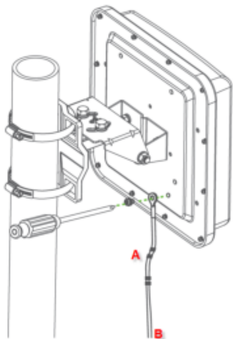
Figure 12 Grounding Example
