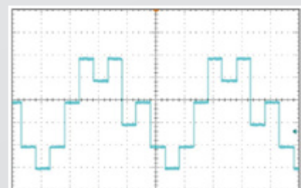
100 Sequences
