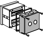
Splashproof rear cover #FPM-5000-SBCK
