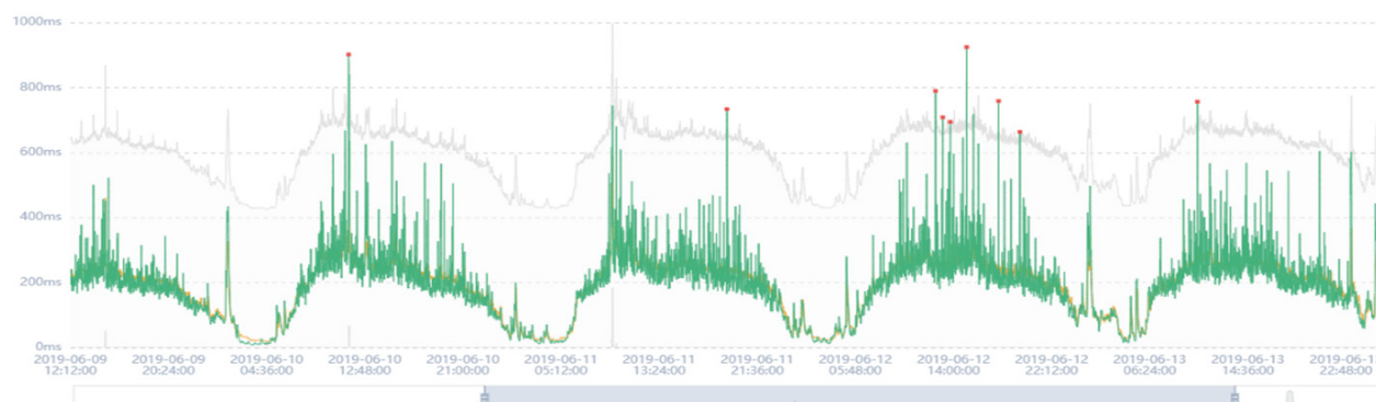
Figure 3-14 Effect of dynamic threshold-based exception detection
