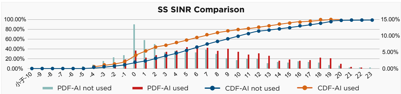
Figure Test Result of Intelligent Parameter Optimization-SS SINR
