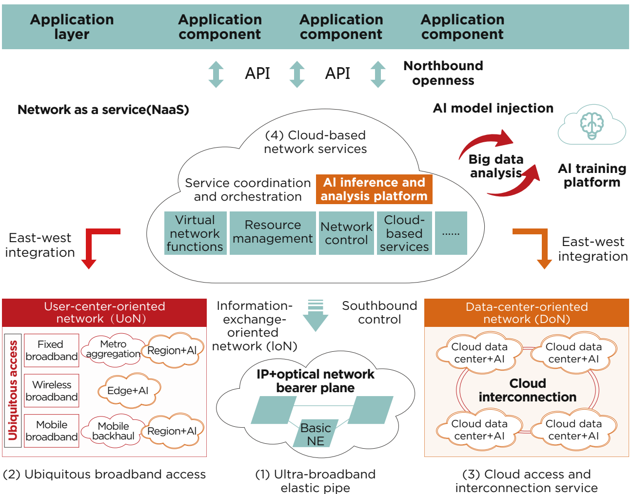
Figure 1-5 Architecture of China Unicom's CUBE-Net2.0+ network
