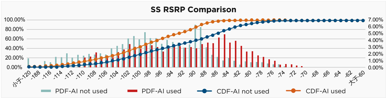
Figure Test Result of Intelligent Parameter Optimization-SS RSRP
