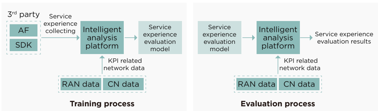
Figure 3-28 Process of offline training and online evaluation
