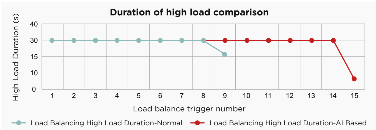
Figure Test Result of Load Balancing - Comparison of Duration of High Load
