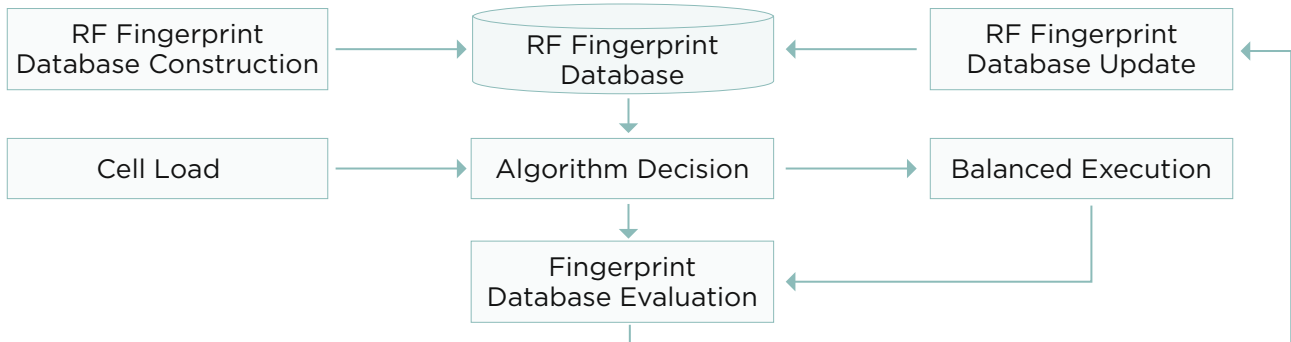
Figure Load Balancing Solution Procedure
