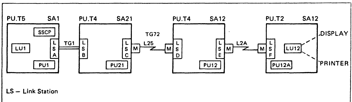
Figure 13-2. Sending a Multiple Element Request Chain
