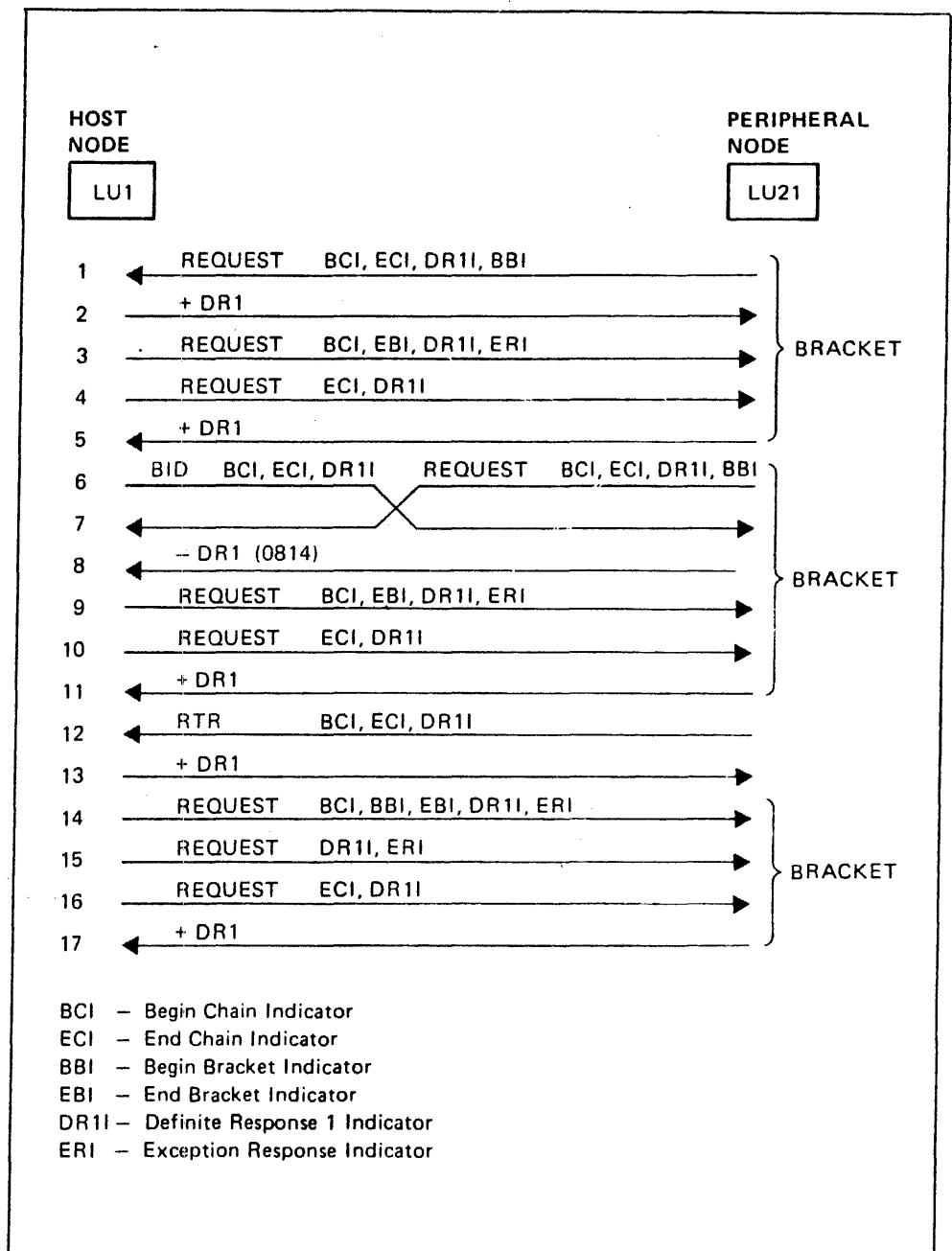
Figure 8-7. Use Of The BID and RTR Request
