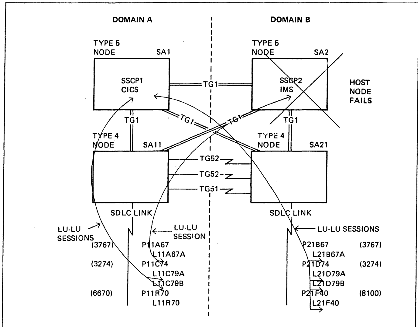
Figure 12-11. Host Node Fails
