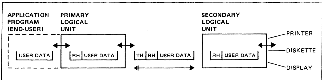
Figure 10-2. Terminal LU With Multiple End Users
