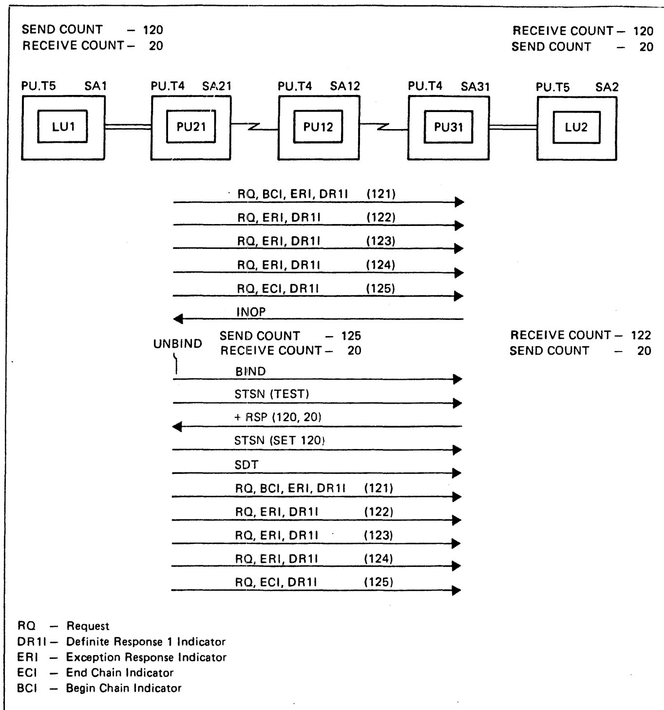
Figure 13-3. Using STSN Request
