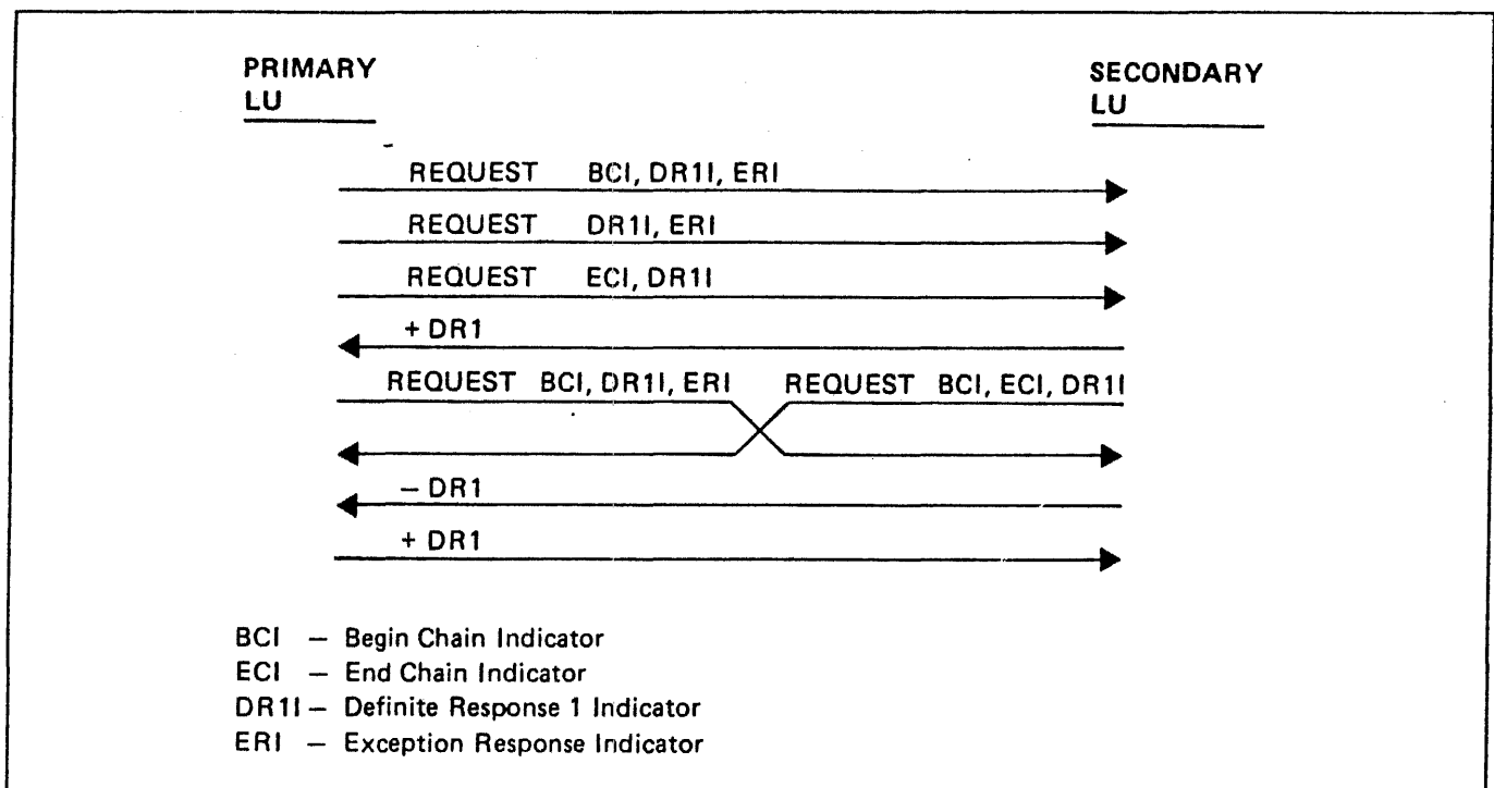
Figure 8-4. Half-Duplex Contention Protocol
