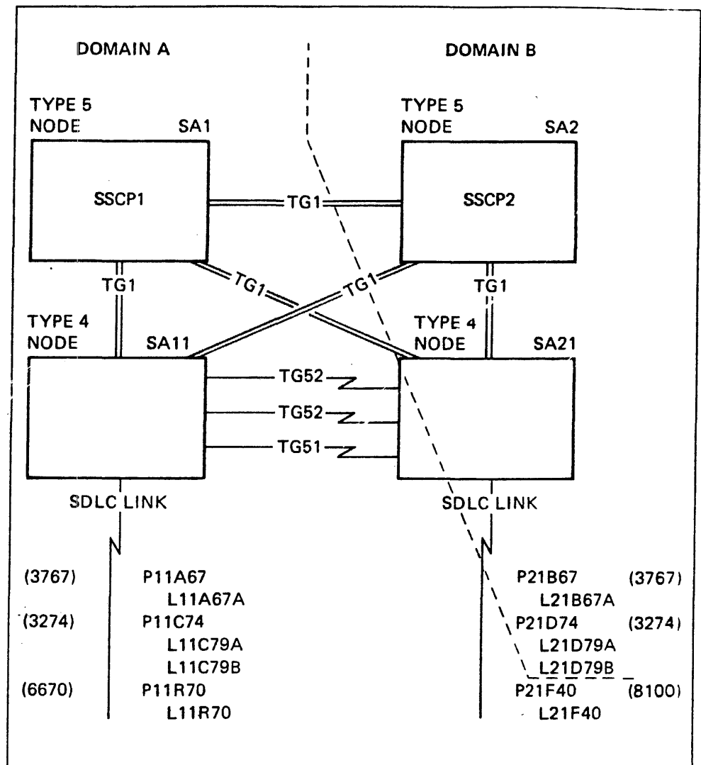
Figure 12-10. Modifying Domains
