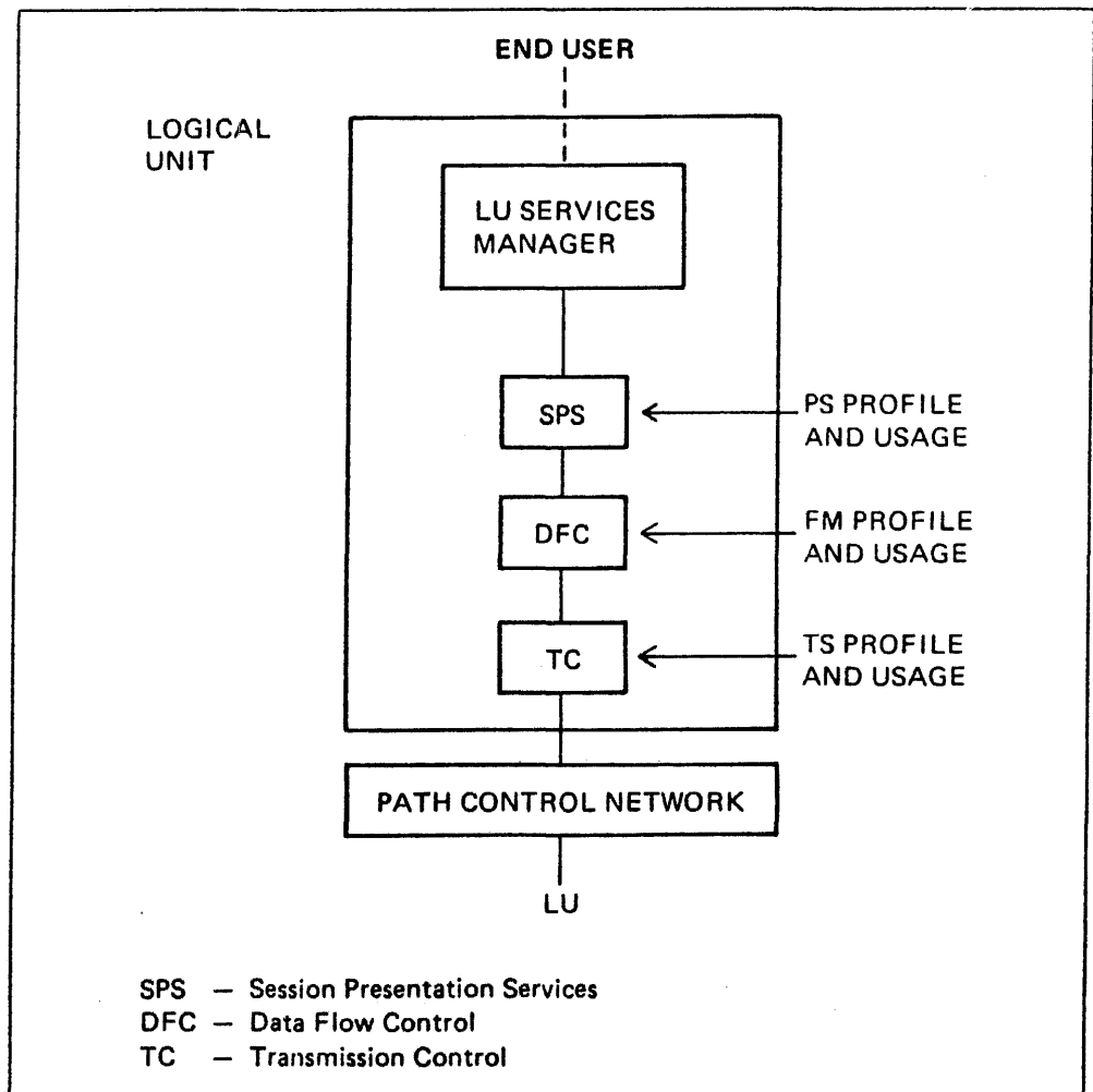
Figure 11-2. BIND Profiles
