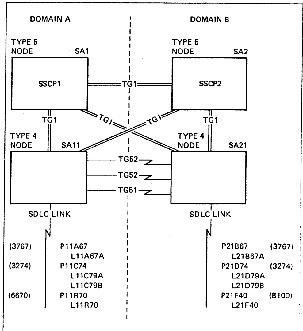
Figure 12-9. Two Domains
