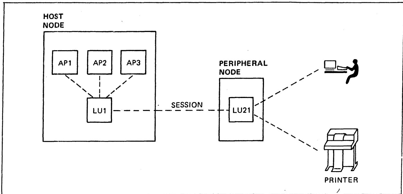
Figure 8-6. Bidding
