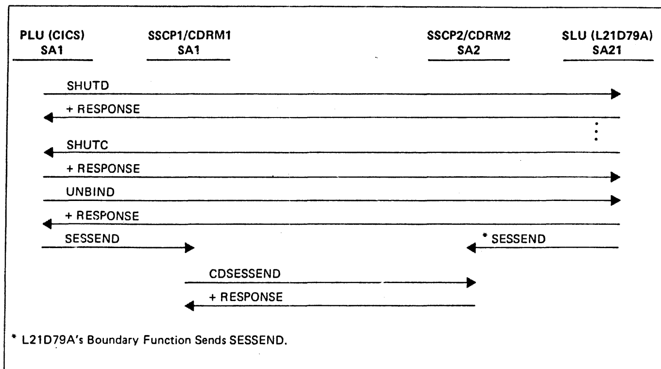
Figure 12-8. Terminating a Cross-Domain LU-LU Session Without SSCP Assistance
