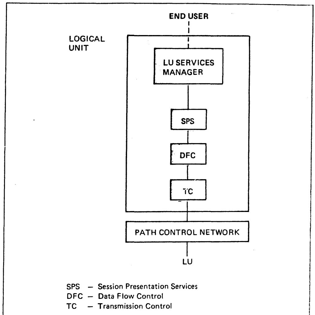
Figure 11-1. Logical Unit Services
