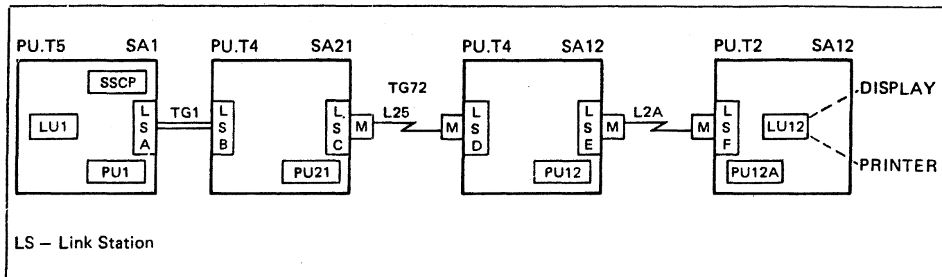
Figure 13-1. Identifying Error Types
