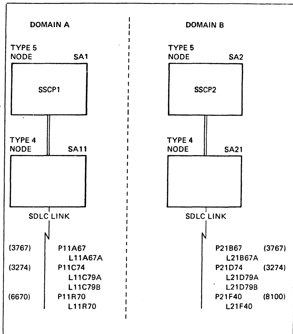
Figure 12-1. SNA Domains
