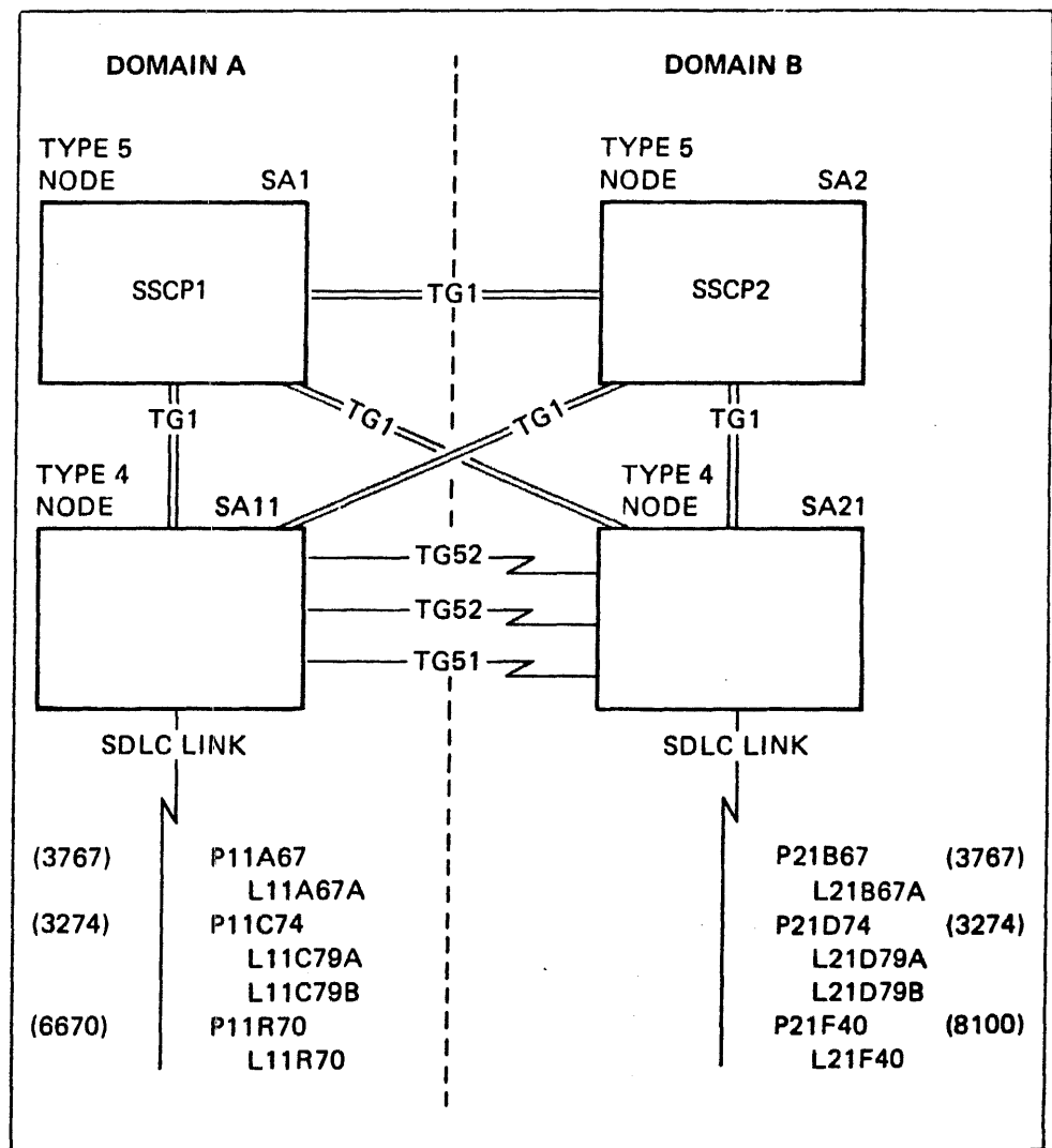
Figure 12-2. Connecting Domains
