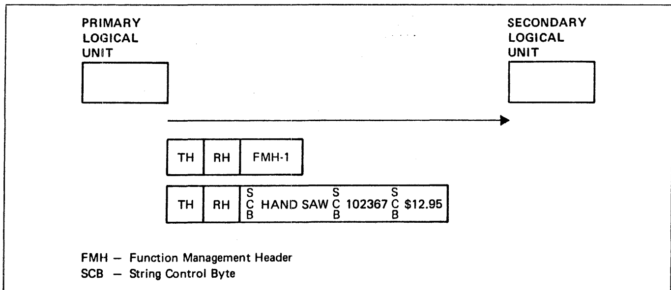
Figure 10-5. Compression
