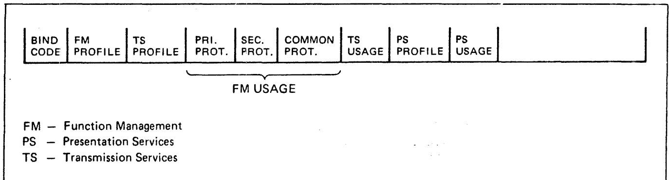
Figure 8-1. BIND Request
