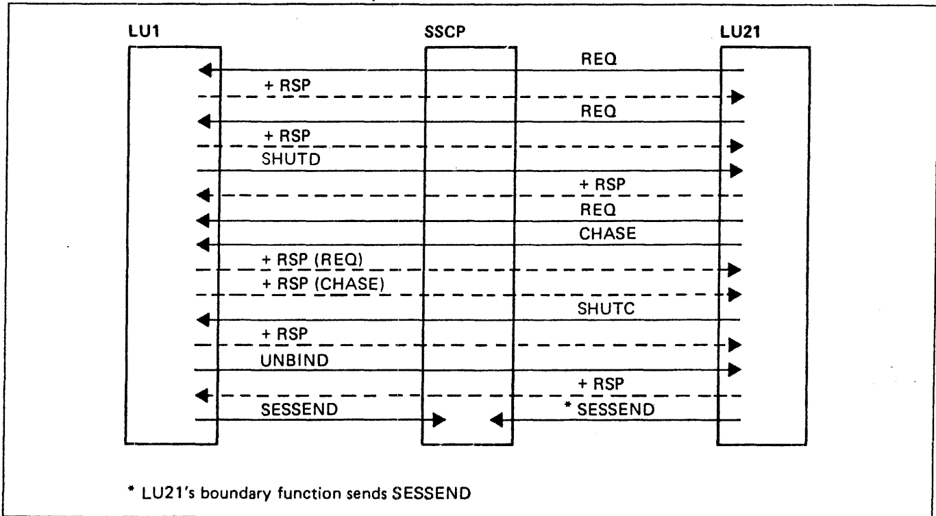
Figure 9-2. Shutdown Protocol
