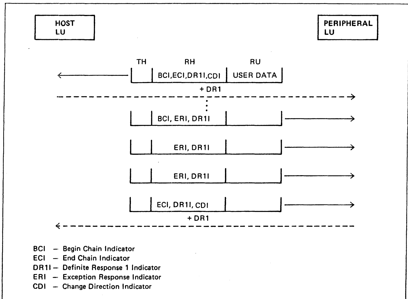
Figure 8-3. Half-Duplex Flip-Flop Mode
