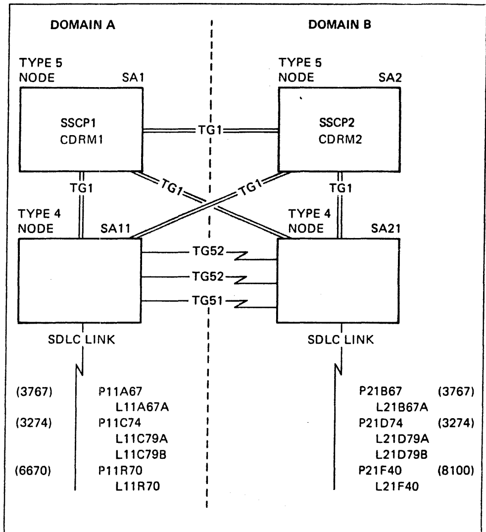
Figure 12-3. Cross-Domain Resource Managers (CDRMs)
