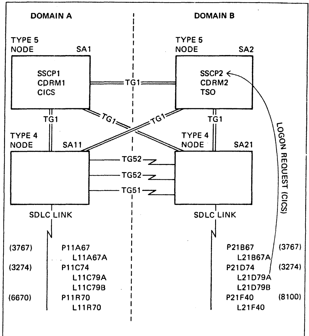
Figure 12-5. Logon Cross Domain
