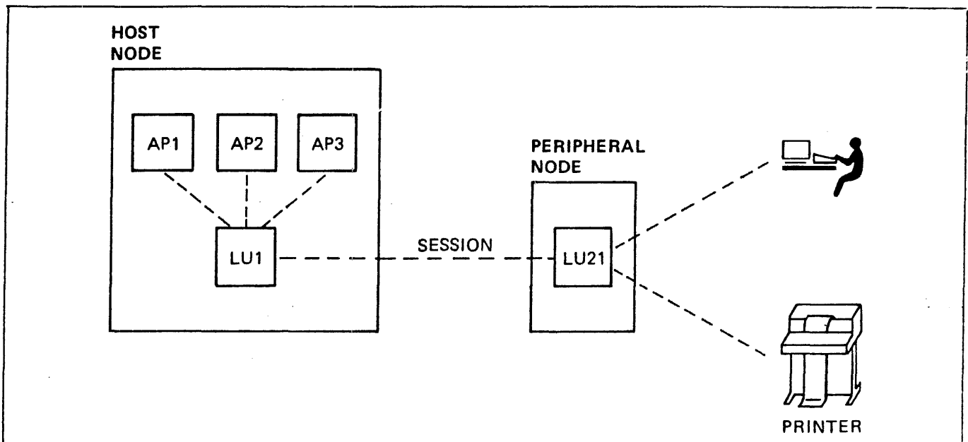
Figure 8-2. Full-Duplex Application
